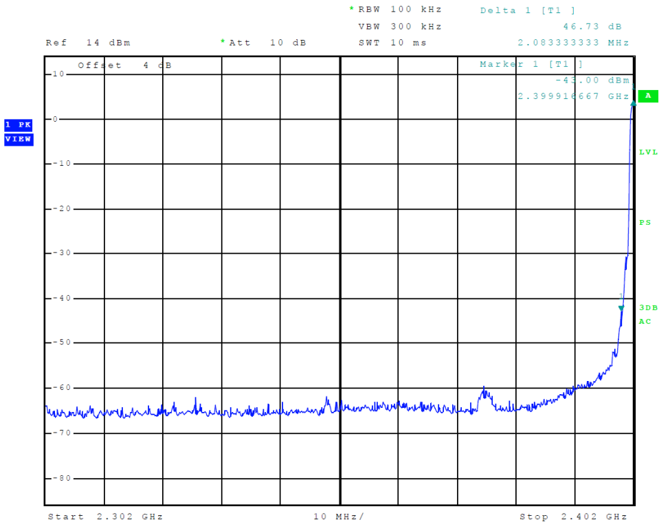
Figure 22 Plot of Transmitter Emissions Low Band Edge Tx 2 (PI/4 DPQSK)
