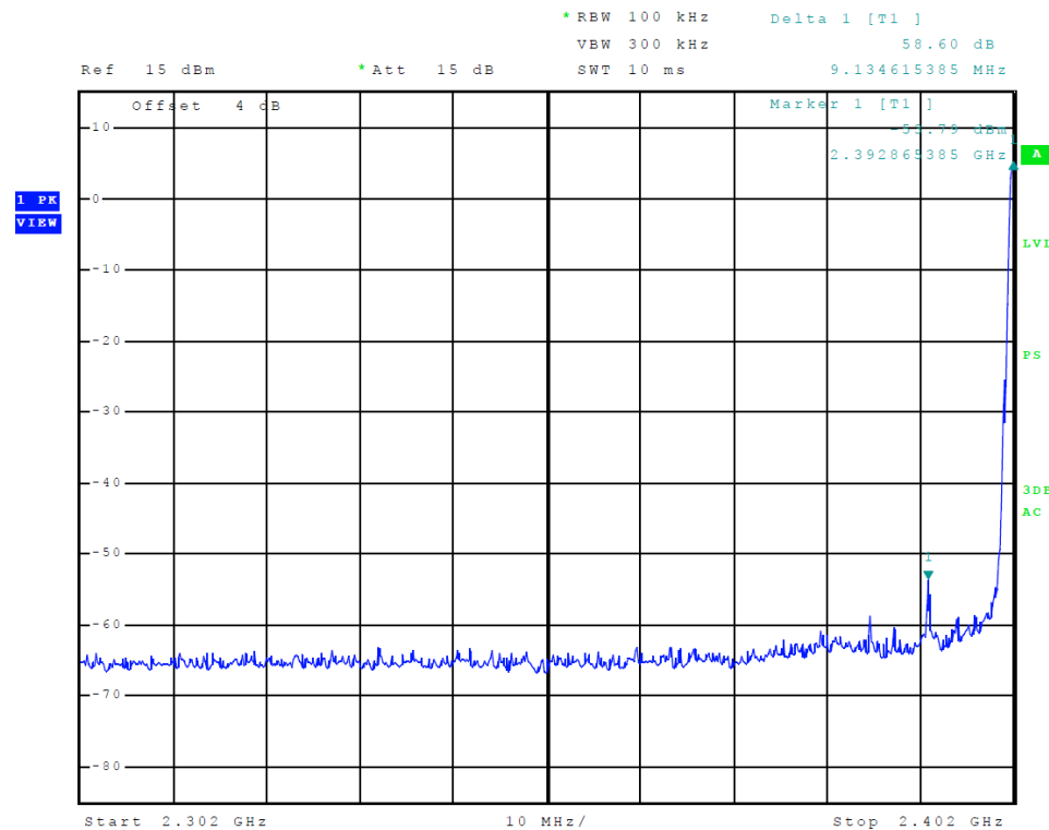
Figure 24 Plot of Transmitter Emissions Low Band Edge Tx 2 (GMSK)
