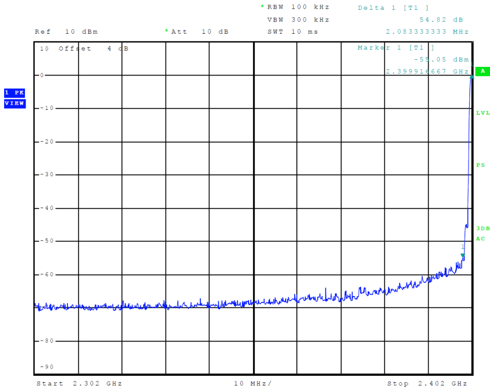
Figure 5 Plot of Transmitter Emissions Low Band Edge Tx 1 (8DPSK)
