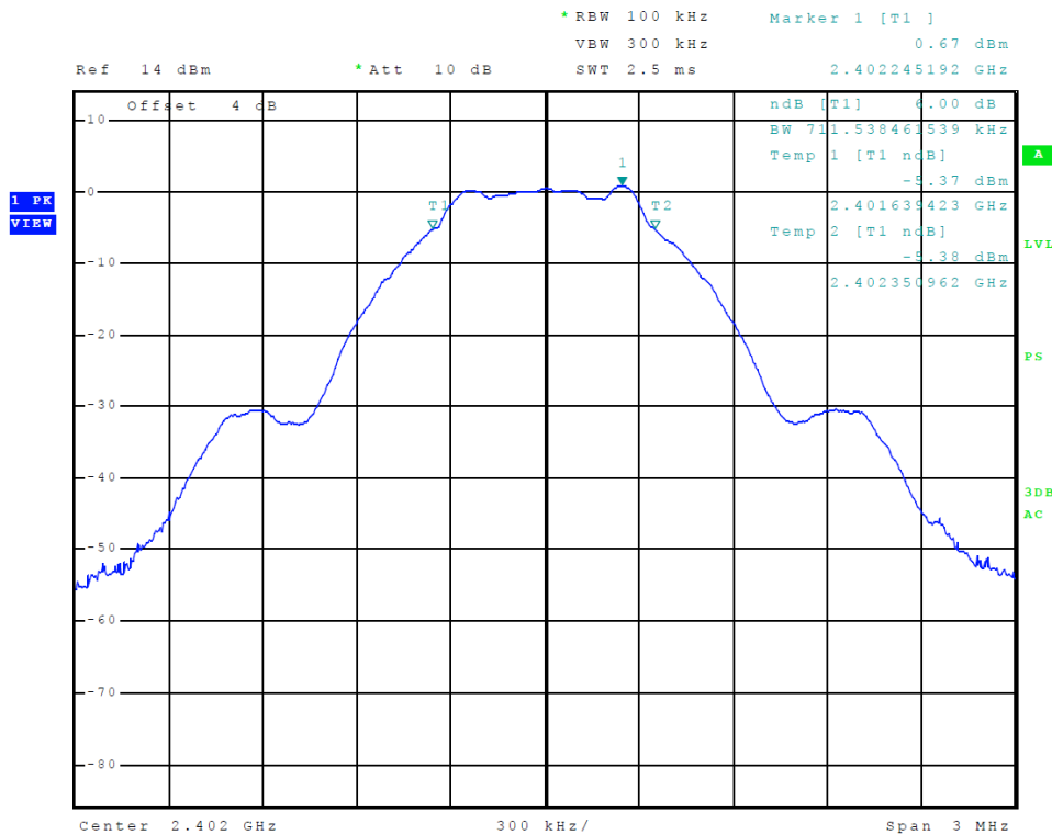
Figure 14 Plot of Transmitter Emissions 6-dB% Occupied Bandwidth Tx 1 (GMSK)
