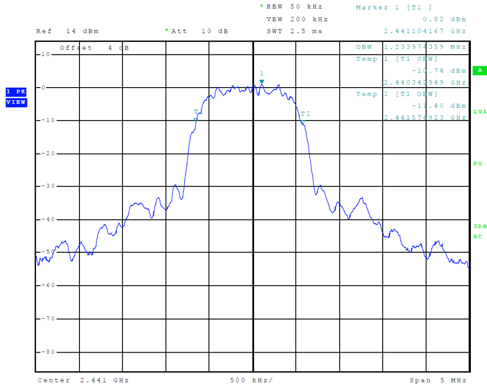
Figure 29 Plot of Transmitter Emissions 99% Occupied Bandwidth Tx 2 (PI/4 DPQSK)
