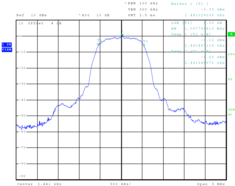
Figure 10 Plot of Transmitter Emissions 6-dB% Occupied Bandwidth Tx 1 (PI/4 DPQSK)
