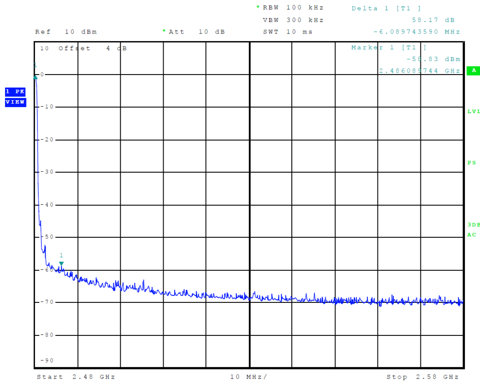
Figure 8 Plot of Transmitter Emissions High Band Edge Tx 1 (8DPSK)
