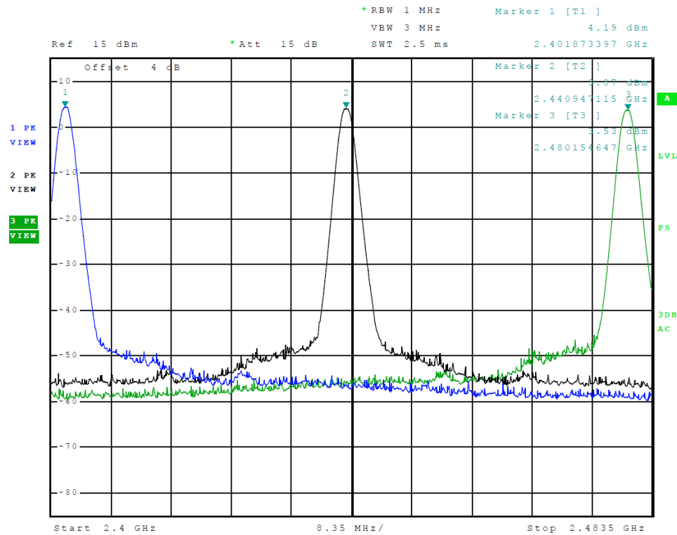
Figure 1 Plot of Transmitter Emissions Operation in 2402-2480 MHz Tx 1 (PI/4 DPQSK)
