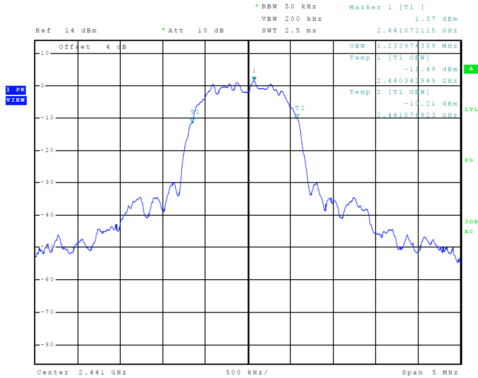
Figure 31 Plot of Transmitter Emissions 99% Occupied Bandwidth Tx 2 (8DPSK)
