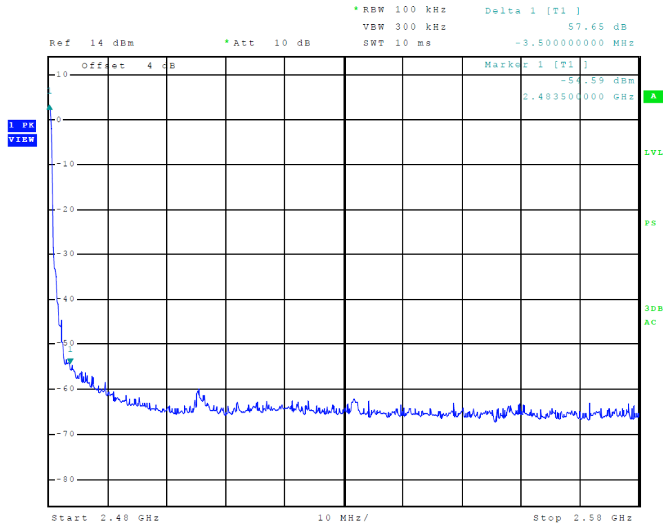
Figure 25 Plot of Transmitter Emissions High Band Edge Tx 2 (PI/4 DPQSK)
