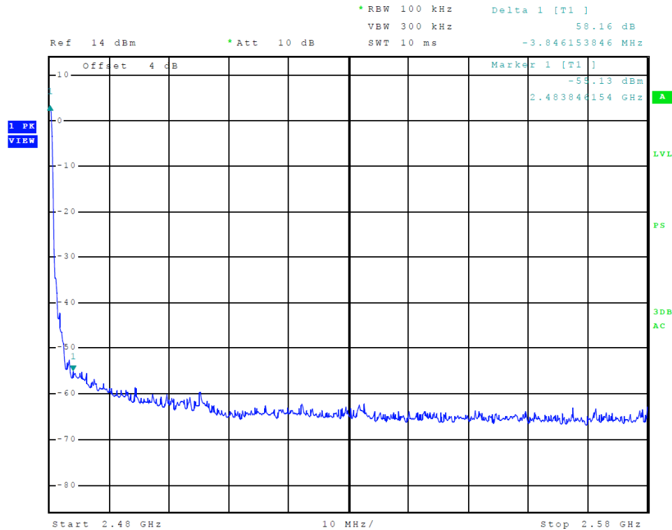
Figure 26 Plot of Transmitter Emissions High Band Edge Tx 2 (8DPSK)
