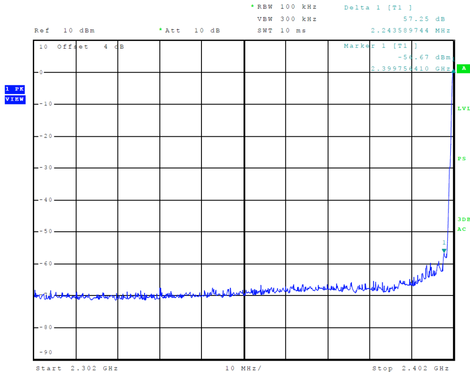
Figure 6 Plot of Transmitter Emissions Low Band Edge Tx 1 (GMSK)
