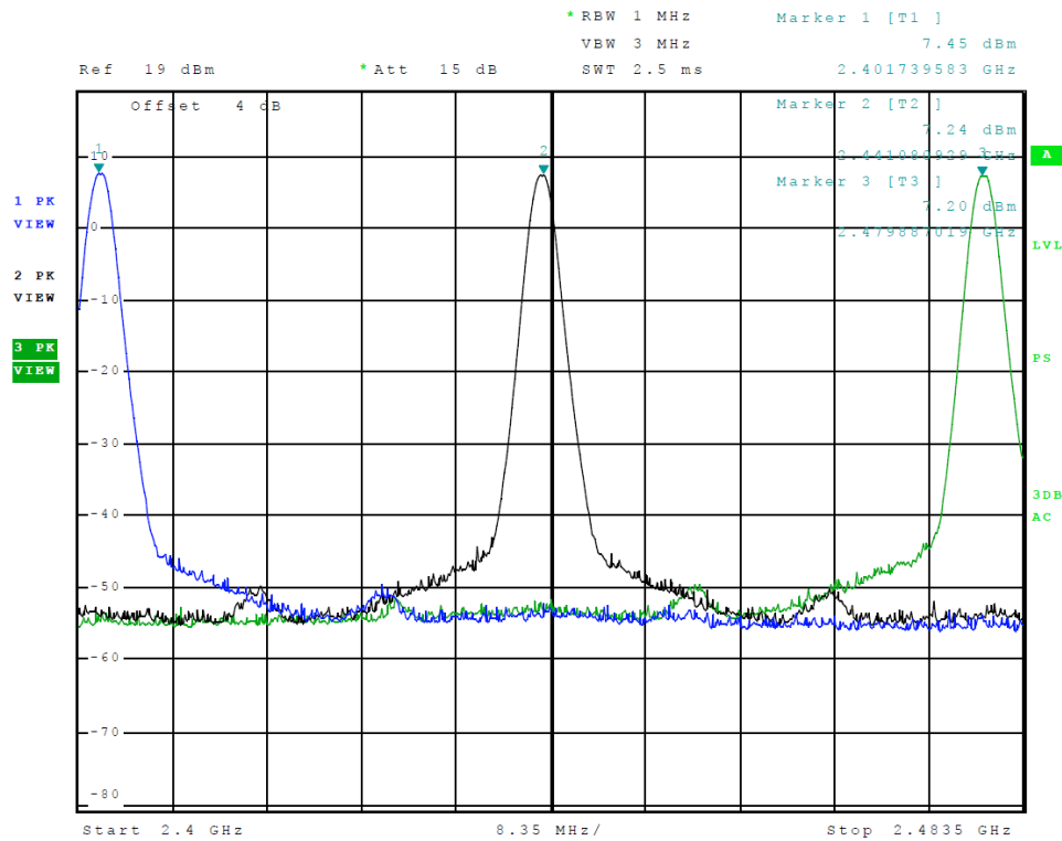
Figure 19 Plot of Transmitter Emissions Operation in 2402-2480 MHz Tx 2 (PI/4 DPQSK)
