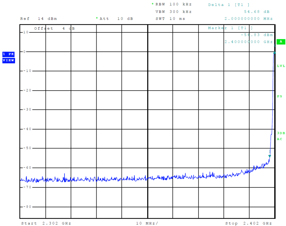
Figure 4 Plot of Transmitter Emissions Low Band Edge Tx 1 (PI/4 DPQSK)
