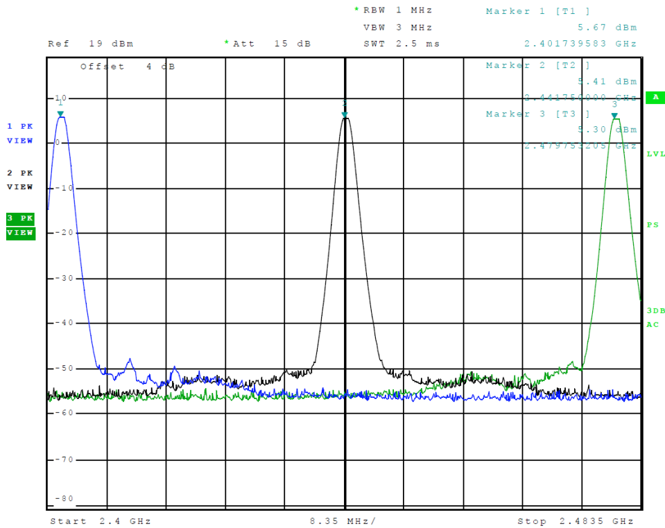
Figure 21 Plot of Transmitter Emissions Operation in 2402-2480 MHz Tx 2 (GMSK)
