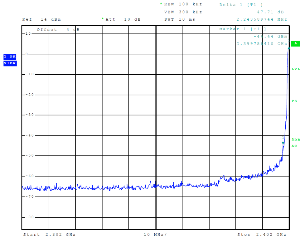
Figure 23 Plot of Transmitter Emissions Low Band Edge Tx 2 (8DPSK)
