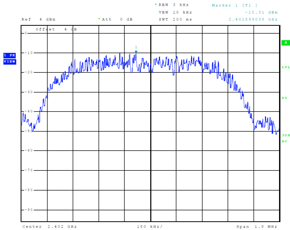
Figure 35 Plot of Transmitter Power Spectral Density Tx 2 (8DPSK)
