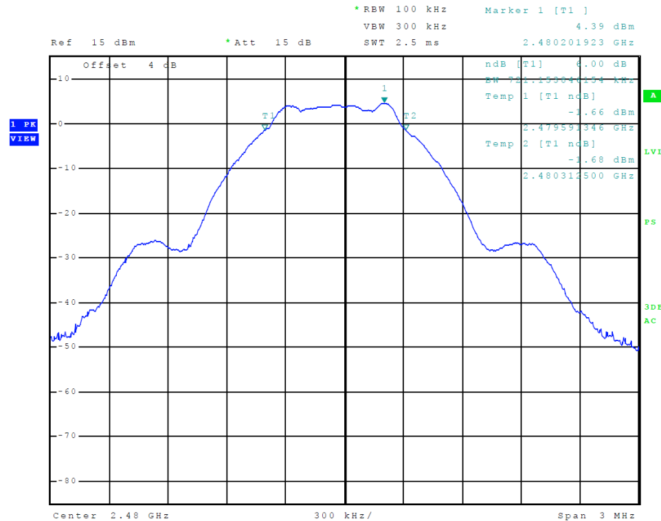
Figure 32 Plot of Transmitter Emissions 6-dB% Occupied Bandwidth Tx 2 (GMSK)
