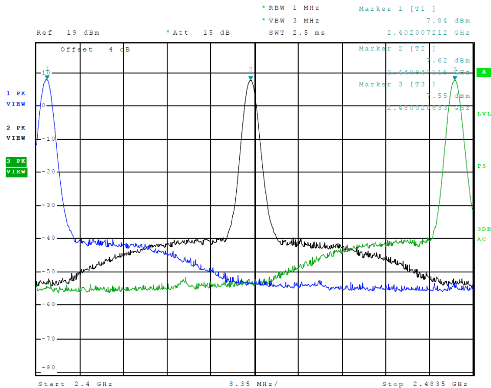
Figure 20 Plot of Transmitter Emissions Operation in 2402-2480 MHz Tx 2 (8DPSK)
