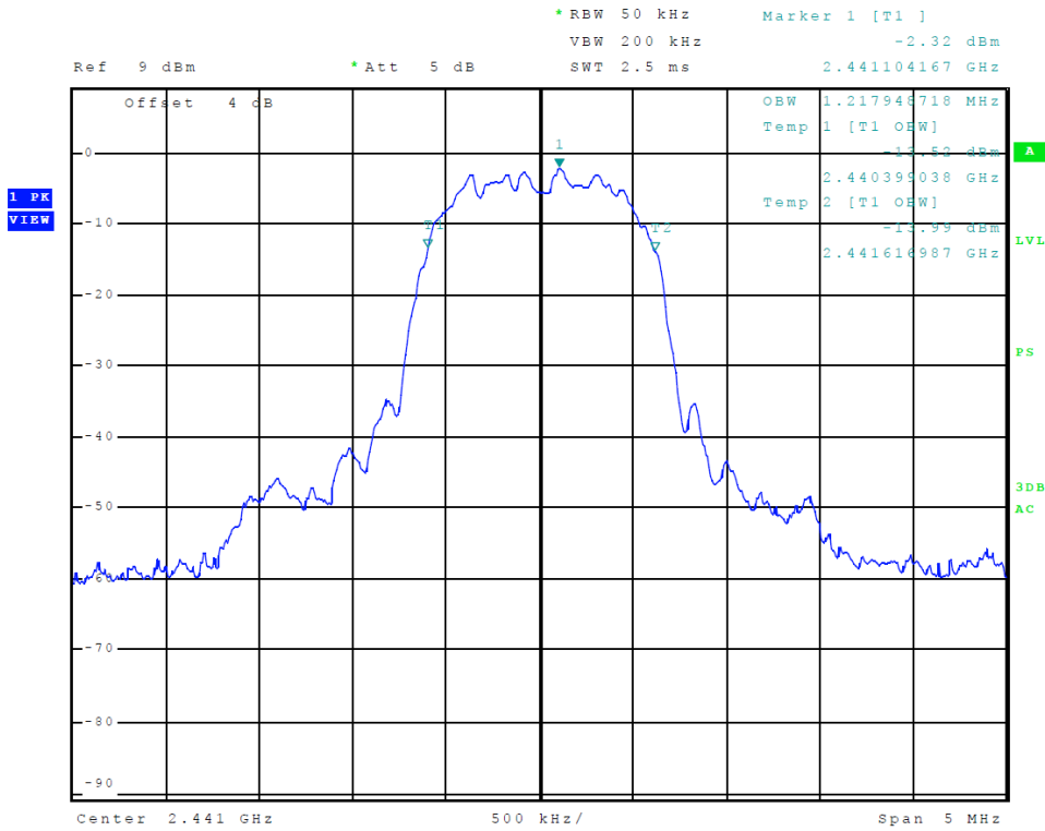
Figure 13 Plot of Transmitter Emissions 99% Occupied Bandwidth Tx 1 (8DPSK)
