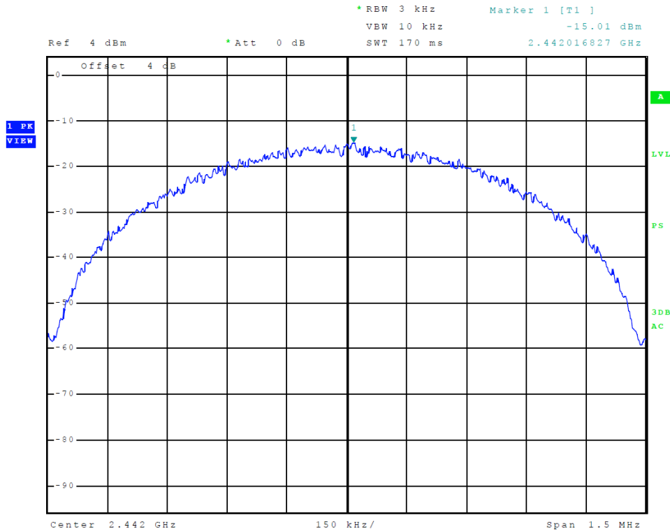
Figure 18 Plot of Transmitter Power Spectral Density Tx 2 (GMSK)
