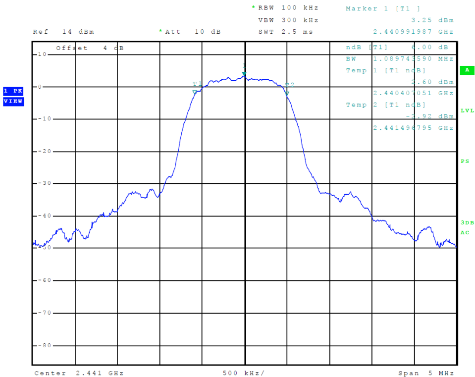
Figure 28 Plot of Transmitter Emissions 6-dB% Occupied Bandwidth Tx 2 (PI/4 DPQSK)
