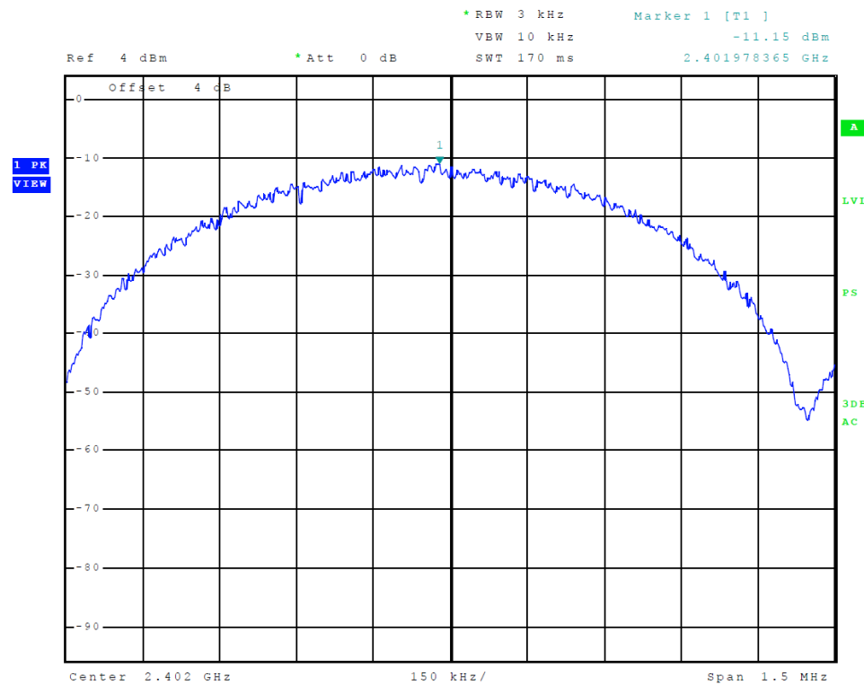
Figure 36 Plot of Transmitter Power Spectral Density Tx 2 (GMSK)
