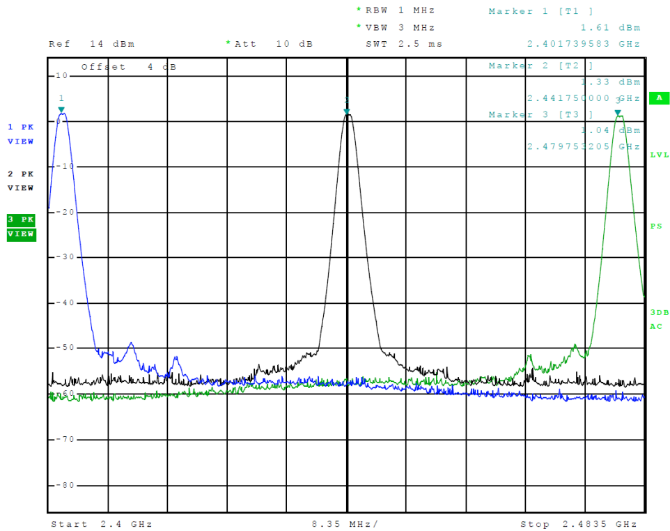
Figure 3 Plot of Transmitter Emissions Operation in 2402-2480 MHz Tx 1 (GMSK)
