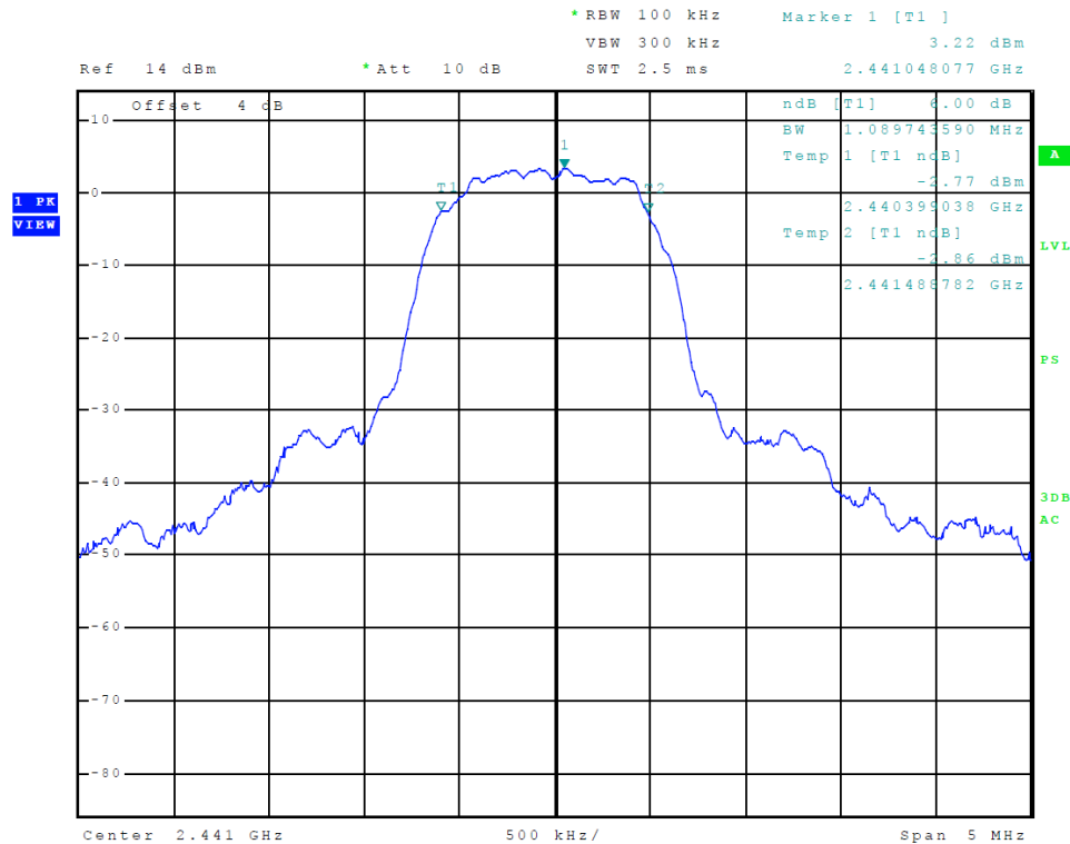
Figure 30 Plot of Transmitter Emissions 6-dB% Occupied Bandwidth Tx 2 (8DPSK)
