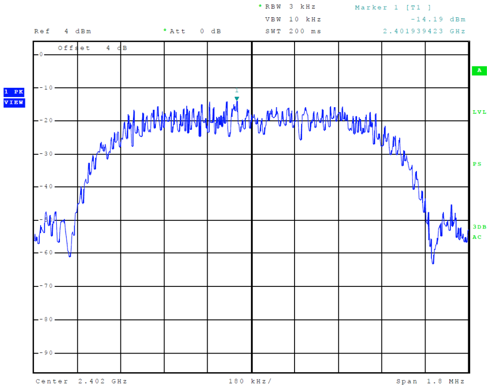
Figure 17 Plot of Transmitter Power Spectral Density Tx 1 (8DPSK)
