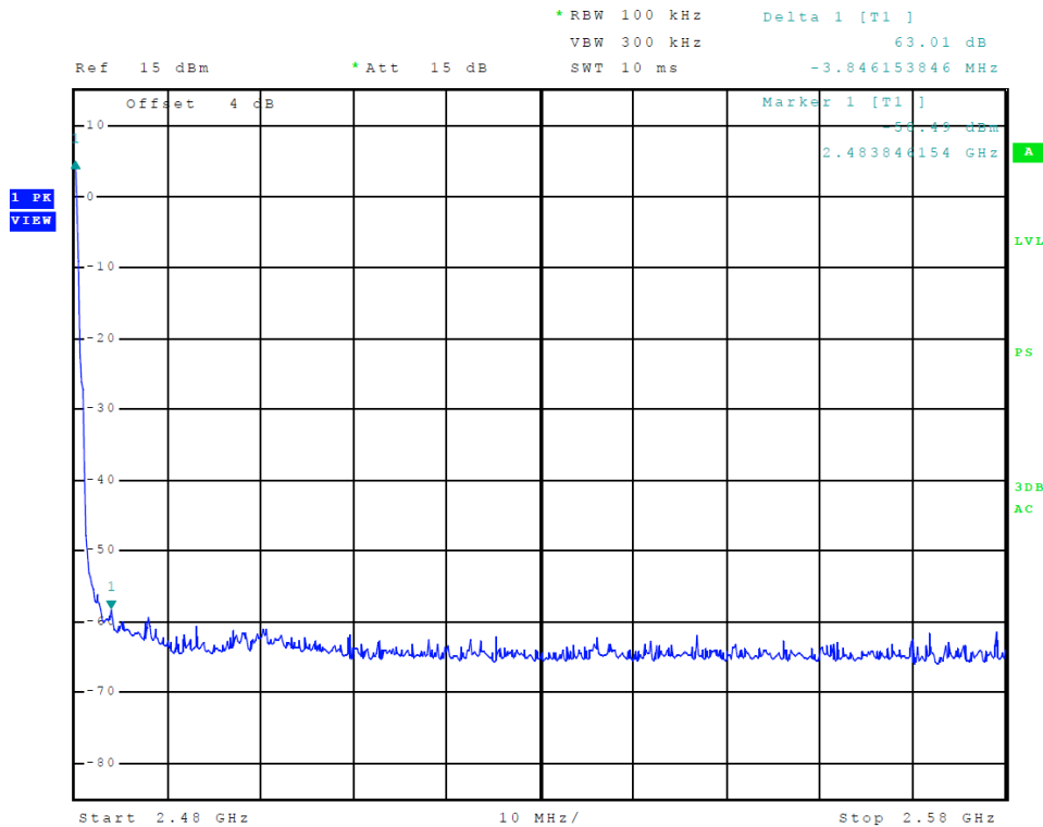
Figure 27 Plot of Transmitter Emissions High Band Edge Tx 2 (GMSK)
