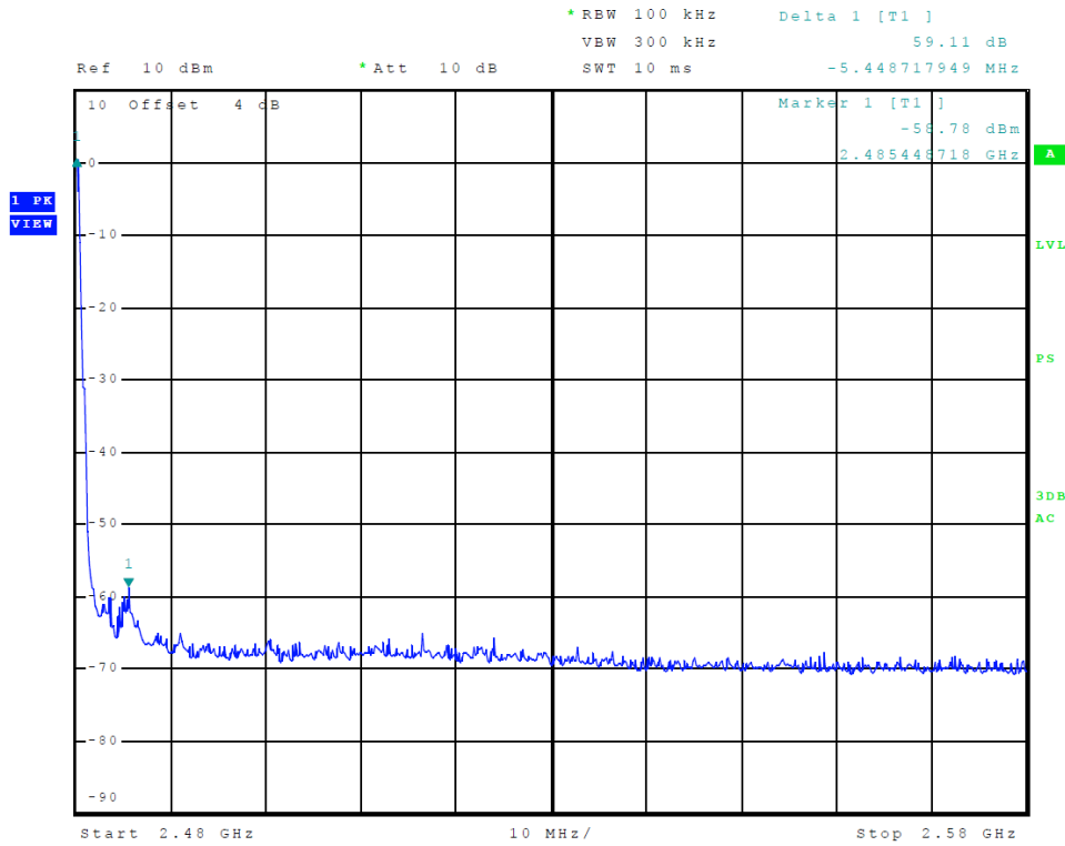
Figure 9 Plot of Transmitter Emissions High Band Edge Tx 1 (GMSK)
