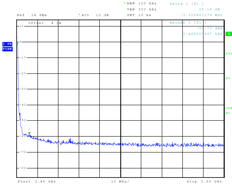
Figure 7 Plot of Transmitter Emissions High Band Edge Tx 1 (PI/4 DPQSK)
