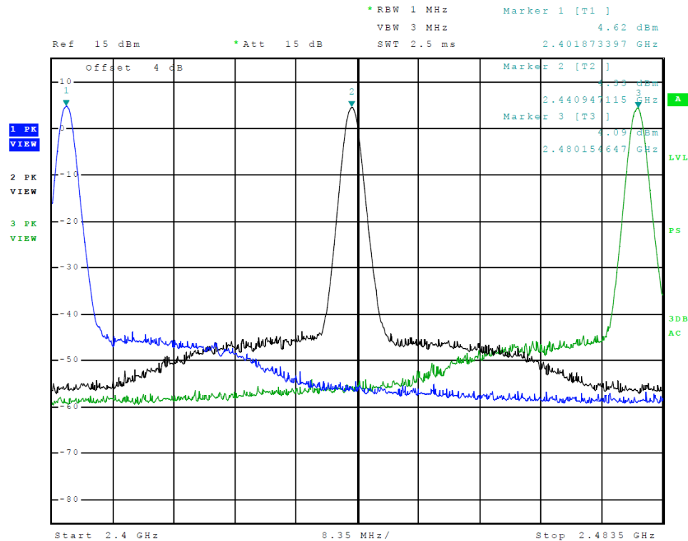
Figure 2 Plot of Transmitter Emissions Operation in 2402-2480 MHz Tx 1 (8DPSK)
