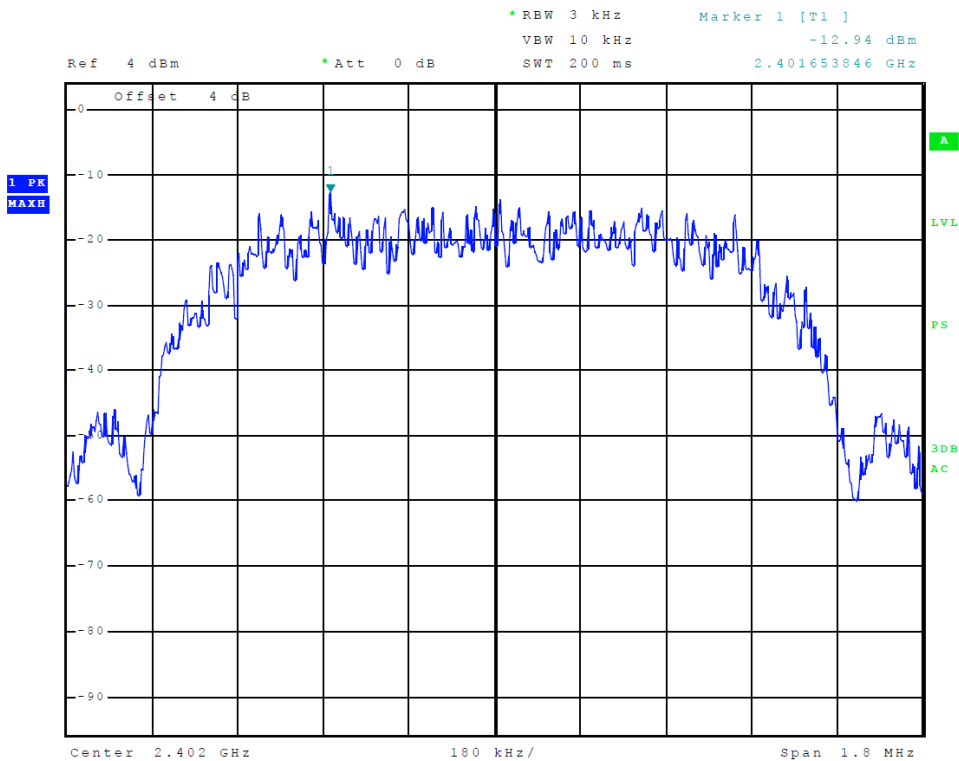
Figure 16 Plot of Transmitter Power Spectral Density Tx 1 (PI/4 DPQSK)
