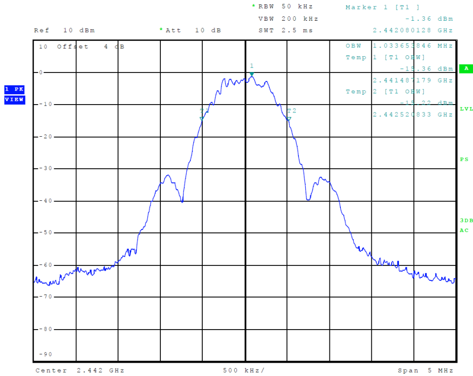
Figure 15 Plot of Transmitter Emissions 99% Occupied Bandwidth Tx 1 (GMSK)
