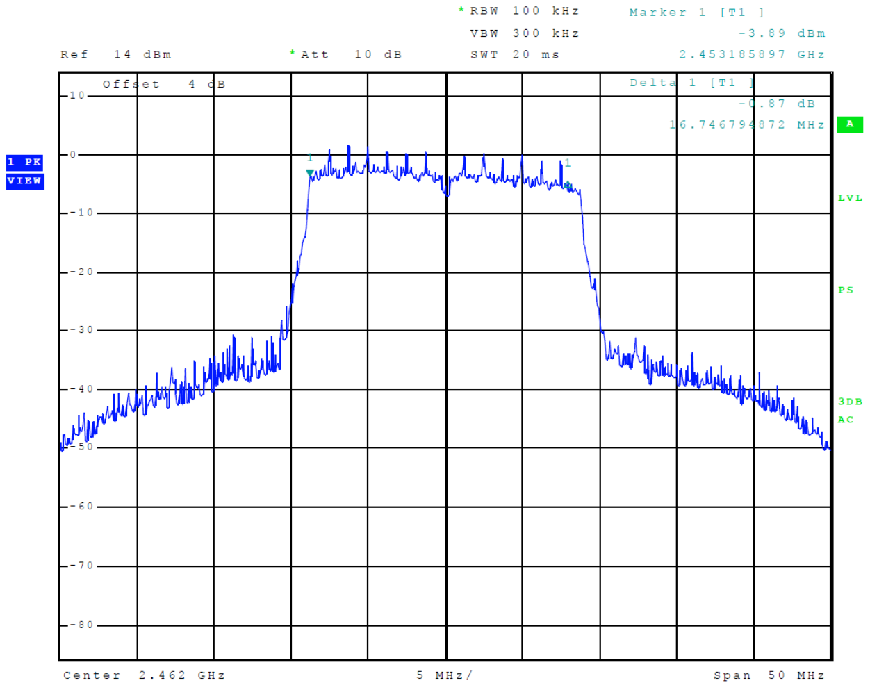
Figure 18 Plot of 6-dB Occupied Bandwidth Mode 7 (MCS)
