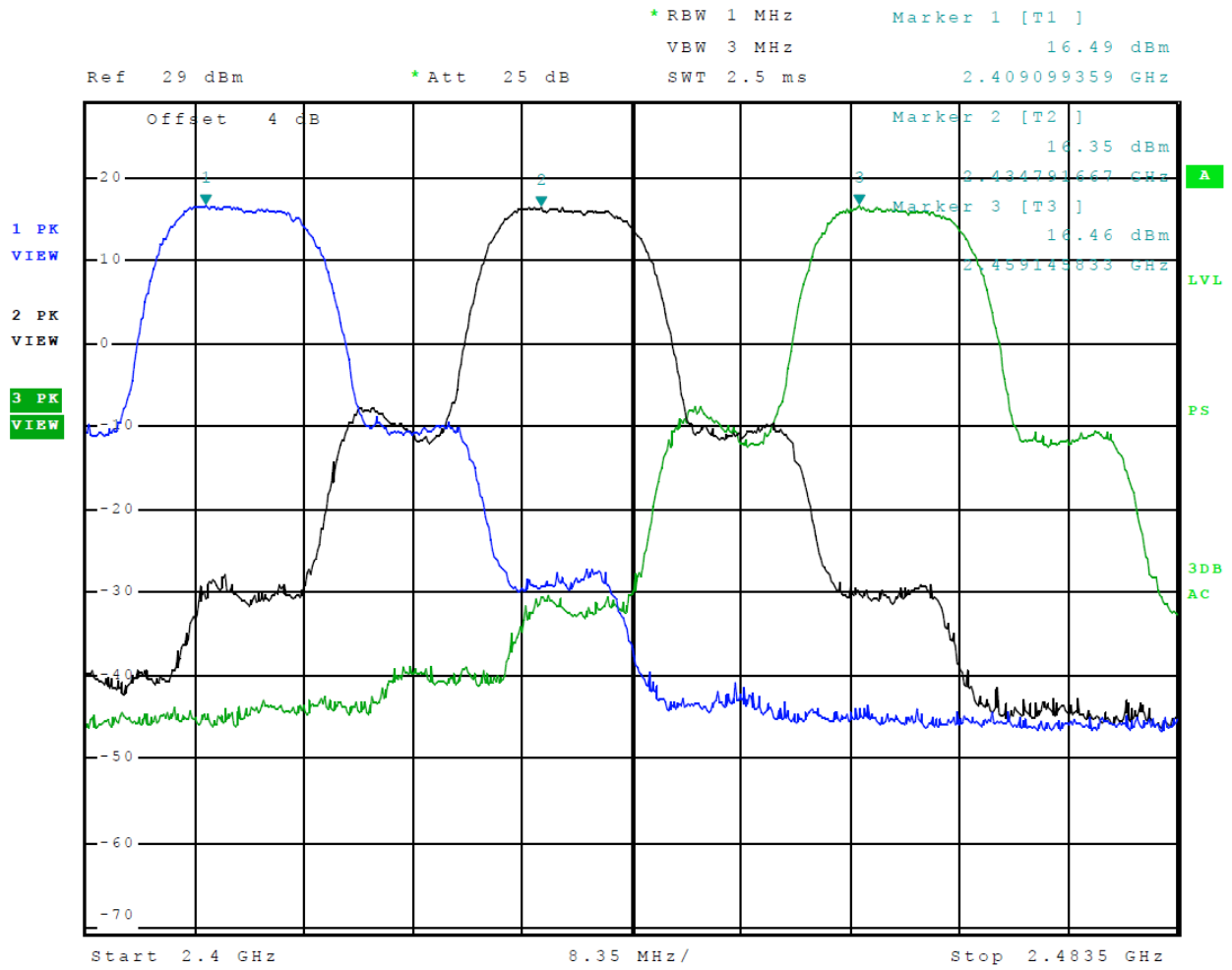
Figure 5 Plot of Transmitter Operation in 2412-2462 MHz Mode 5 (DSSS)
