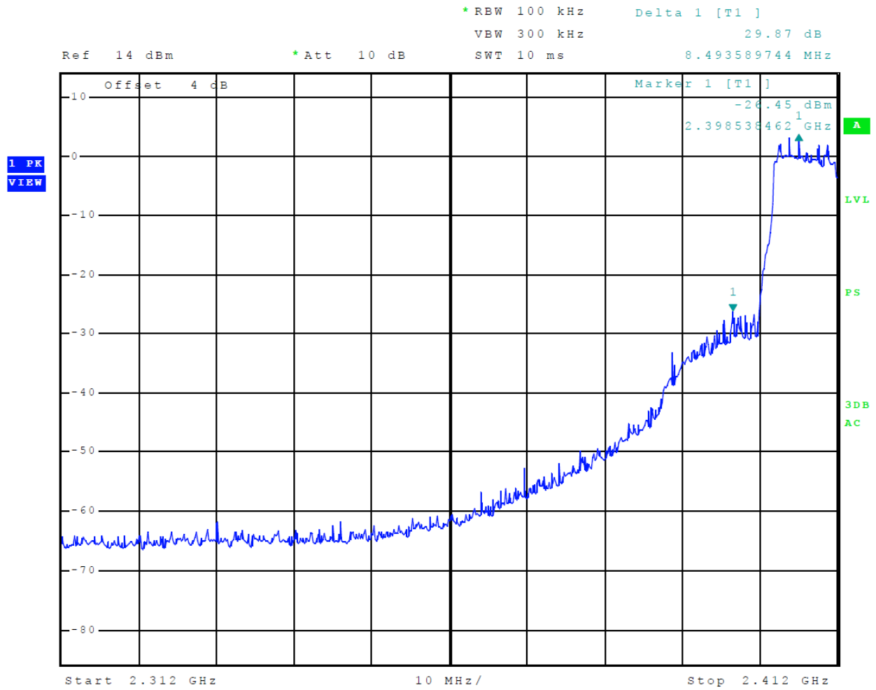
Figure 9 Plot of Transmitter Emissions Low Band Edge Mode 6 (OFDM)
