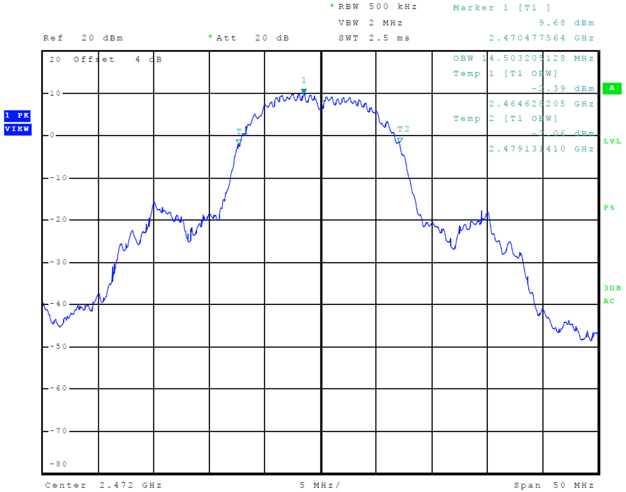
Figure 15 Plot of 99% Occupied Bandwidth Mode 5 (DSSS)
