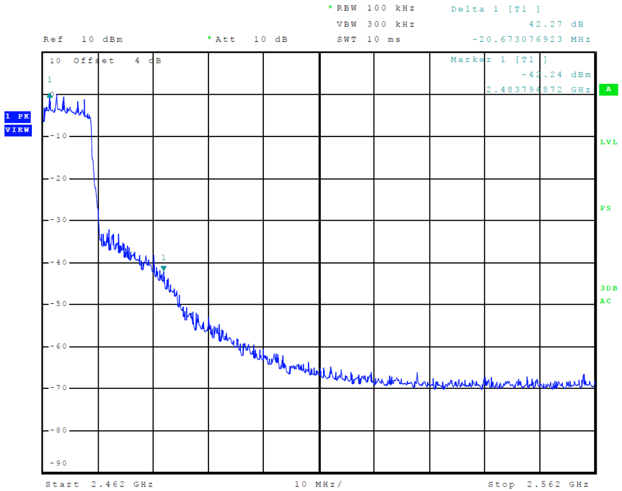
Figure 13 Plot of Transmitter Emissions High Band Edge Mode 7 (MCS)
