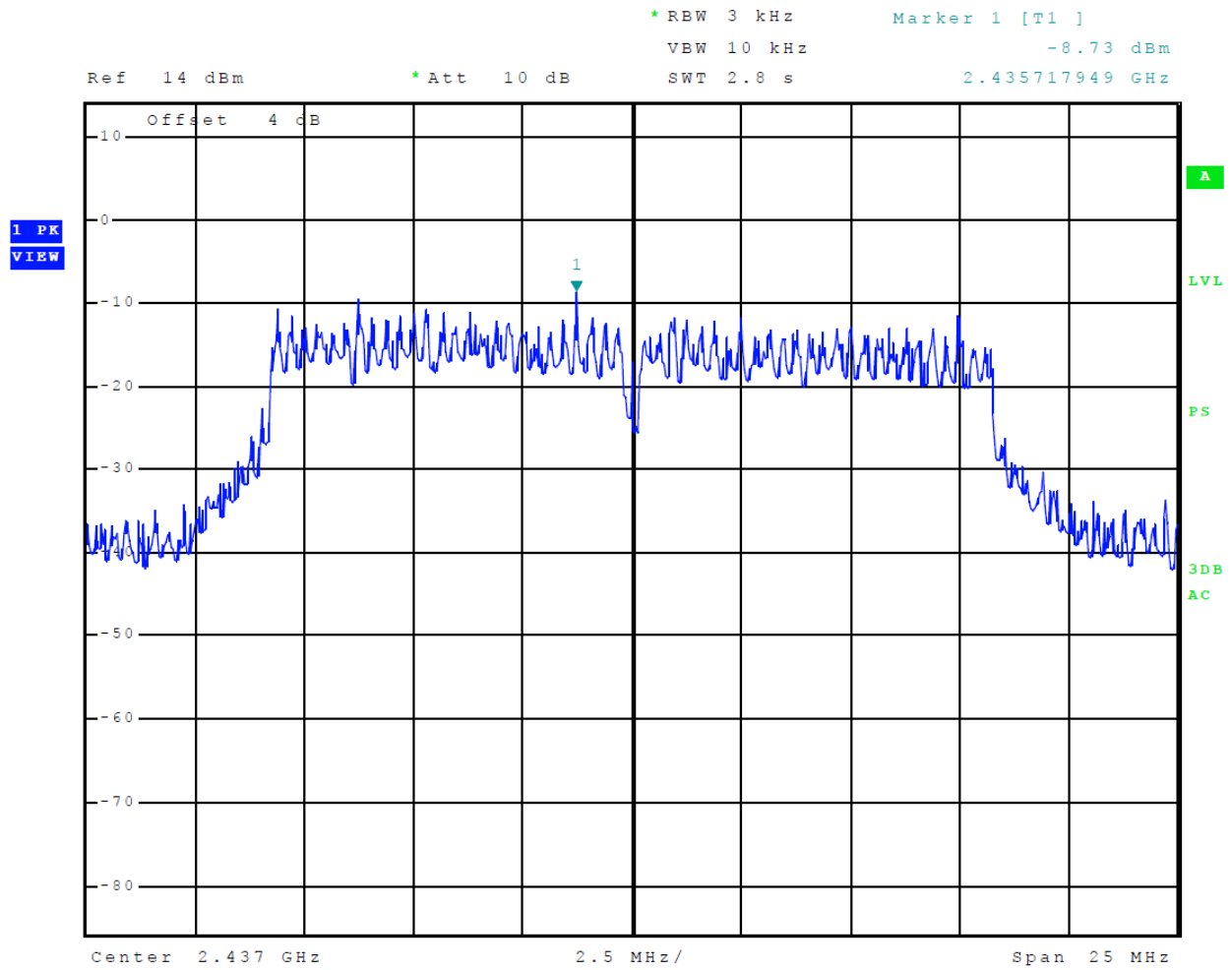
Figure 21 Plot of Transmitter Power Spectral Density Mode 6 (OFDM)
