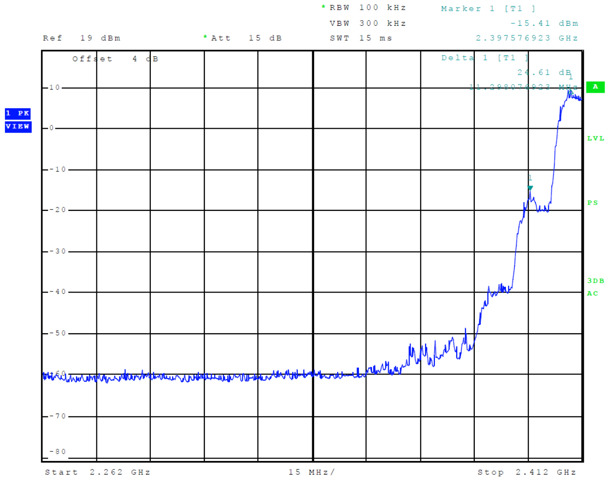
Figure 8 Plot of Transmitter Emissions Low Band Edge Mode 5 (DSSS)
