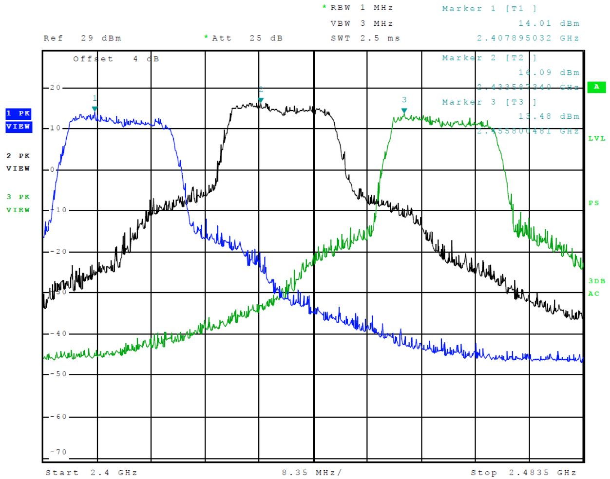
Figure 6 Plot of Transmitter Operation in 2412-2462 MHz Mode 6 (OFDM)
