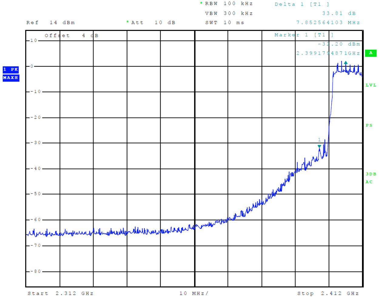
Figure 10 Plot of Transmitter Emissions Low Band Edge Mode 7 (MCS)
