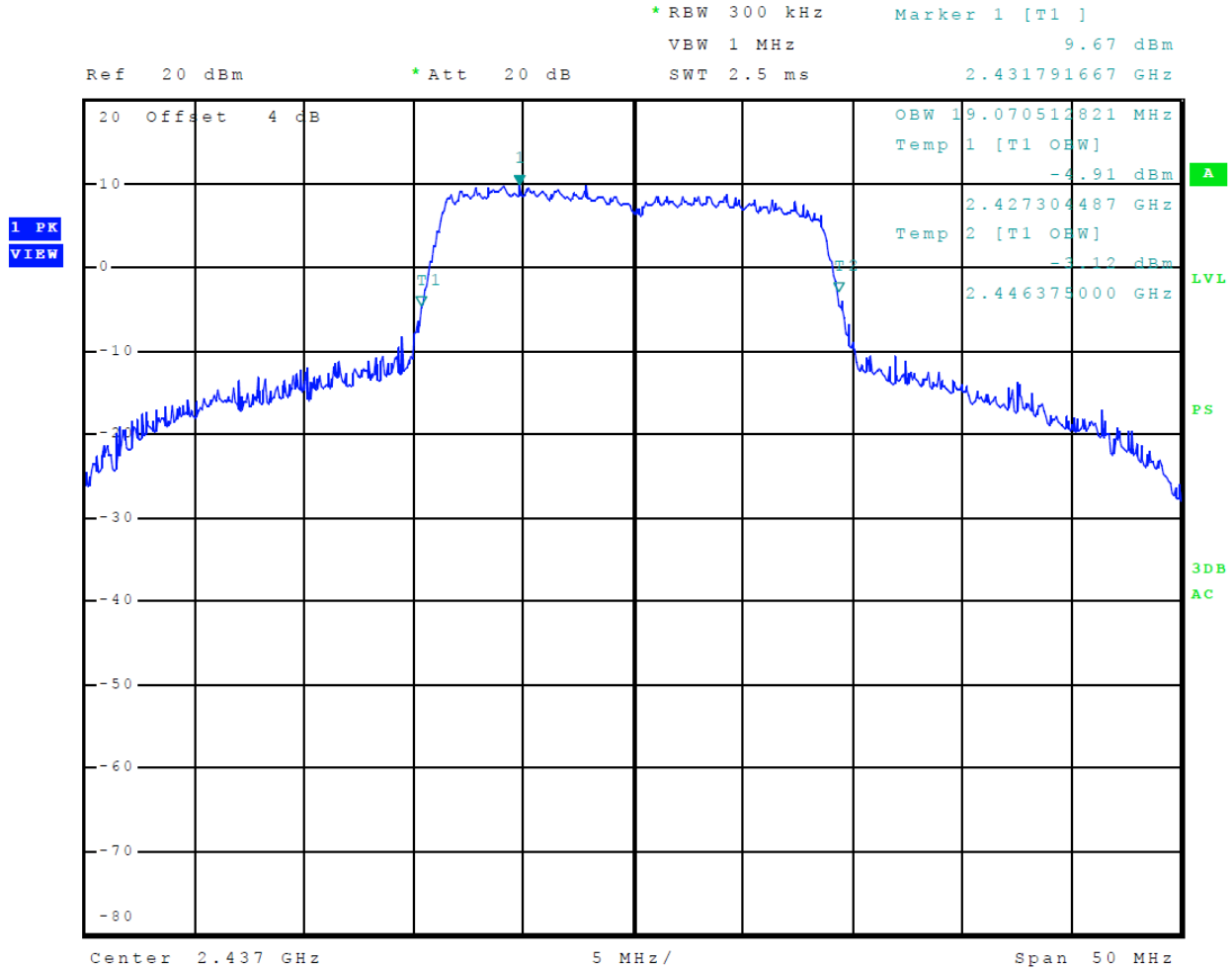
Figure 19 Plot of 99% Occupied Bandwidth Mode 7 (MCS)
