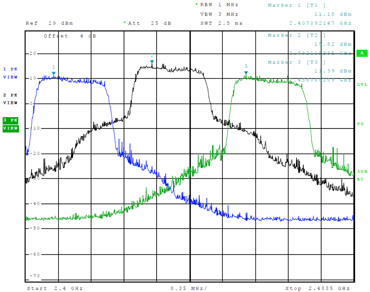
Figure 7 Plot of Transmitter Operation in 2412-2462 MHz Mode 7 (MCS)
