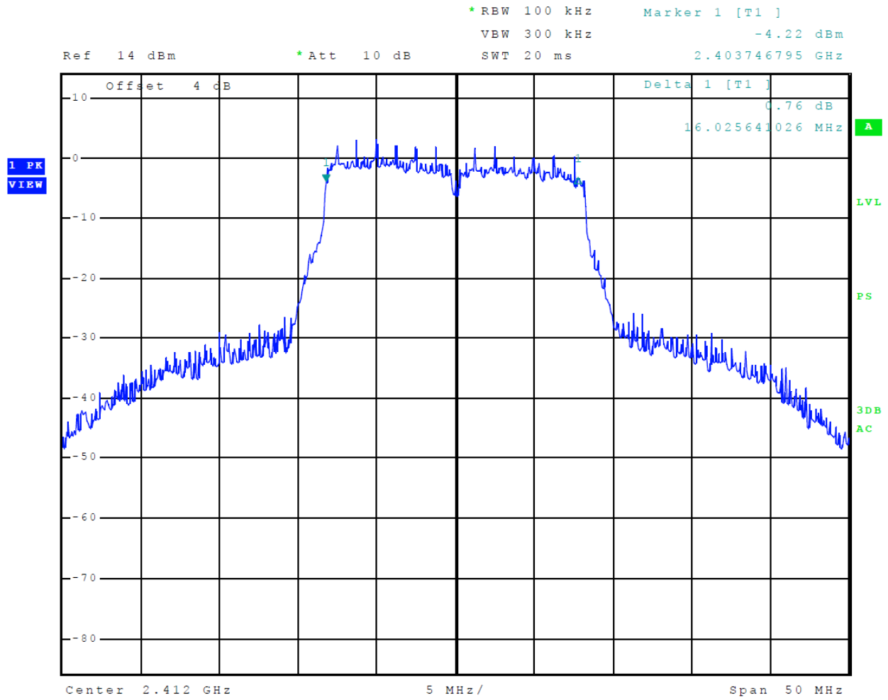
Figure 16 Plot of 6-dB Occupied Bandwidth Mode 6 (OFDM)
