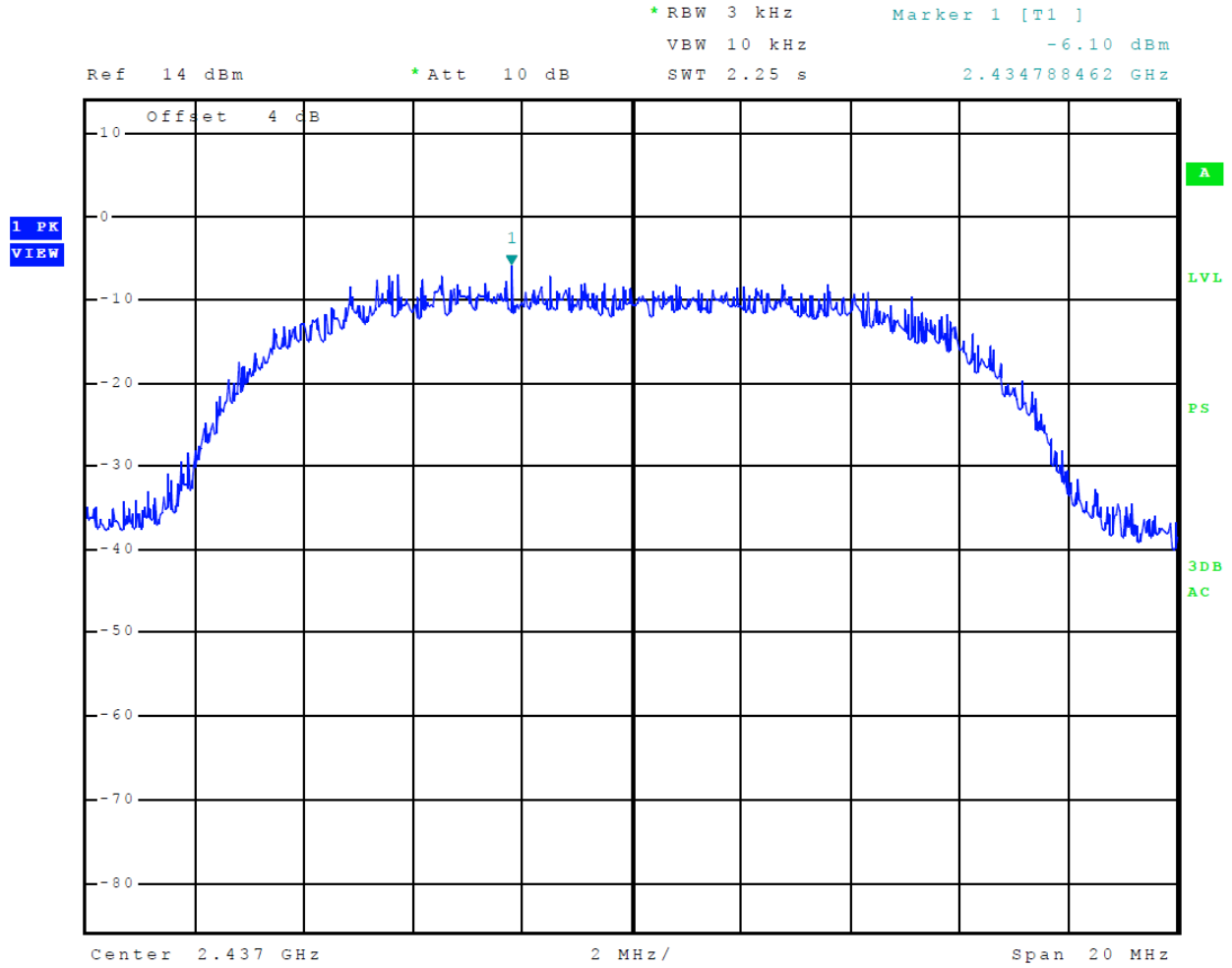
Figure 20 Plot of Transmitter Power Spectral Density Mode 5 (DSSS)
