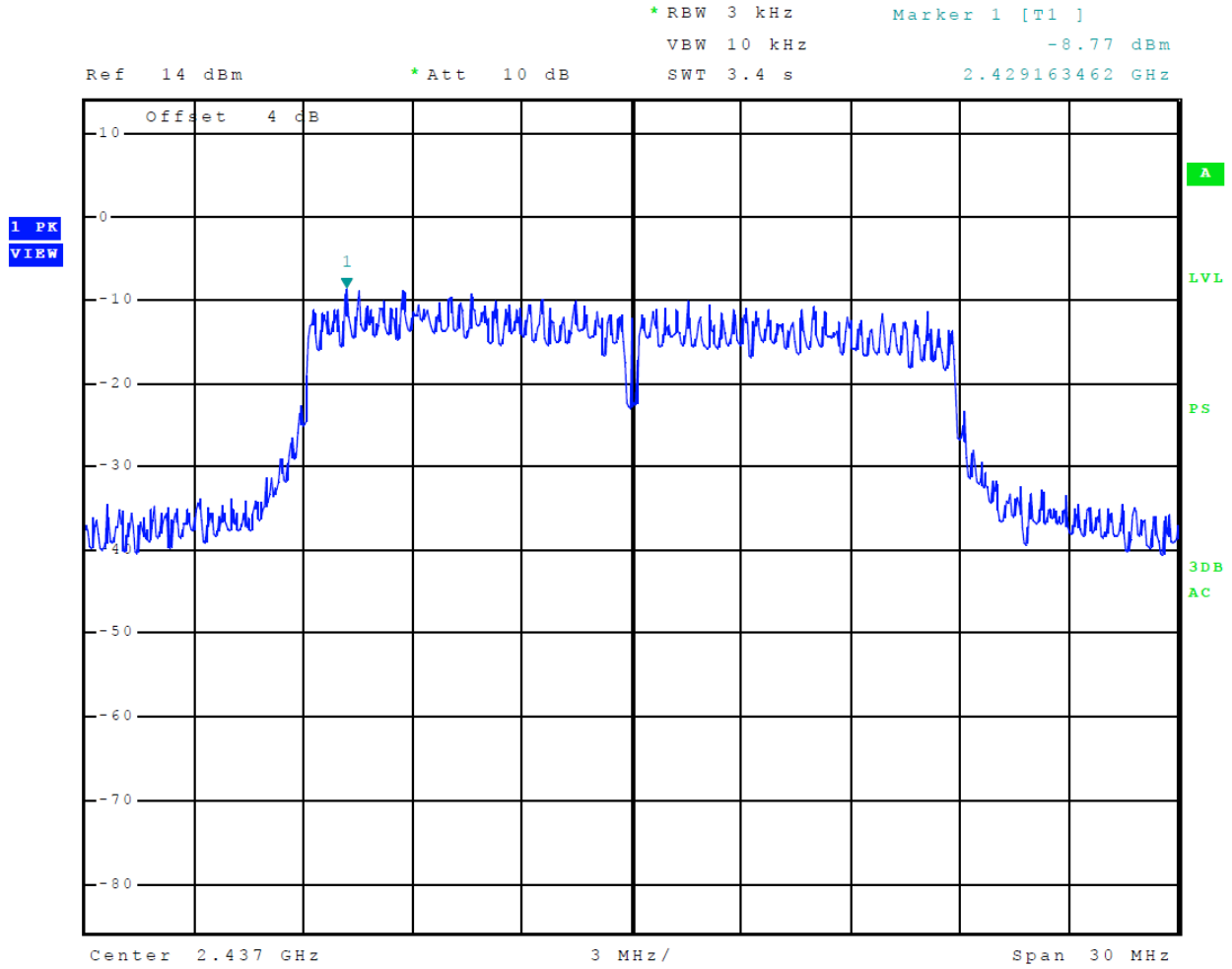
Figure 22 Plot of Transmitter Power Spectral Density Mode 7 (MCS)
