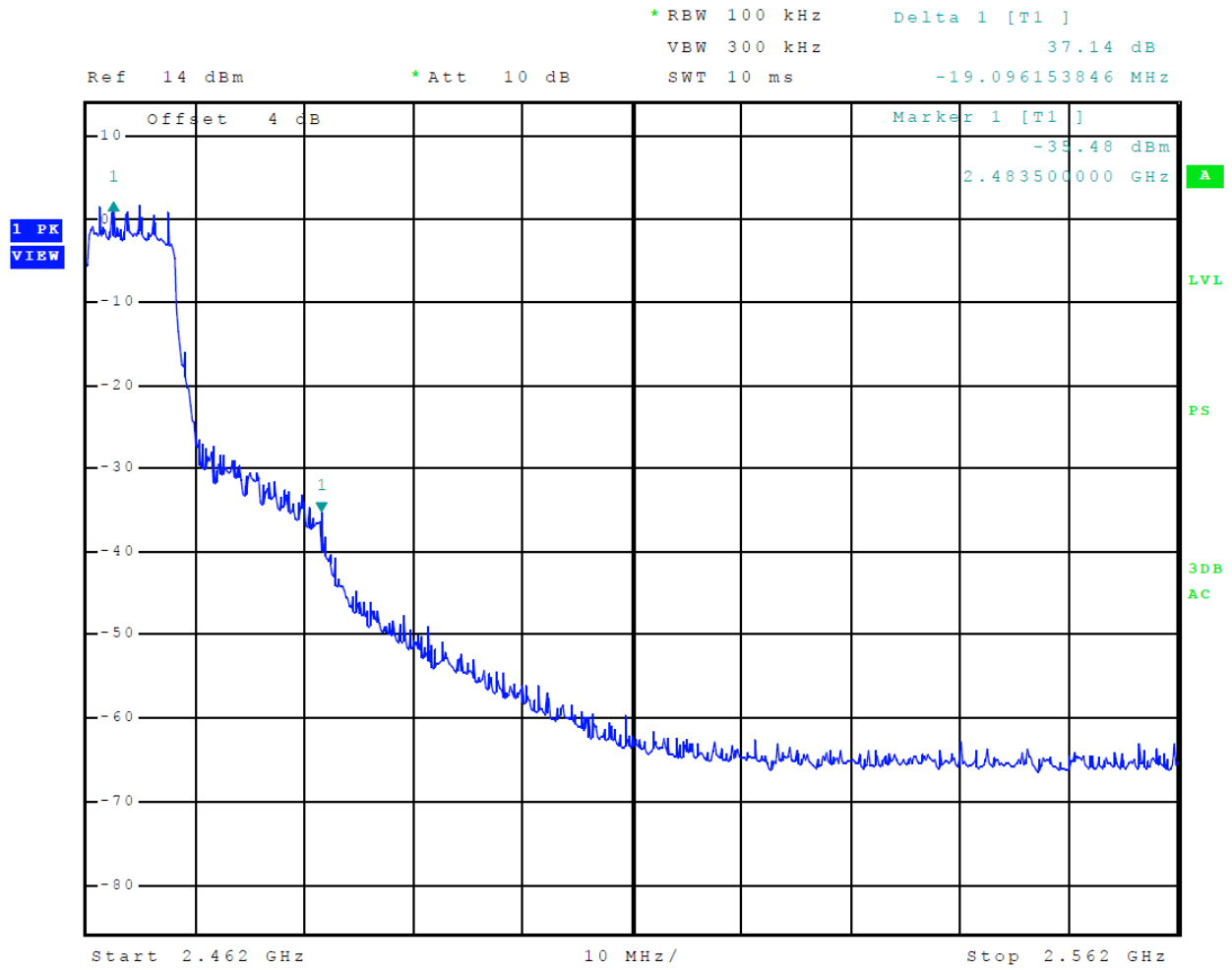
Figure 12 Plot of Transmitter Emissions High Band Edge Mode 6 (OFDM)
