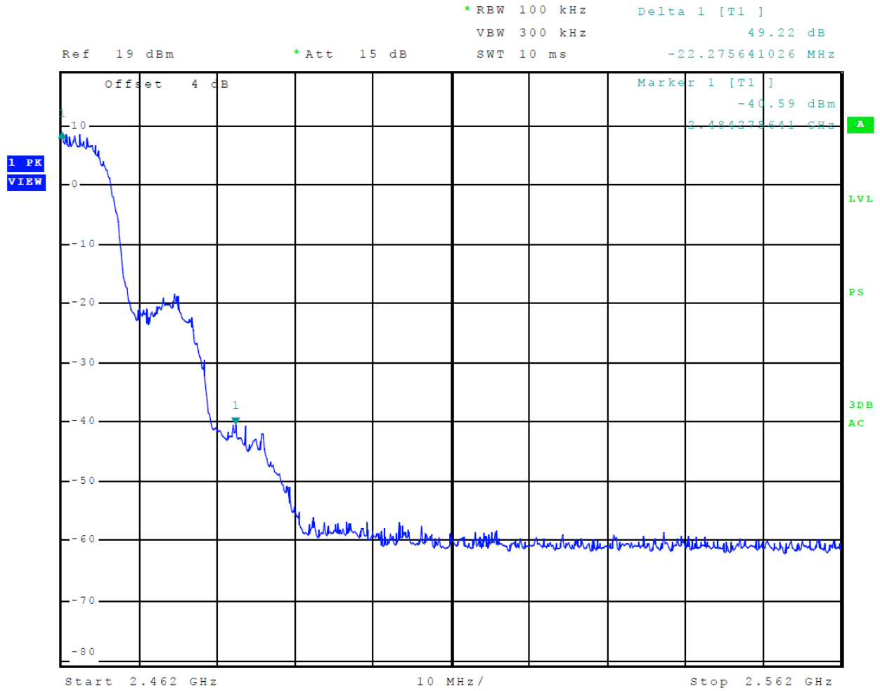
Figure 11 Plot of Transmitter Emissions High Band Edge Mode 5 (DSSS)
