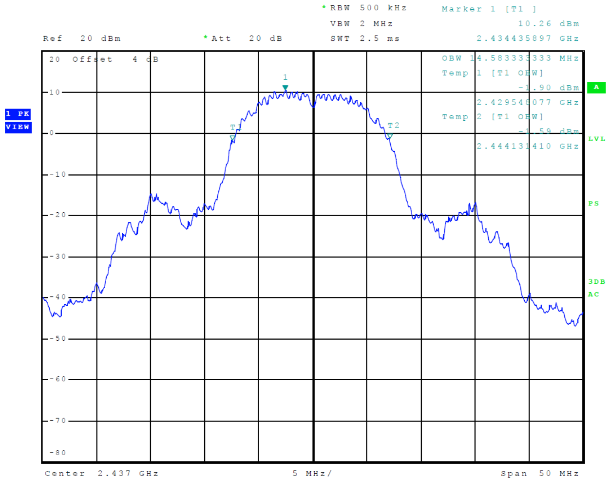
Figure 14 Plot of 6-dB Occupied Bandwidth Mode 5 (DSSS)
