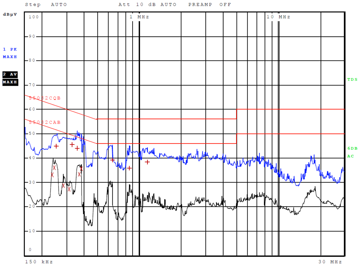
Figure 1 AC Line Conducted emissions of EUT line 1 Configuration #2, (EUT – Computer)
