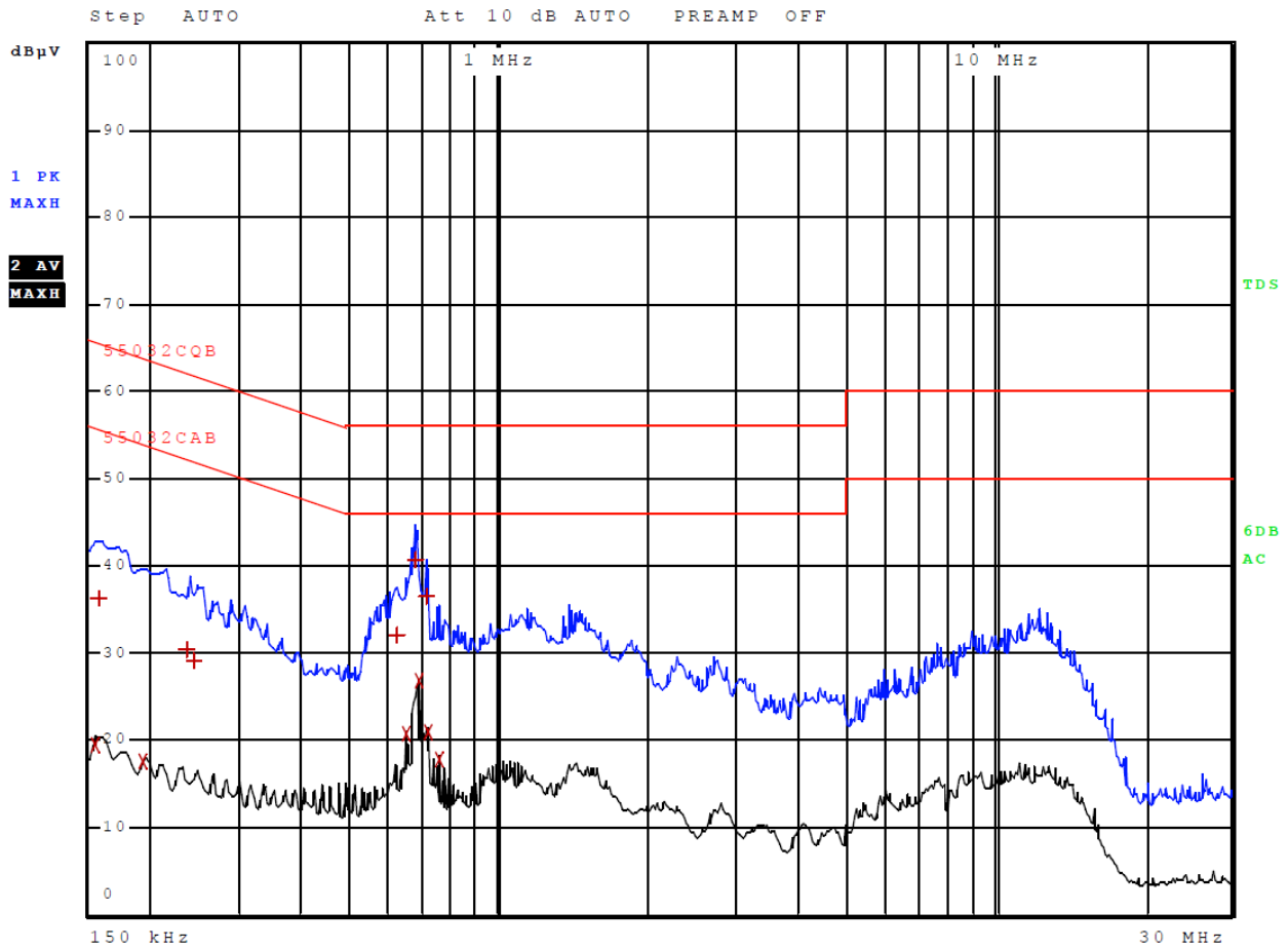
Figure 4 AC Line Conducted emissions of EUT line 2 Configuration #3, (EUT – 362-00096-00)
