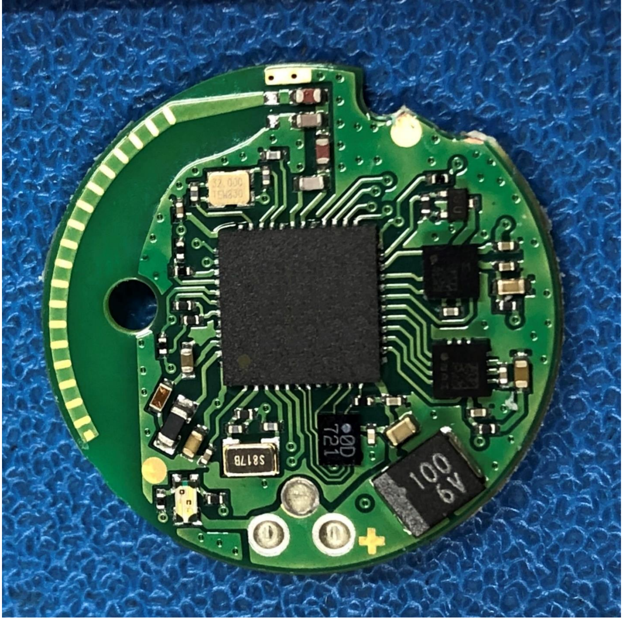
Figure 3 - PCB, Top
