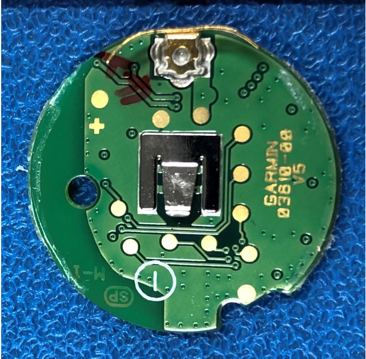
Figure 2 - PCB, Bottom
