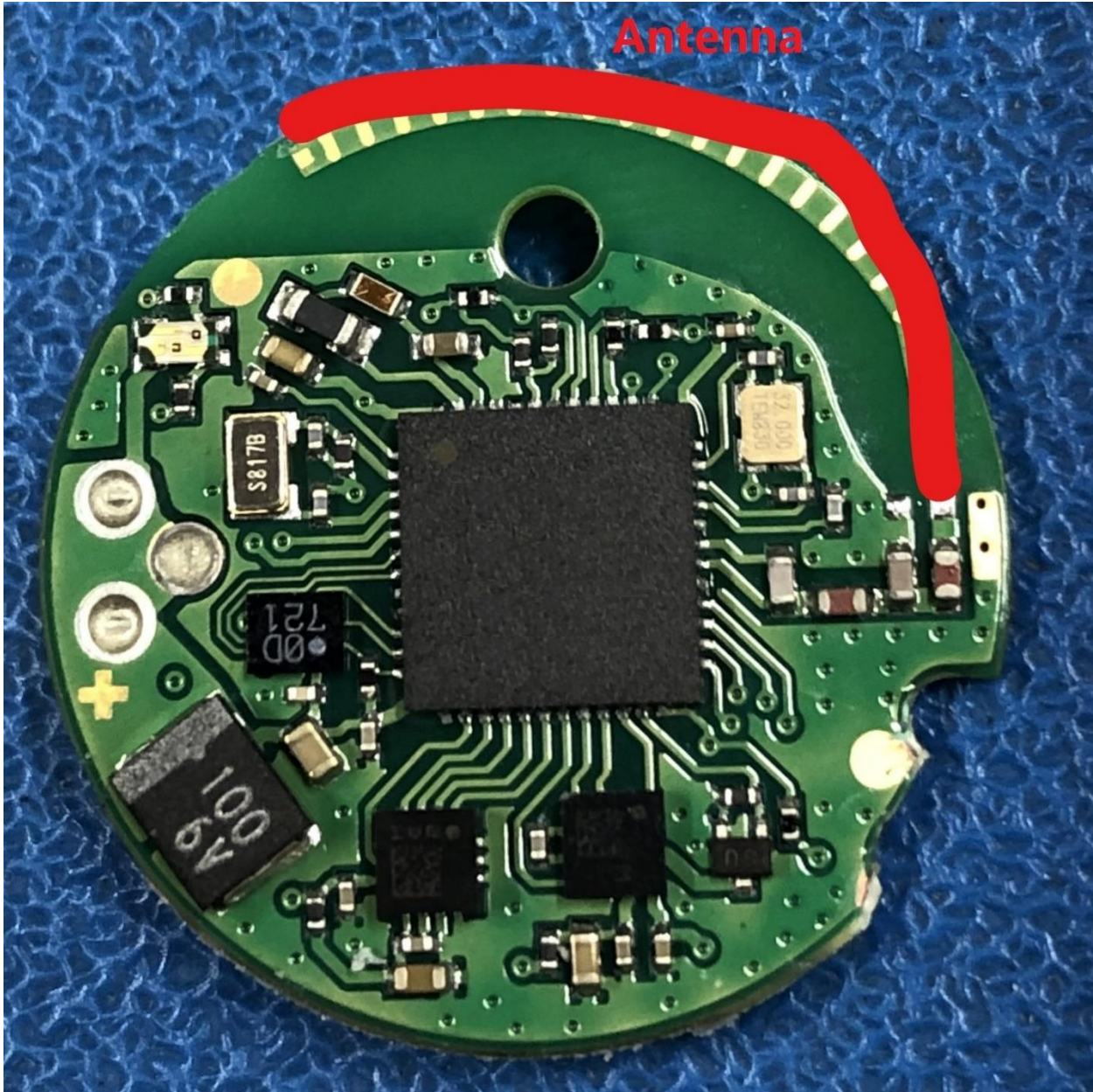
Figure 1 - PCB, Antenna
