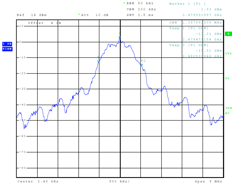
Figure 19 Plot of Transmitter Emissions 99% Occupied Bandwidth (GMSK)
