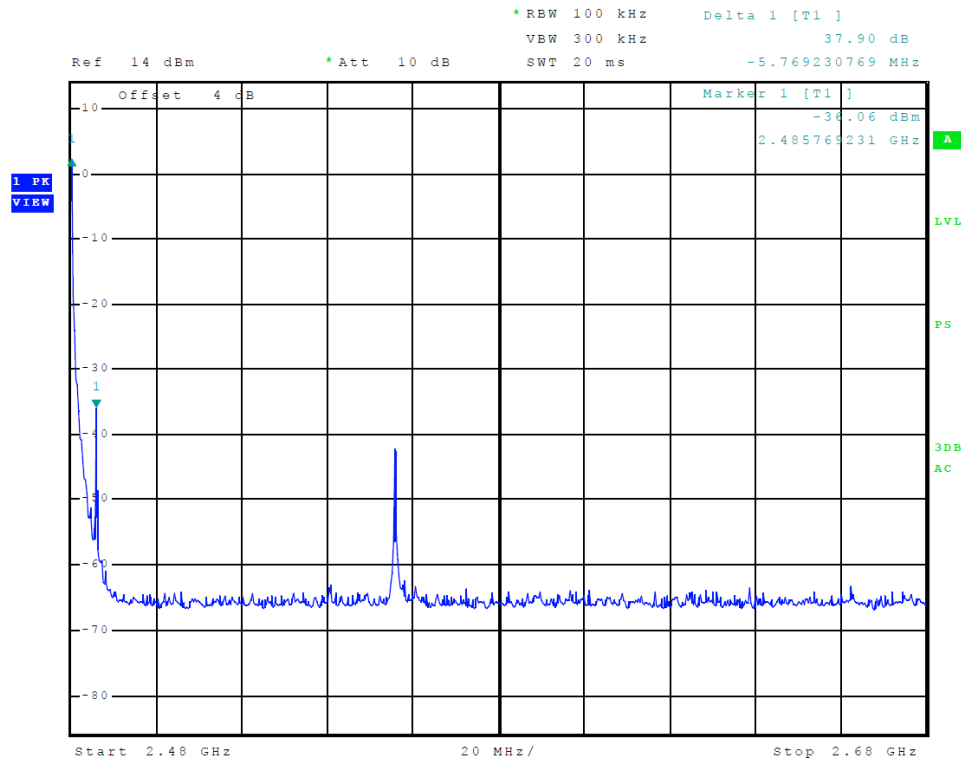
Figure 12 Plot of Transmitter Emissions High Band Edge (GMSK)
