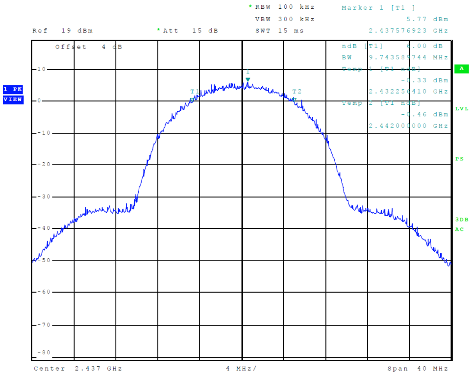
Figure 20 Plot of Transmitter 6-dB Occupied Bandwidth (802.11 b-mode)
