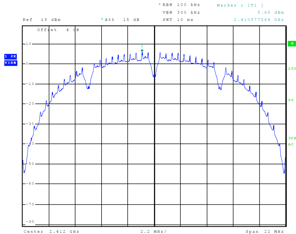
Figure 28 Plot of Transmitter Power Spectral Density (802.11 b-mode)
