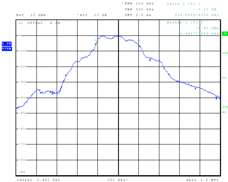
Figure 16 Plot of Transmitter Emissions 6-dB Occupied Bandwidth (GFSK)
