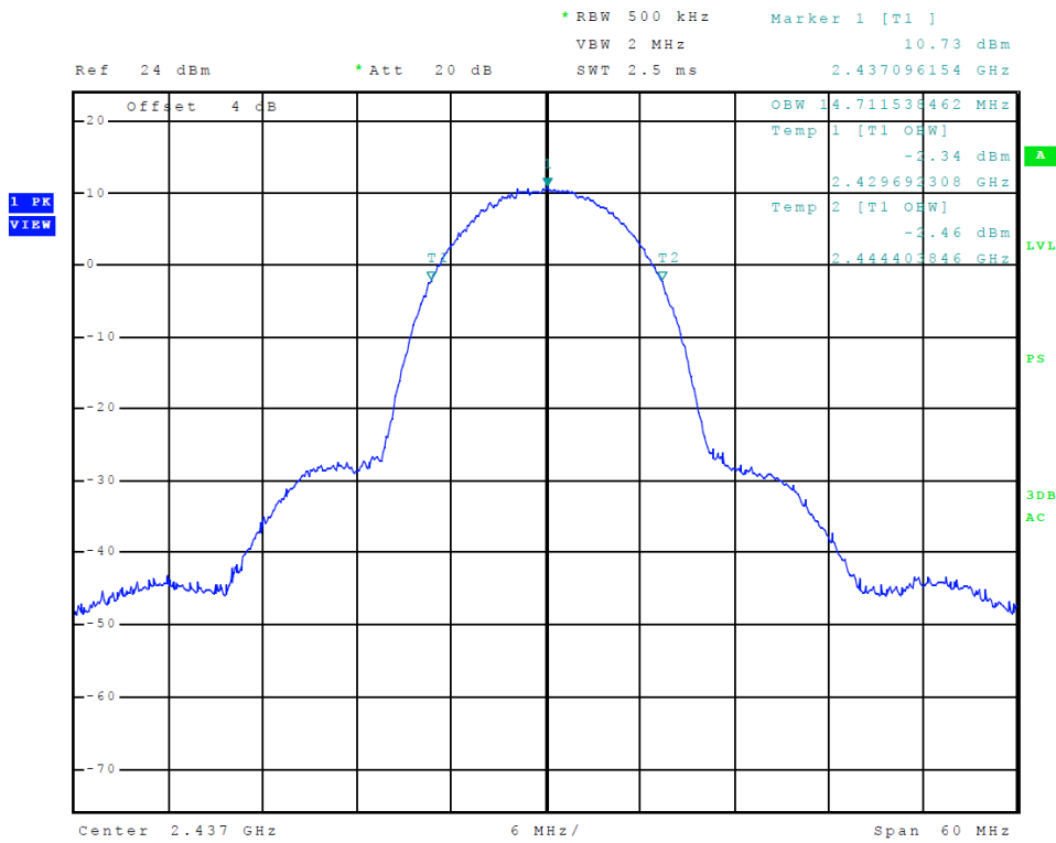
Figure 21 Plot of Transmitter 99% Occupied Bandwidth (802.11 b-mode)
