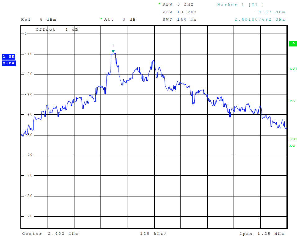
Figure 26 Plot of Transmitter Power Spectral Density (GFSK)
