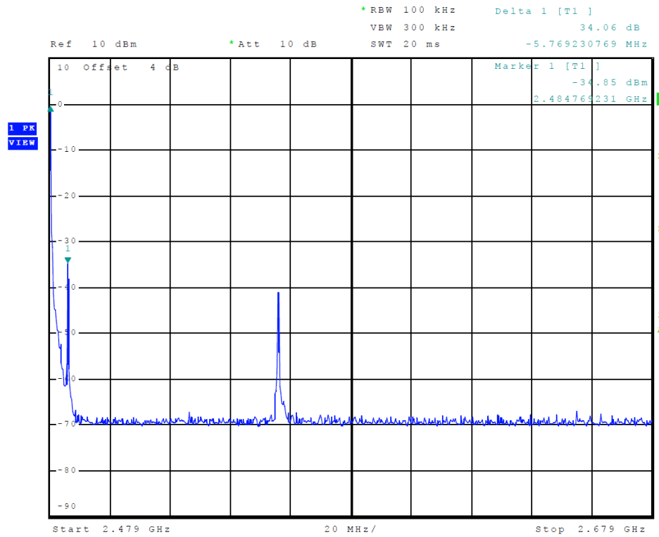
Figure 11 Plot of Transmitter Emissions High Band Edge (GFSK)
