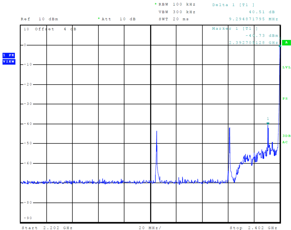
Figure 6 Plot of Transmitter Emissions Low Band Edge (GFSK)
