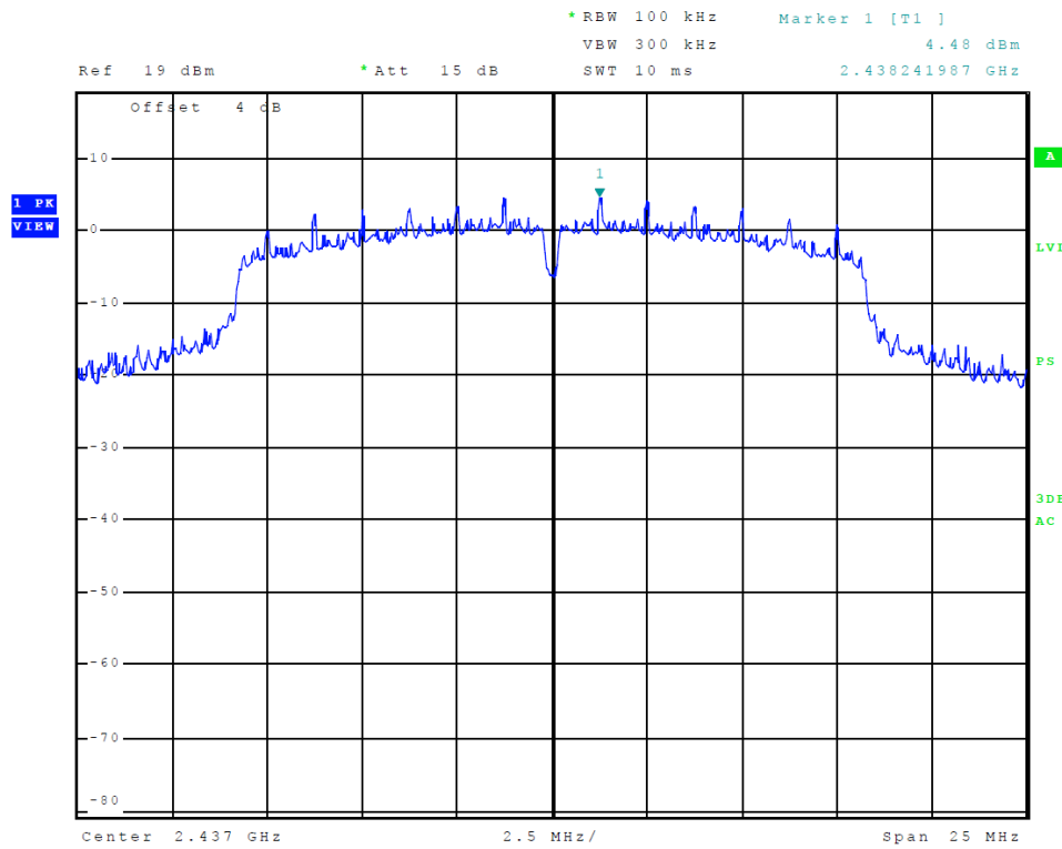
Figure 29 Plot of Transmitter Power Spectral Density (802.11 g-mode)
