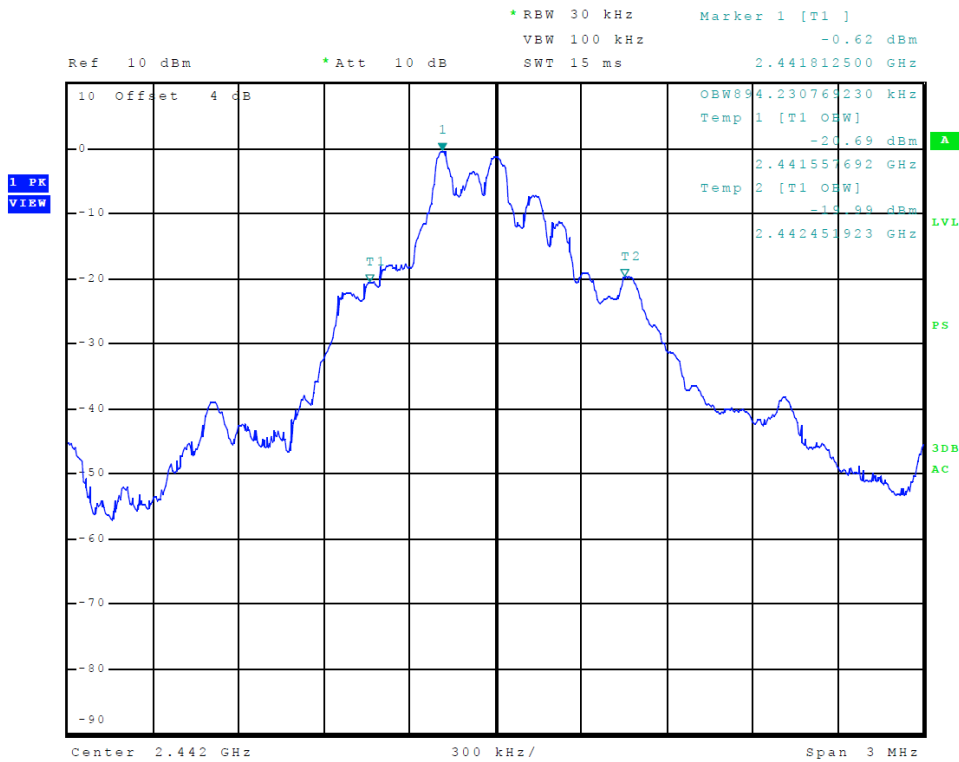
Figure 17 Plot of Transmitter Emissions 99% Occupied Bandwidth (GFSK)
