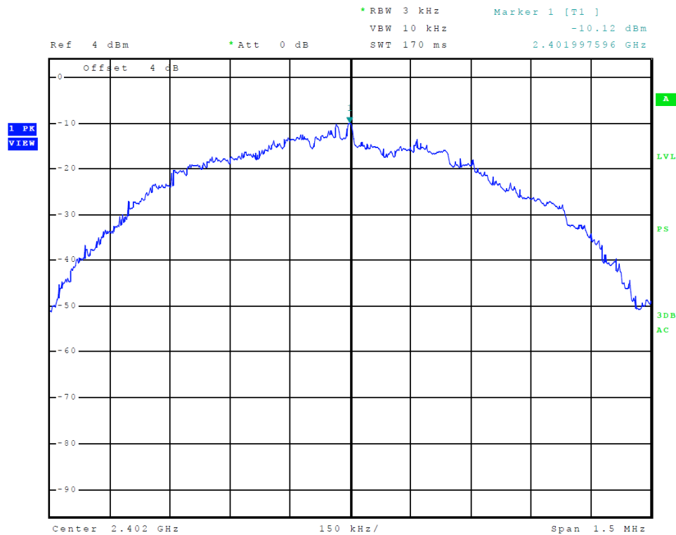
Figure 27 Plot of Transmitter Power Spectral Density (GMSK)
