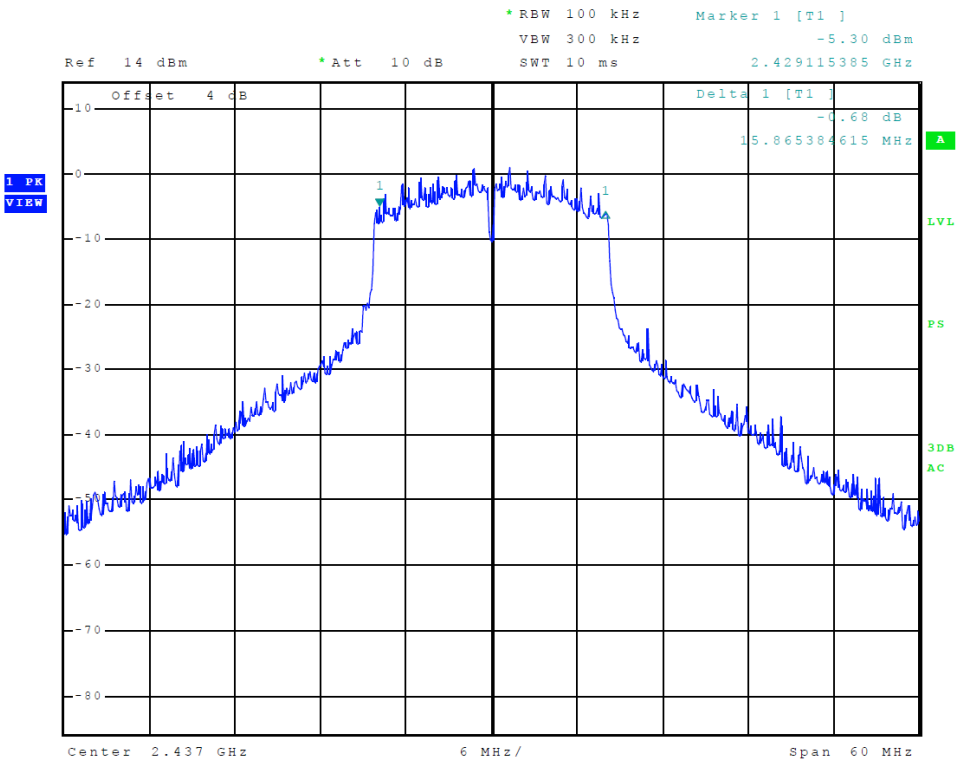
Figure 22 Plot of Transmitter 6-dB Occupied Bandwidth (802.11 g-mode)
