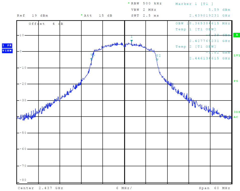
Figure 25 Plot of Transmitter 99% Occupied Bandwidth (802.11 n-mode)
