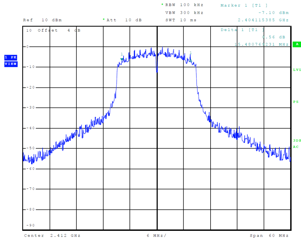
Figure 24 Plot of Transmitter 6-dB Occupied Bandwidth (802.11 n-mode)
