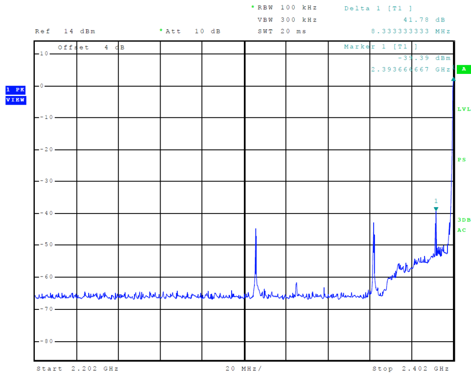
Figure 7 Plot of Transmitter Emissions Low Band Edge (GMSK)
