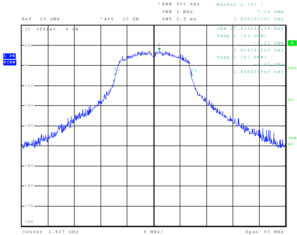
Figure 23 Plot of Transmitter 99% Occupied Bandwidth (802.11 g-mode)
