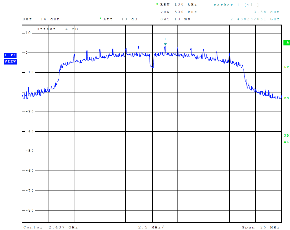
Figure 30 Plot of Transmitter Power Spectral Density (802.11 n-mode)
