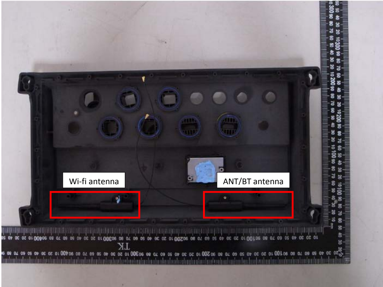
Figure 5 - ANTENNA LOCATION
