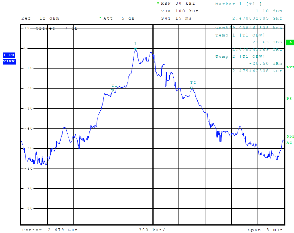
Figure 3 Plot of Transmitter Emissions 99% Occupied Bandwidth (GFSK)
