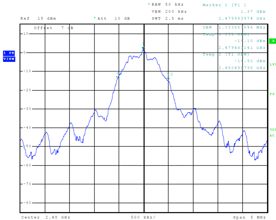
Figure 4 Plot of Transmitter Emissions 99% Occupied Bandwidth (GMSK)
