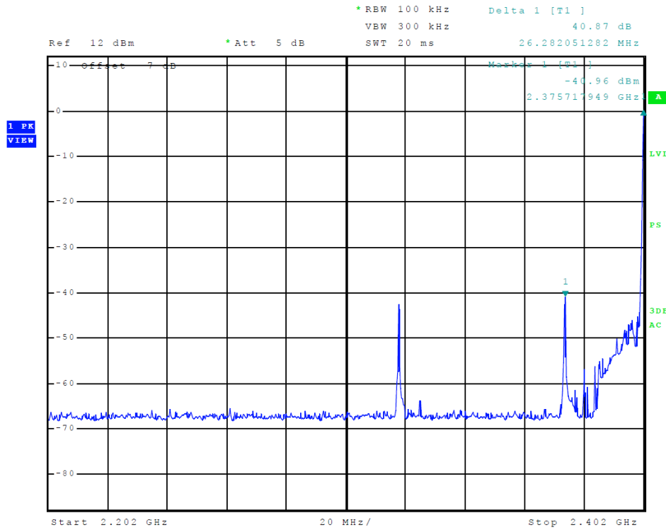
Figure 5 Plot of Transmitter Emissions Low Band Edge (GFSK)
