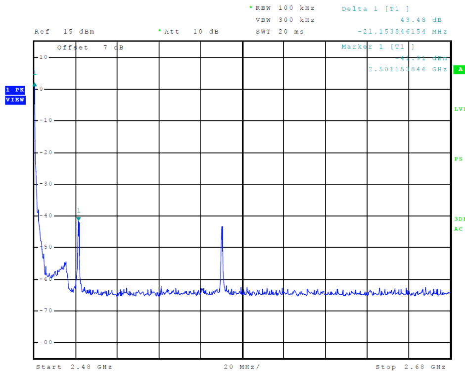
Figure 8 Plot of Transmitter Emissions High Band Edge (GMSK)
