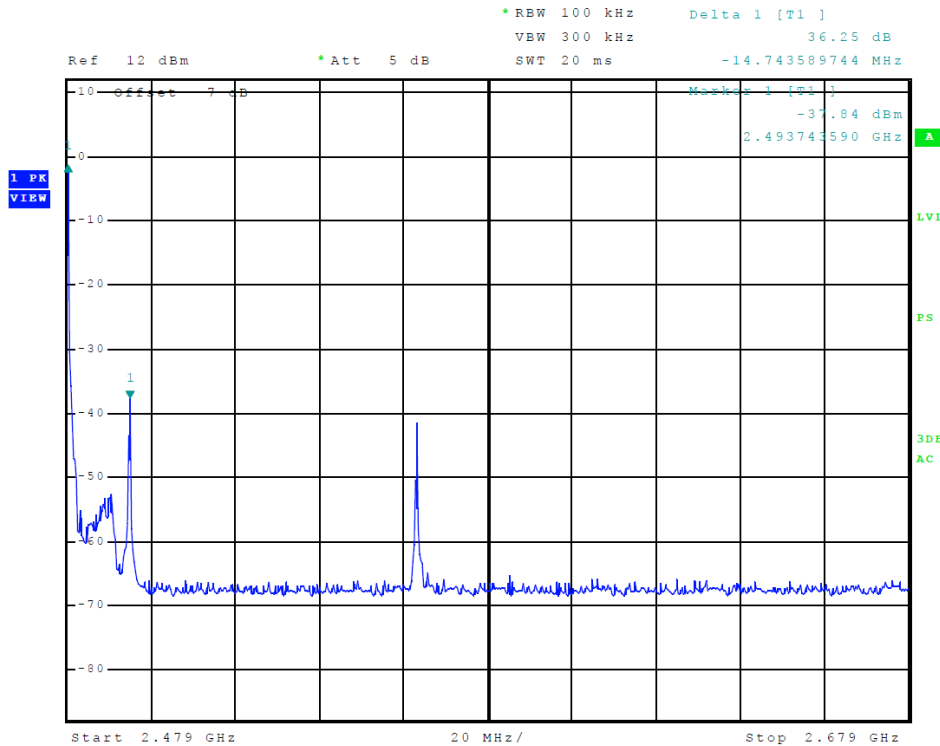
Figure 7 Plot of Transmitter Emissions High Band Edge (GFSK)
