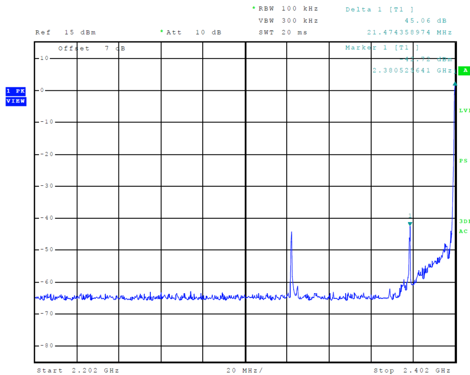
Figure 6 Plot of Transmitter Emissions Low Band Edge (GMSK)
