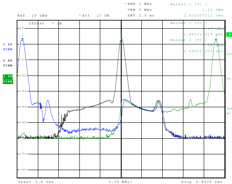
Figure 2 Plot of Transmitter Emissions Operation in 2402-2480 MHz (GMSK)
