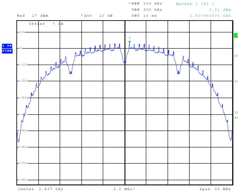
Figure 16 Plot of Transmitter Power Spectral Density (802.11 b-mode)
