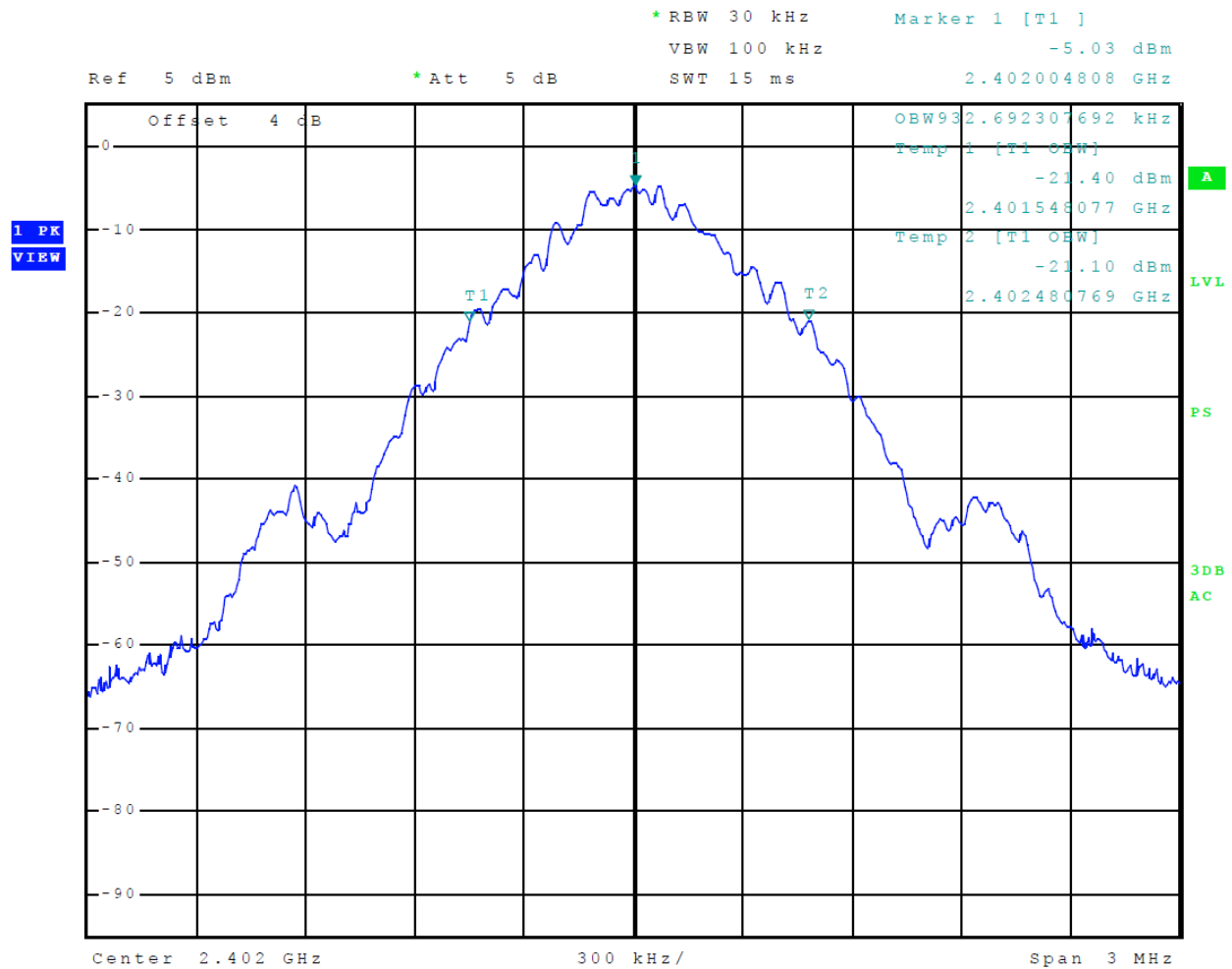
Figure 7 Plot of Transmitter Emissions 99% Occupied Bandwidth ANT (GFSK)
