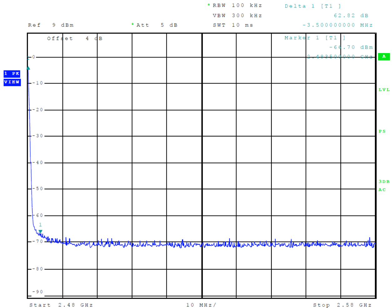
Figure 11 Plot of Transmitter Emissions High Band Edge ANT (GFSK)
