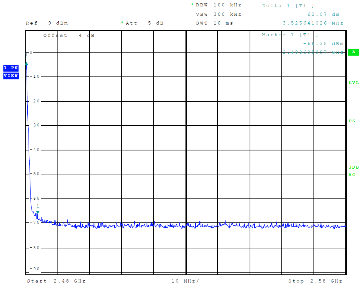
Figure 12 Plot of Transmitter Emissions High Band Edge BT BLE (GMSK)
