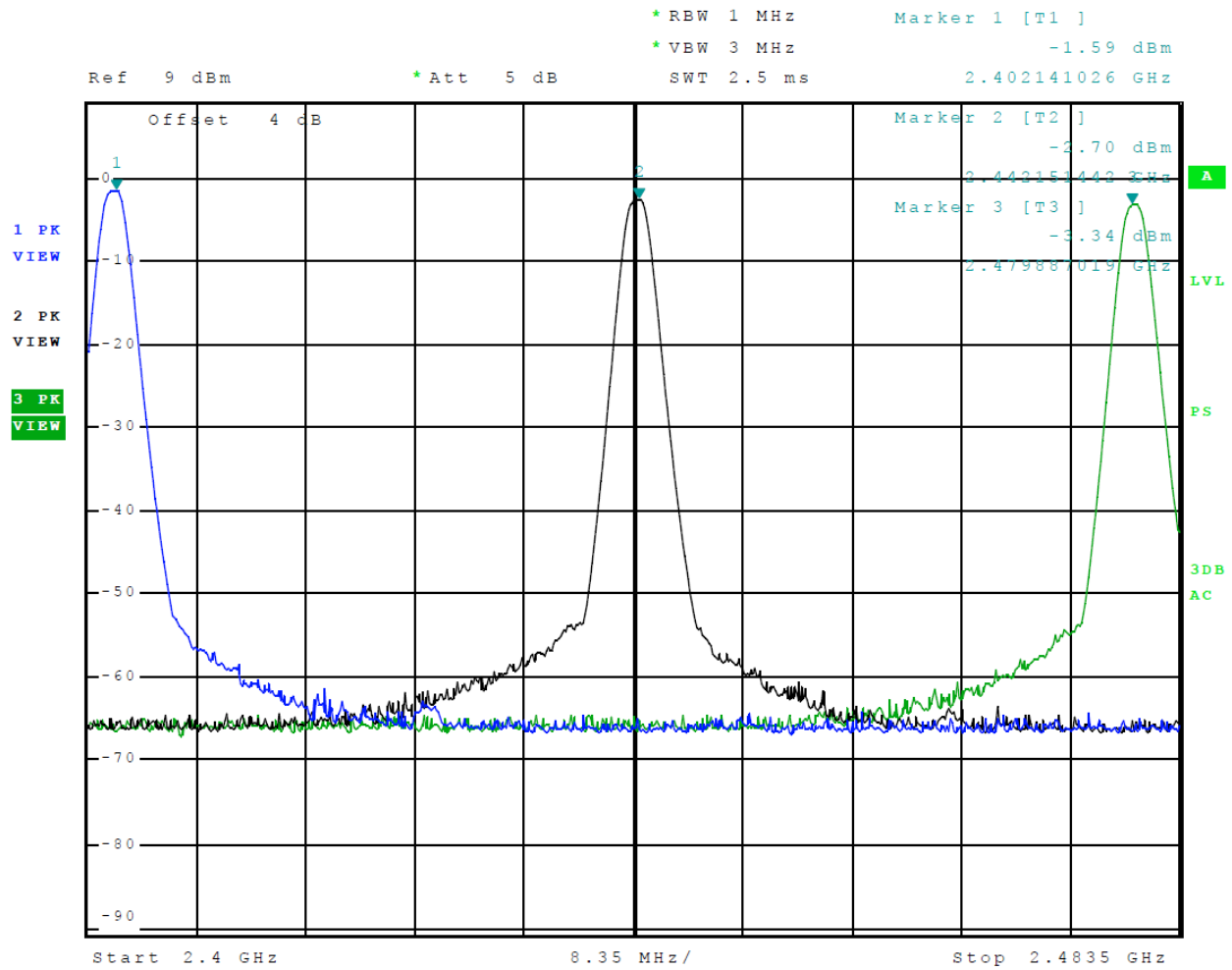
Figure 6 Plot of Transmitter Emissions Operation in 2402-2480 MHz BT BLE (GMSK)
