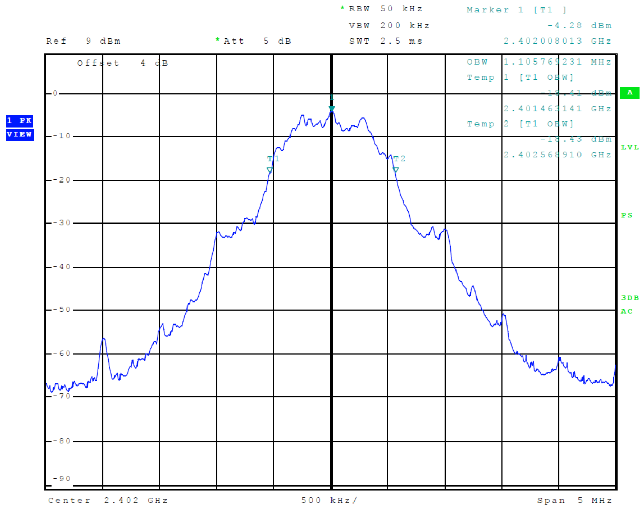
Figure 8 Plot of Transmitter Emissions 99% Occupied Bandwidth BT BLE (GMSK)
