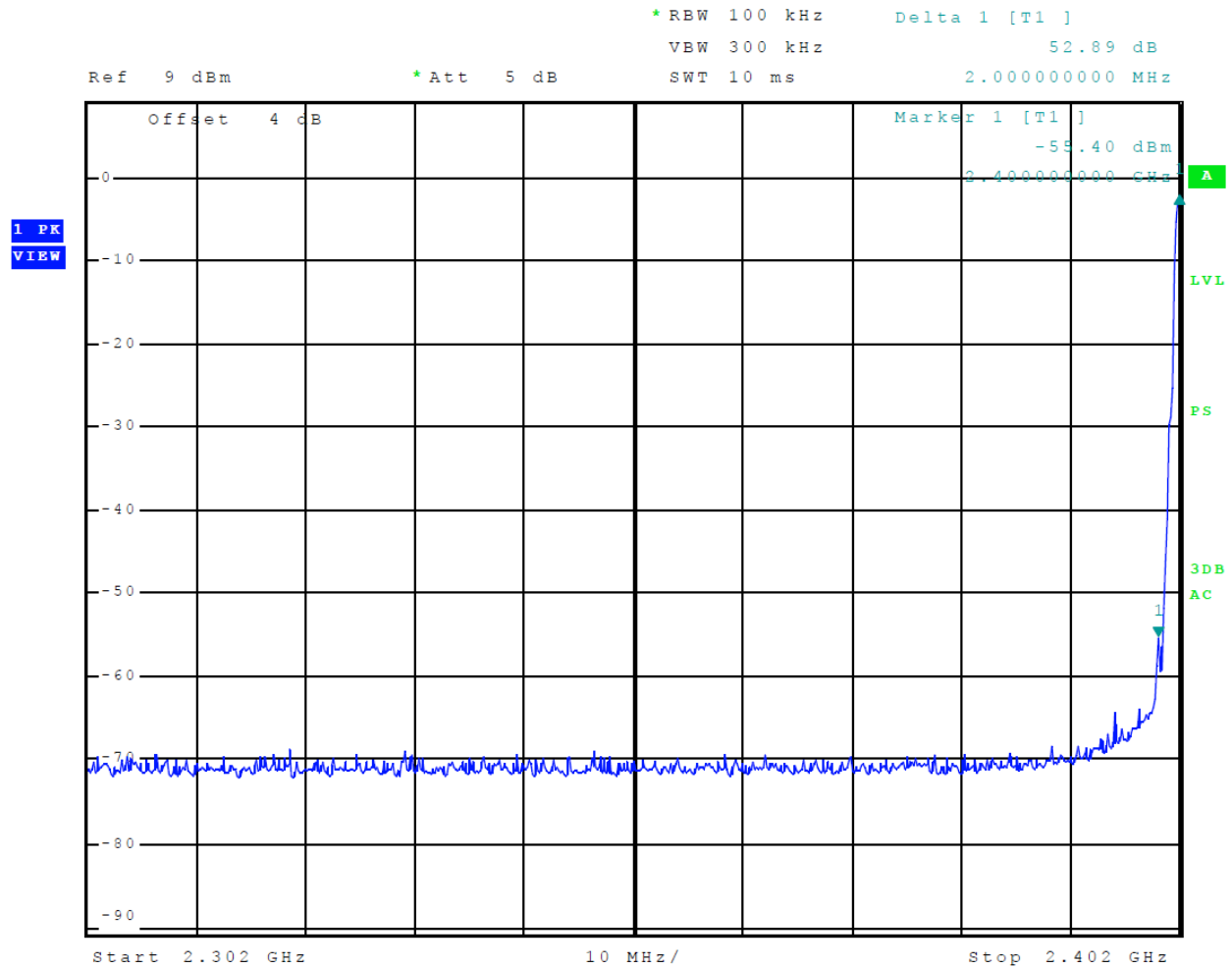
Figure 10 Plot of Transmitter Emissions Low Band Edge BT BLE (GMSK)
