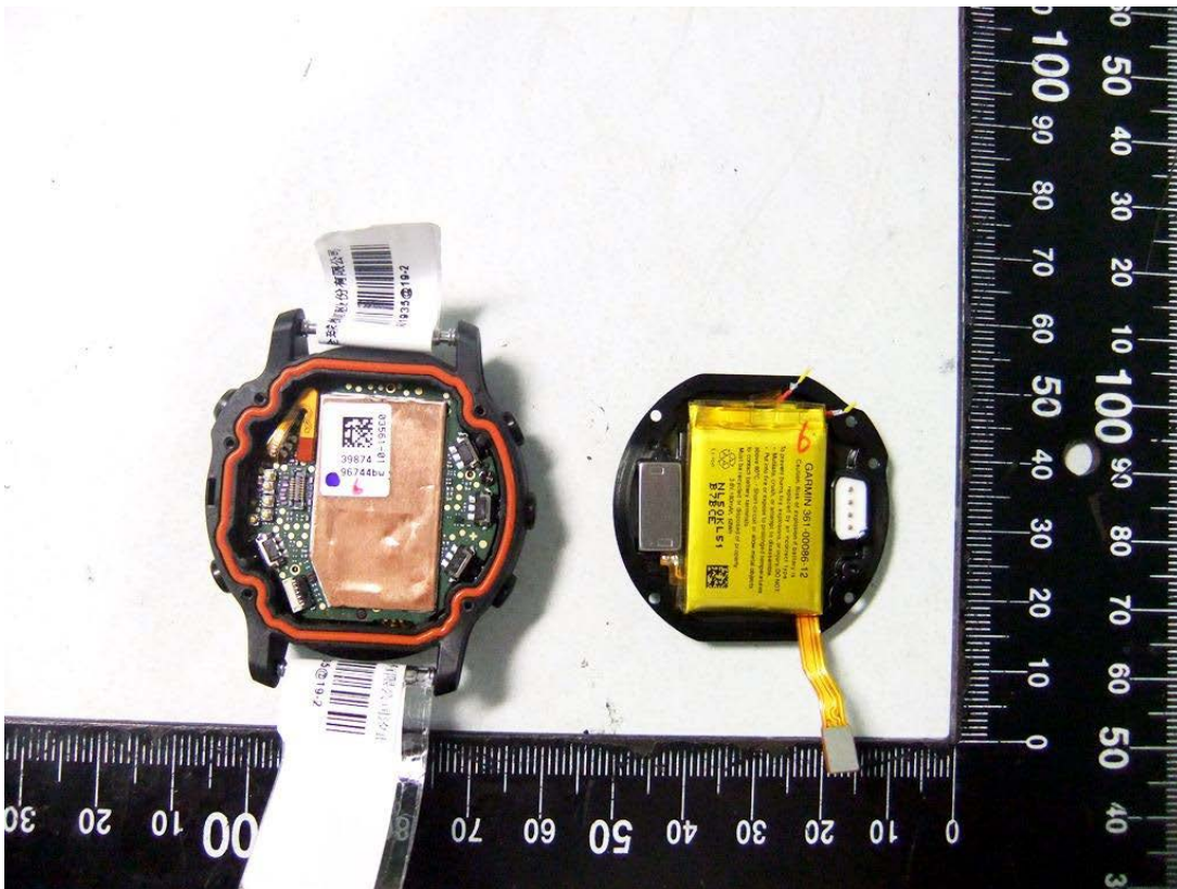
Figure 3- PCB Rear
