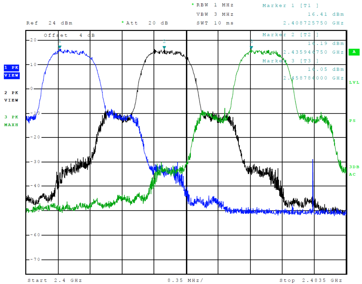
Figure 7 Plot of Transmitter Operation in 2402-2480 MHz (Mode 5 802.11b)
