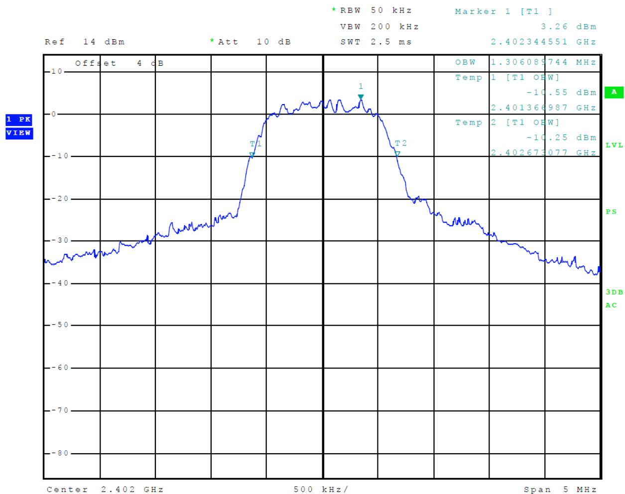
Figure 23 Plot of 6-dB% Occupied Bandwidth (Mode 3 2EDR (PI/4 DPQSK))
