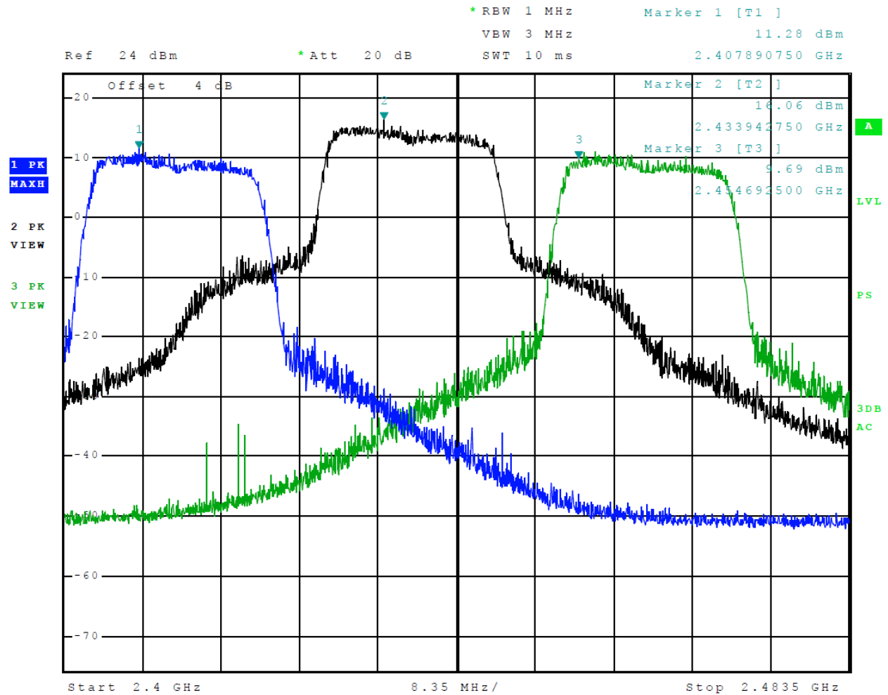
Figure 9 Plot of Transmitter Operation in 2402-2480 MHz (Mode 5 802.11n)
