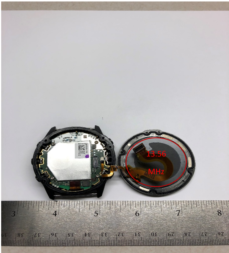
Figure 4 - EUT Rear (shielded), 13.56MHz Antenna
