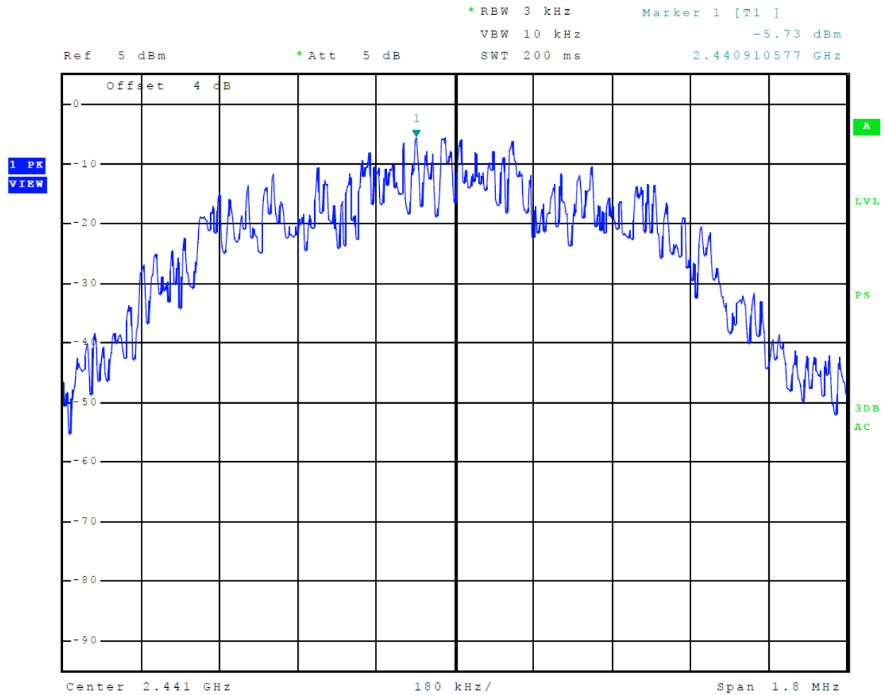
Figure 30 Plot of Transmitter Power Spectral Density (Mode 2 BT BR (GFSK))
