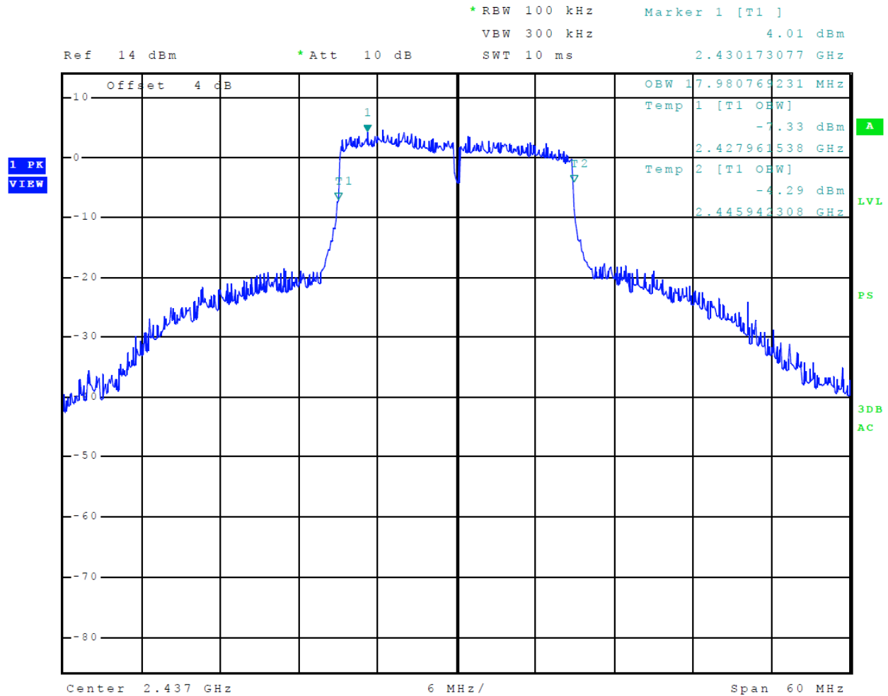
Figure 29 Plot of 99% Occupied Bandwidth (Mode 5 802.11n)
