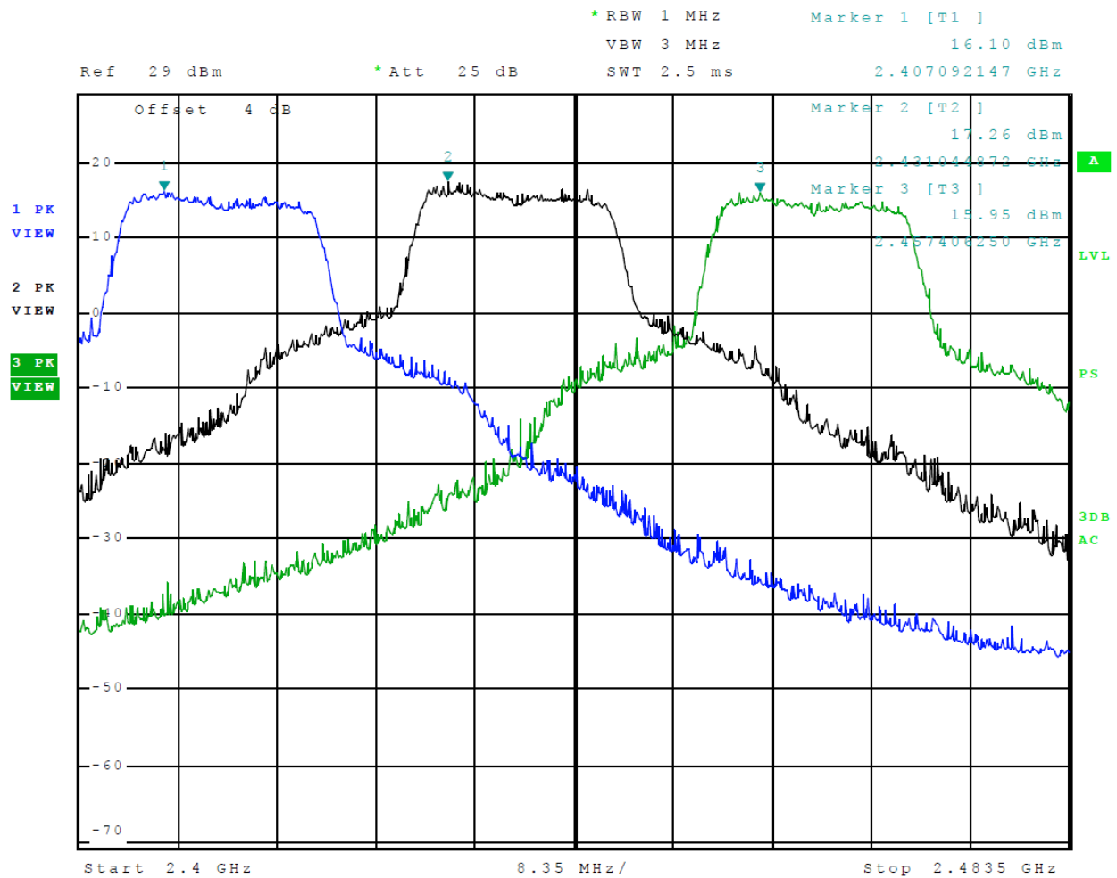
Figure 8 Plot of Transmitter Operation in 2412-2462 MHz (Mode 5 802.11g)
