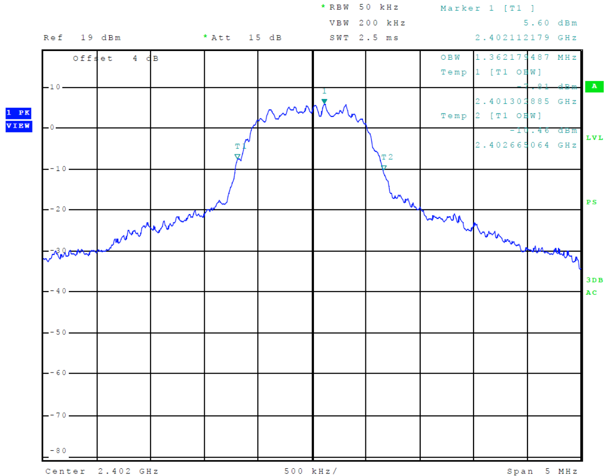
Figure 23 Plot of 99% Occupied Bandwidth (Mode 3 2EDR (PI/4 DPQSK))
