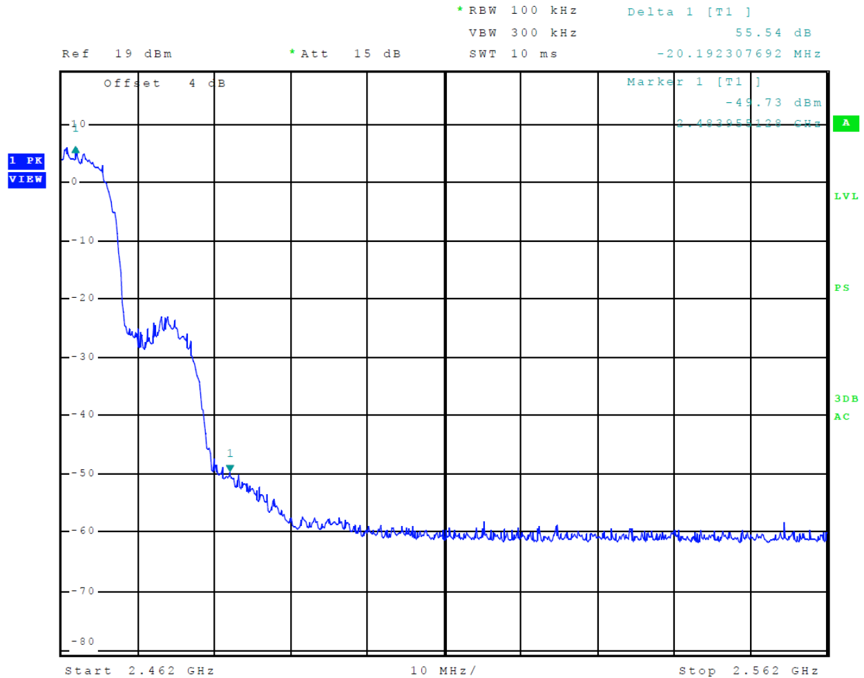
Figure 17 Plot of Transmitter Emissions High Band Edge (Mode 5 802.11b)
