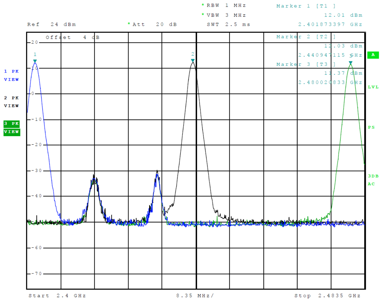
Figure 5 Plot of Transmitter Operation in 2402-2480 MHz (Mode 2 BT BR (GFSK))
