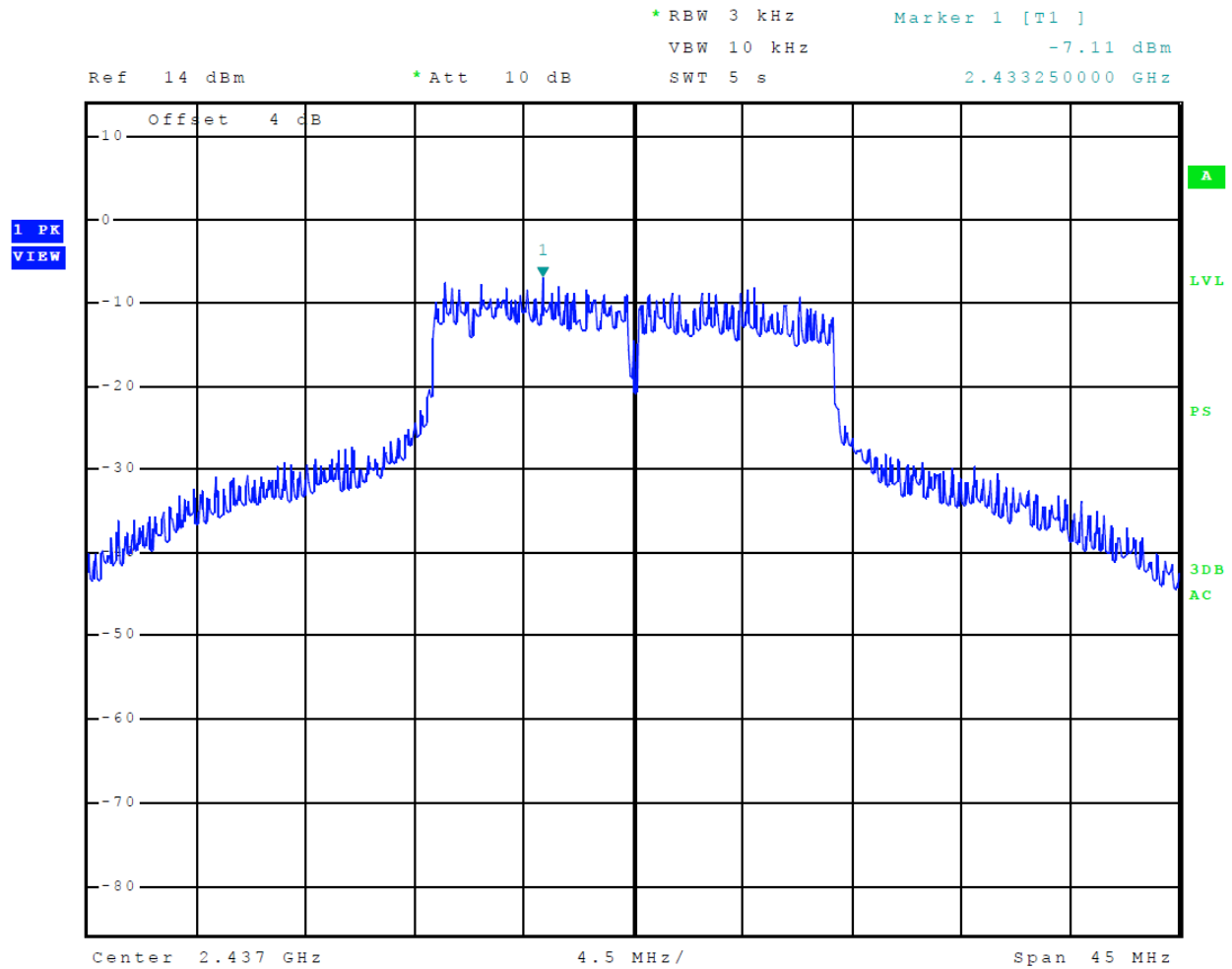
Figure 33 Plot of Transmitter Power Spectral Density (Mode 5 802.11g)
