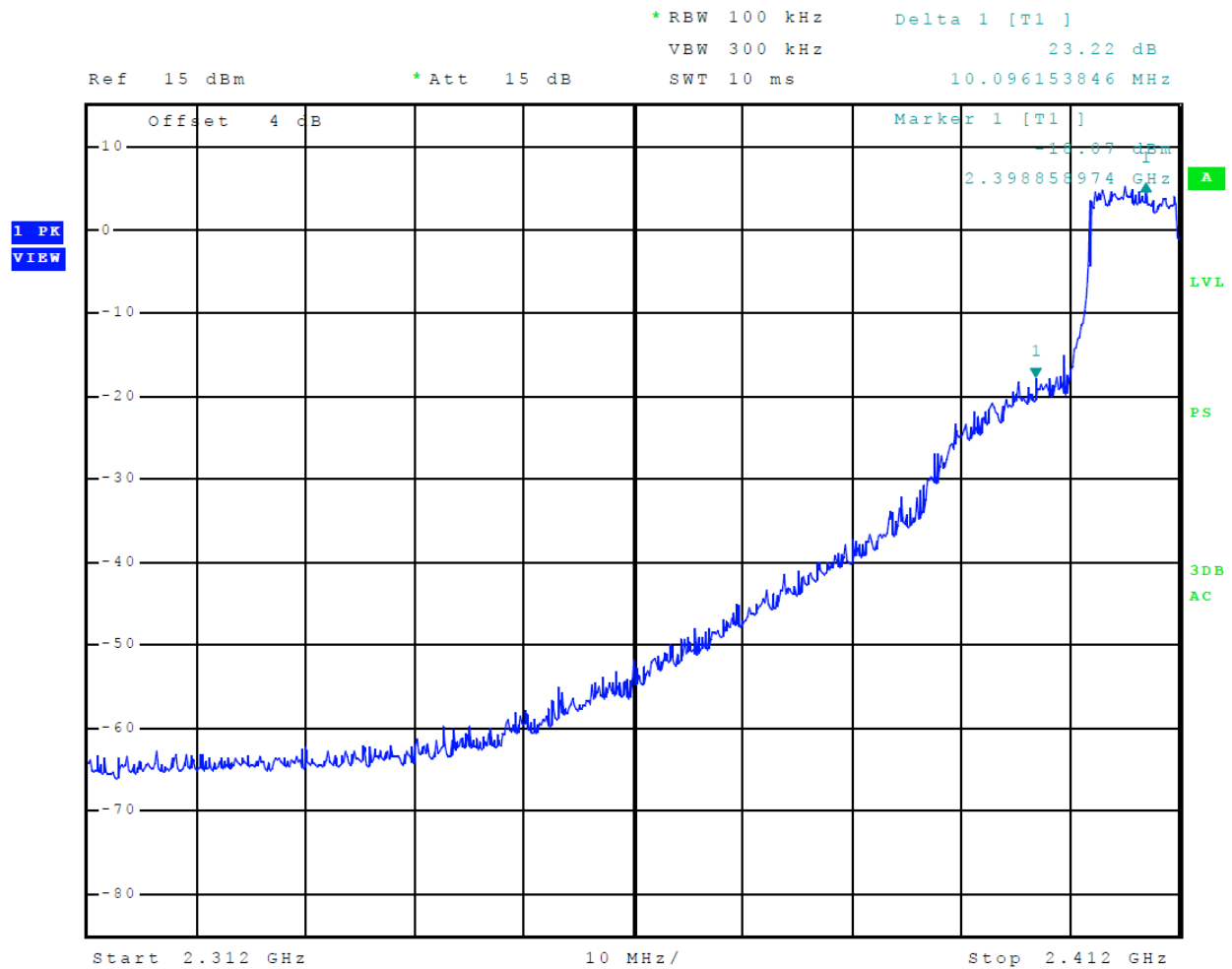
Figure 13 Plot of Transmitter Emissions Low Band Edge (Mode 5 802.11g)
