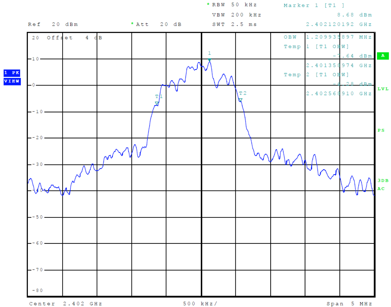
Figure 21 Plot of 99% Occupied Bandwidth (Mode 2 BT BR (GFSK))
