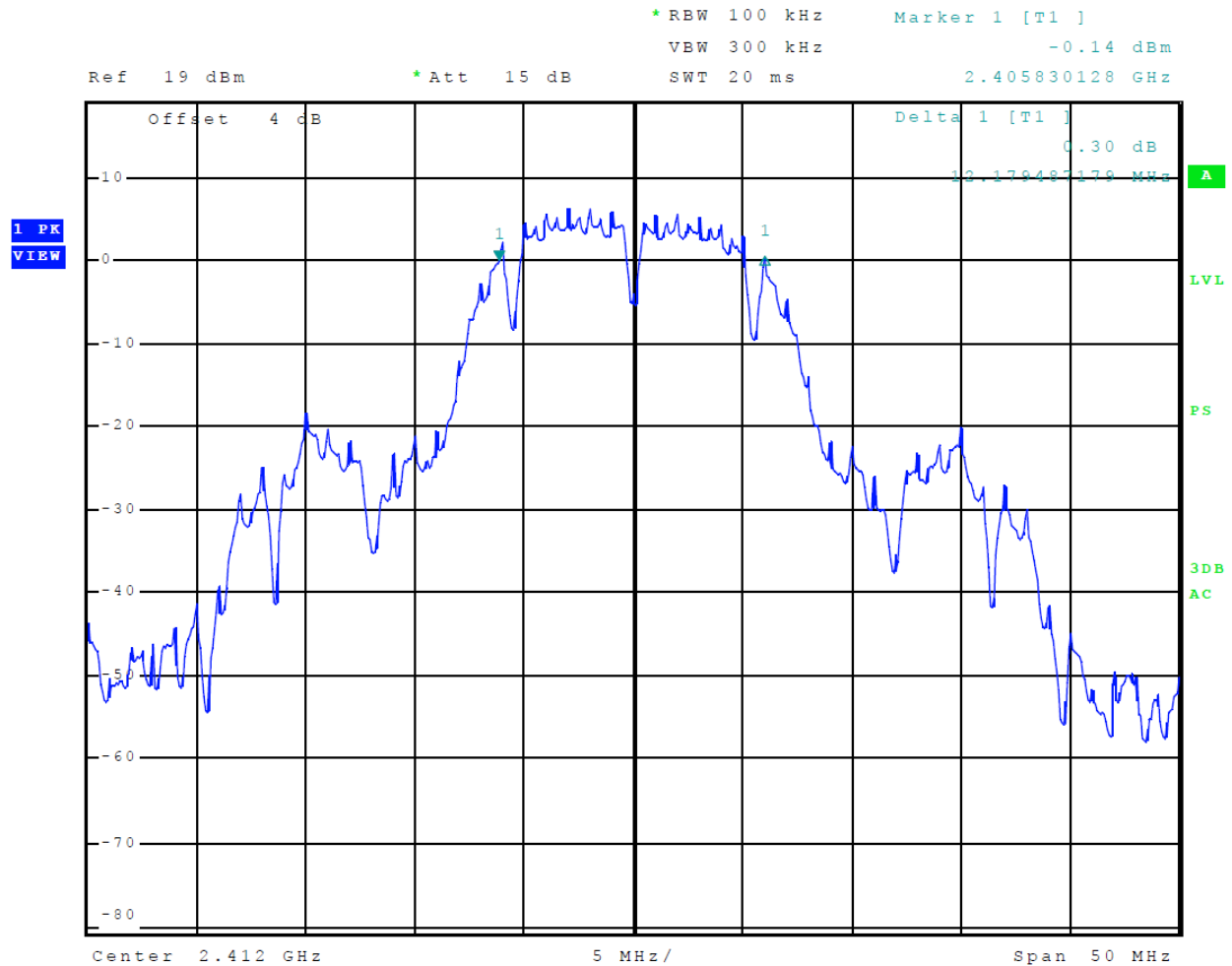
Figure 24 Plot of 6-dB% Occupied Bandwidth (Mode 5 802.11b)
