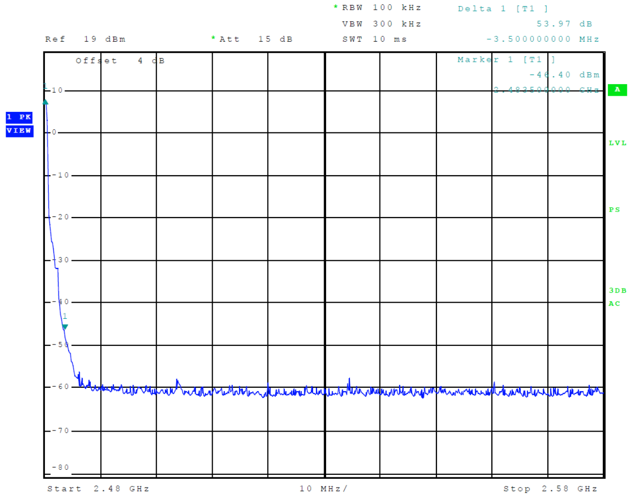
Figure 16 Plot of Transmitter Emissions High Band Edge (Mode 3 2EDR (PI/4 DPQSK))
