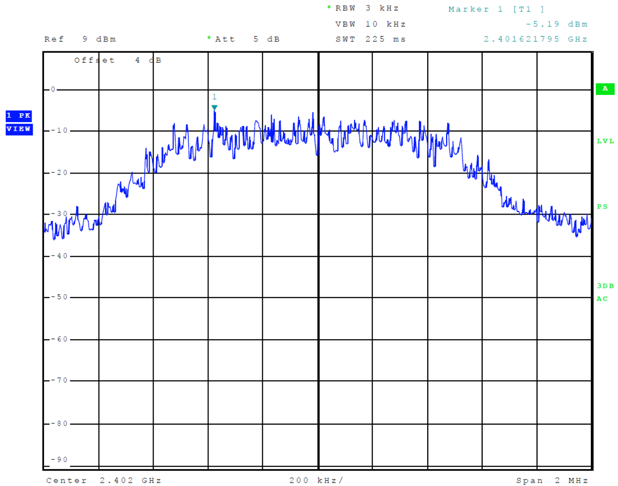
Figure 31 Plot of Transmitter Power Spectral Density (Mode 3 2EDR (PI/4 DPQSK))
