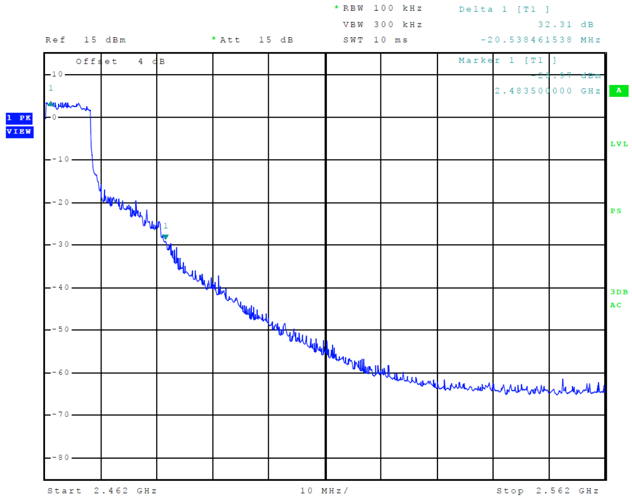
Figure 18 Plot of Transmitter Emissions High Band Edge (Mode 5 802.11g)
