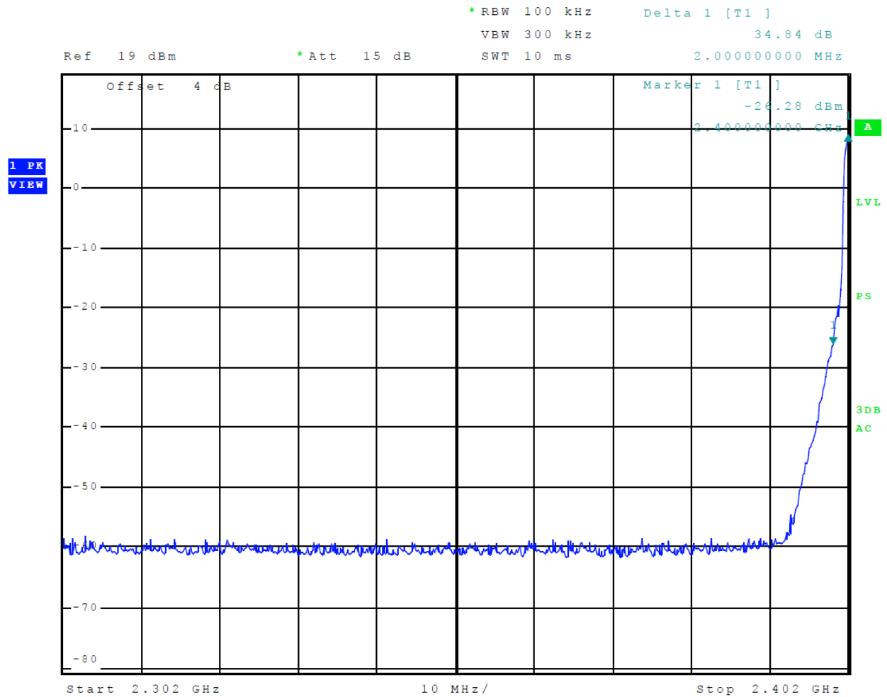
Figure 11 Plot of Transmitter Emissions Low Band Edge (Mode 3 2EDR (PI/4 DPQSK))
