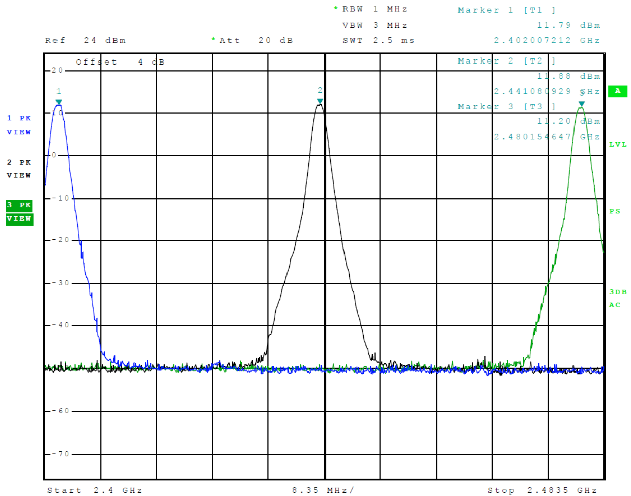
Figure 6 Plot of Transmitter Operation in 2402-2480 MHz (Mode 3 2EDR (PI/4 DPQSK))
