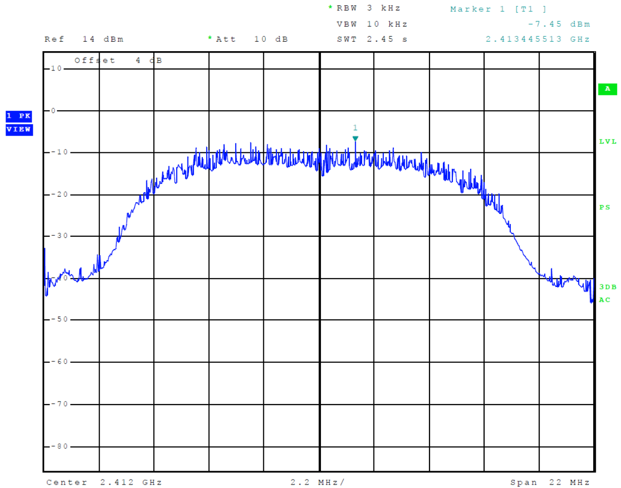
Figure 32 Plot of Transmitter Power Spectral Density (Mode 5 802.11b)
