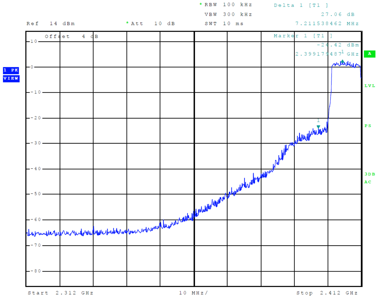
Figure 14 Plot of Transmitter Emissions Low Band Edge (Mode 5 802.11n)
