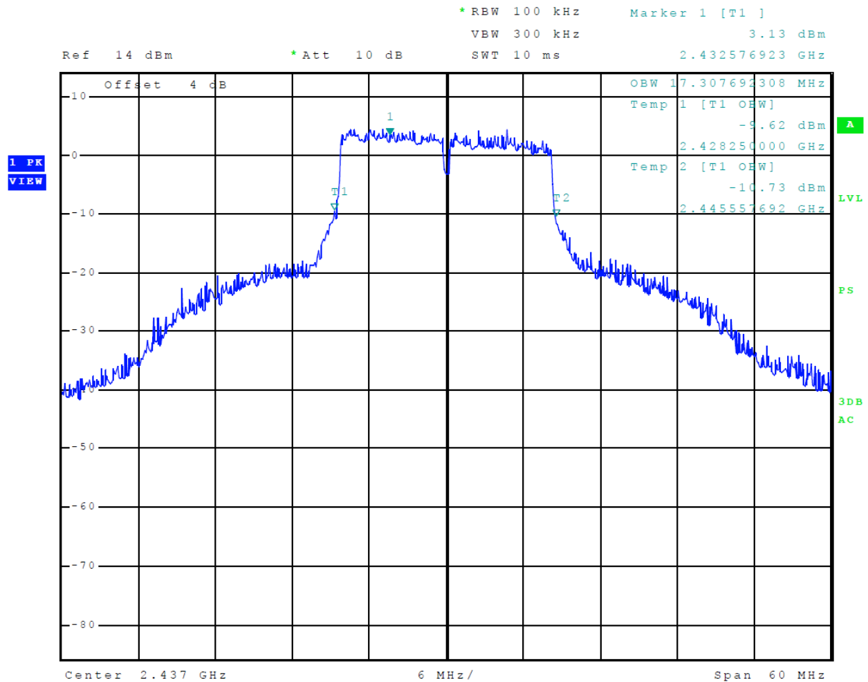
Figure 27 Plot of 99% Occupied Bandwidth (Mode 5 802.11g)
