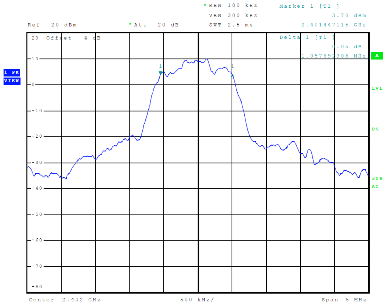
Figure 20 Plot of 6-dB% Occupied Bandwidth (Mode 2 BT BR (GFSK))
