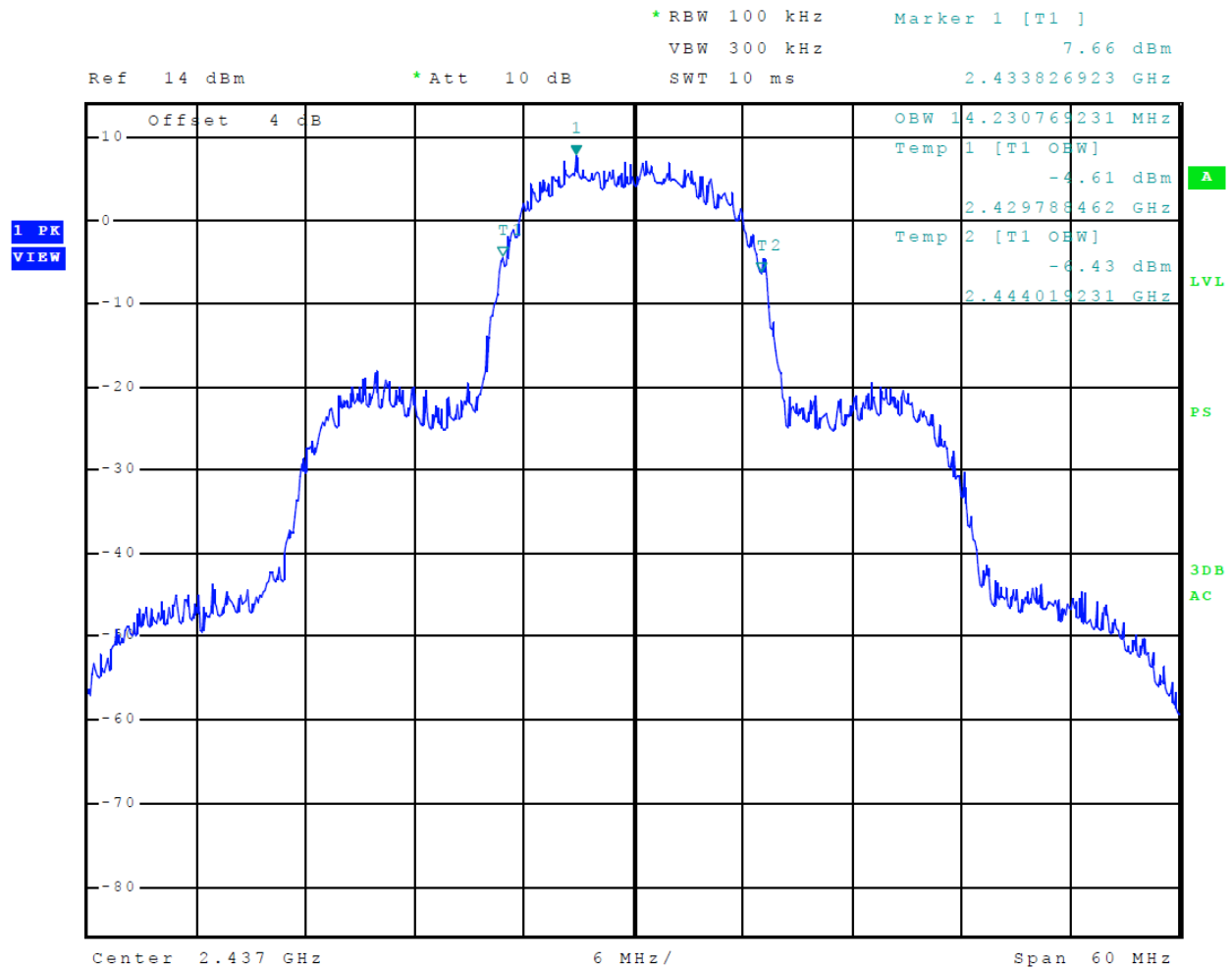
Figure 25 Plot of 99% Occupied Bandwidth (Mode 5 802.11b)
