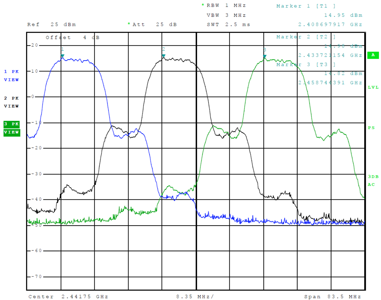
Figure 7 Plot of Transmitter Operation in 2412-2462 MHz (Mode 5 802.11b)
