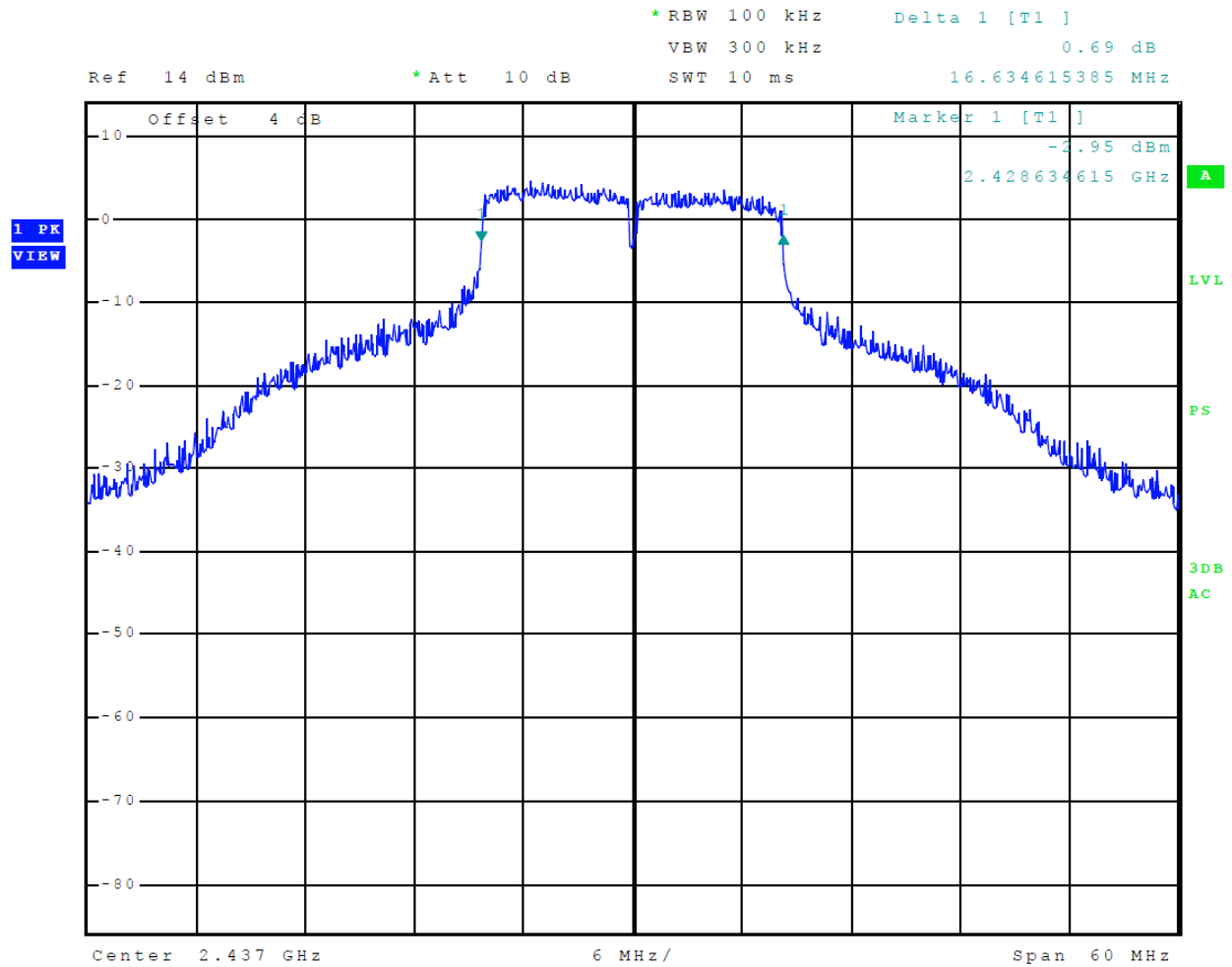
Figure 26 Plot of 6-dB% Occupied Bandwidth (Mode 5 802.11g)
