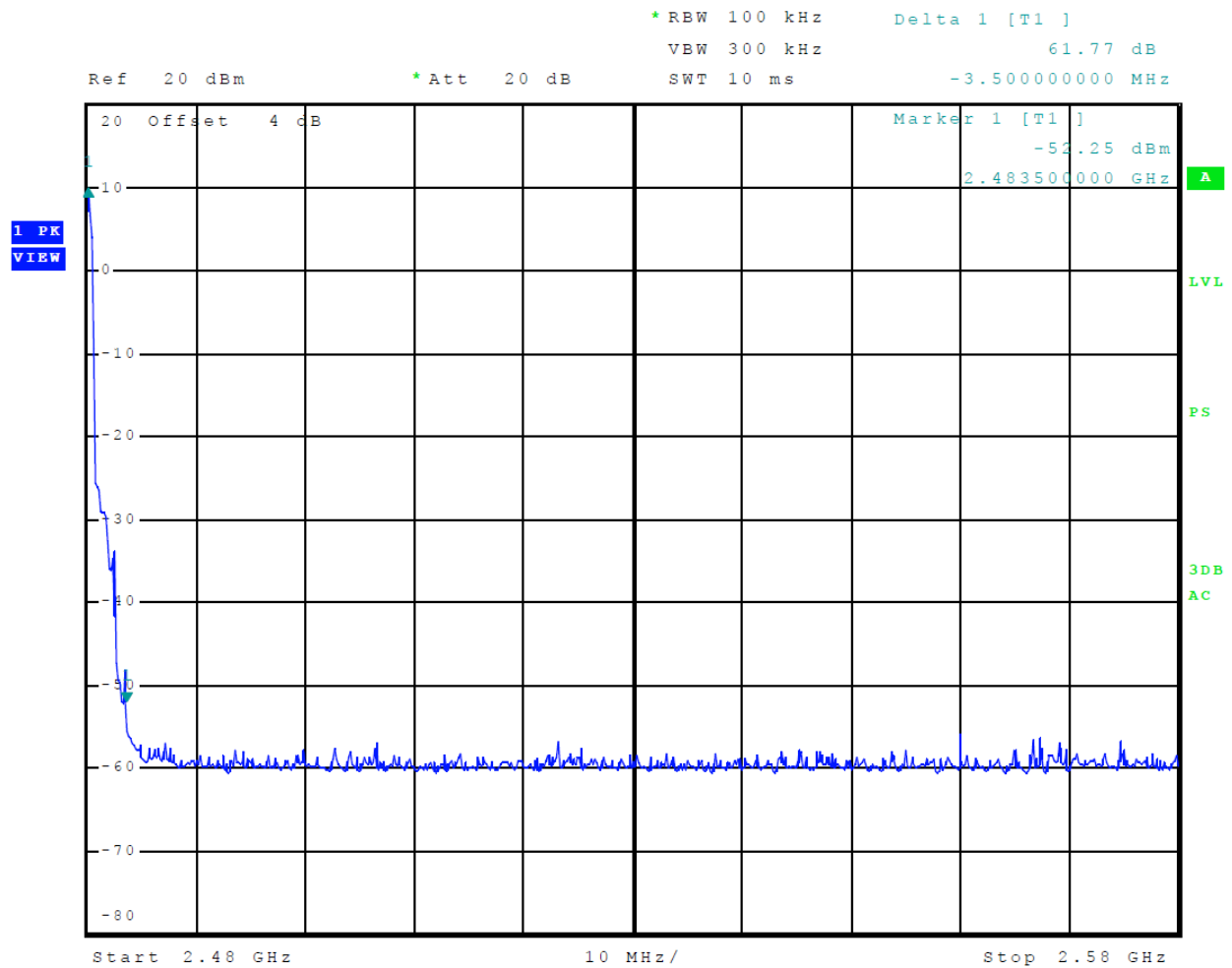
Figure 15 Plot of Transmitter Emissions High Band Edge (Mode 2 BT BR (GFSK))
