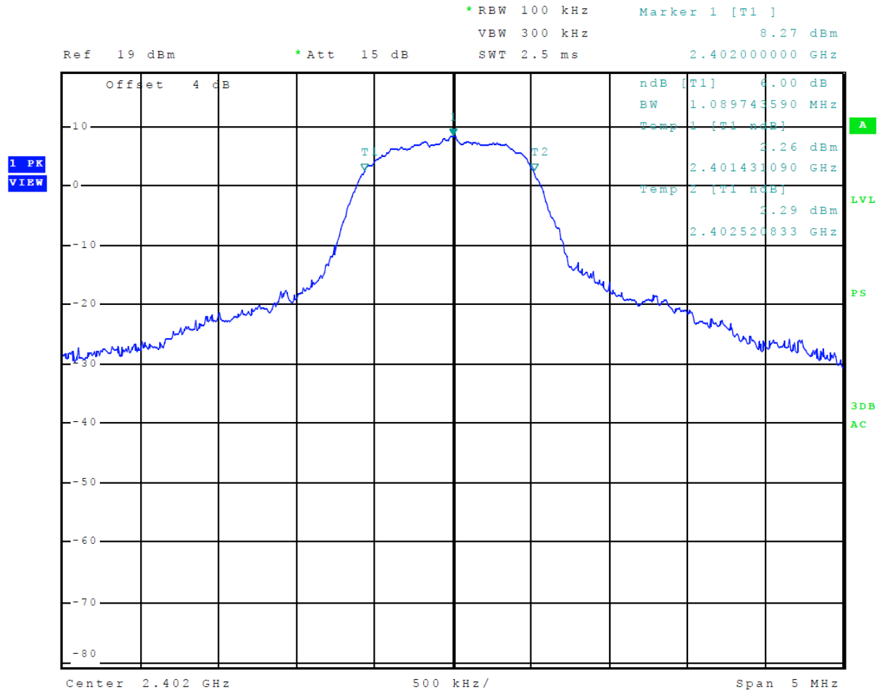
Figure 22 Plot of 6-dB% Occupied Bandwidth (Mode 3 2EDR (PI/4 DPQSK))
