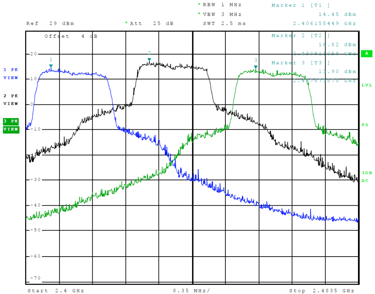
Figure 9 Plot of Transmitter Operation in 2412-2462 MHz (Mode 5 802.11n)
