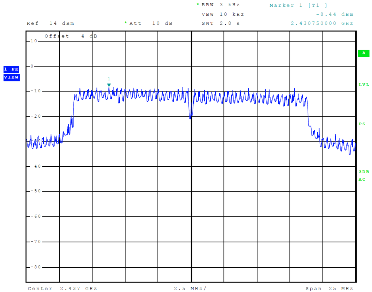
Figure 34 Plot of Transmitter Power Spectral Density (Mode 5 802.11n)
