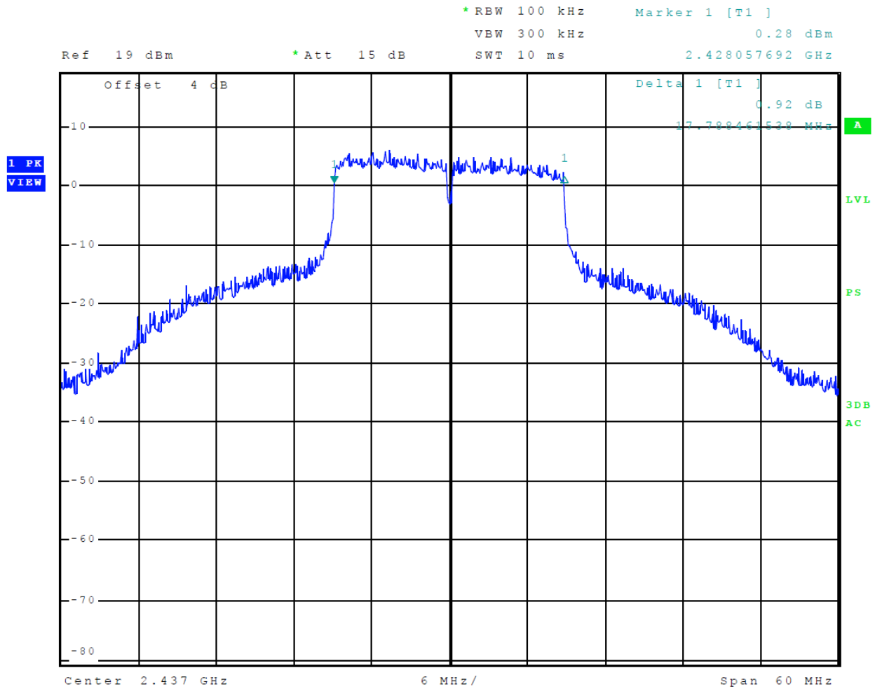
Figure 28 Plot of 6-dB% Occupied Bandwidth (Mode 5 802.11n)
