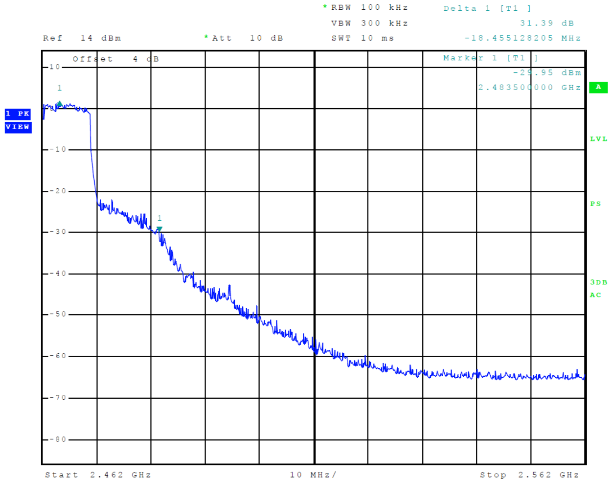
Figure 19 Plot of Transmitter Emissions High Band Edge (Mode 5 802.11n)
