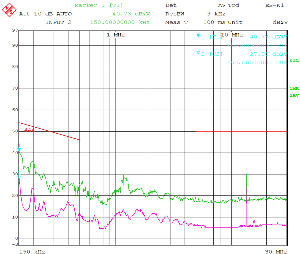
Figure 9 - Conducted Emissions, Line
