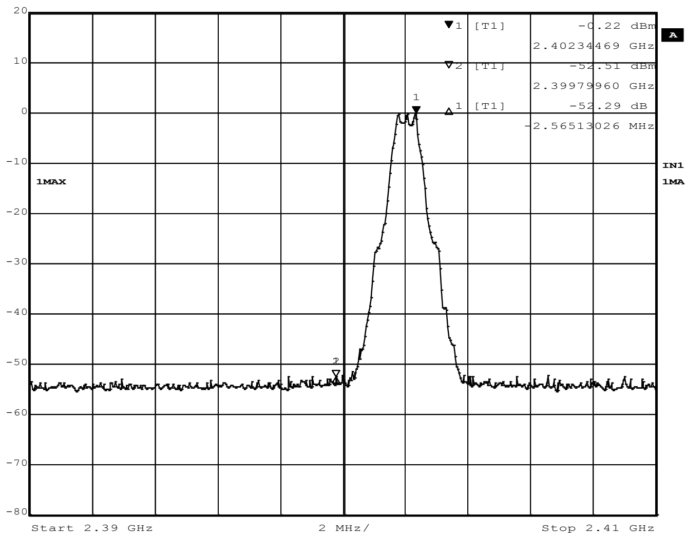
Figure 26 –Band Edge, Low Channel, GMSK
