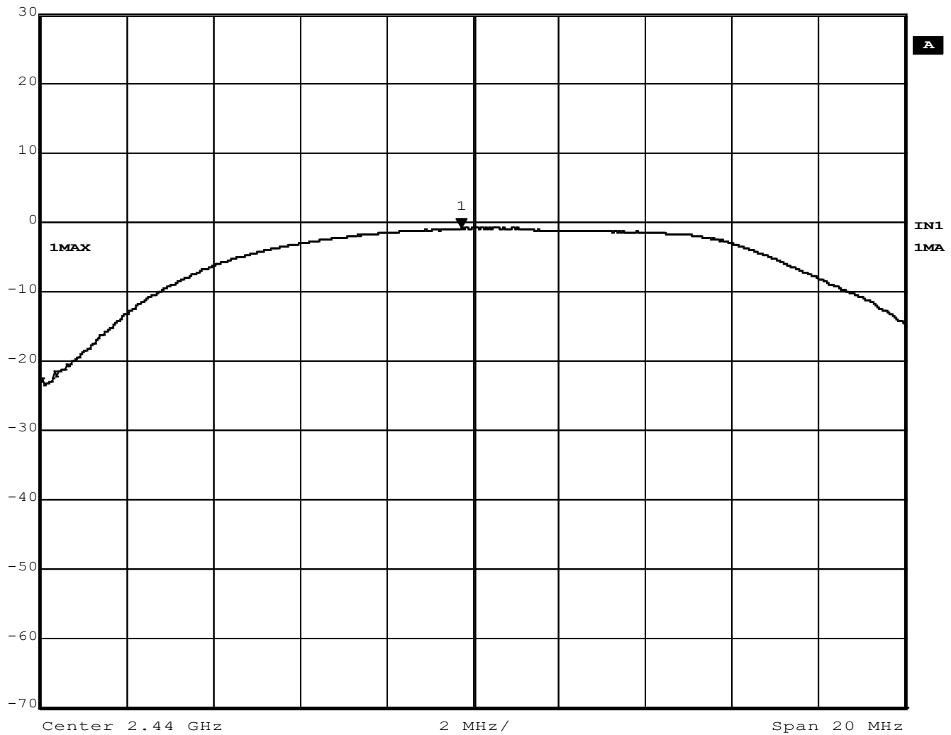
Figure 2 - Output Power, Mid Channel, GMSK
