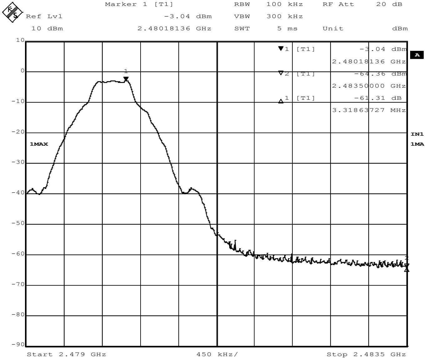
Figure 25 –Band Edge Measurement, High Channel, GFSK
