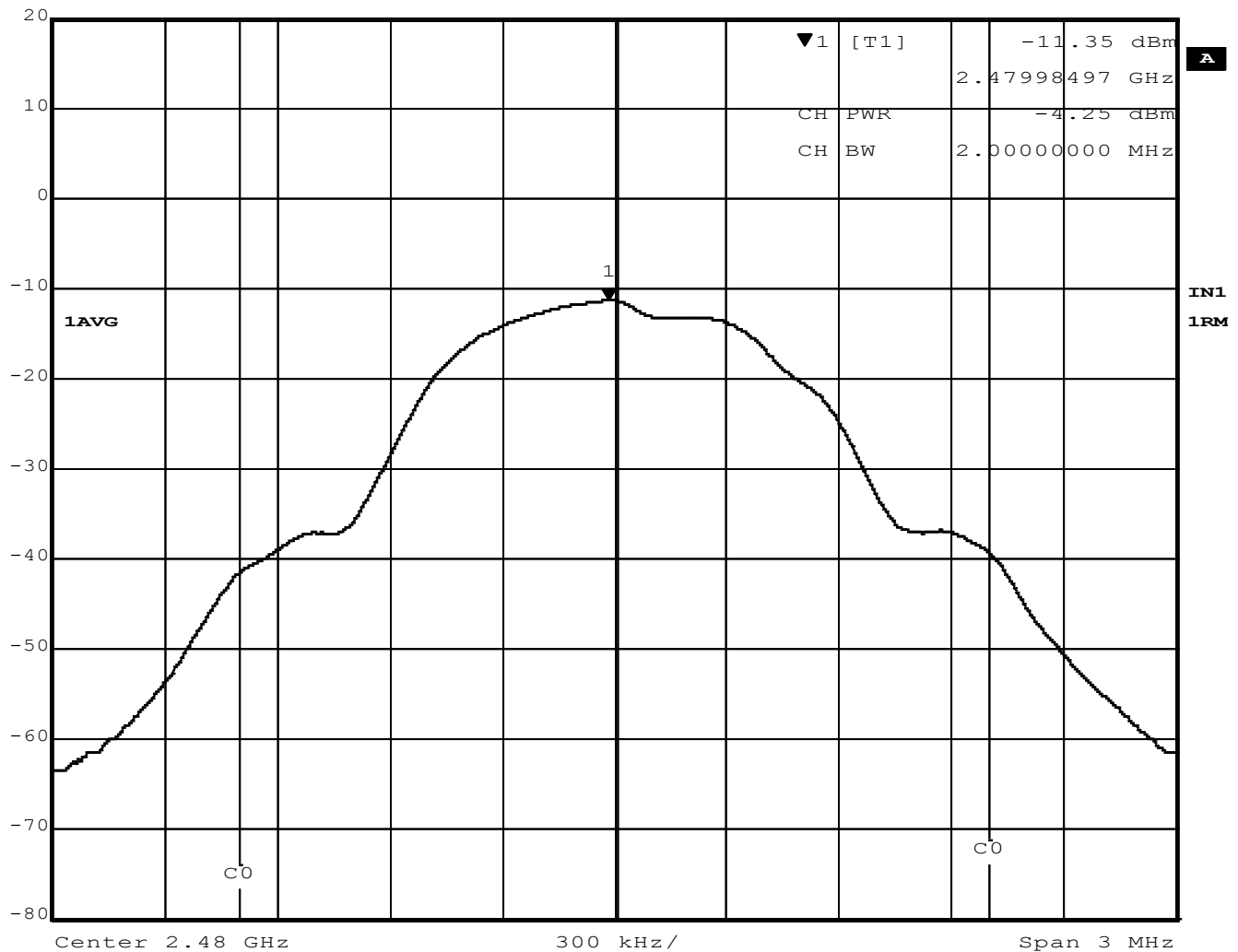
Figure 9 - Output Power, High Channel, GMSK
