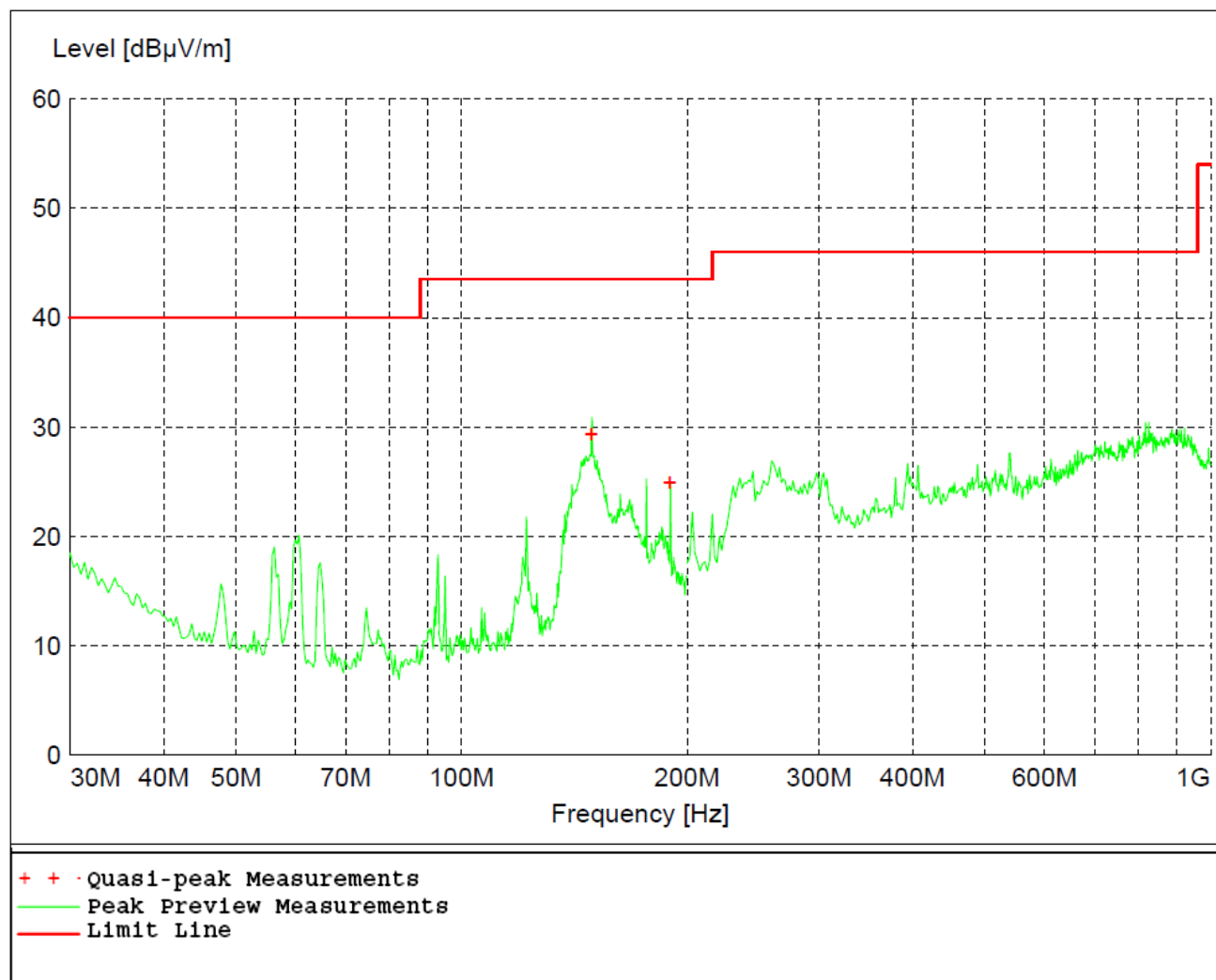
Figure 22 - Radiated Emissions Plot, GMSK
