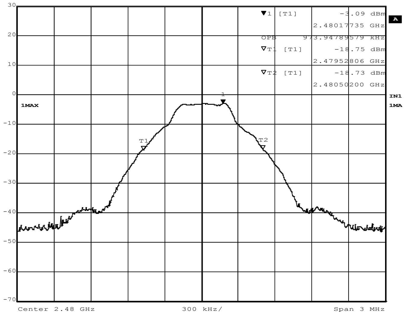
Figure 19 – Occupied Bandwidth, High Channel, GFSK
