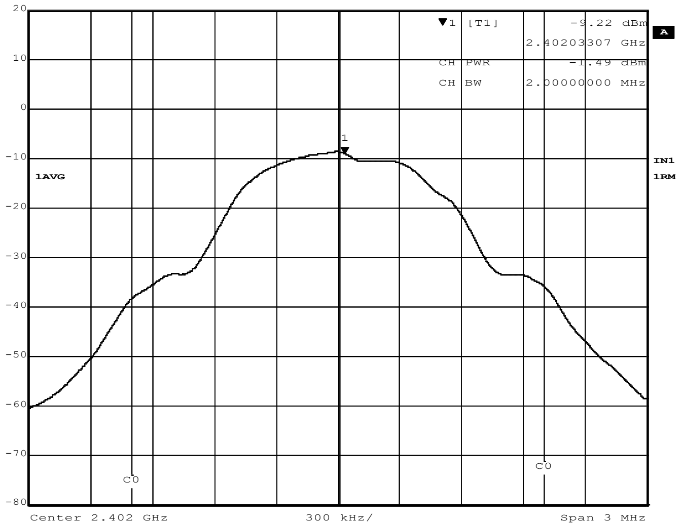
Figure 7 - Output Power, Low Channel, GMSK
