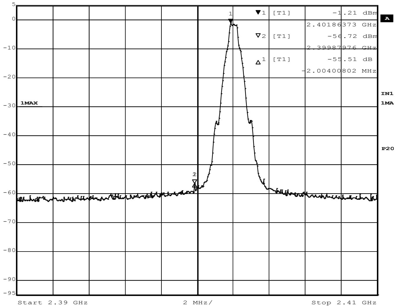
Figure 24 - Band Edge, Low Channel, GFSK
