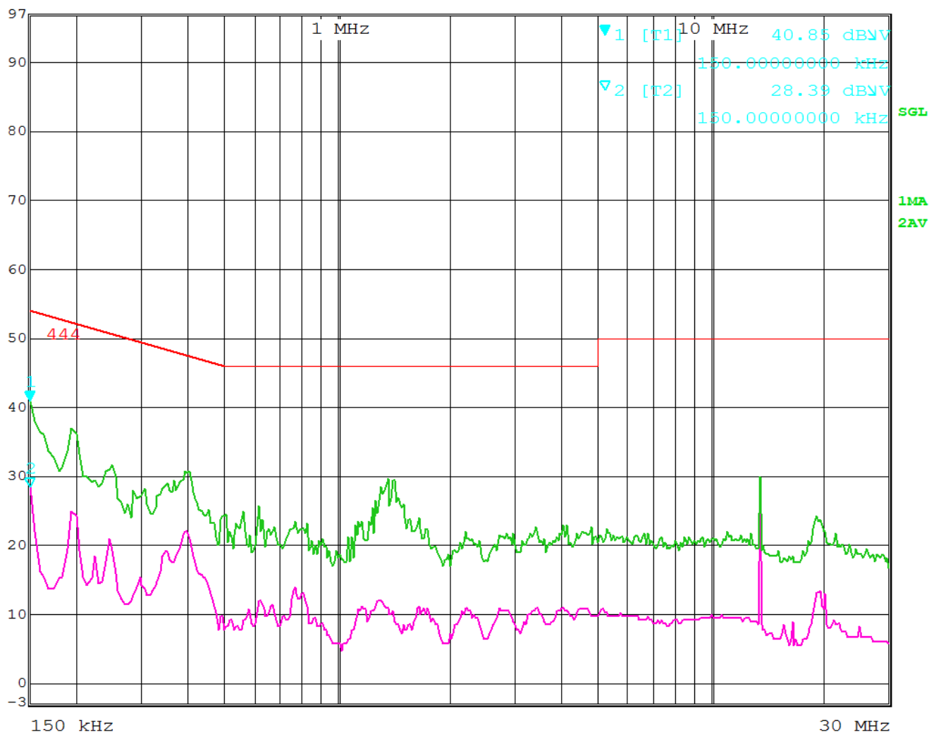
Figure 29 - Conducted Emissions Plot, Neutral
