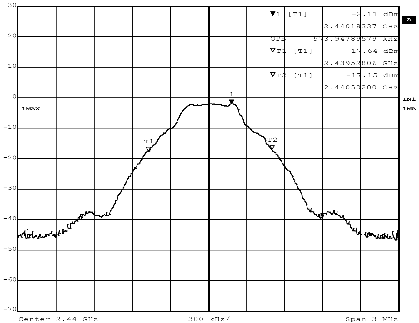
Figure 18 - Occupied Bandwidth, Mid Channel, GFSK
