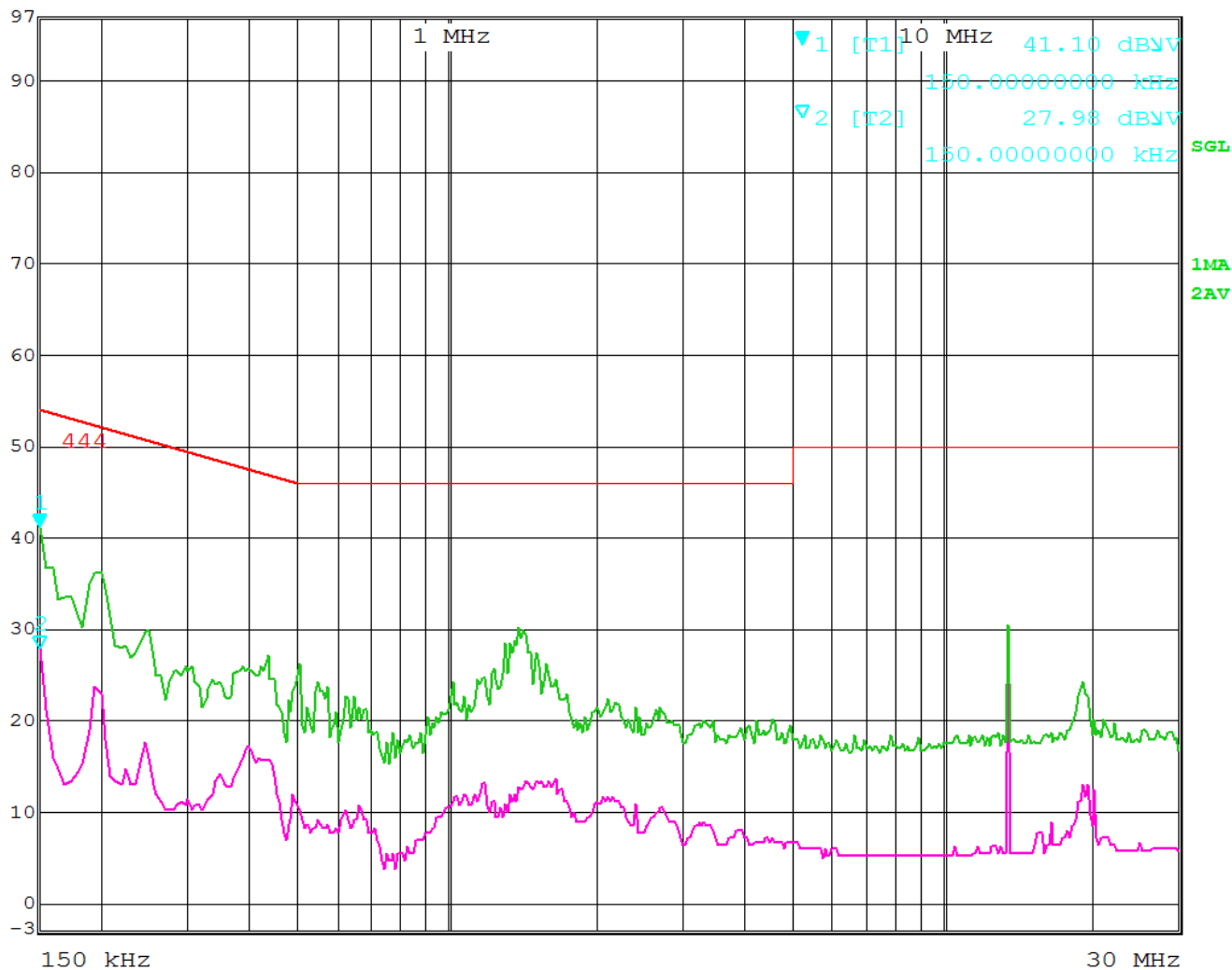
Figure 28 - Conducted Emissions Plot, Line
