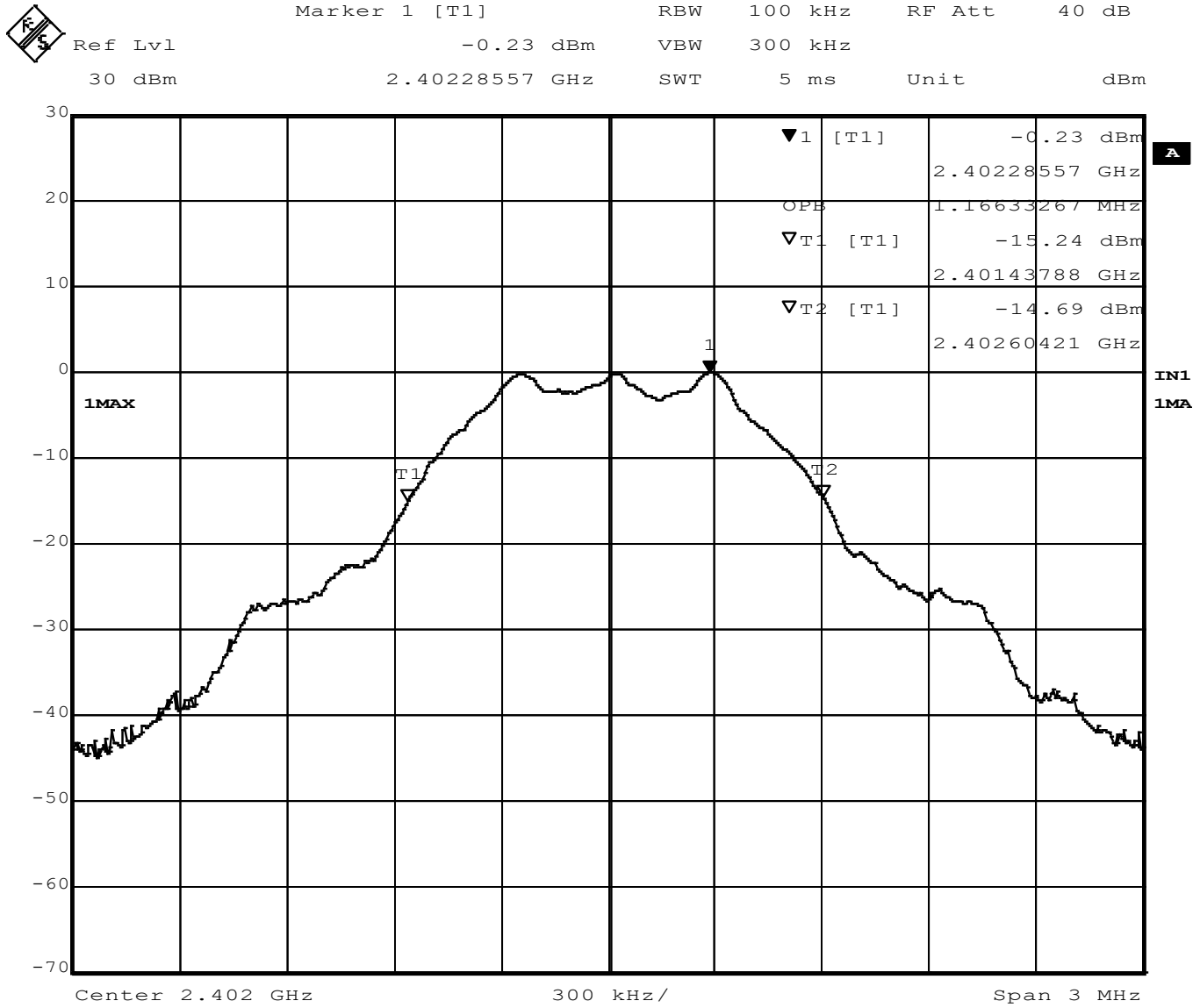
Figure 14 – Occupied Bandwidth, Low Channel, GMSK
