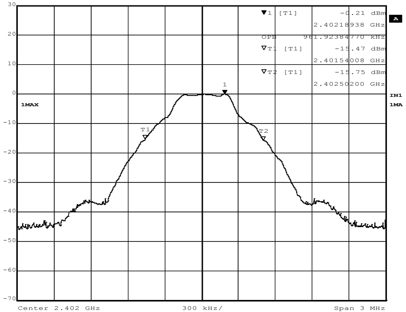
Figure 17 - Occupied Bandwidth, Low Channel, GFSK
