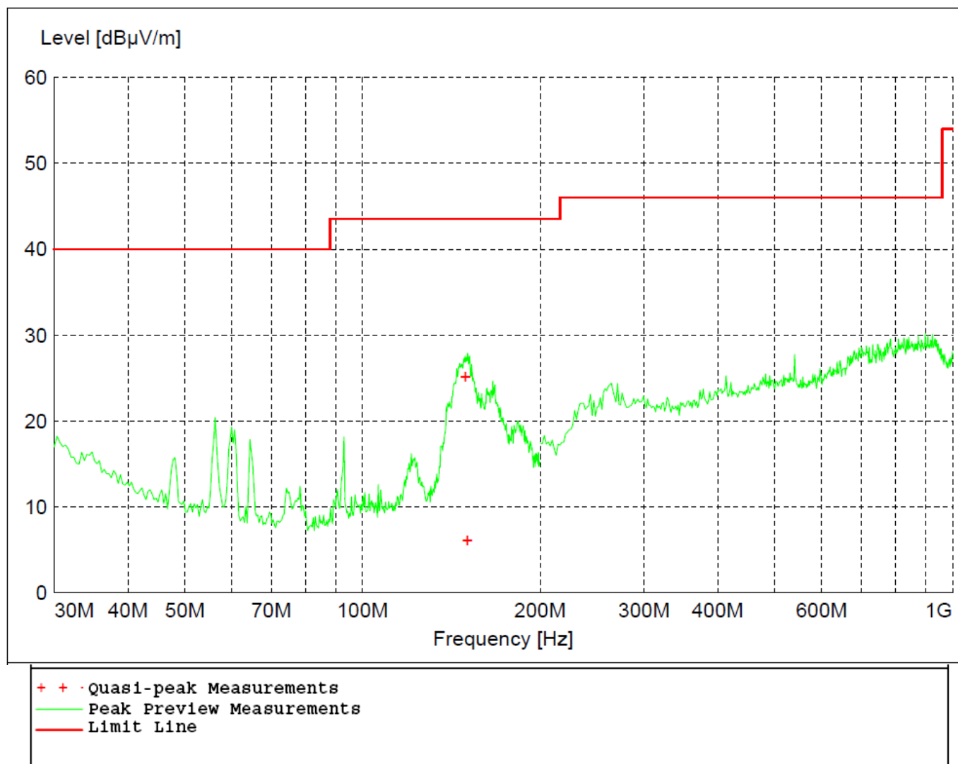
Figure 23 - Radiated Emissions Plot, GFSK
