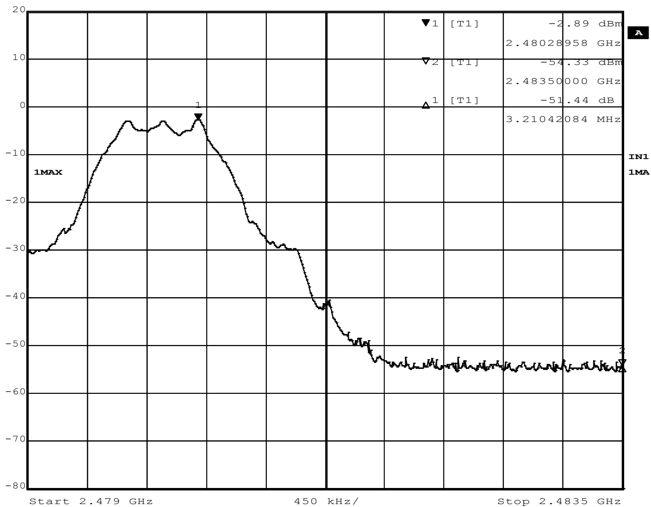
Figure 27 – Band Edge Measurement, High Channel, GMSK
