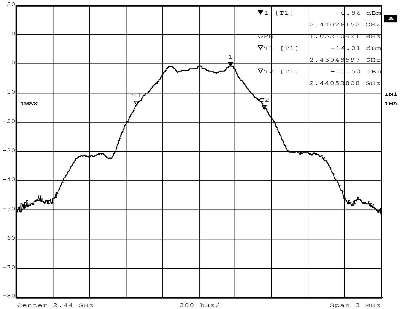
Figure 15 - Occupied Bandwidth, Mid Channel, GMSK
