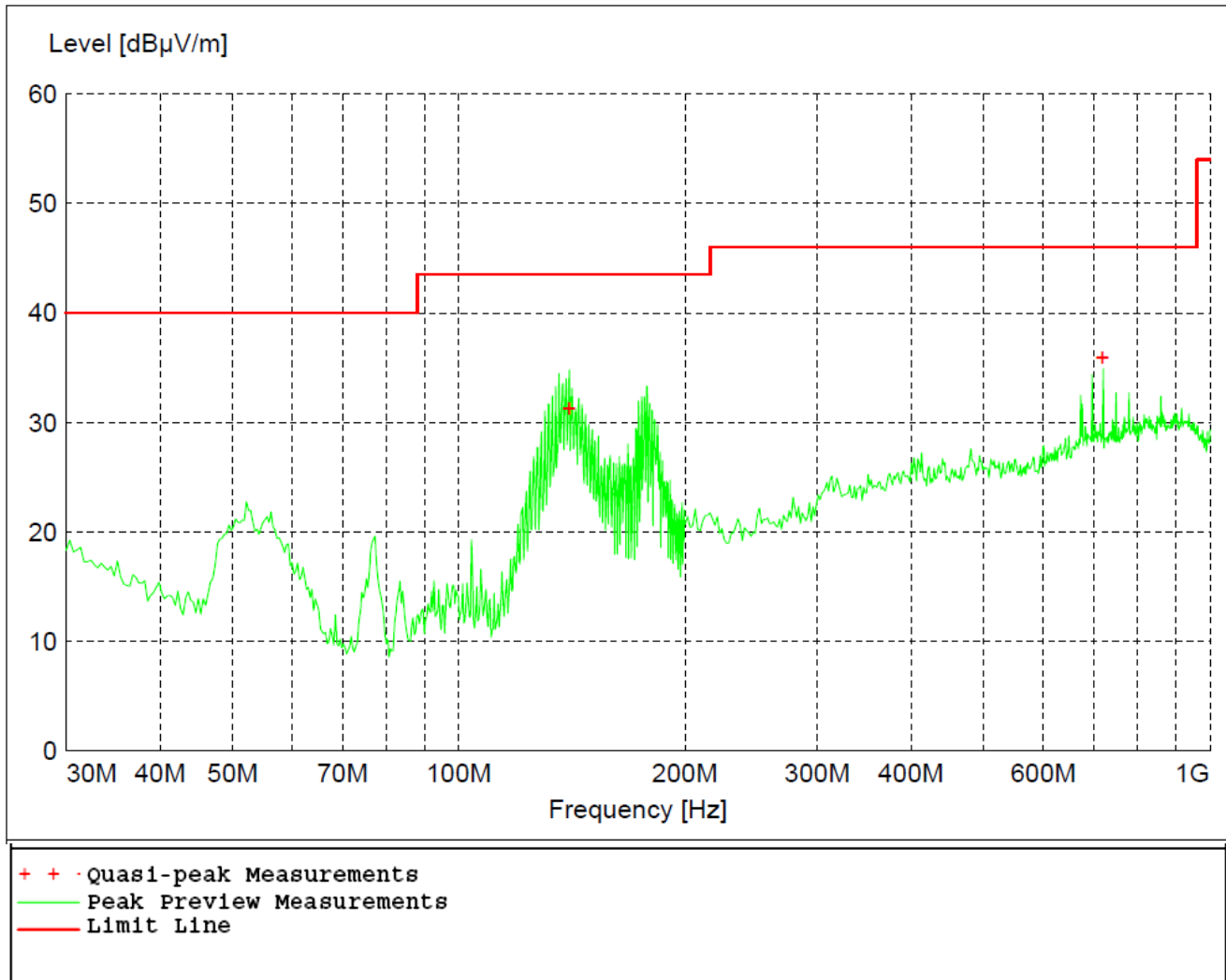
Figure 25 - Radiated Emissions Plot, Low Channel, GFSK
