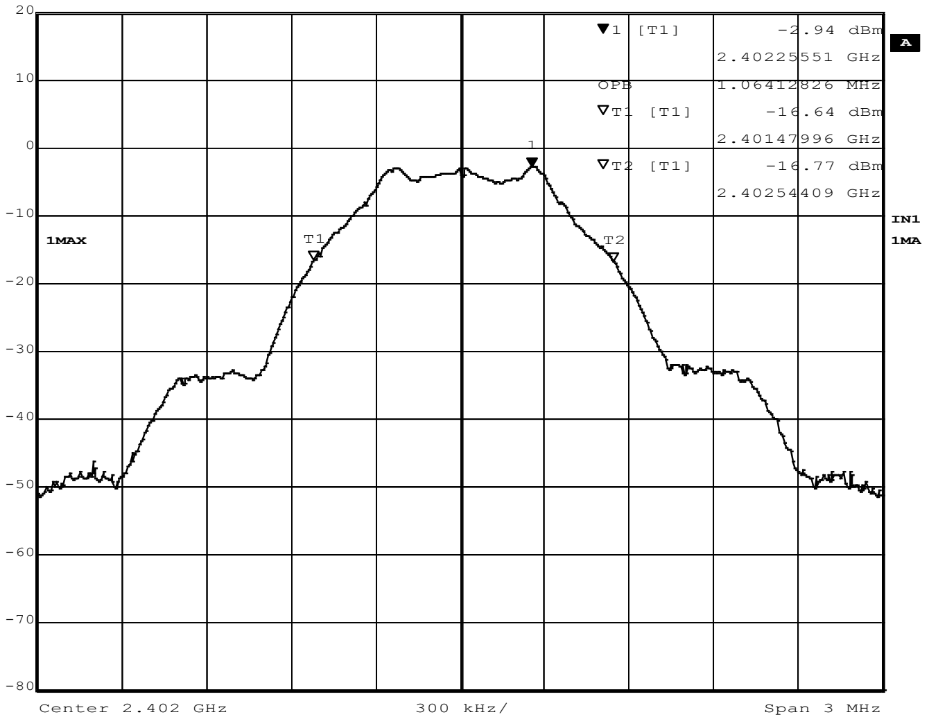
Figure 14 – Occupied Bandwidth, Low Channel, GMSK
