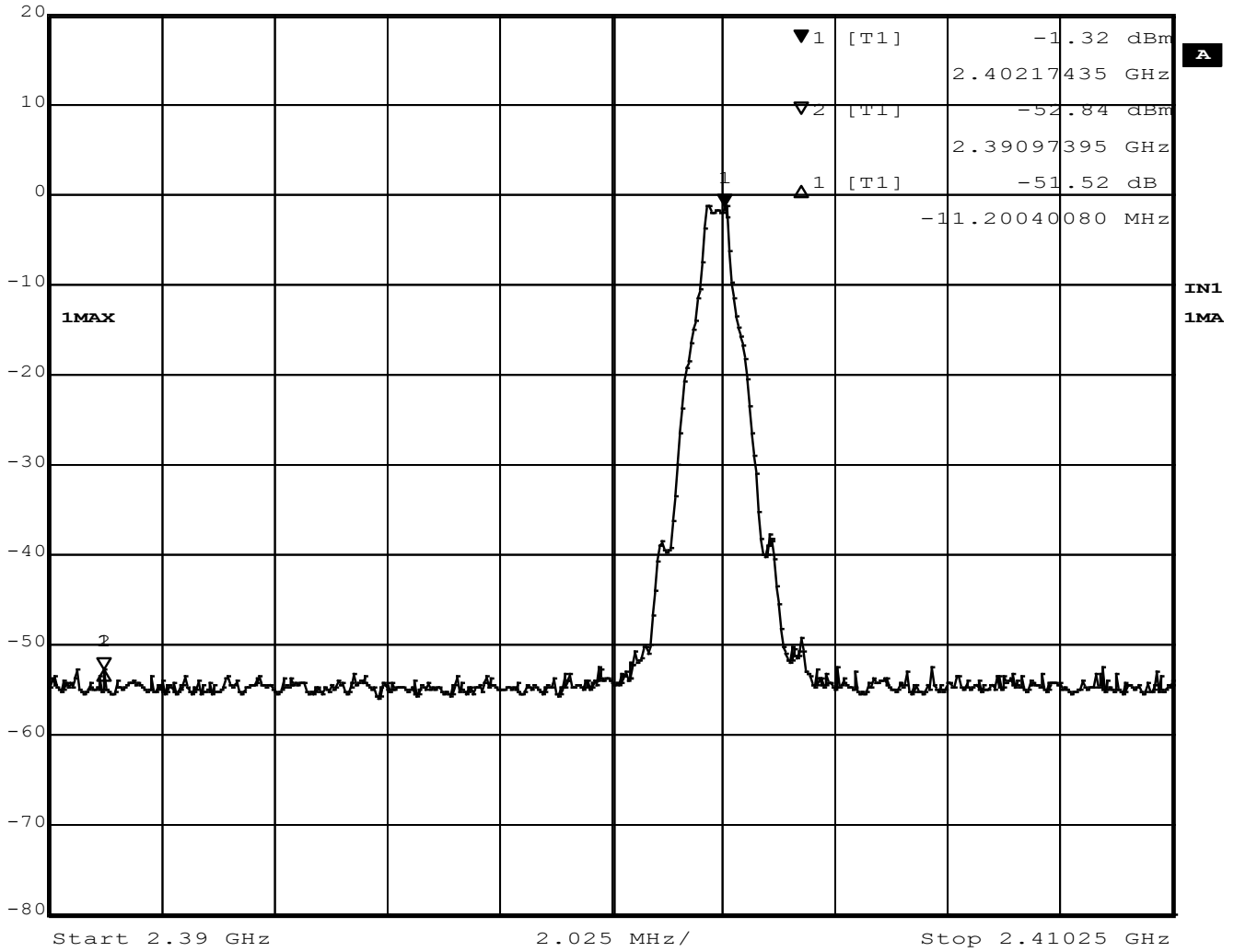
Figure 31 - Band Edge, Low Channel, Unrestricted, GFSK
