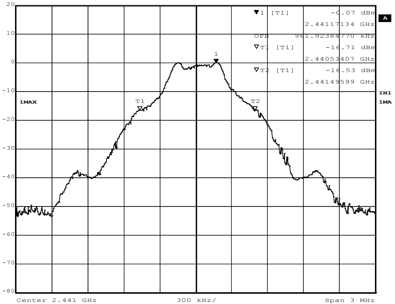
Figure 18 - Occupied Bandwidth, Mid Channel, GFSK (BT BR)
