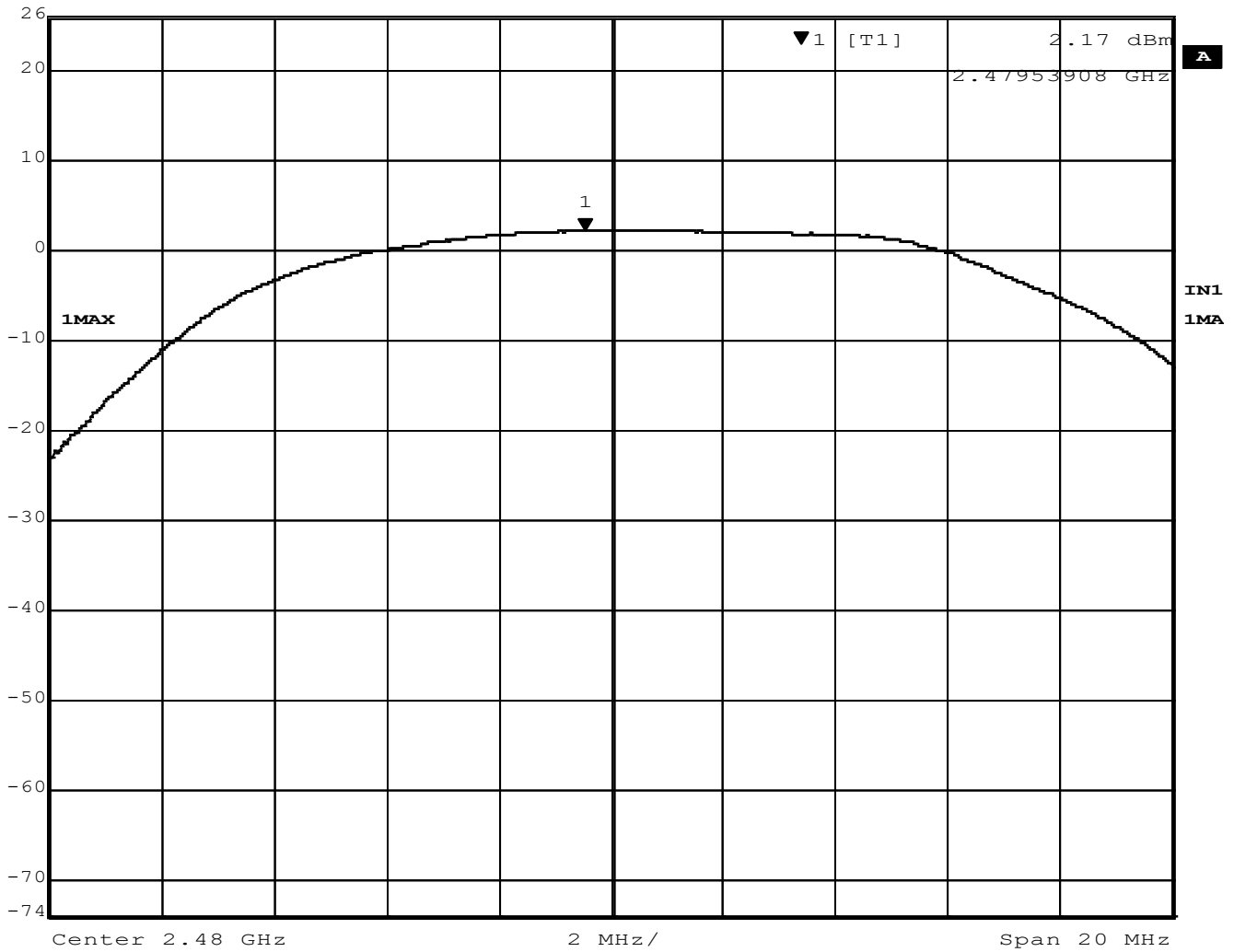
Figure 9 – Output Power, High Channel, GFSK (BT BR)
