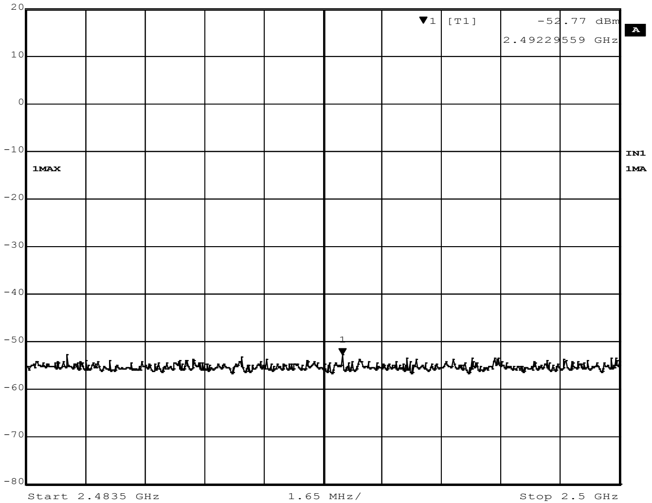
Figure 42 –Band Edge Measurement, High Channel, Restricted, GFSK (BT BR)
