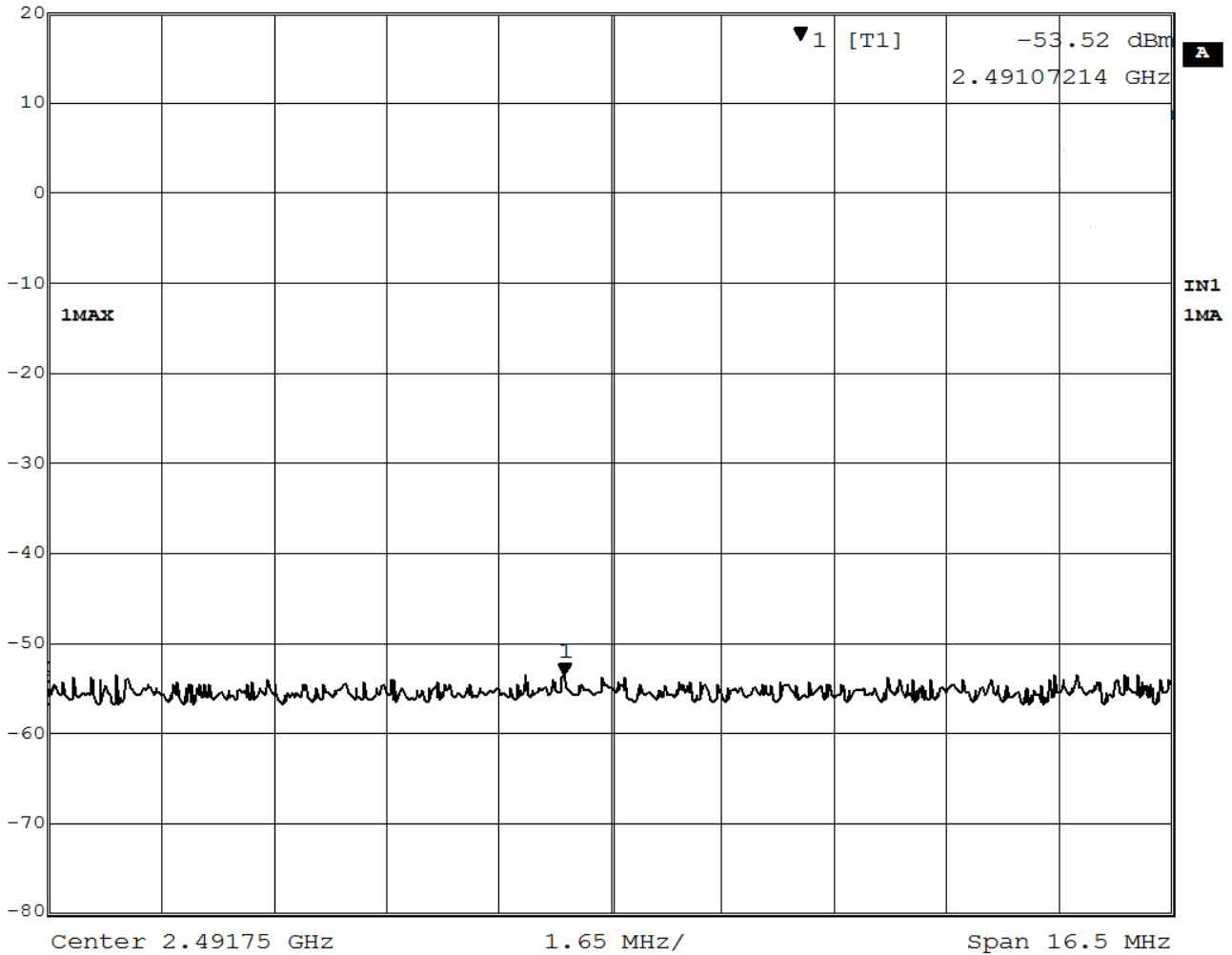
Figure 38 –Band Edge Measurement, High Channel, Restricted, GFSK
