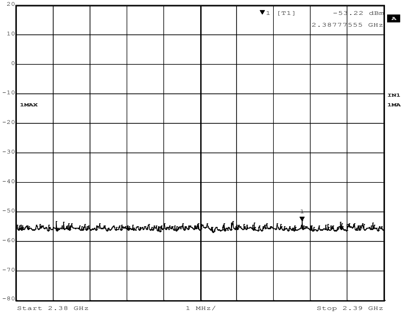
Figure 39 –Band Edge, Low Channel, Restricted, GMSK
