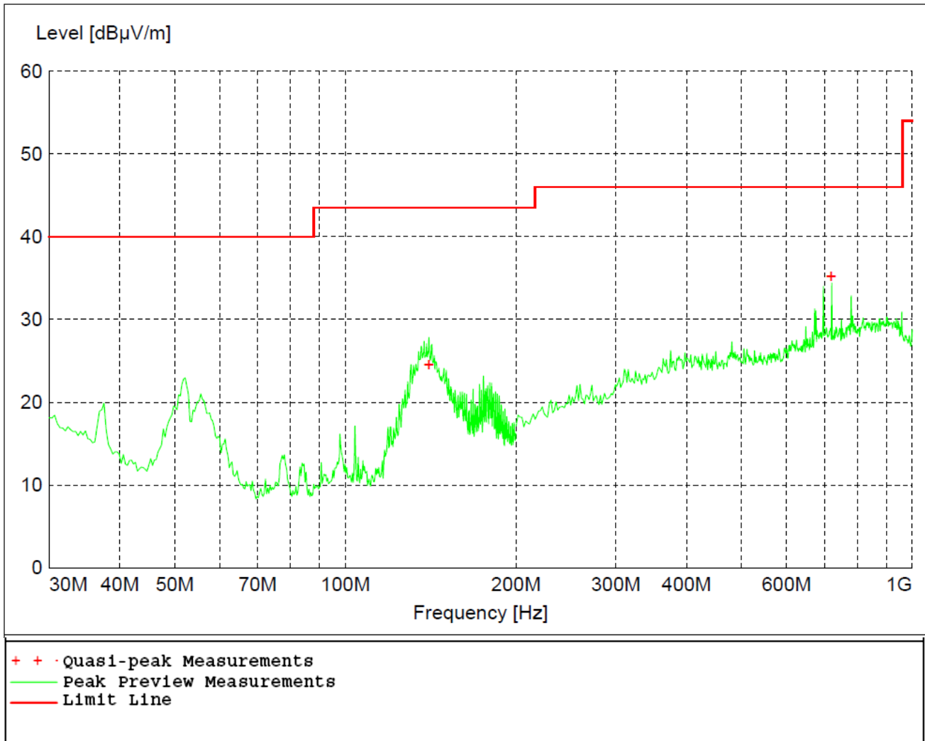
Figure 29 - Radiated Emissions Plot, Mid Channel, GFSK (BT BR)
