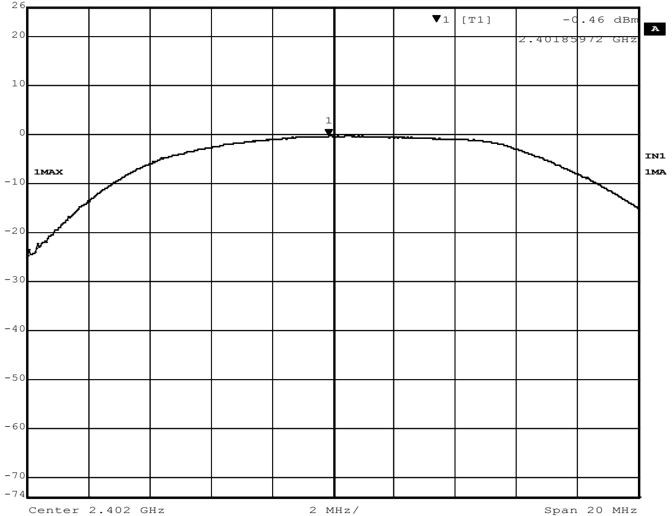
Figure 1 – Output Power, Low Channel, GFSK
