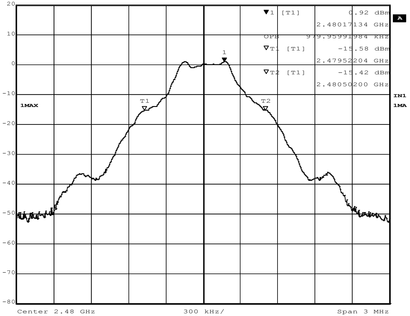
Figure 19 - Occupied Bandwidth, High Channel, GFSK (BT BR)
