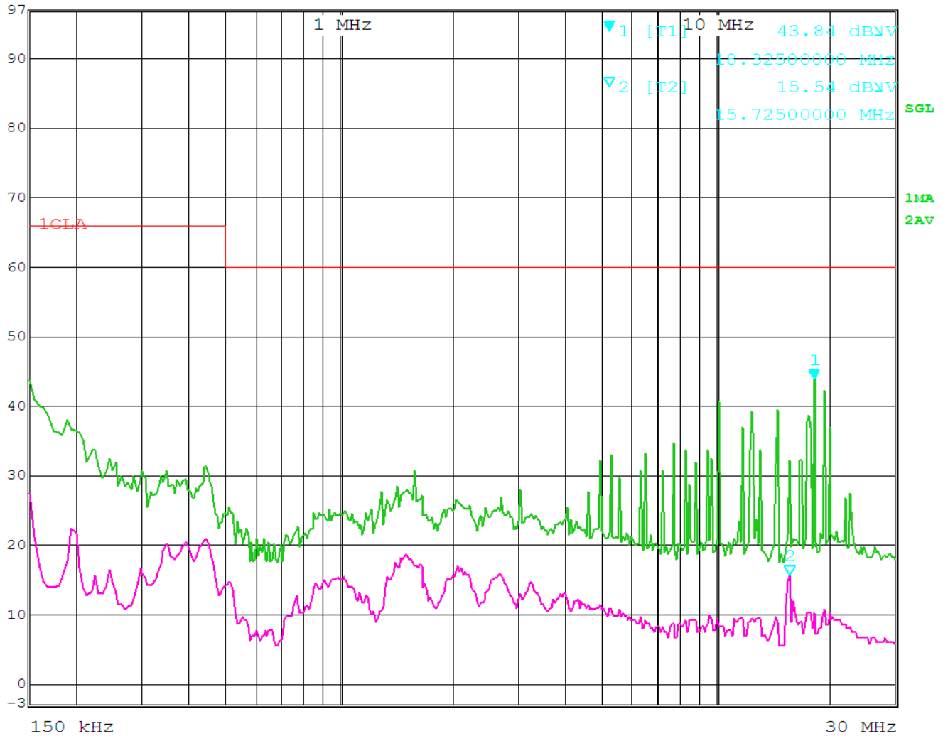
Figure 44 - Conducted Emissions Plot, N-F
