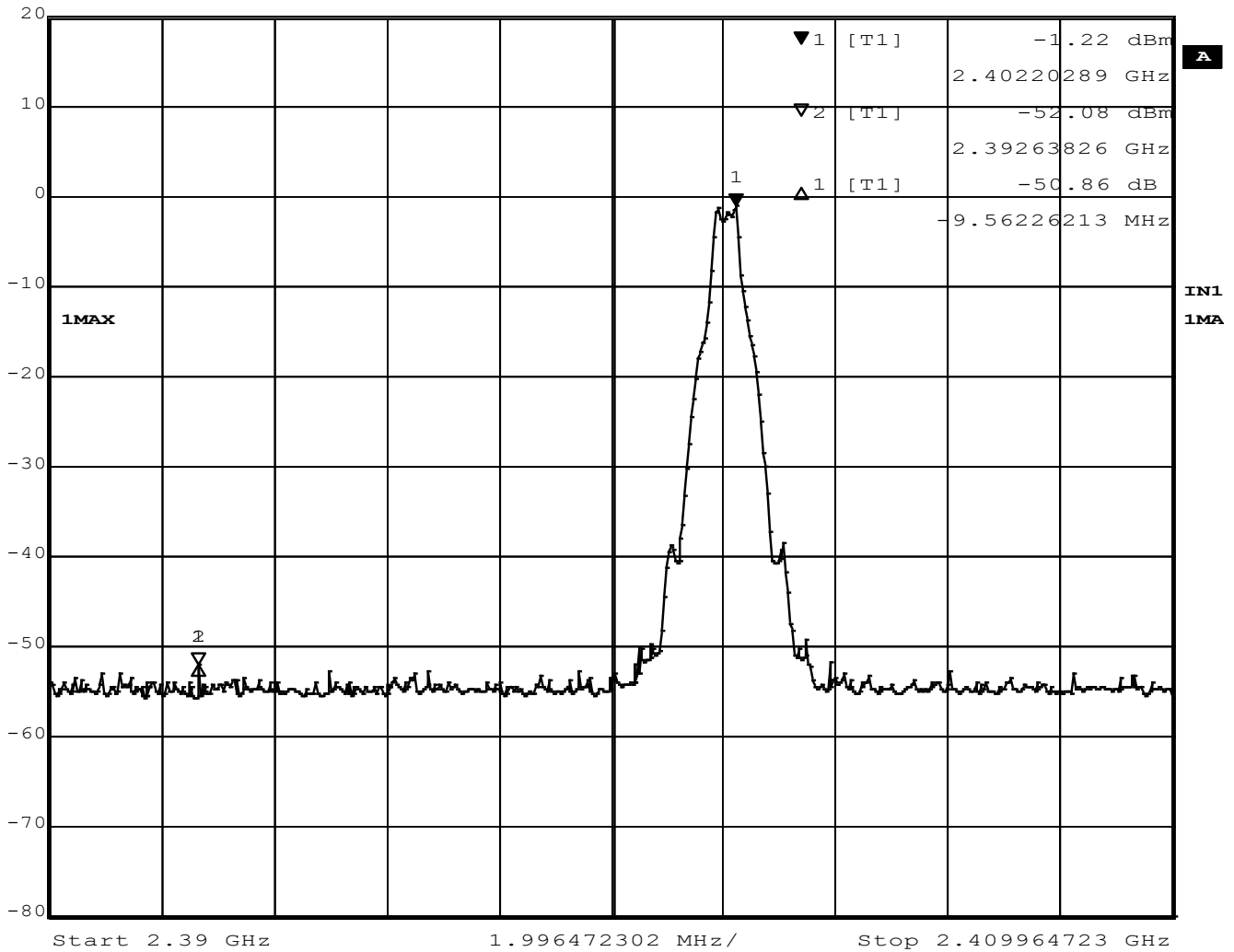
Figure 35 - Band Edge, Low Channel, Unrestricted, GFSK (BT BR)
