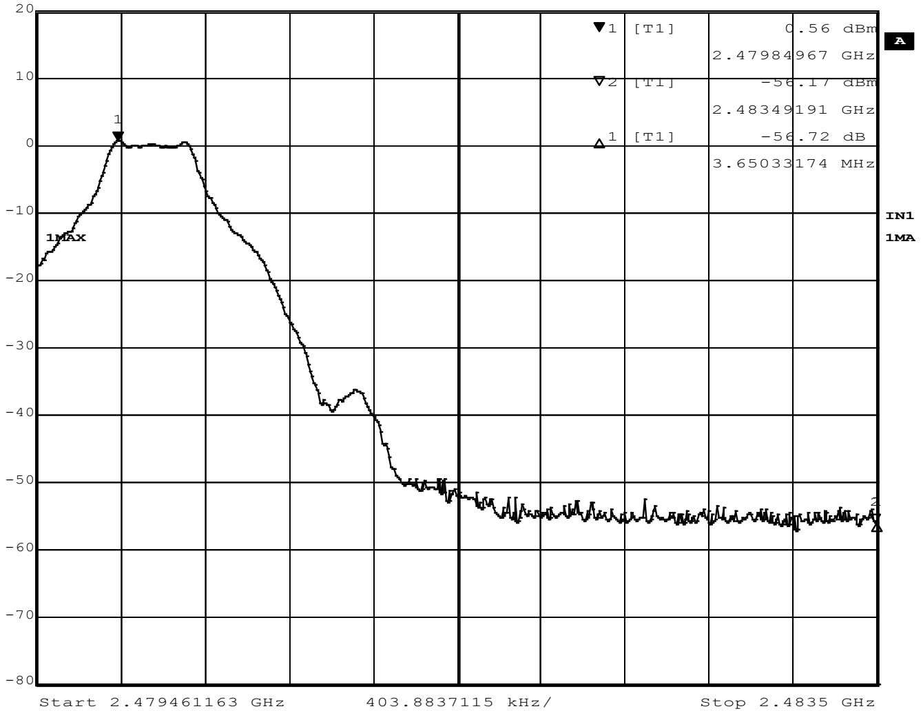
Figure 32 –Band Edge Measurement, High Channel, Unrestricted, GFSK
