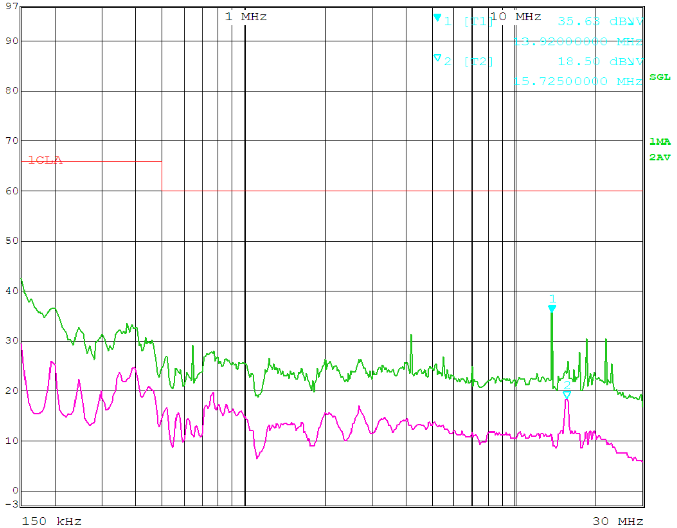
Figure 43 - Conducted Emissions Plot, L-F
