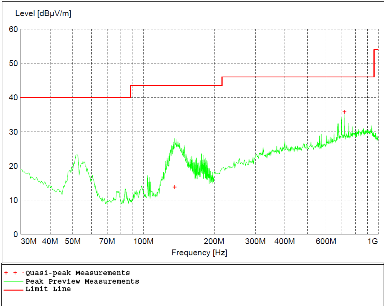
Figure 27 - Radiated Emissions Plot, High Channel, GFSK
