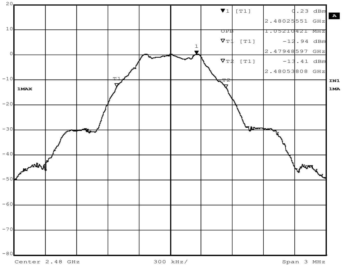
Figure 16 - Occupied Bandwidth, High Channel, GMSK
