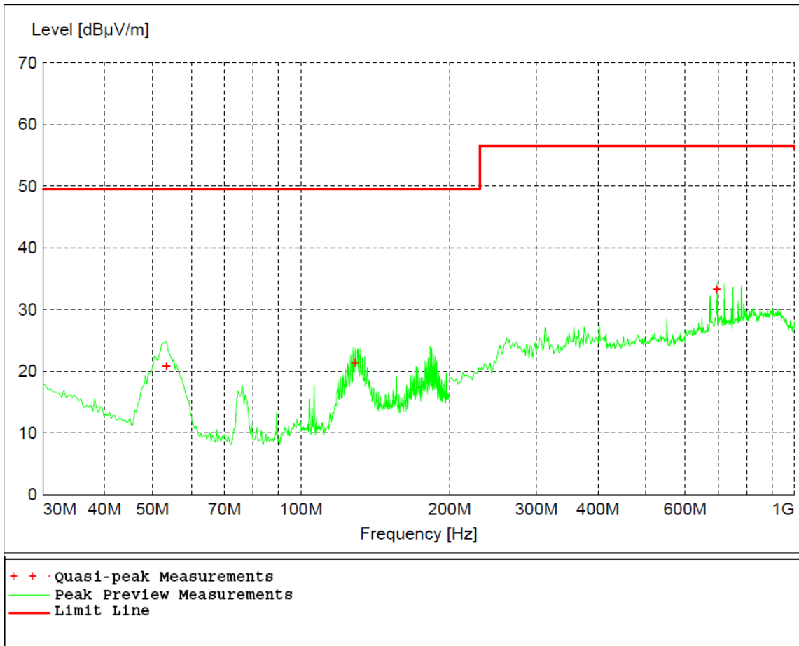
Figure 28 - Radiated Emissions Plot, Low Channel, GFSK (BT BR)
