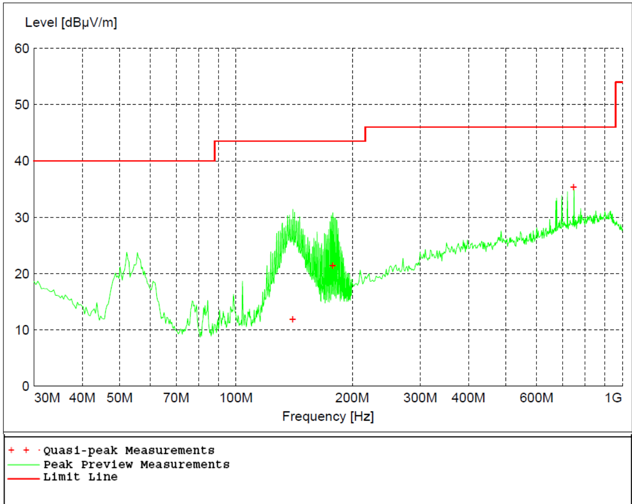
Figure 26 - Radiated Emissions Plot, Mid Channel, GFSK
