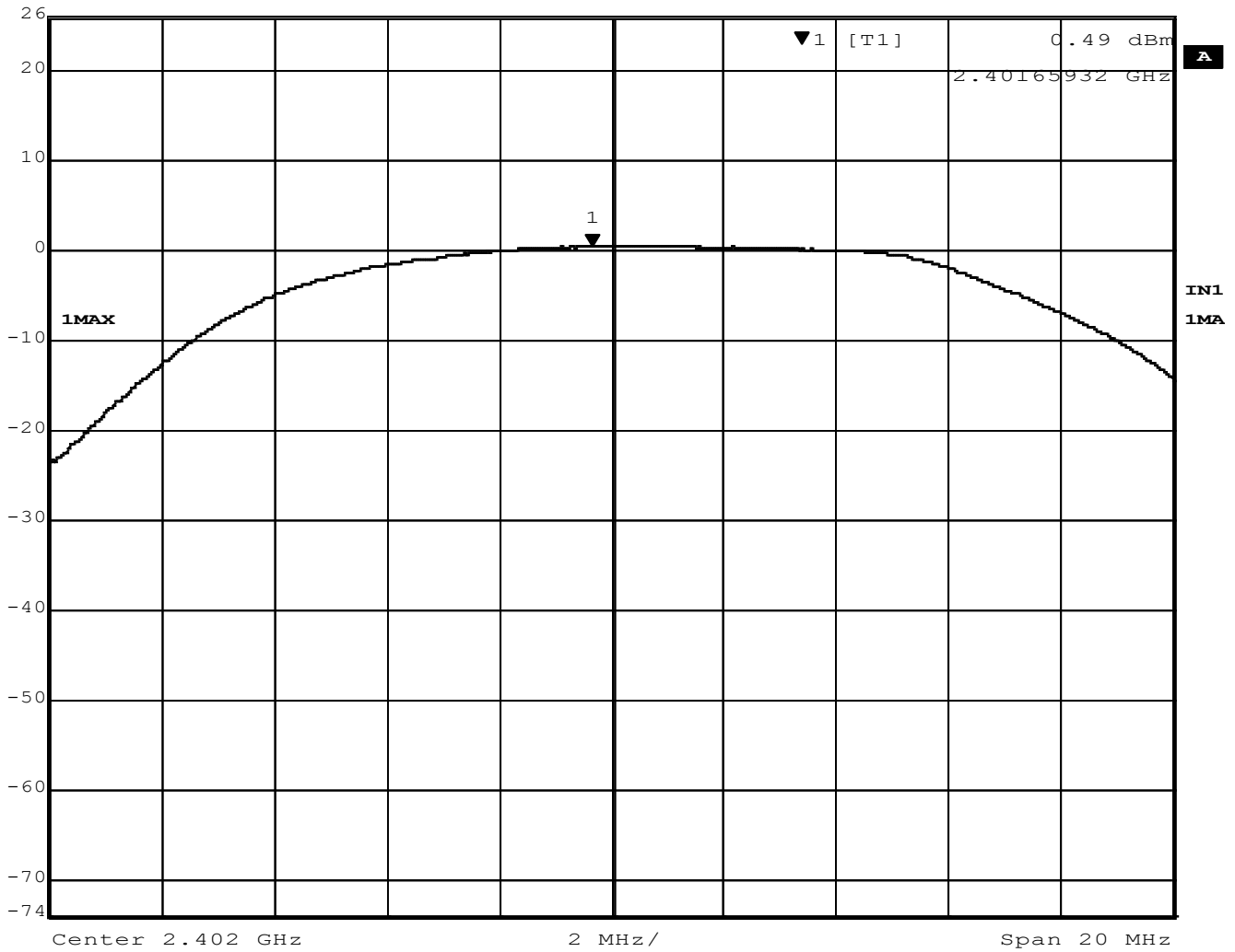
Figure 7 – Output Power, Low Channel, GFSK (BT BR)
