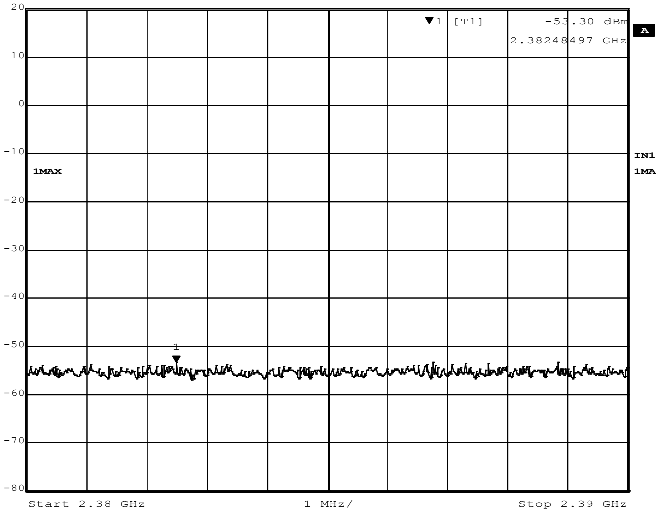
Figure 41 - Band Edge, Low Channel, Restricted, GFSK (BT BR)
