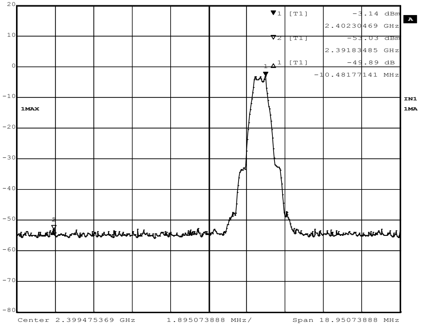
Figure 33 –Band Edge, Low Channel, Unrestricted, GMSK
