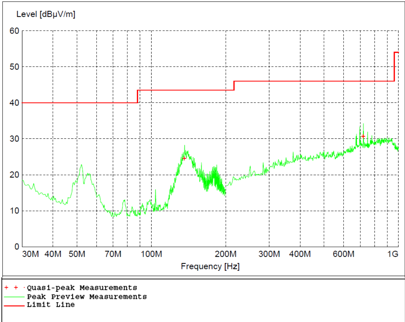
Figure 30 - Radiated Emissions Plot, High Channel, GFSK (BT BR)
