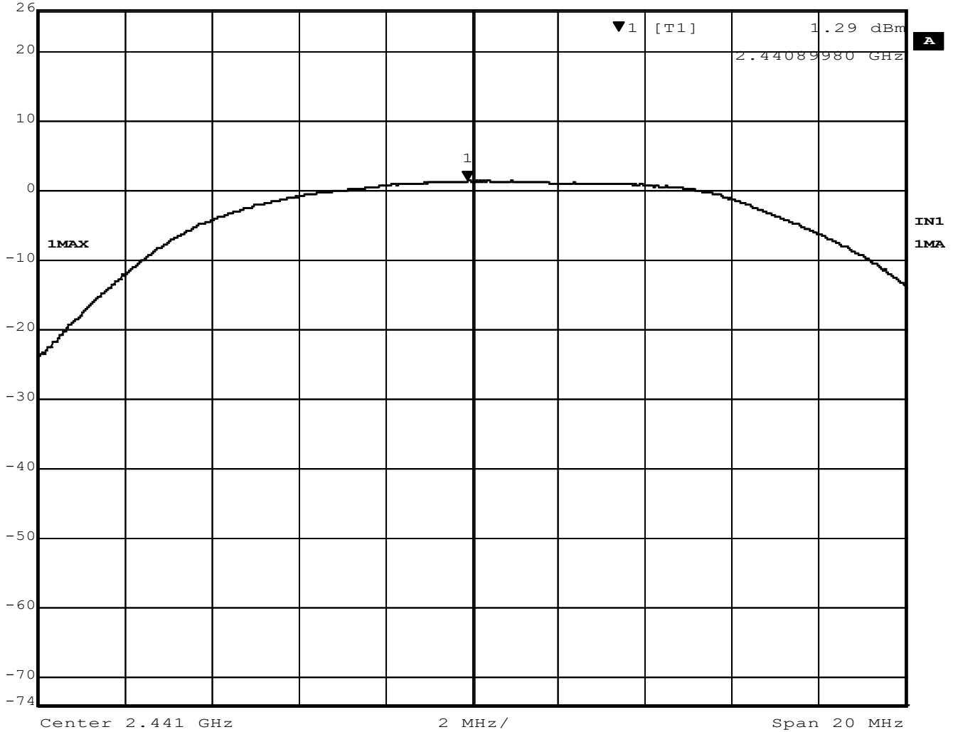
Figure 8 – Output Power, Mid Channel, GFSK (BT BR)
