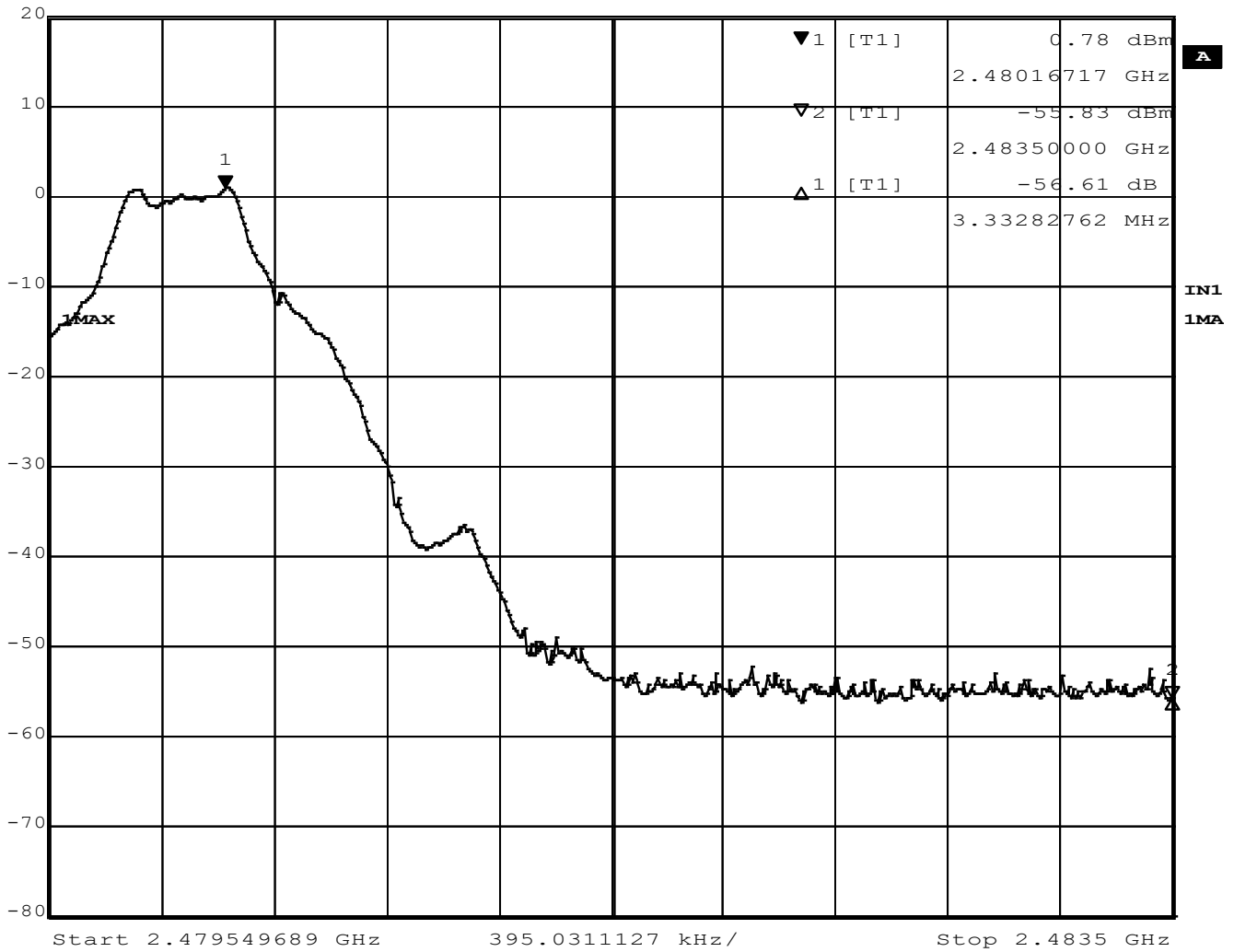
Figure 36 –Band Edge Measurement, High Channel, Unrestricted, GFSK (BT BR)
