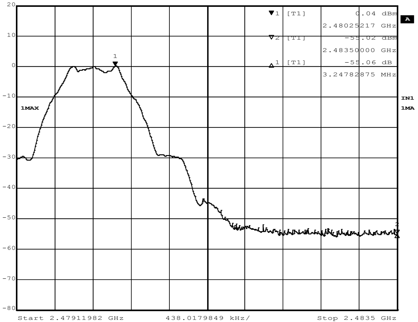
Figure 34 – Band Edge Measurement, High Channel, Unrestricted, GMSK
