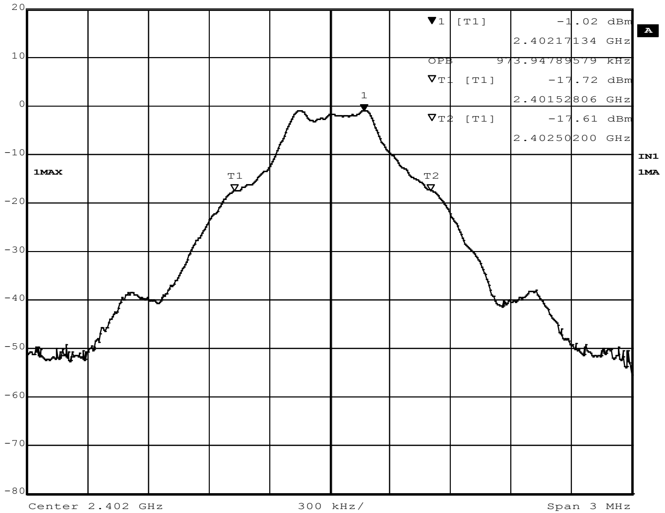
Figure 17 - Occupied Bandwidth, Low Channel, GFSK (BT BR)
