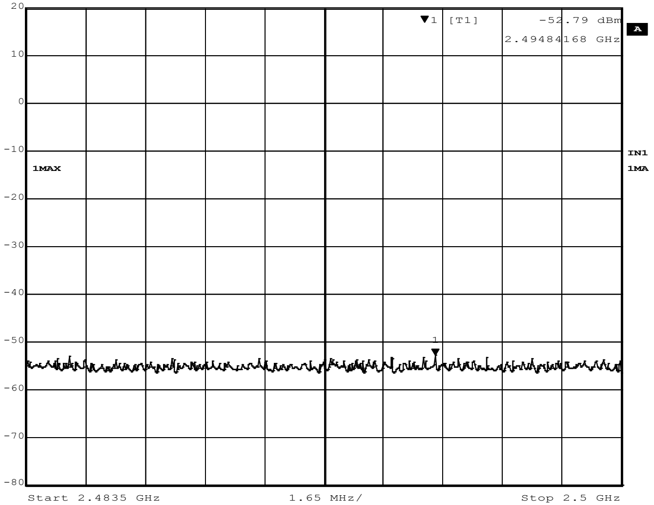
Figure 40 – Band Edge Measurement, High Channel, Restricted, GMSK
