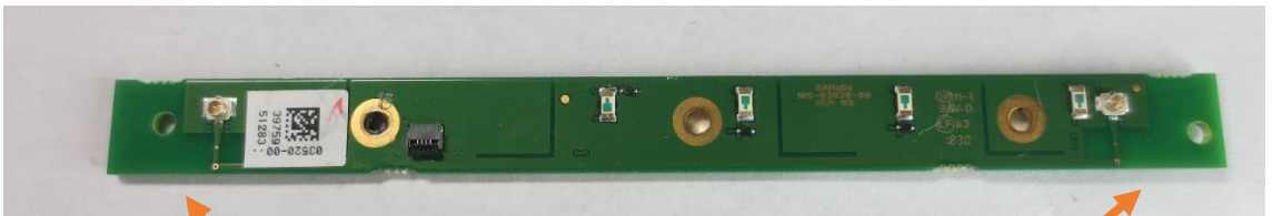
Printed board antennas on Keypad Board edges Left in picture is for L subsystem, Right for A subsystem
