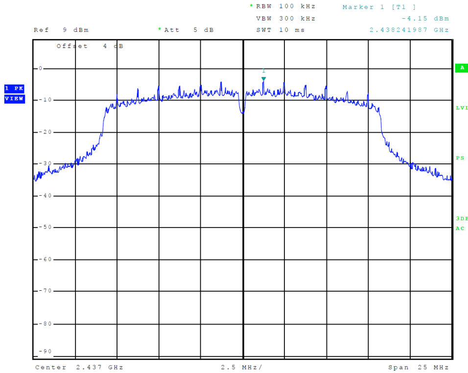
Figure 33 Plot of Transmitter Power Spectral Density (L6 - 802.11g)
