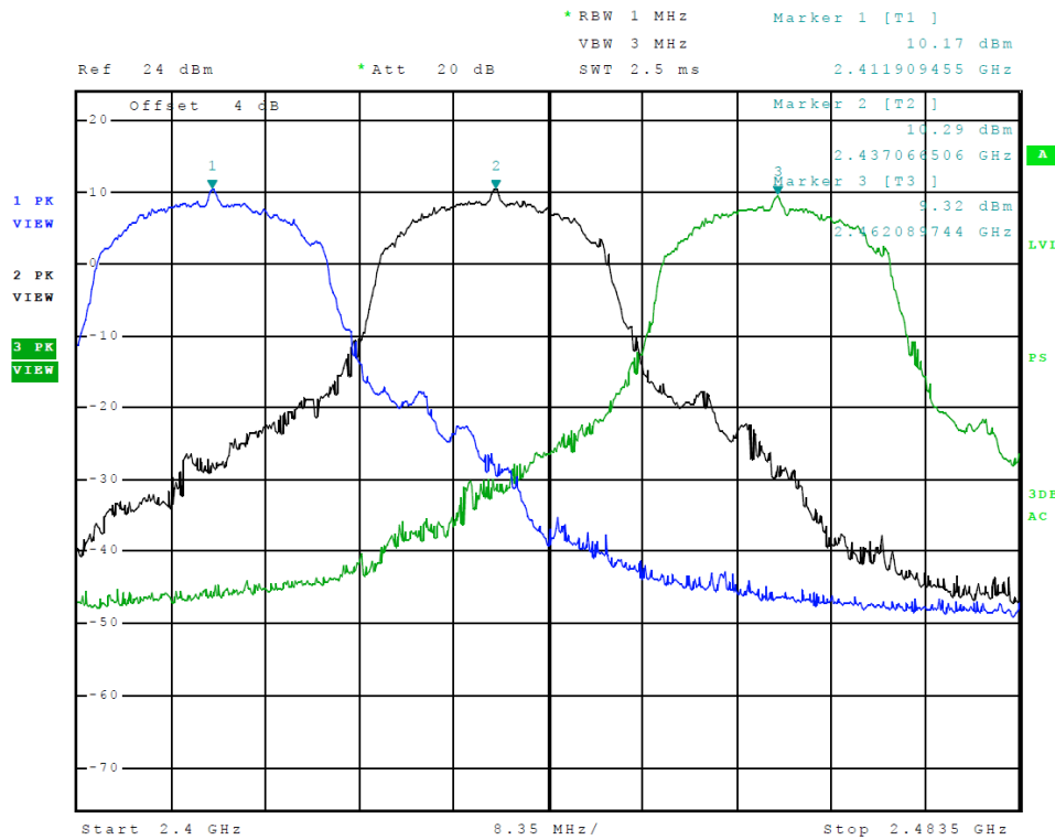
Figure 3 Plot of Transmitter Emissions in Operational Frequency (A7 - 802.11n)
