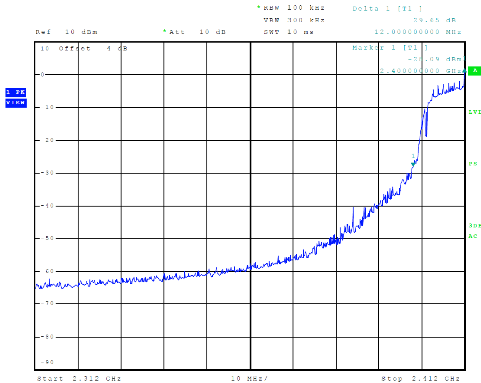
Figure 6 Plot of Lower Band Edge (A7 - 802.11n)
