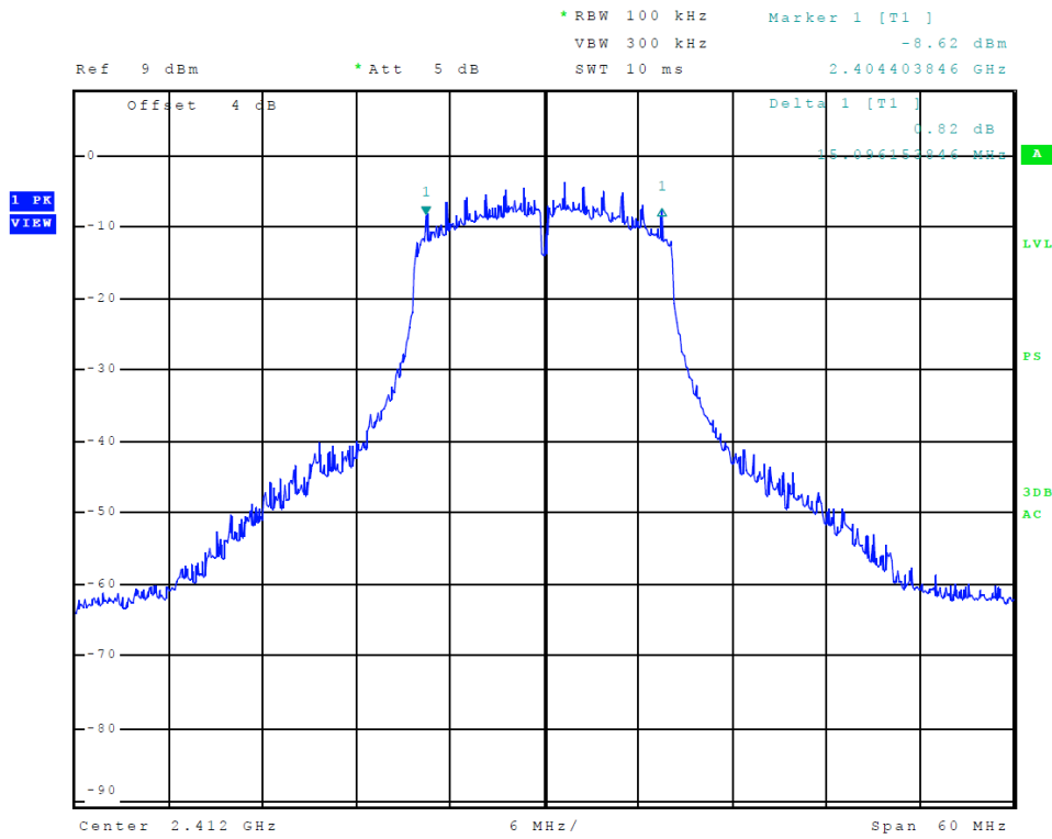
Figure 31 Plot of Transmitter 6-dB Occupied Bandwidth (L6 - 802.11g)
