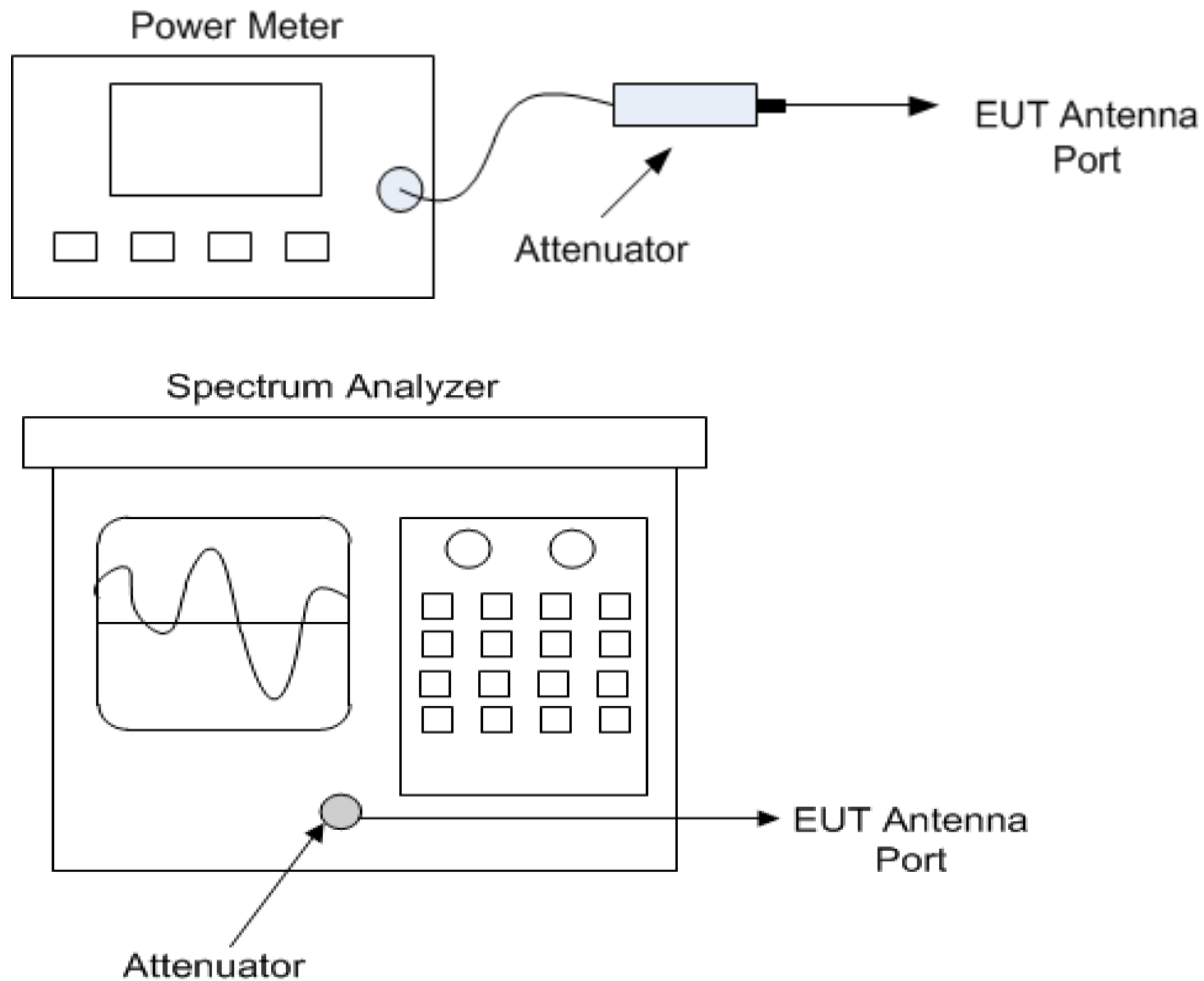
Diagram 3 Test arrangement for Antenna Port Conducted emissions
