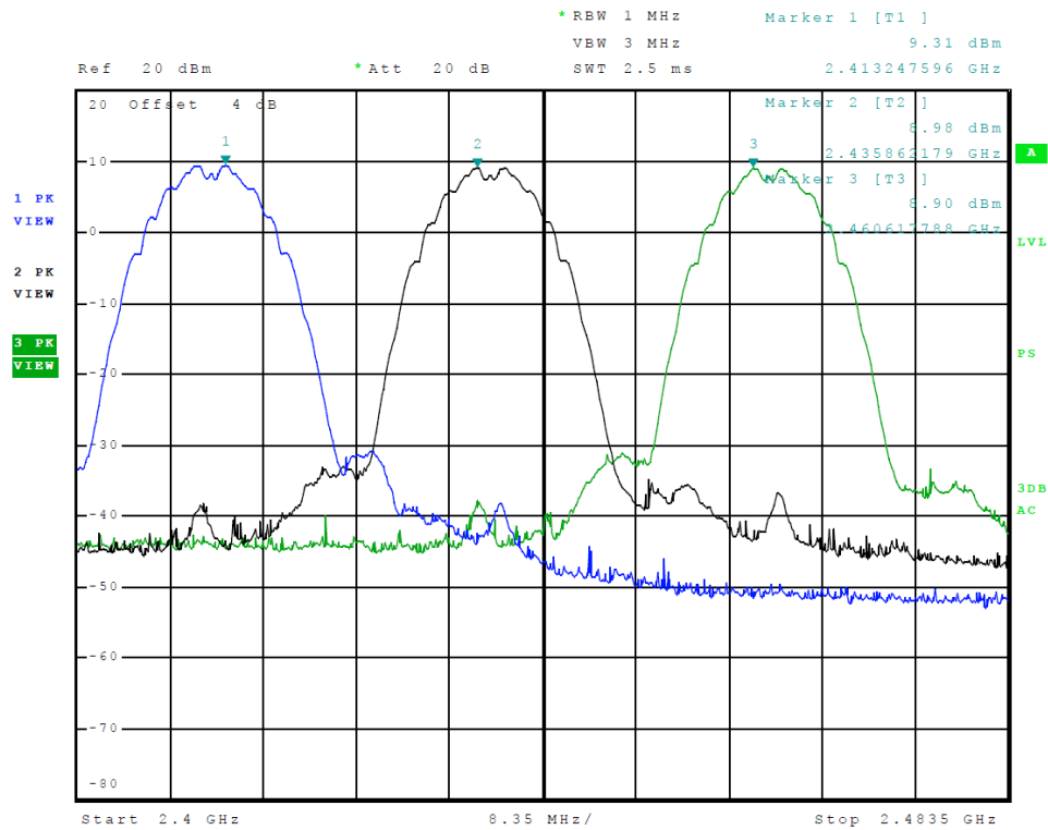
Figure 1 Plot of Transmitter Emissions in Operational Frequency (A5 - 802.11b)
