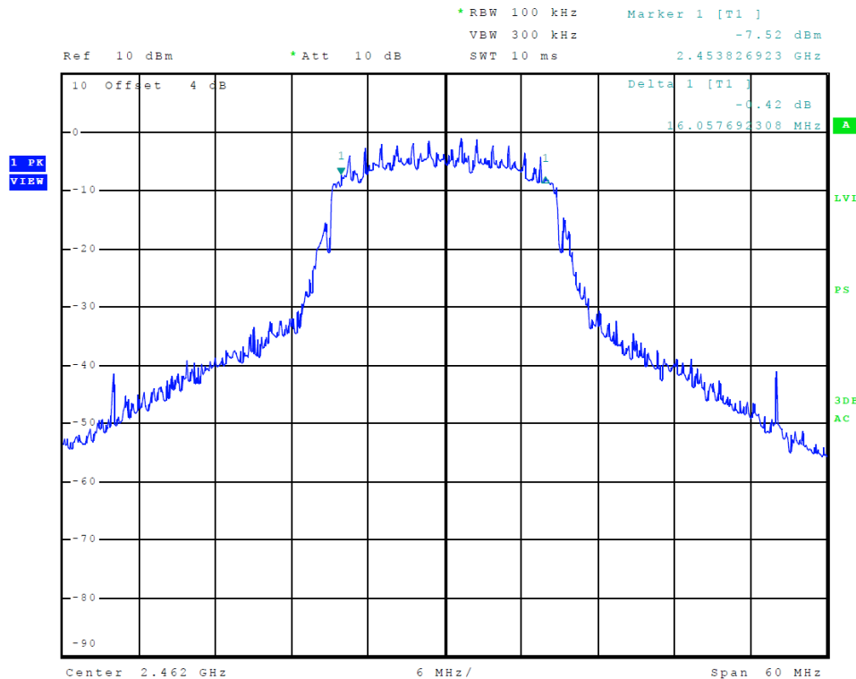
Figure 16 Plot of Transmitter 6-dB Occupied Bandwidth (A7 - 802.11n)
