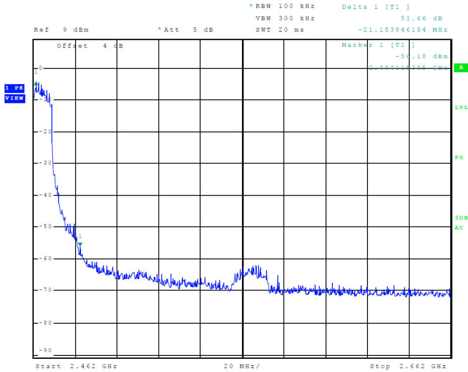
Figure 27 Plot of Upper Band Edge (L7 - 802.11n)
