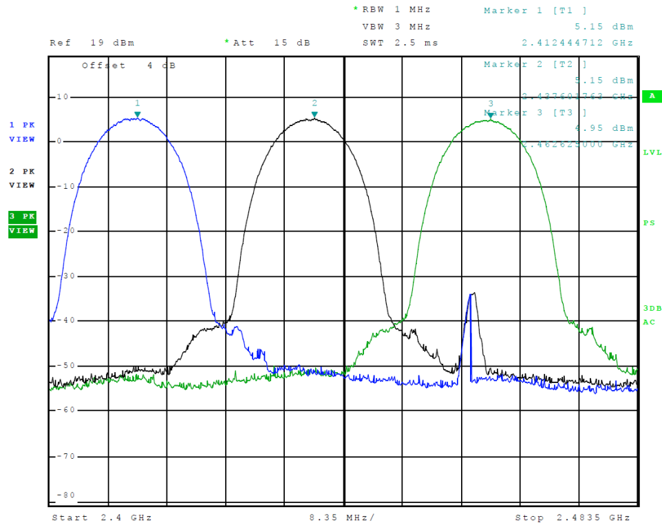
Figure 19 Plot of Transmitter Emissions in Operational Frequency (L5 - 802.11b)
