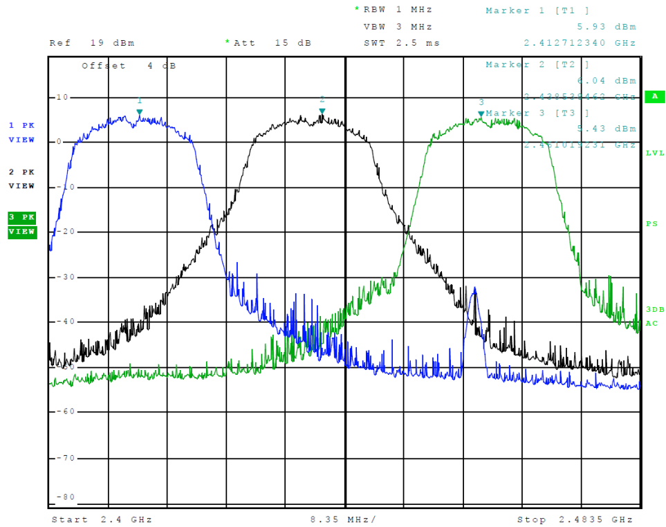
Figure 21 Plot of Transmitter Emissions in Operational Frequency (L7 - 802.11n)
