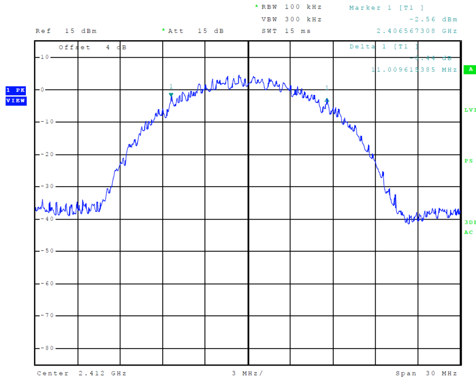
Figure 10 Plot of Transmitter 6-dB Occupied Bandwidth (A5 - 802.11b)
