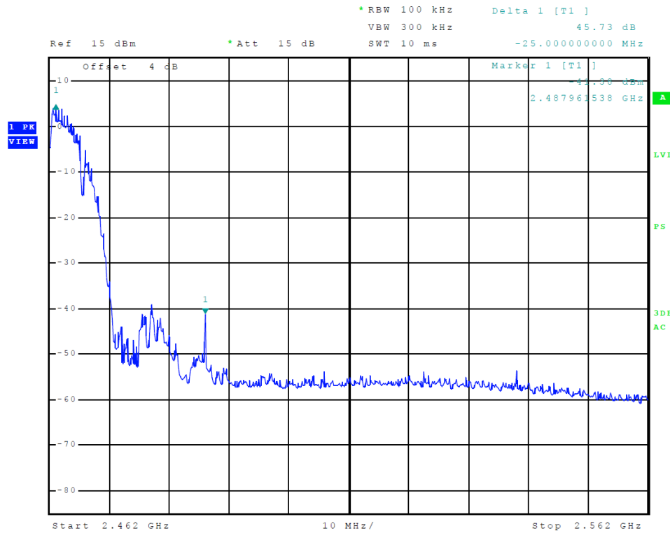
Figure 7 Plot of Upper Band Edge (A5 - 802.11b)
