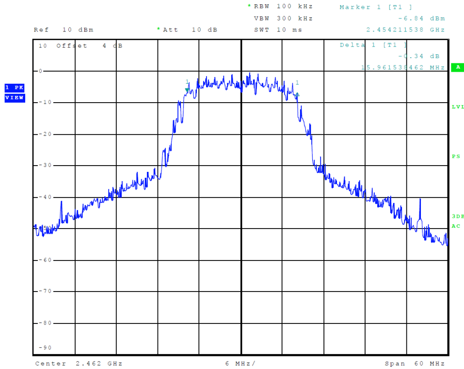
Figure 13 Plot of Transmitter 6-dB Occupied Bandwidth (A6 - 802.11g)
