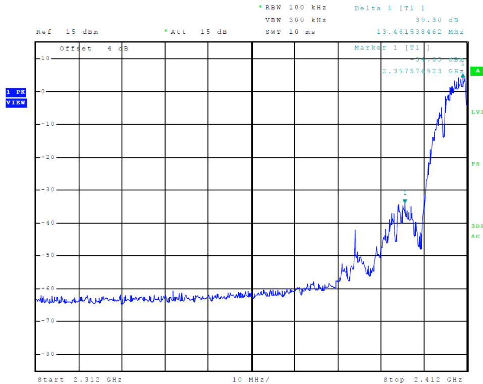
Figure 4 Plot of Lower Band Edge (A5 - 802.11b)
