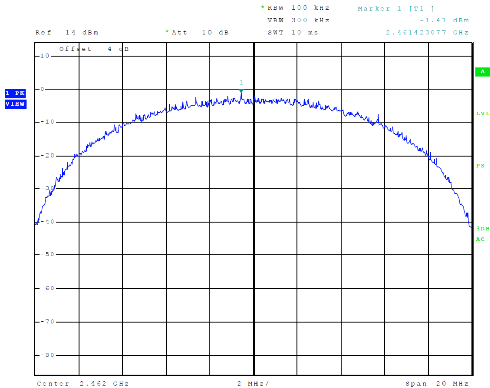
Figure 30 Plot of Transmitter Power Spectral Density (L5 - 802.11b)
