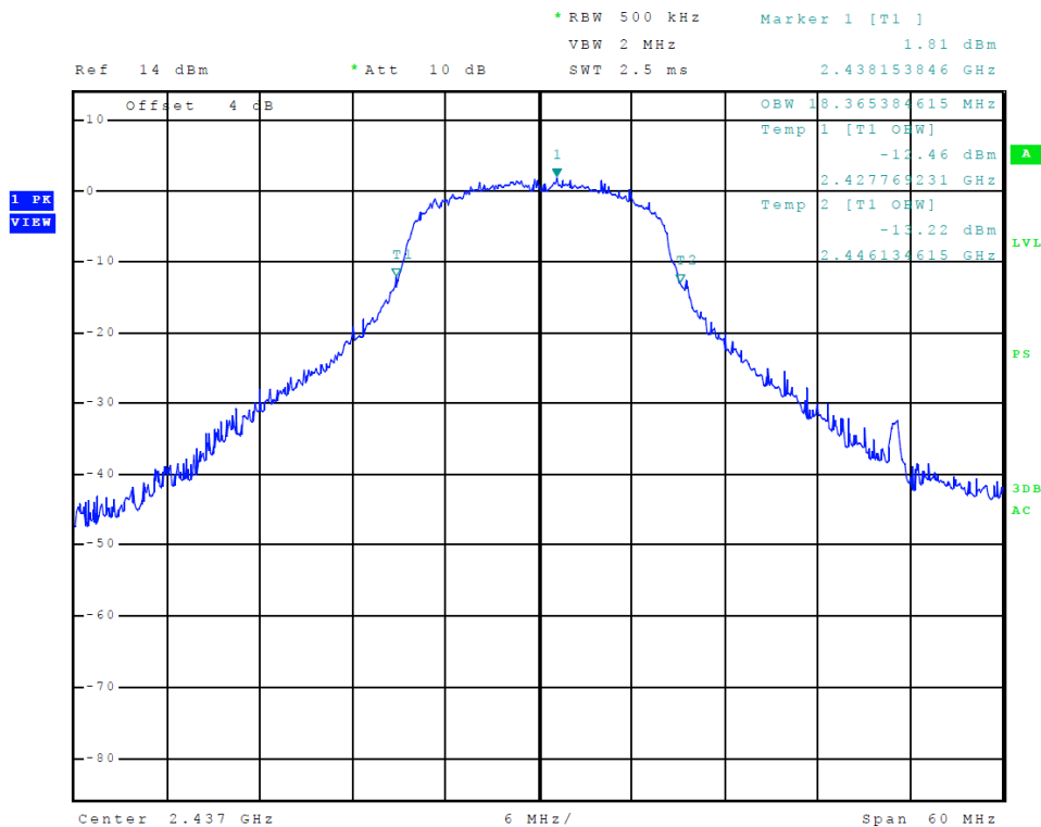
Figure 32 Plot of Transmitter 99% Occupied Bandwidth (L6 - 802.11g)
