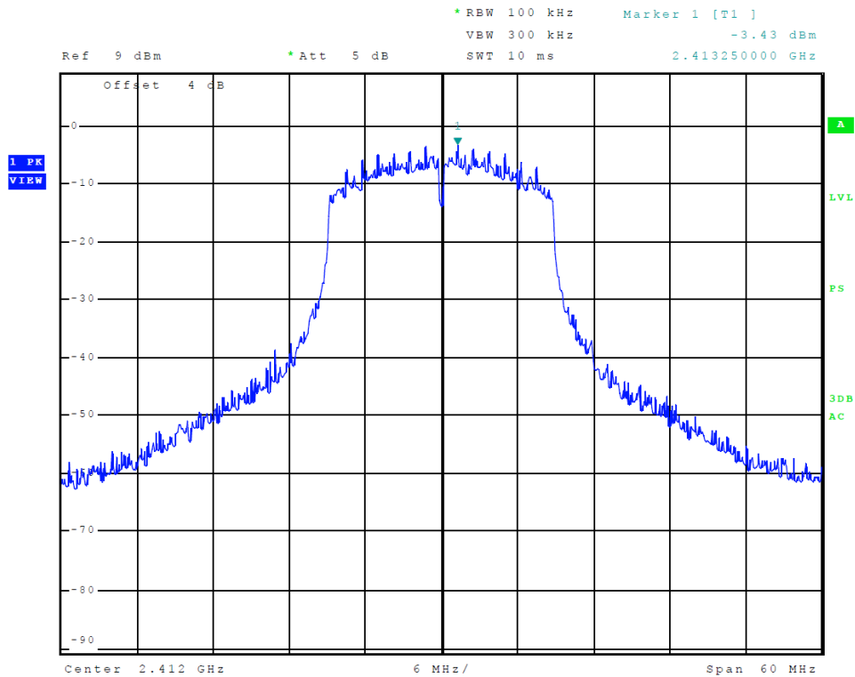
Figure 36 Plot of Transmitter Power Spectral Density (L7 - 802.11n)
