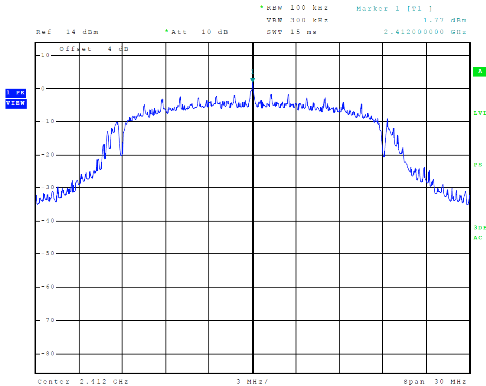
Figure 18 Plot of Transmitter Power Spectral Density (A7 - 802.11n)
