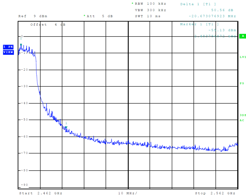
Figure 26 Plot of Upper Band Edge (L6 - 802.11g)
