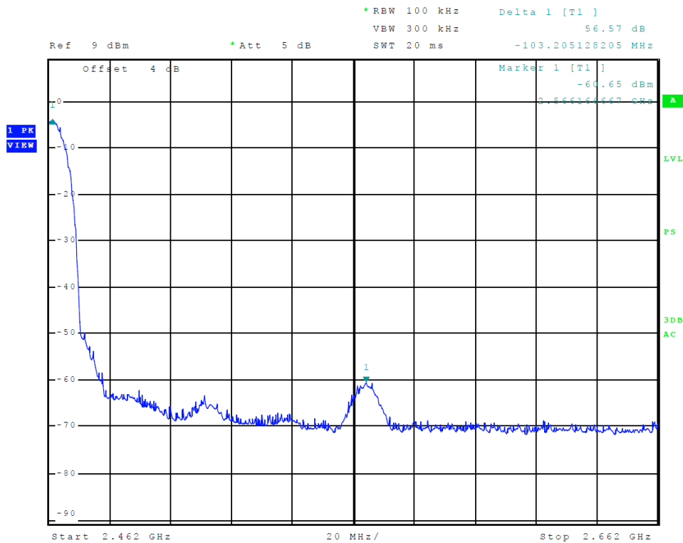
Figure 25 Plot of Upper Band Edge (L5 - 802.11b)
