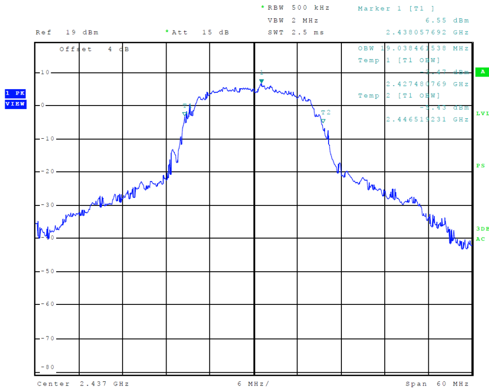
Figure 14 Plot of Transmitter 99% Occupied Bandwidth (A6 - 802.11g)
