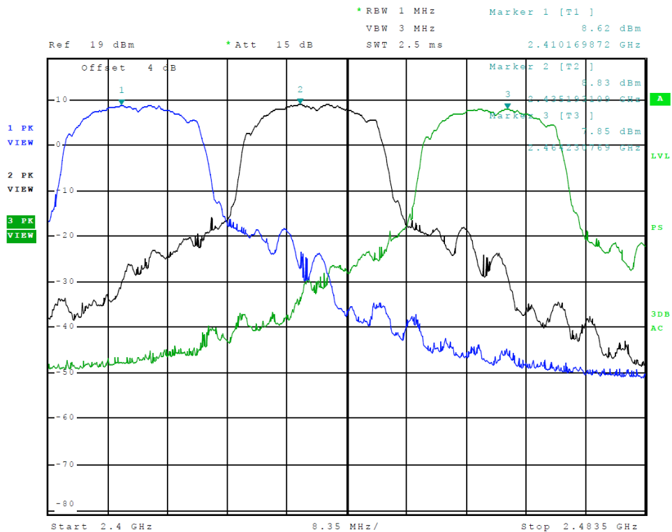
Figure 2 Plot of Transmitter Emissions in Operational Frequency (A6 - 802.11g)
