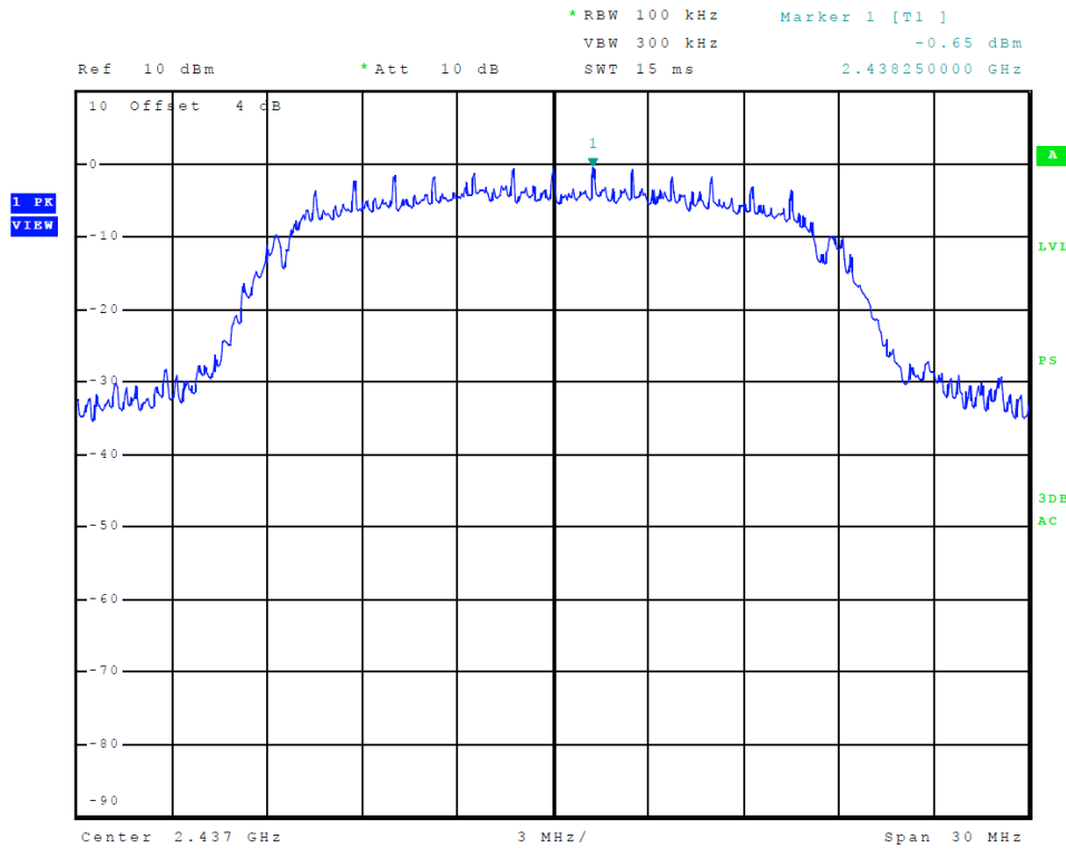
Figure 15 Plot of Transmitter Power Spectral Density (A6 - 802.11g)
