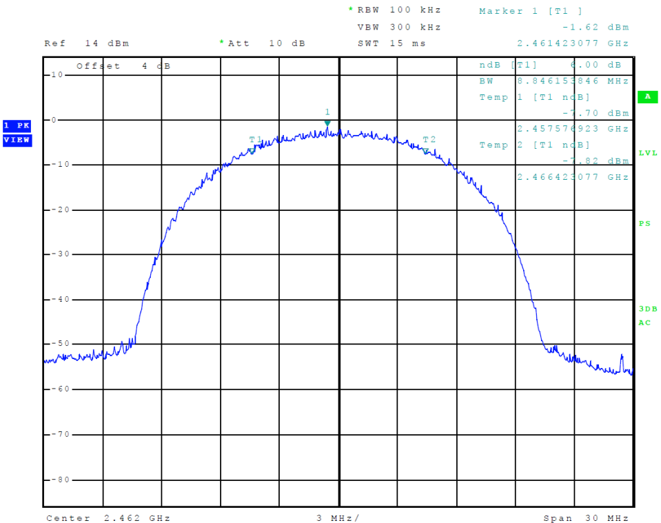
Figure 28 Plot of Transmitter 6-dB Occupied Bandwidth (L5 - 802.11b)
