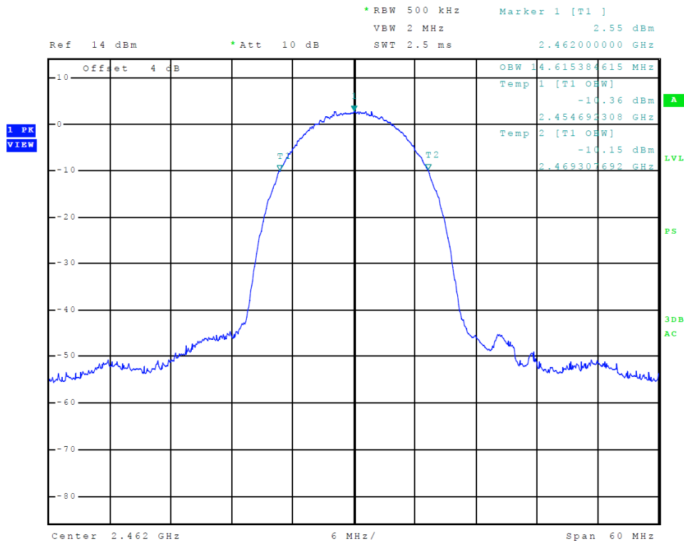
Figure 29 Plot of Transmitter 99% Occupied Bandwidth (L5, 802.11 b)
