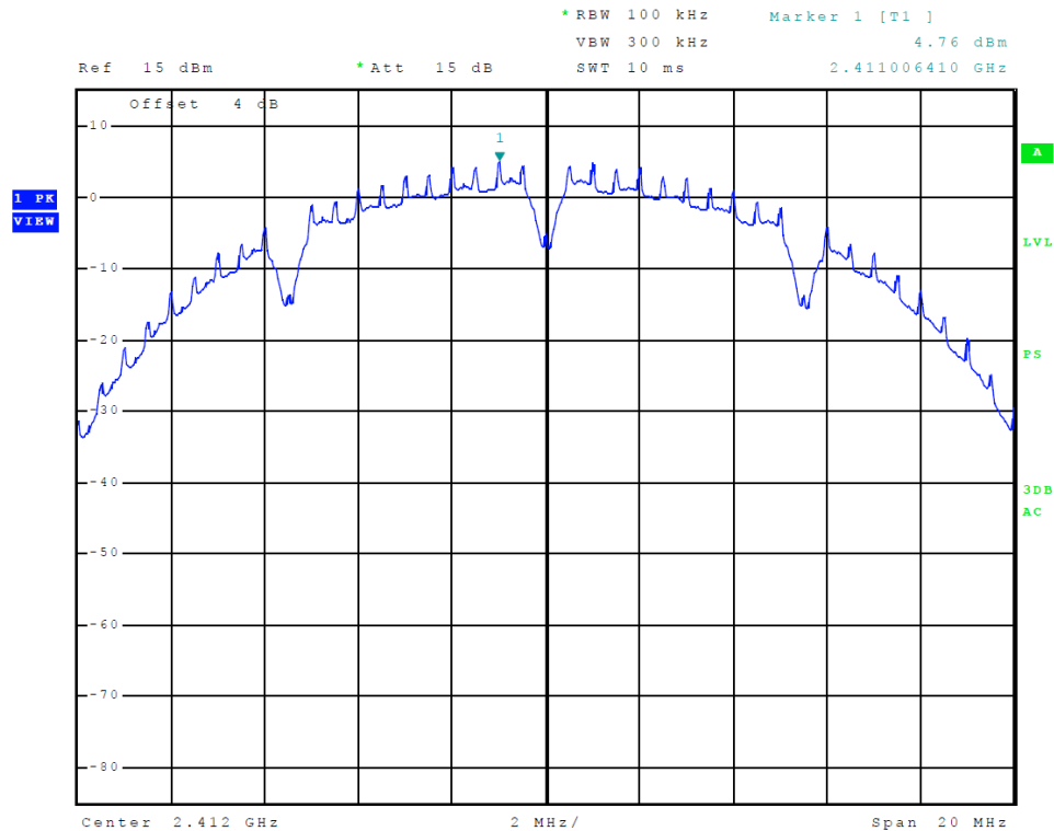
Figure 12 Plot of Transmitter Power Spectral Density (A5 - 802.11b)
