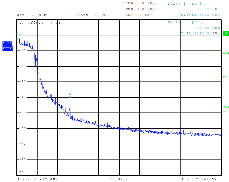
Figure 9 Plot of Upper Band Edge (A7 - 802.11n)
