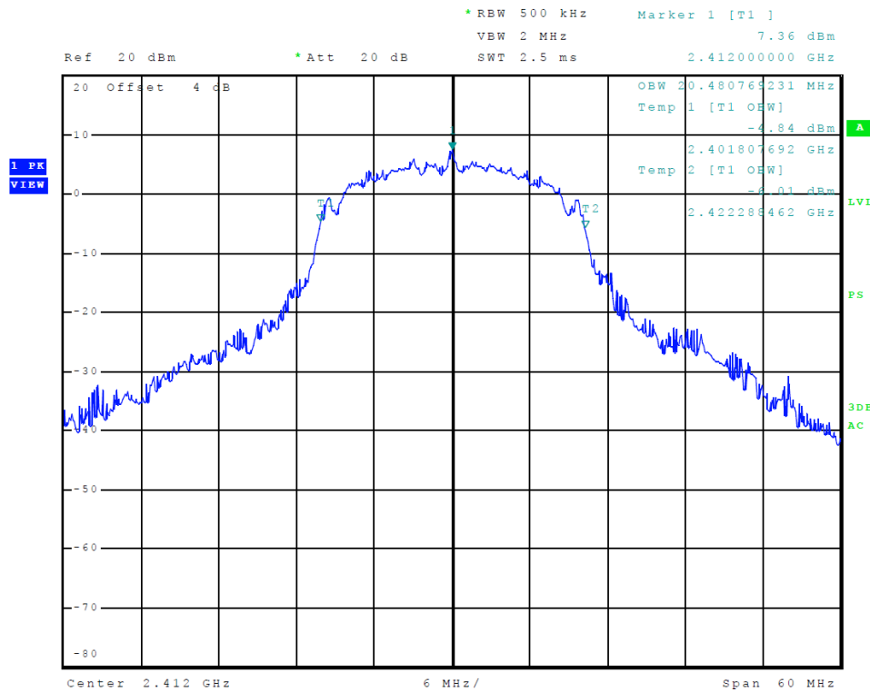
Figure 17 Plot of Transmitter 99% Occupied Bandwidth (A7 - 802.11n)
