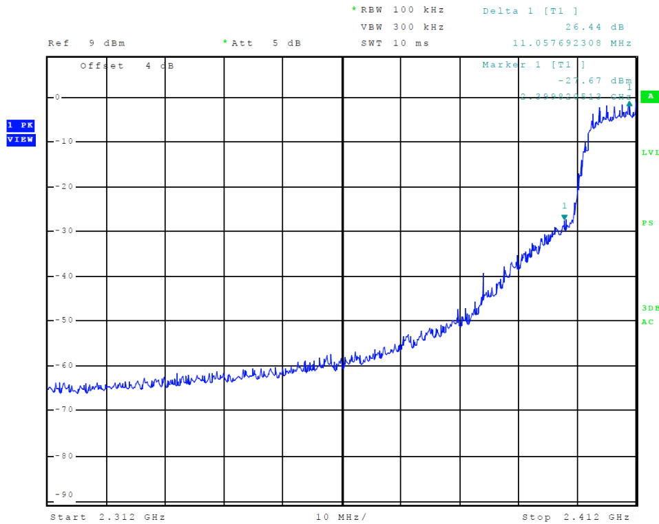
Figure 5 Plot of Lower Band Edge (A6 - 802.11g)
