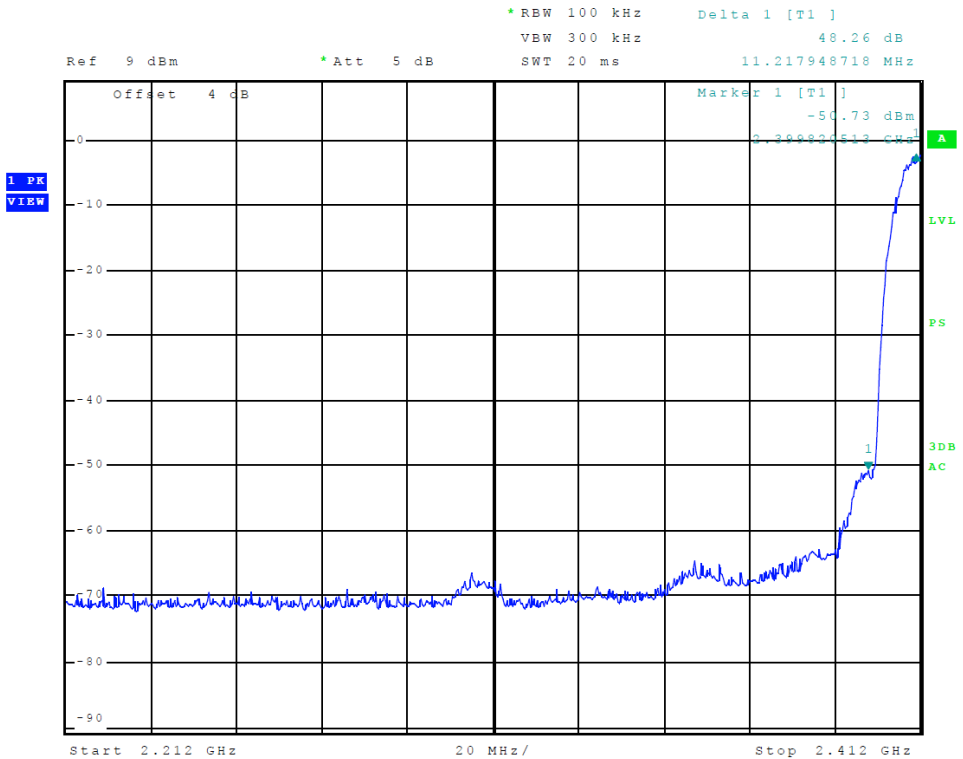
Figure 22 Plot of Lower Band Edge (L5, 802.1b)
