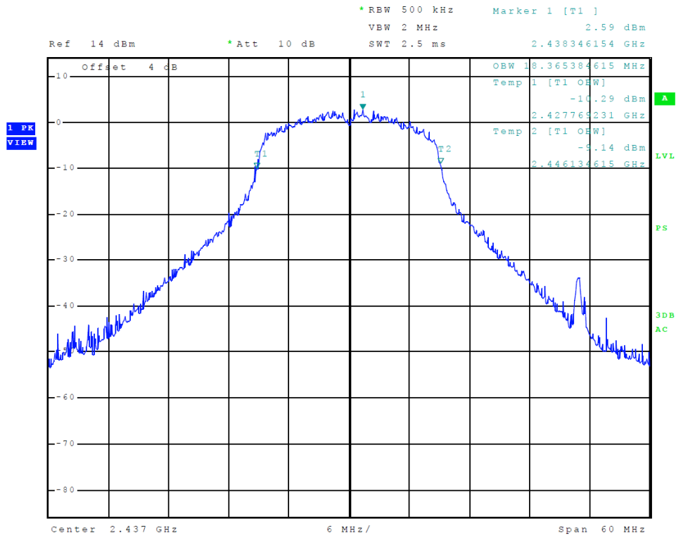
Figure 35 Plot of Transmitter 99% Occupied Bandwidth (L7 - 802.11n)
