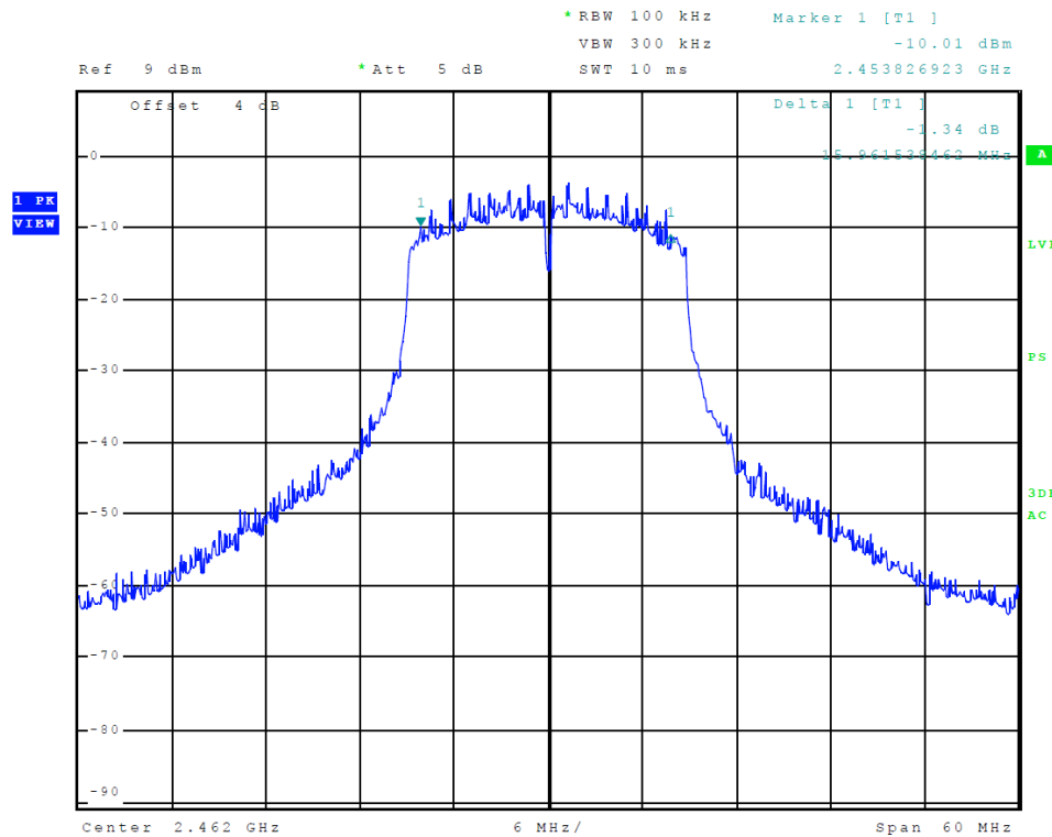
Figure 34 Plot of Transmitter 6-dB Occupied Bandwidth (L7 - 802.11n)
