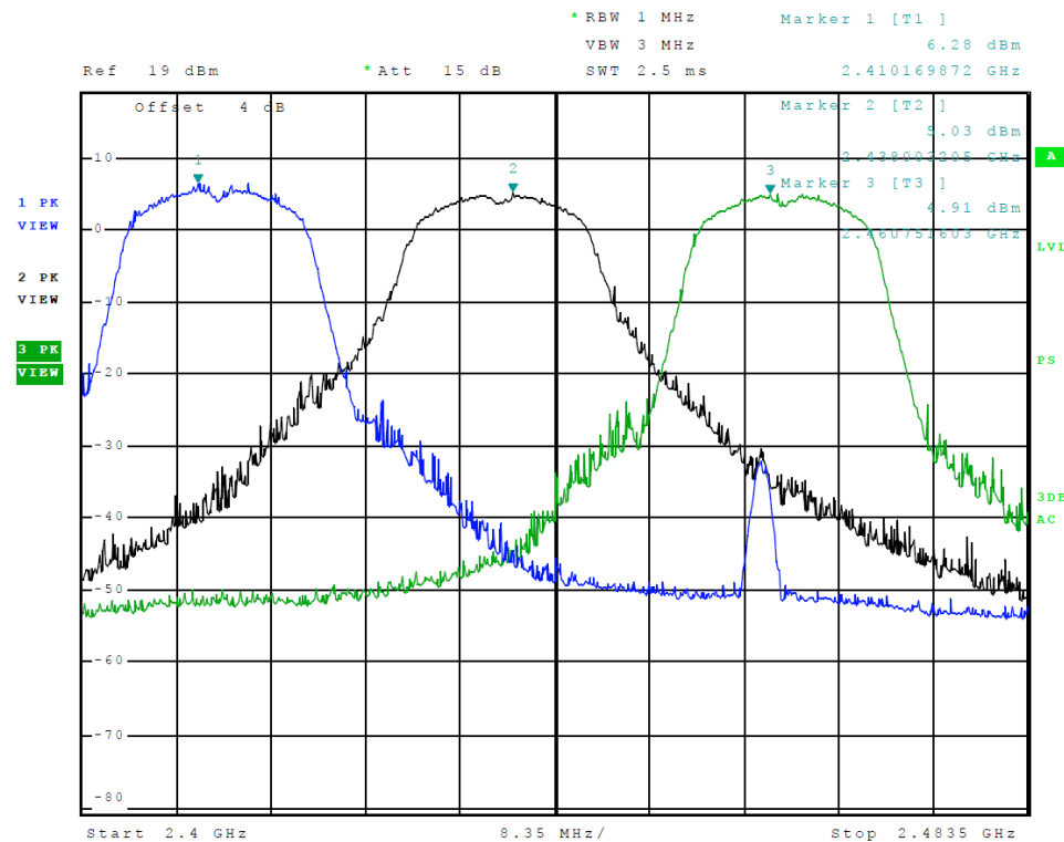
Figure 20 Plot of Transmitter Emissions in Operational Frequency (L6, 802.1g)
