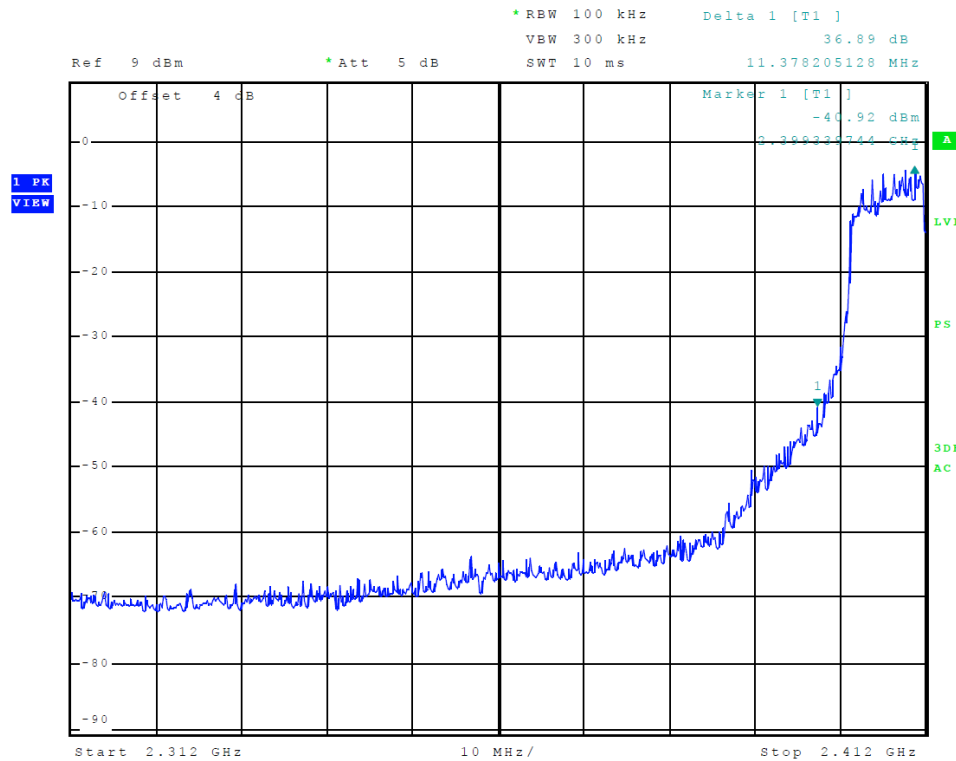
Figure 24 Plot of Lower Band Edge (L7 - 802.11n)
