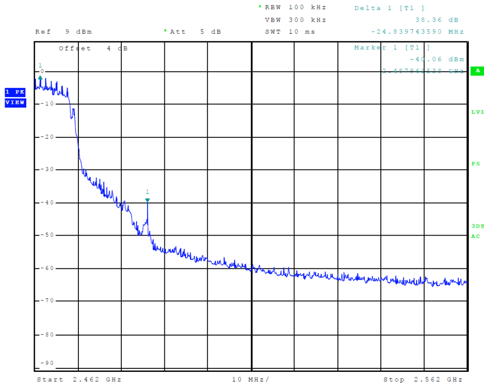
Figure 8 Plot of Upper Band Edge (A6 - 802.11g)
