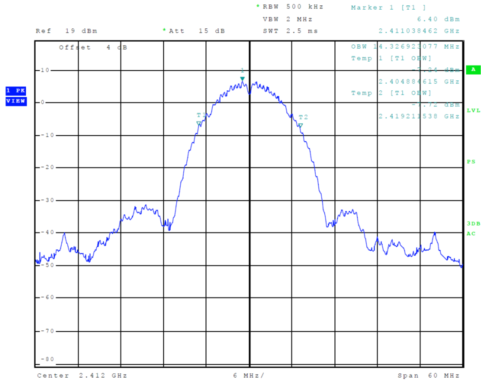
Figure 11 Plot of Transmitter 99% Occupied Bandwidth (A5, 802.11 b)
