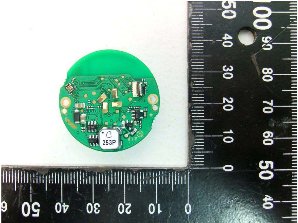
Figure 3 - PCB Bottom
