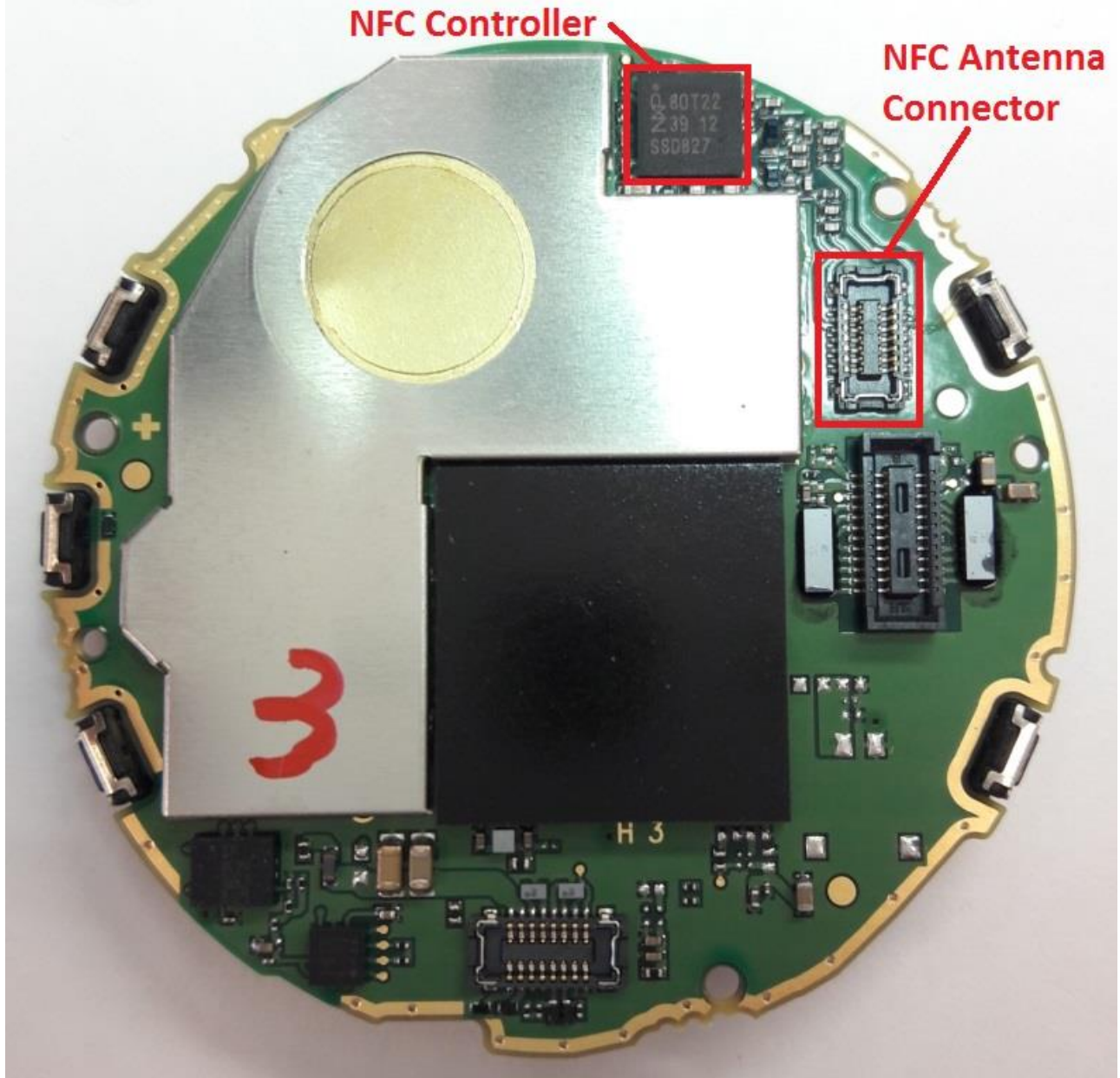
Figure 6 - Top PCB, with Shield
