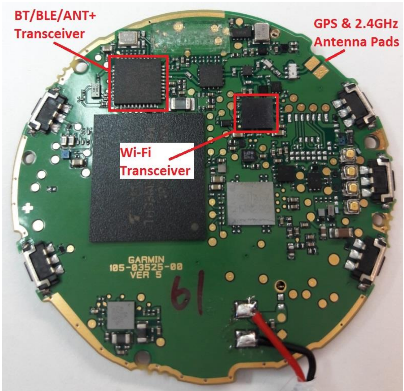
Figure 3 - Bottom PCB
