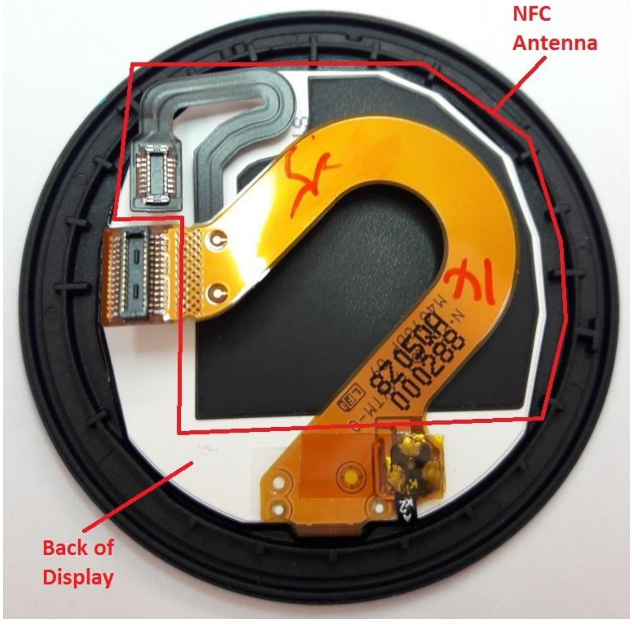
Figure 4 - NFC Antenna
