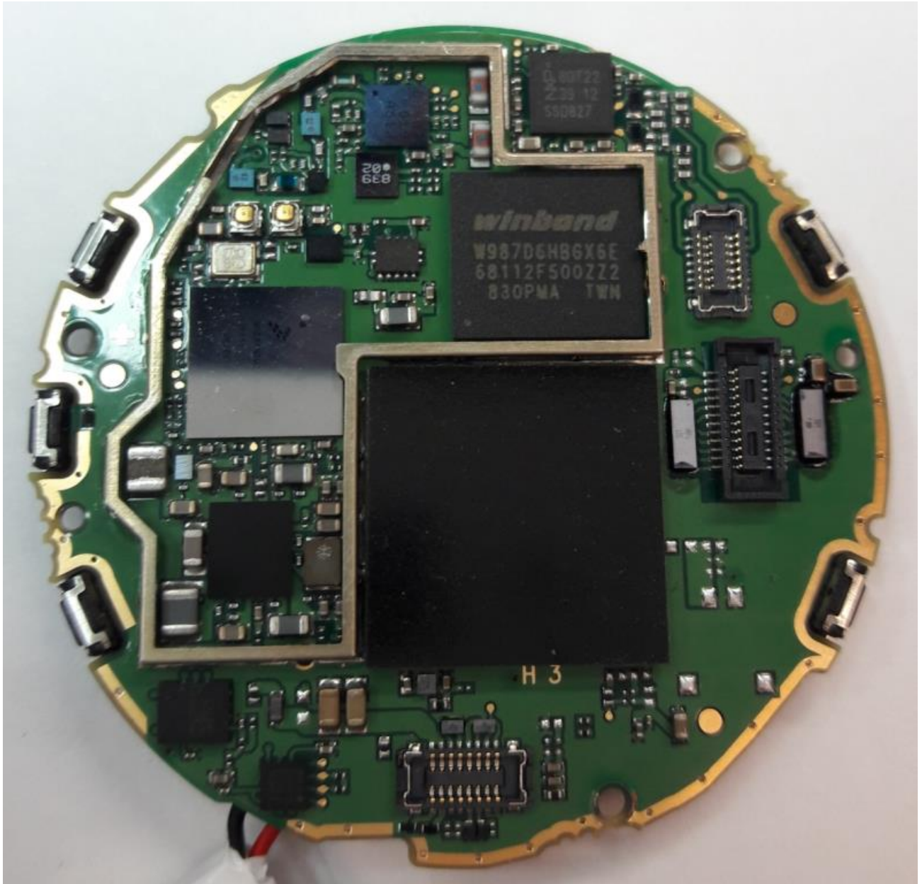
Figure 5 - Top PCB, No Shield
