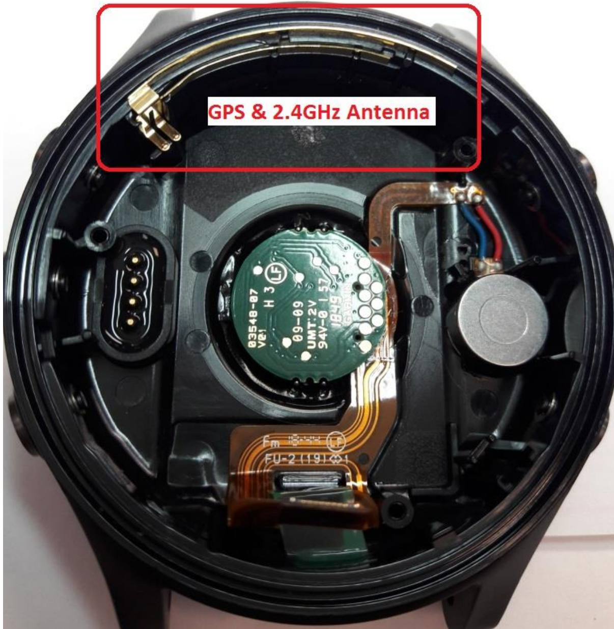
Figure 1 - 2.4 GHz Antenna
