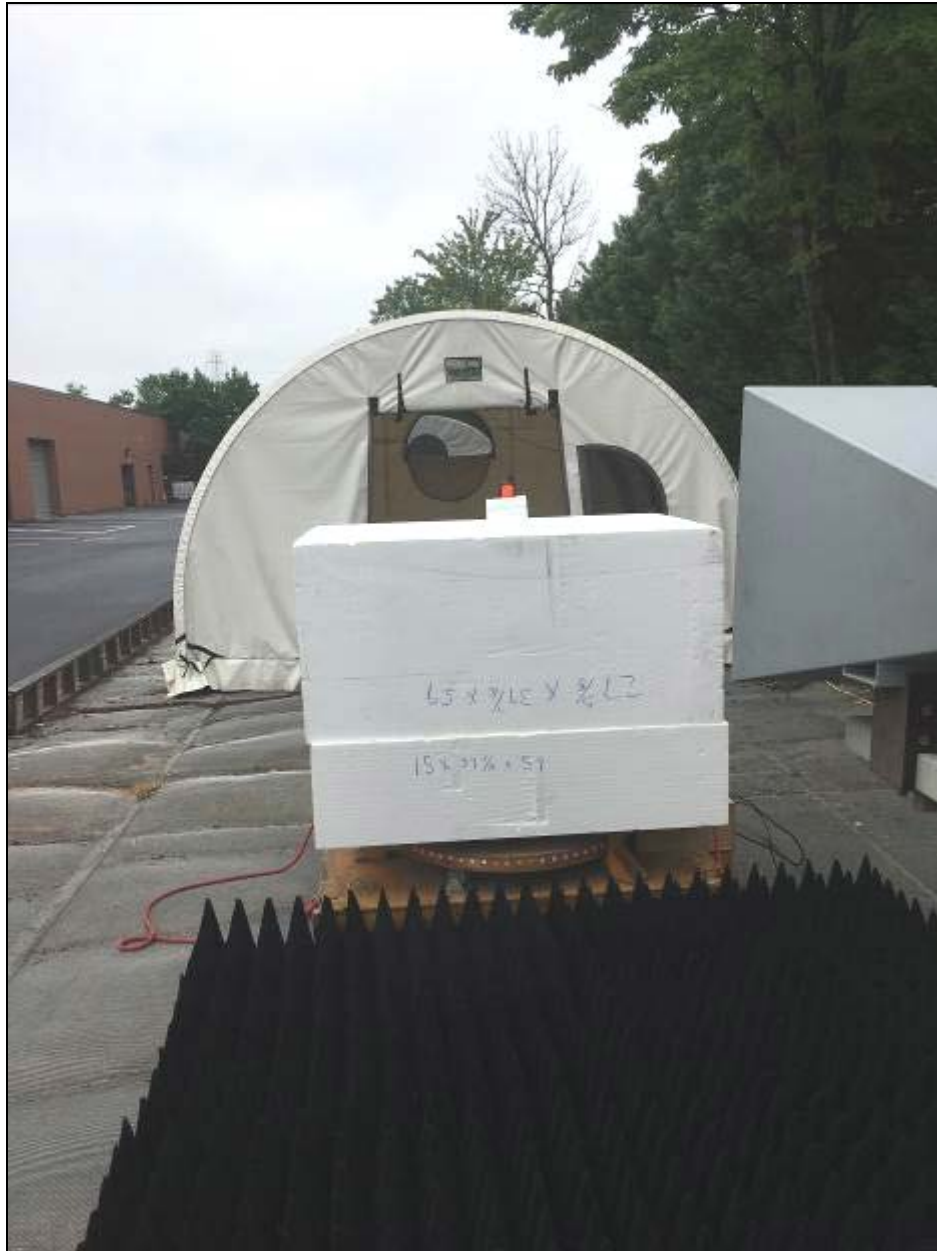
Photograph 2: Radiated Emissions Testing – Back View
