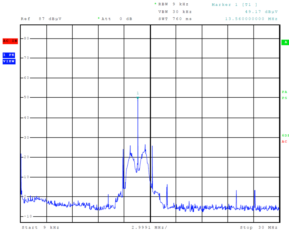
Figure 6 Plot of NFC Operation Across Authorized Band
