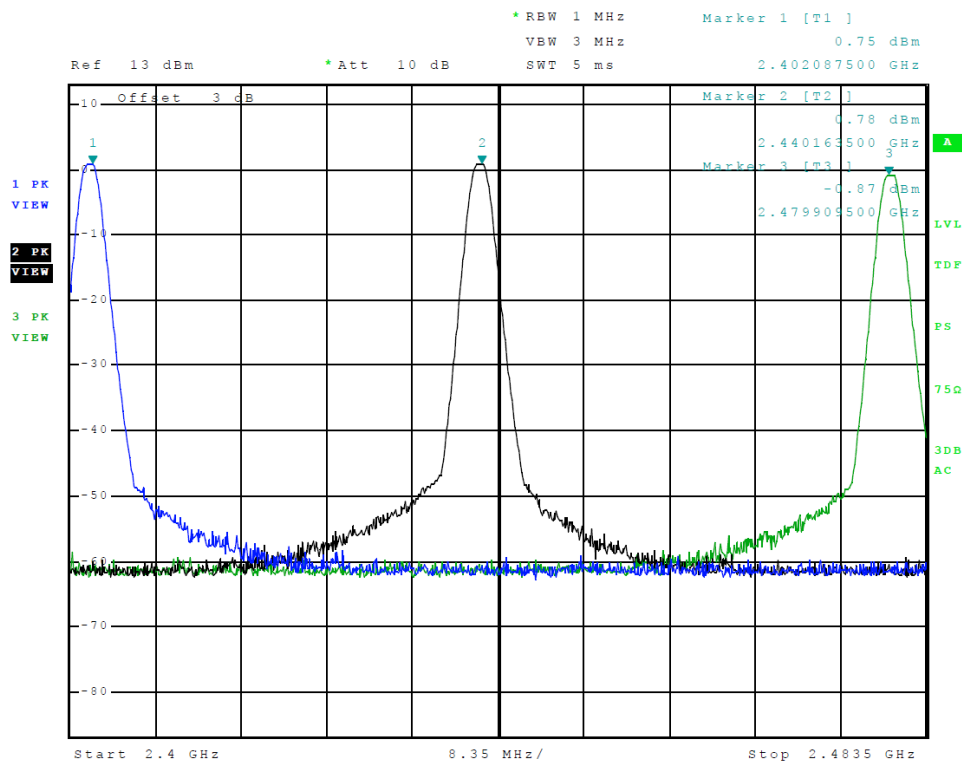
Figure 8 Plot of Transmitter Emissions Operation in 2402-2480 MHz BT BLE (GMSK)
