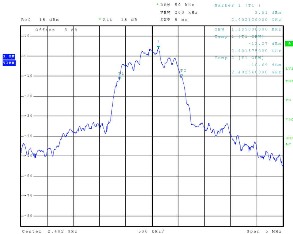
Figure 10 Plot of Transmitter Emissions 99% Occupied Bandwidth BT BR (GFSK)
