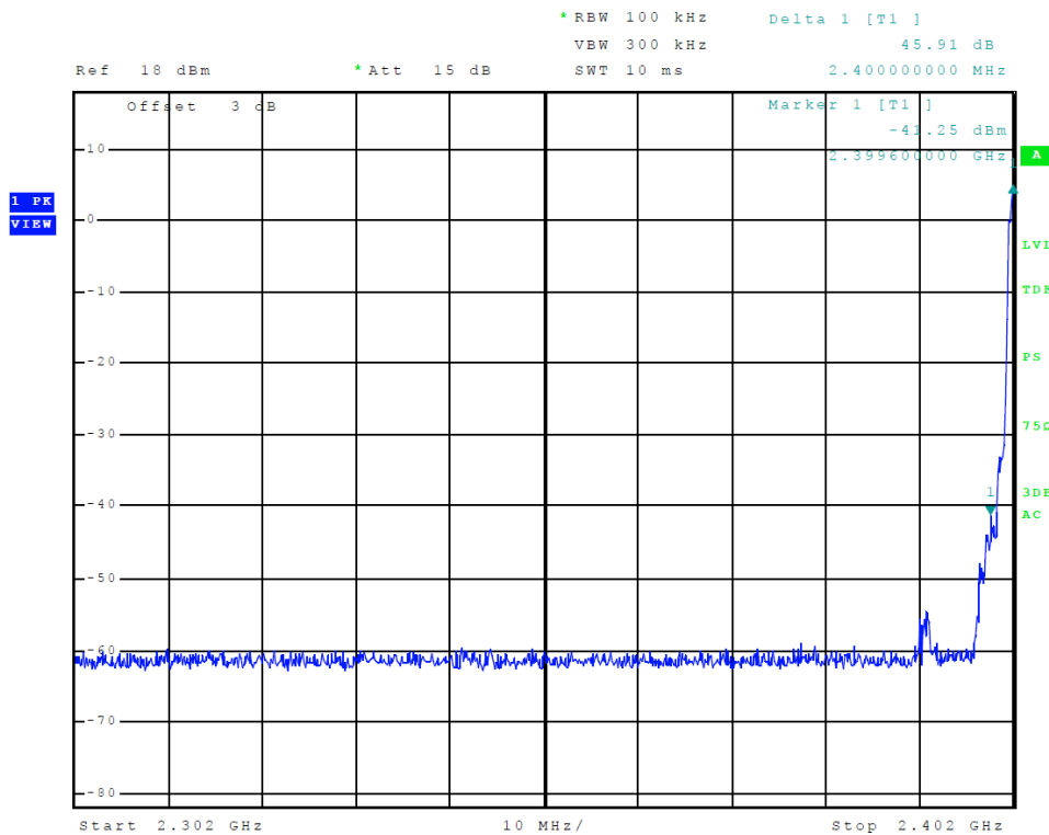
Figure 14 Plot of Transmitter Emissions Low Band Edge BT BR (GFSK)
