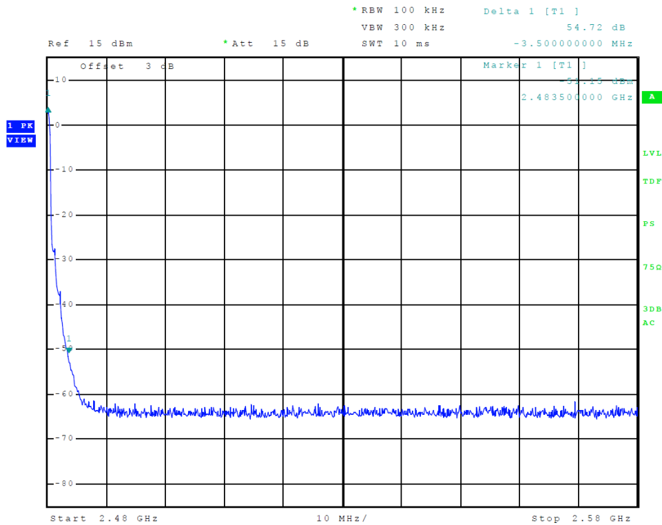
Figure 19 Plot of Transmitter Emissions High Band Edge BT 2EDR (PI/4 DPQSK)
