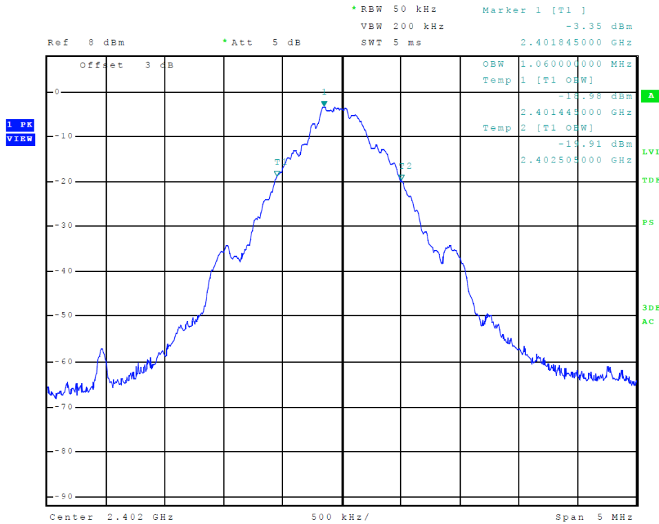
Figure 9 Plot of Transmitter Emissions 99% Occupied Bandwidth ANT (GFSK)
