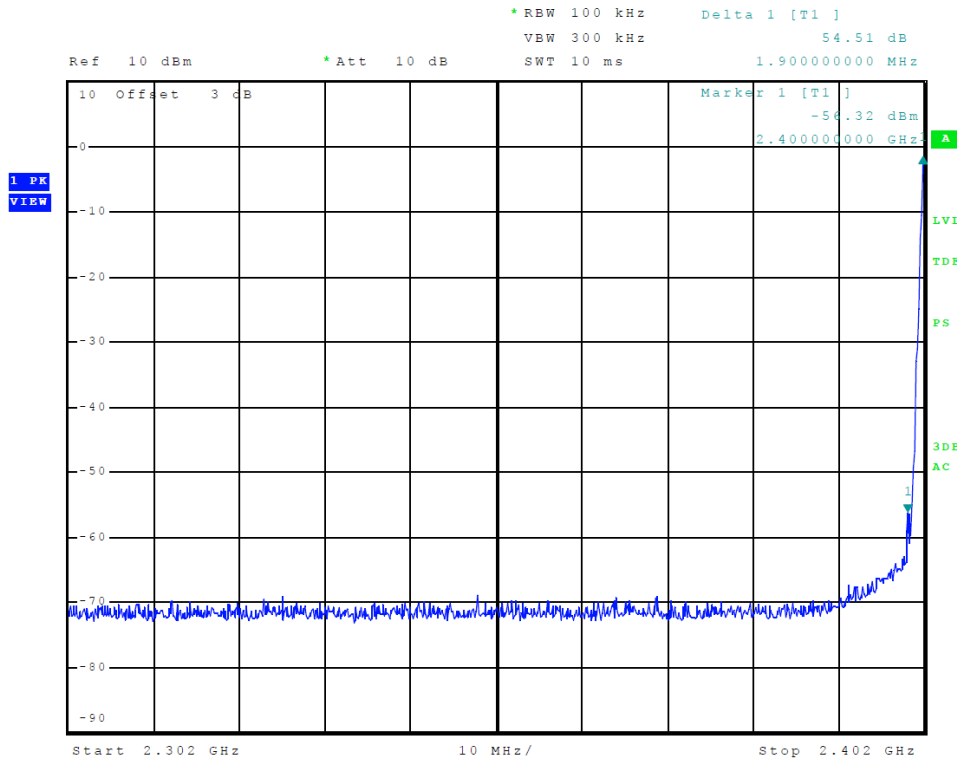
Figure 13 Plot of Transmitter Emissions Low Band Edge ANT (GFSK)
