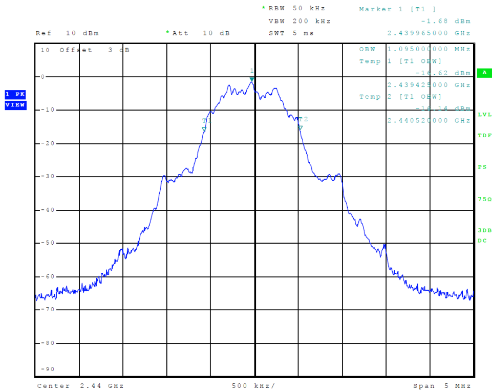
Figure 12 Plot of Transmitter Emissions 99% Occupied Bandwidth BT BLE (GMSK)
