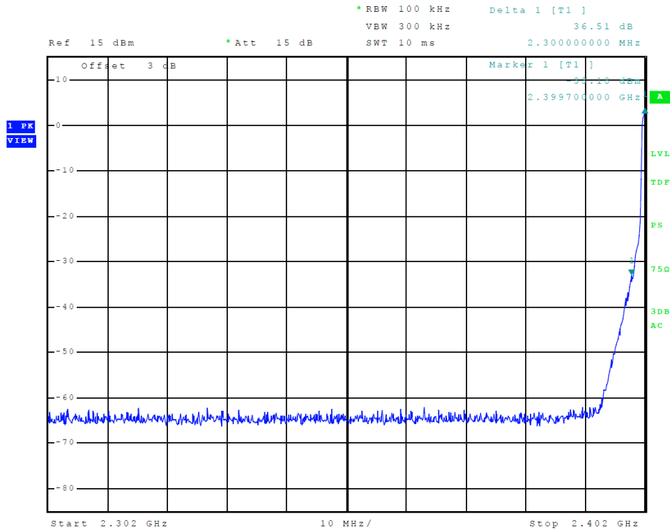
Figure 15 Plot of Transmitter Emissions Low Band Edge BT 2EDR (PI/4 DPQSK)
