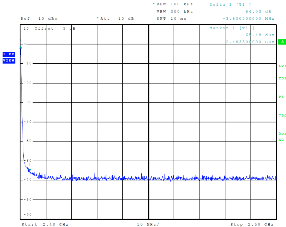
Figure 17 Plot of Transmitter Emissions High Band Edge ANT (GFSK)
