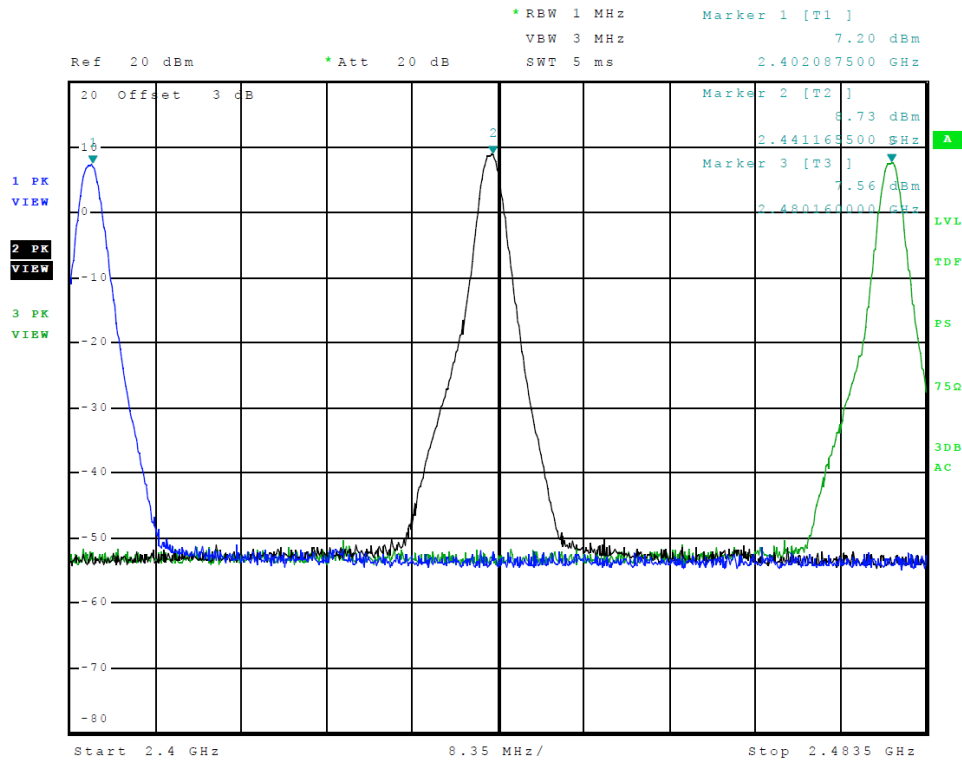
Figure 7 Plot of Transmitter Emissions Operation in 2402-2480 MHz BT 2EDR (PI/4 DPQSK)
