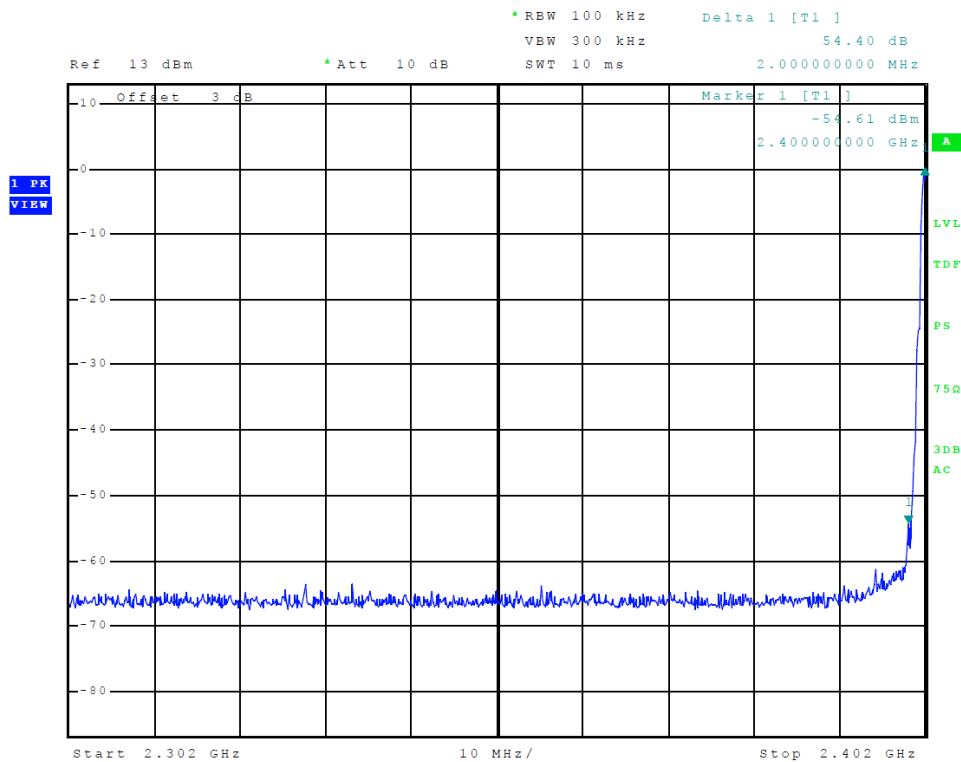
Figure 16 Plot of Transmitter Emissions Low Band Edge BT BLE (GMSK)
