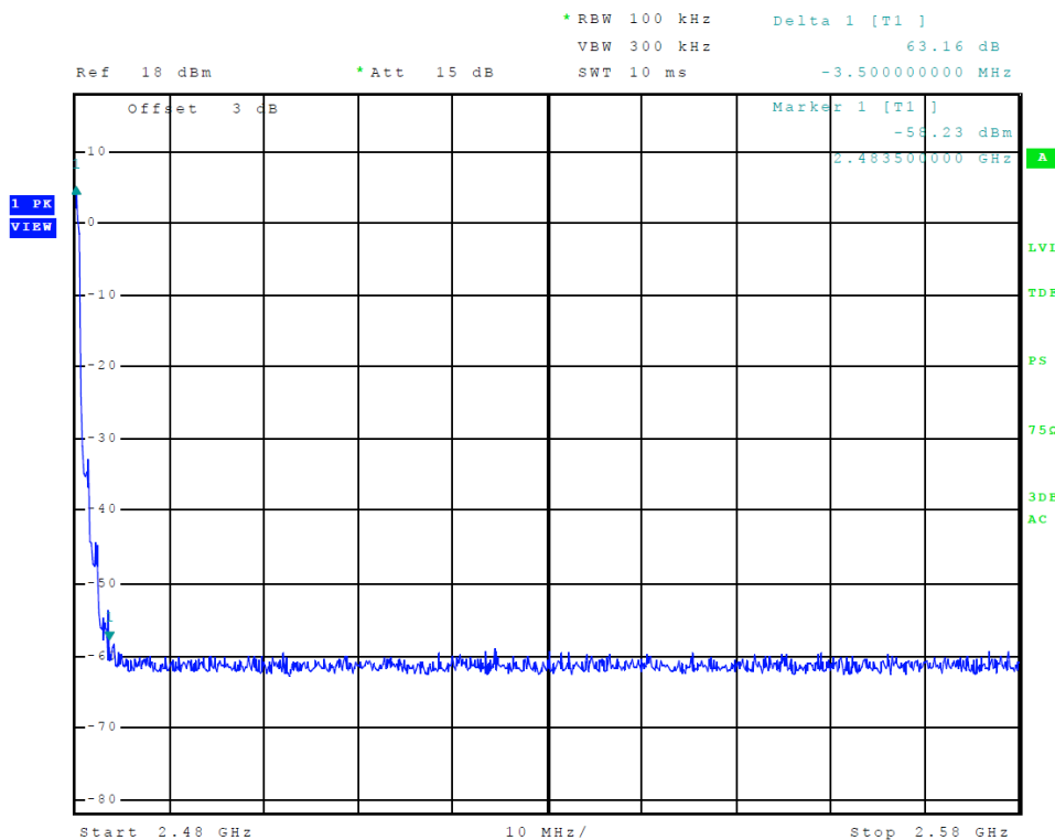
Figure 18 Plot of Transmitter Emissions High Band Edge BT BR (GFSK)
