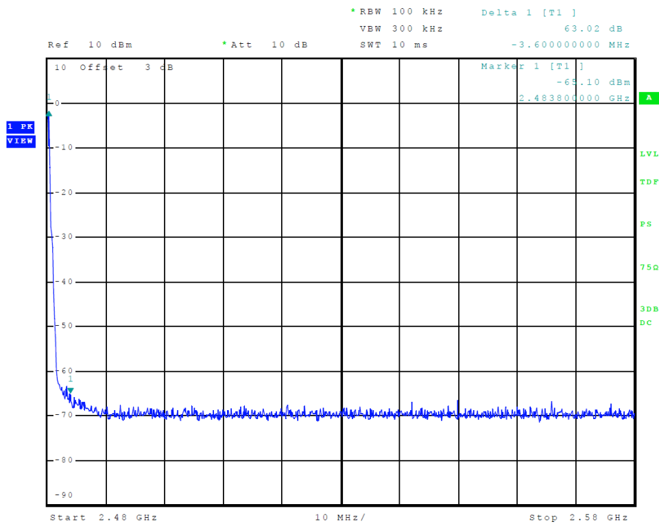
Figure 20 Plot of Transmitter Emissions High Band Edge BT BLE (GMSK)
