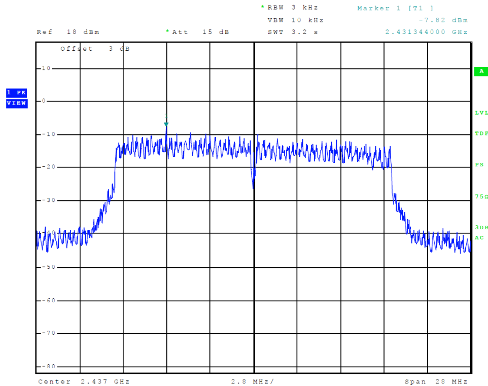
Figure 22 Plot of Transmitter Power Spectral Density (802.11 n-mode)
