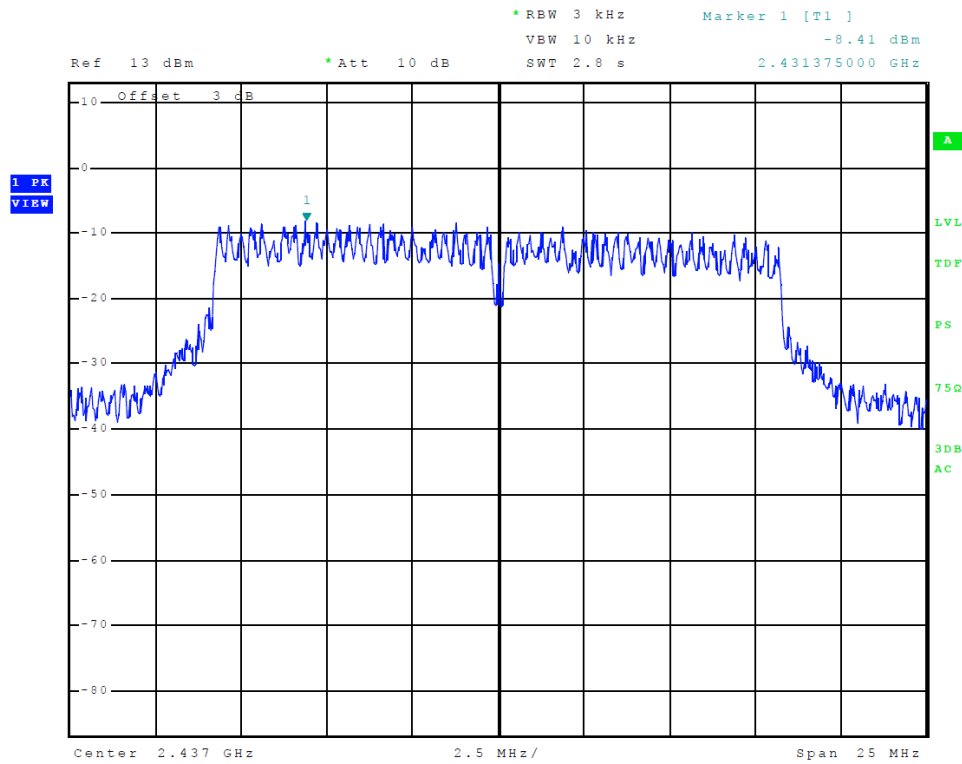
Figure 21 Plot of Transmitter Power Spectral Density (802.11 g-mode)
