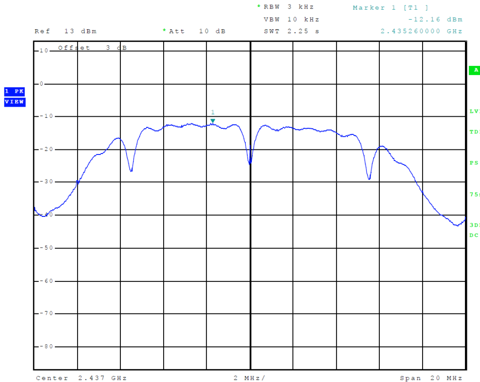
Figure 20 Plot of Transmitter Power Spectral Density (802.11 b-mode)
