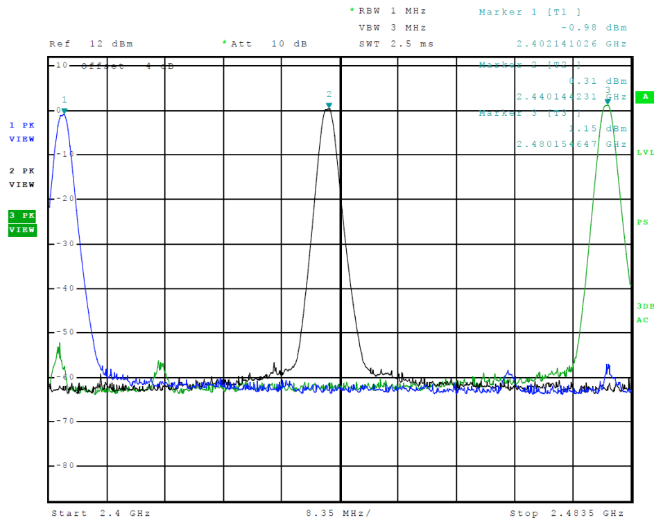
Figure 8 Plot of Transmitter Emissions Operation in 2402-2480 MHz (GMSK)
