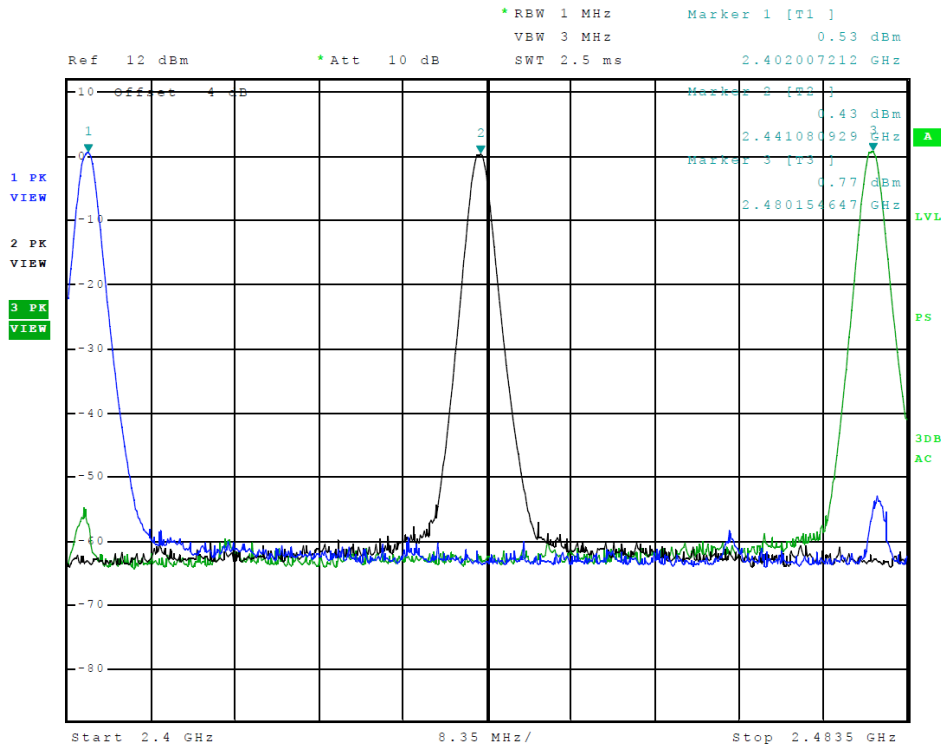
Figure 5 Plot of Transmitter Emissions Operation in 2402-2480 MHz (GFSK)
