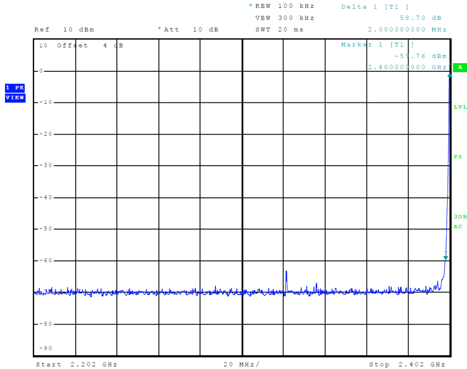
Figure 15 Plot of Transmitter Emissions Low Band Edge (8DPSK)
