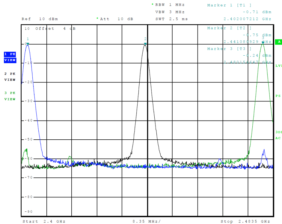
Figure 6 Plot of Transmitter Emissions Operation in 2402-2480 MHz (PI/4 DPQSK)
