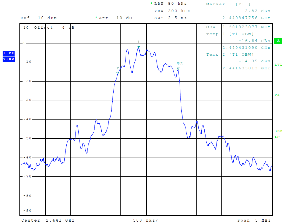
Figure 11 Plot of Transmitter Emissions 99% Occupied Bandwidth (8DPSK)
