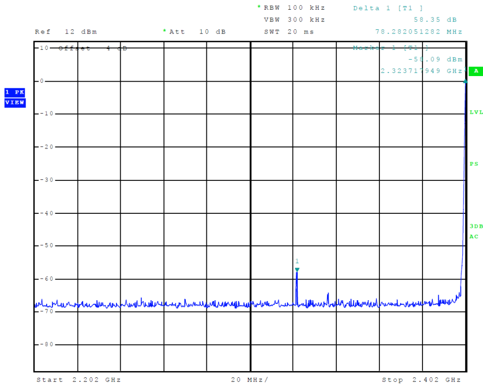
Figure 13 Plot of Transmitter Emissions Low Band Edge (GFSK)
