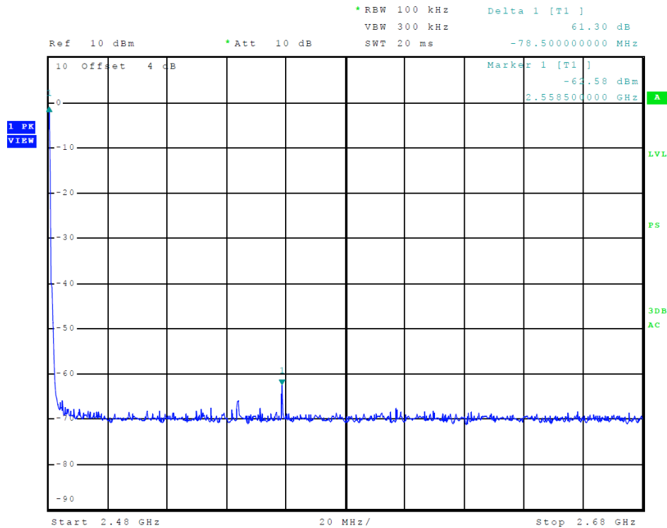
Figure 19 Plot of Transmitter Emissions High Band Edge (8DPSK)
