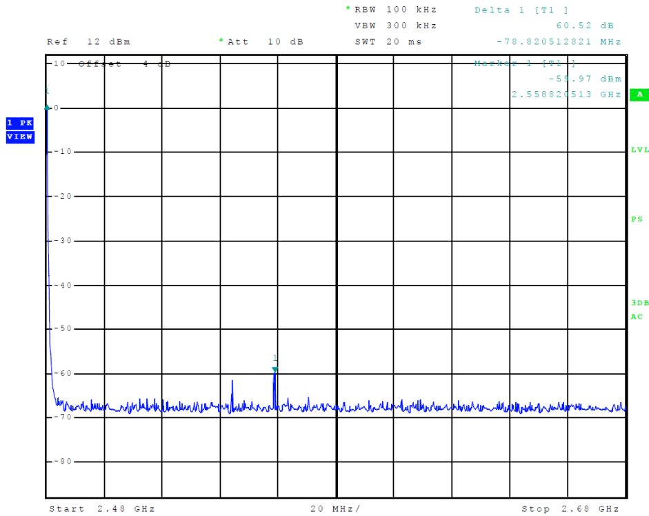
Figure 17 Plot of Transmitter Emissions High Band Edge (GFSK)
