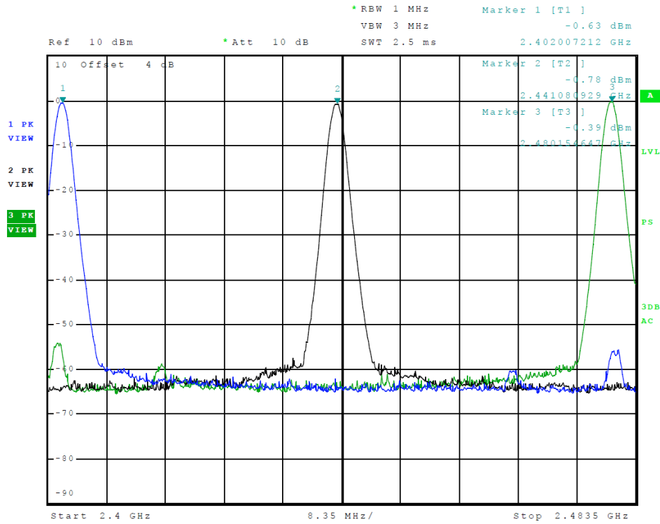
Figure 7 Plot of Transmitter Emissions Operation in 2402-2480 MHz (8DPSK)
