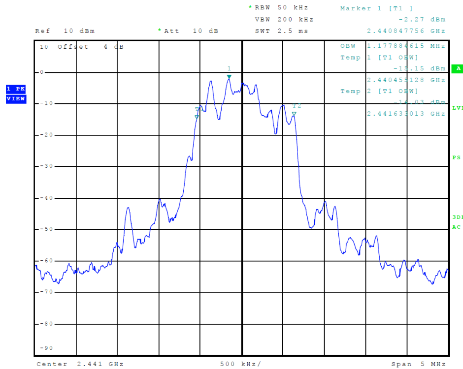
Figure 10 Plot of Transmitter Emissions 99% Occupied Bandwidth (PI/4 DPQSK)
