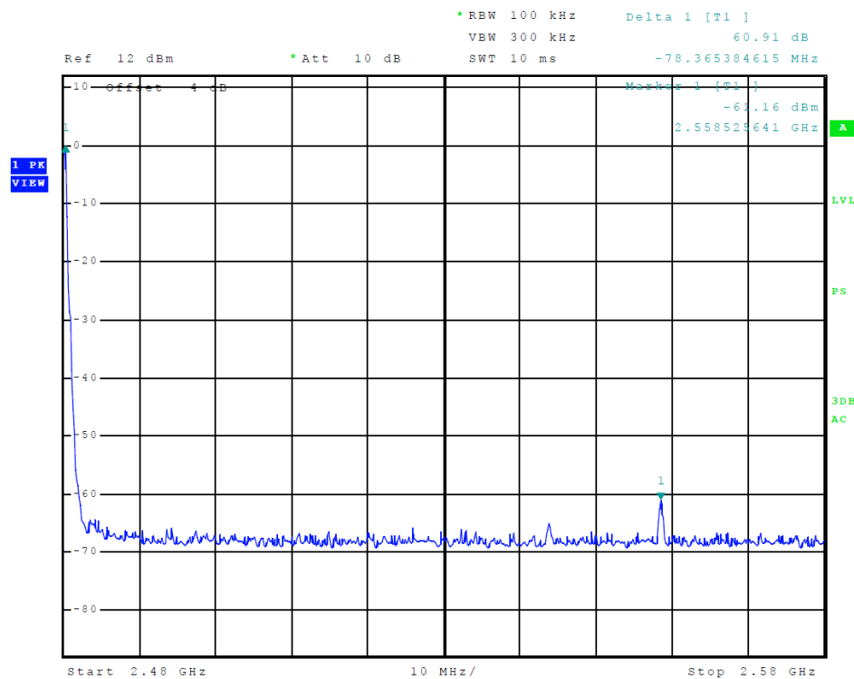
Figure 20 Plot of Transmitter Emissions High Band Edge (GMSK)
