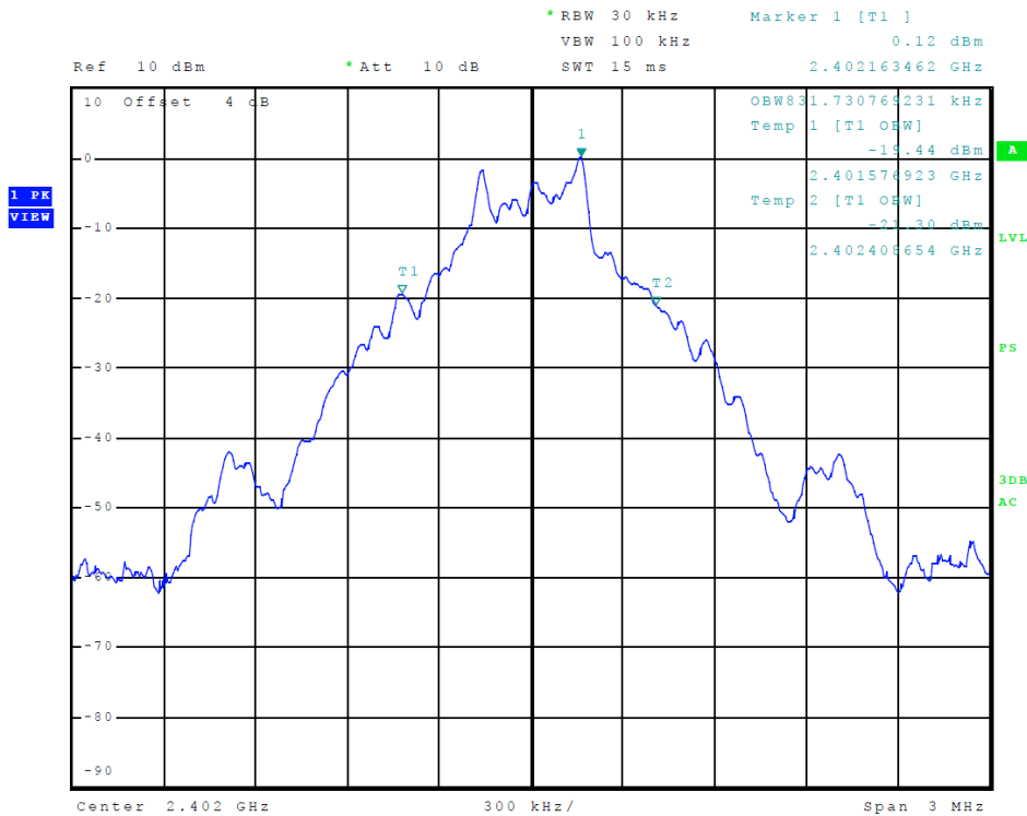
Figure 9 Plot of Transmitter Emissions 99% Occupied Bandwidth (GFSK)
