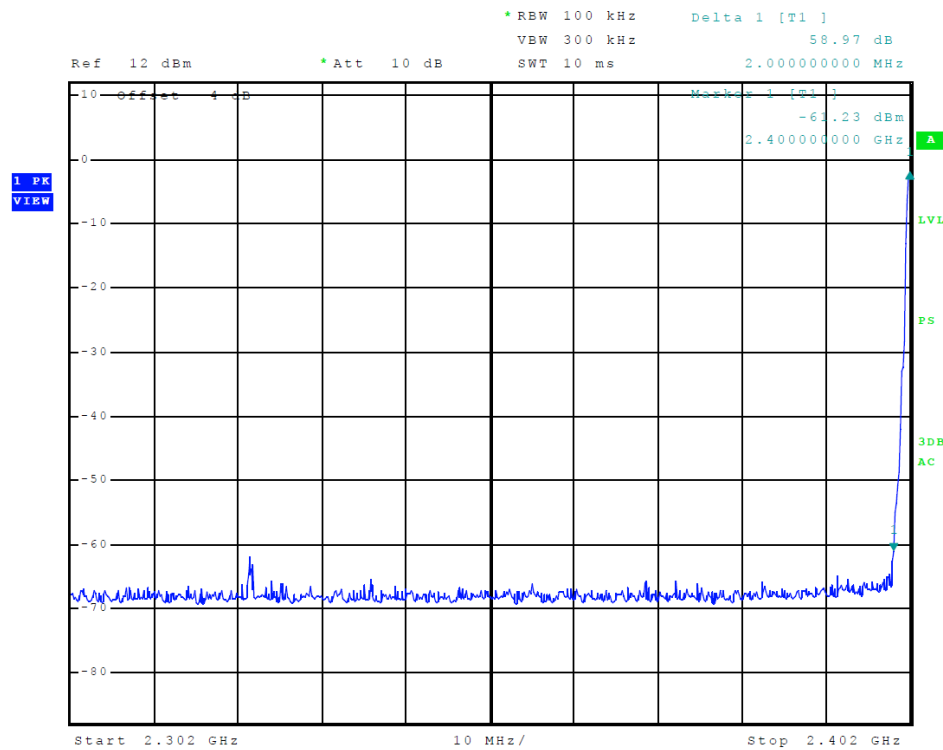
Figure 16 Plot of Transmitter Emissions Low Band Edge (GMSK)
