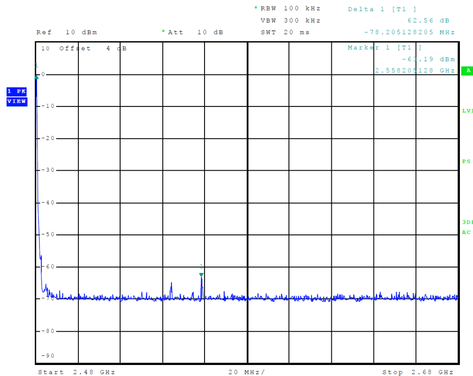
Figure 18 Plot of Transmitter Emissions High Band Edge (PI/4 DPQSK)
