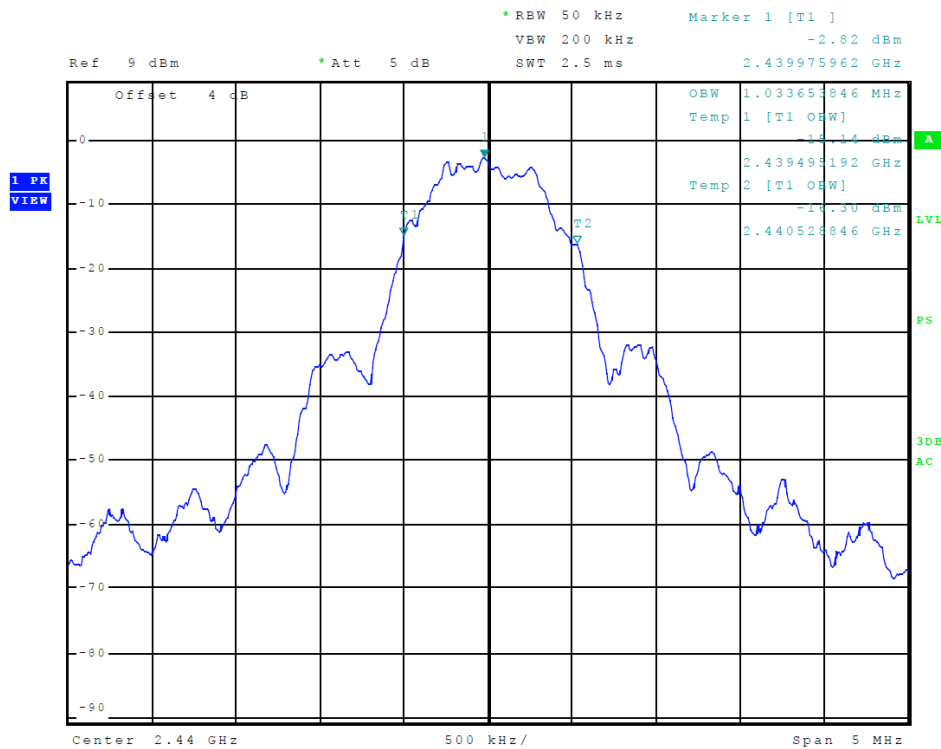
Figure 12 Plot of Transmitter Emissions 99% Occupied Bandwidth (GMSK)
