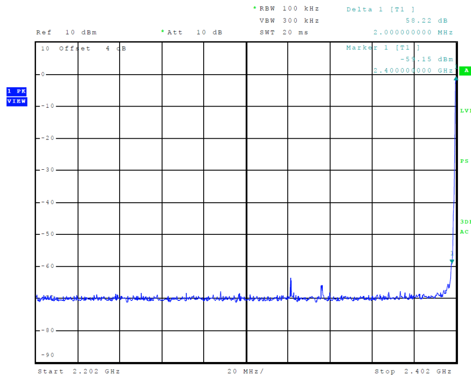
Figure 14 Plot of Transmitter Emissions Low Band Edge (PI/4 DPQSK)
