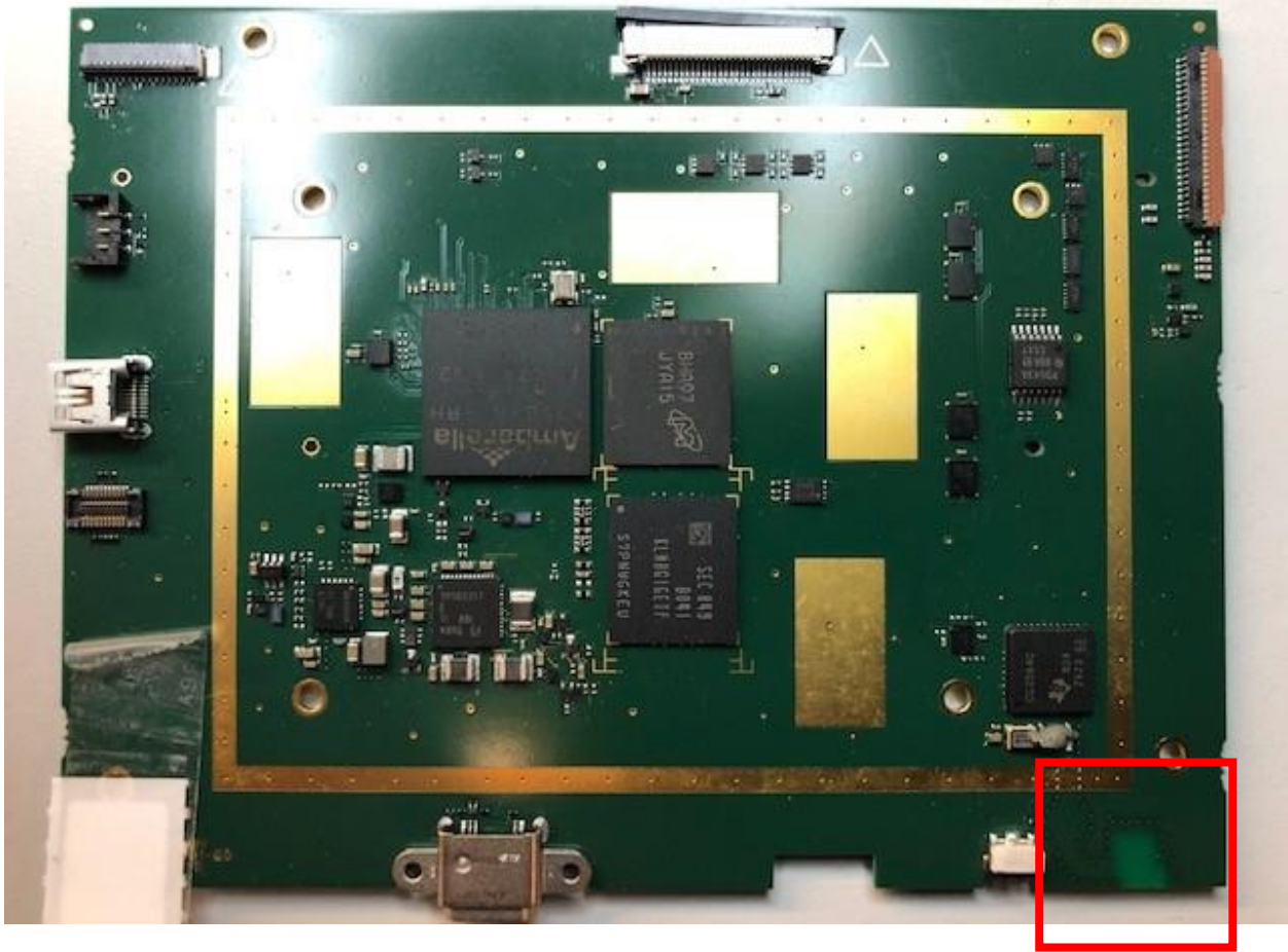
2.4 GHz antenna shown in red box
