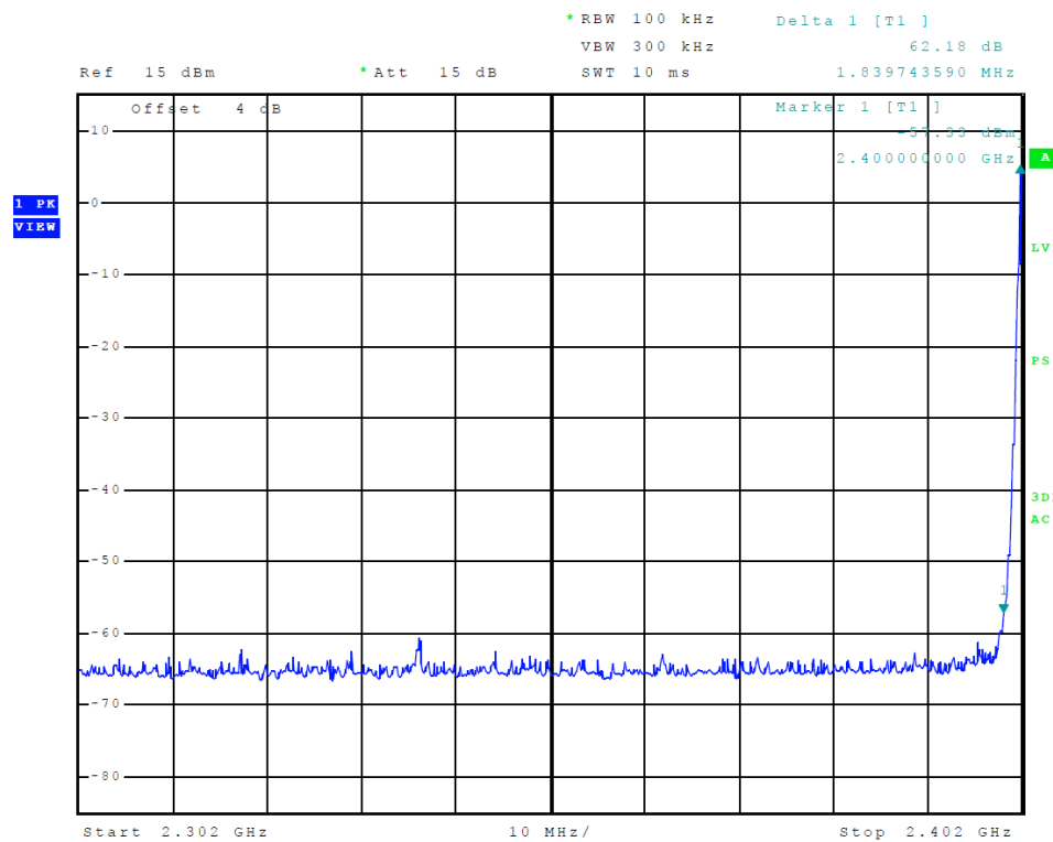
Figure 16 Plot of Transmitter Emissions Low Band Edge BT BR (GFSK)
