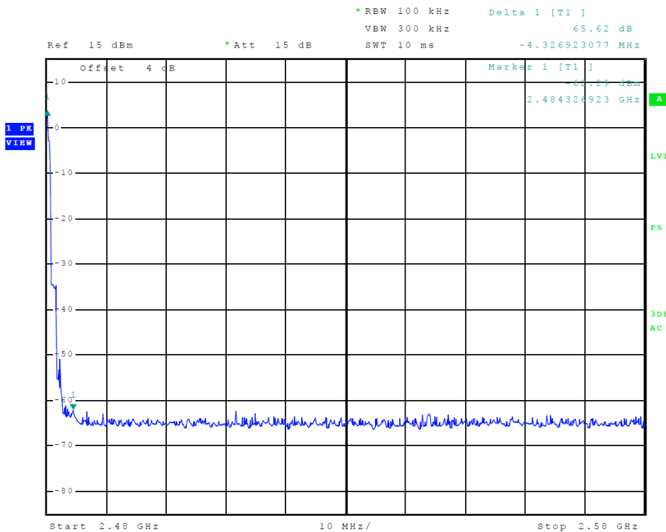
Figure 22 Plot of Transmitter Emissions High Band Edge 2EDR (PI/4 DPQSK)
