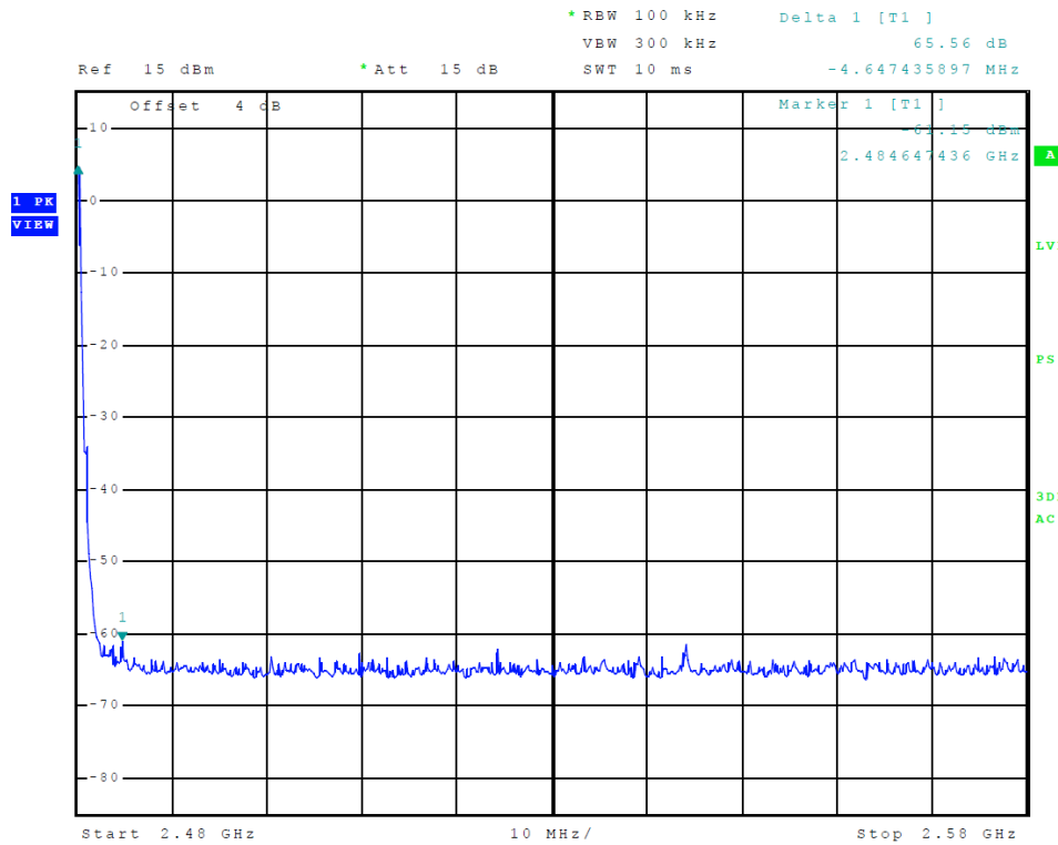
Figure 21 Plot of Transmitter Emissions High Band Edge BT BR (GFSK)
