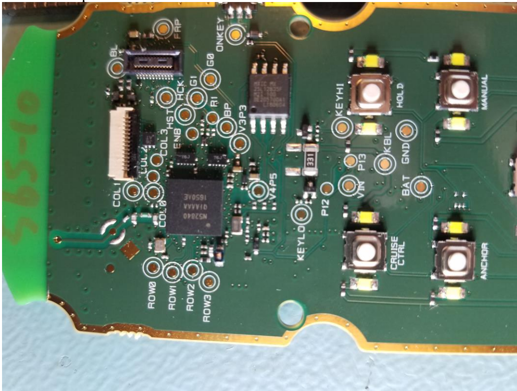
Transmitter portion of Board
