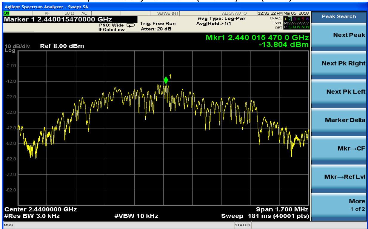
Plot 8-5: Power Spectral Density: Channel 19 (2440 MHz): BLE (PRB29)
