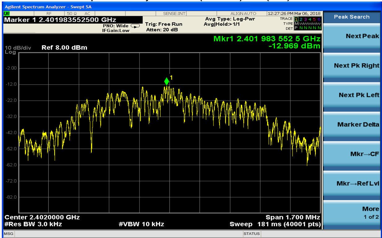
Plot 8-10: Power Spectral Density: Channel 0 (2402 MHz): BLE (0x55)
