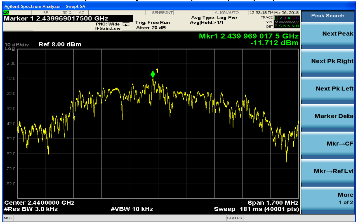
Plot 8-8: Power Spectral Density: Channel 19 (2440 MHz): BLE (0x0F)
