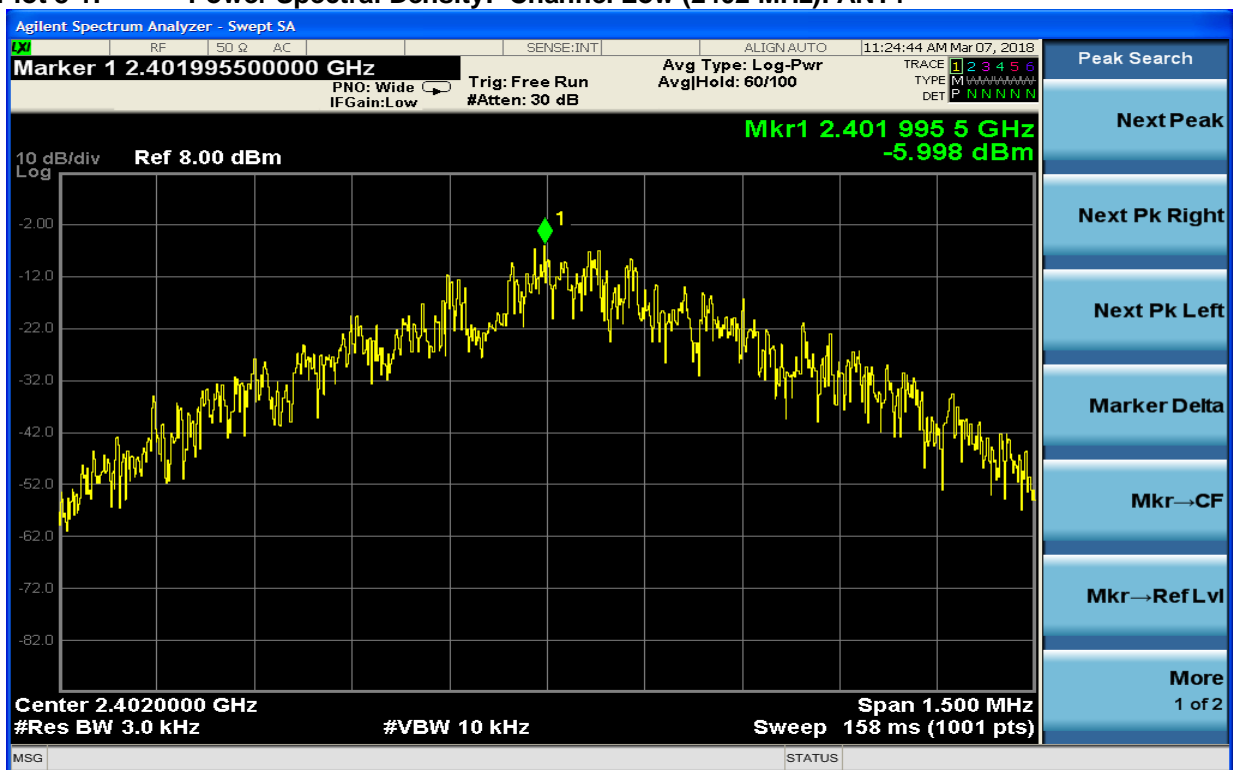
Plot 8-1: Power Spectral Density: Channel Low (2402 MHz): ANT+
