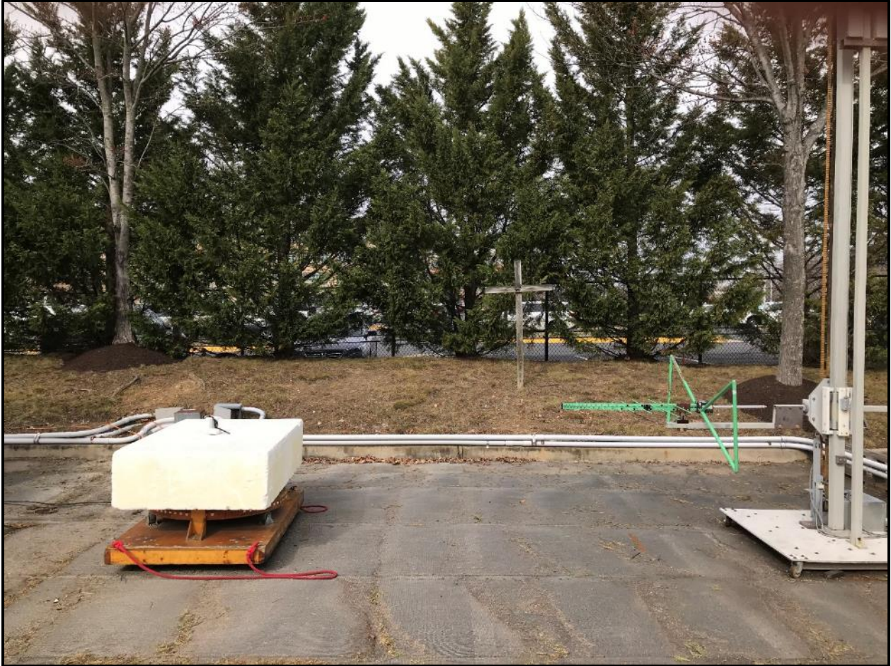
Photograph 1: Radiated Emissions Testing – Side View (Above 30 MHz, below 1 GHz)
