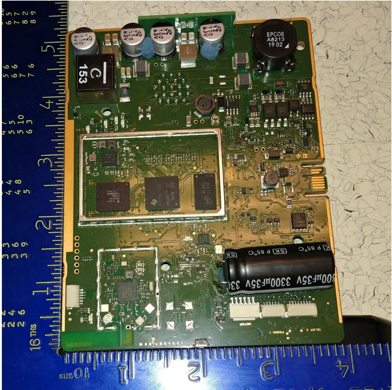
Main board top, shield off
