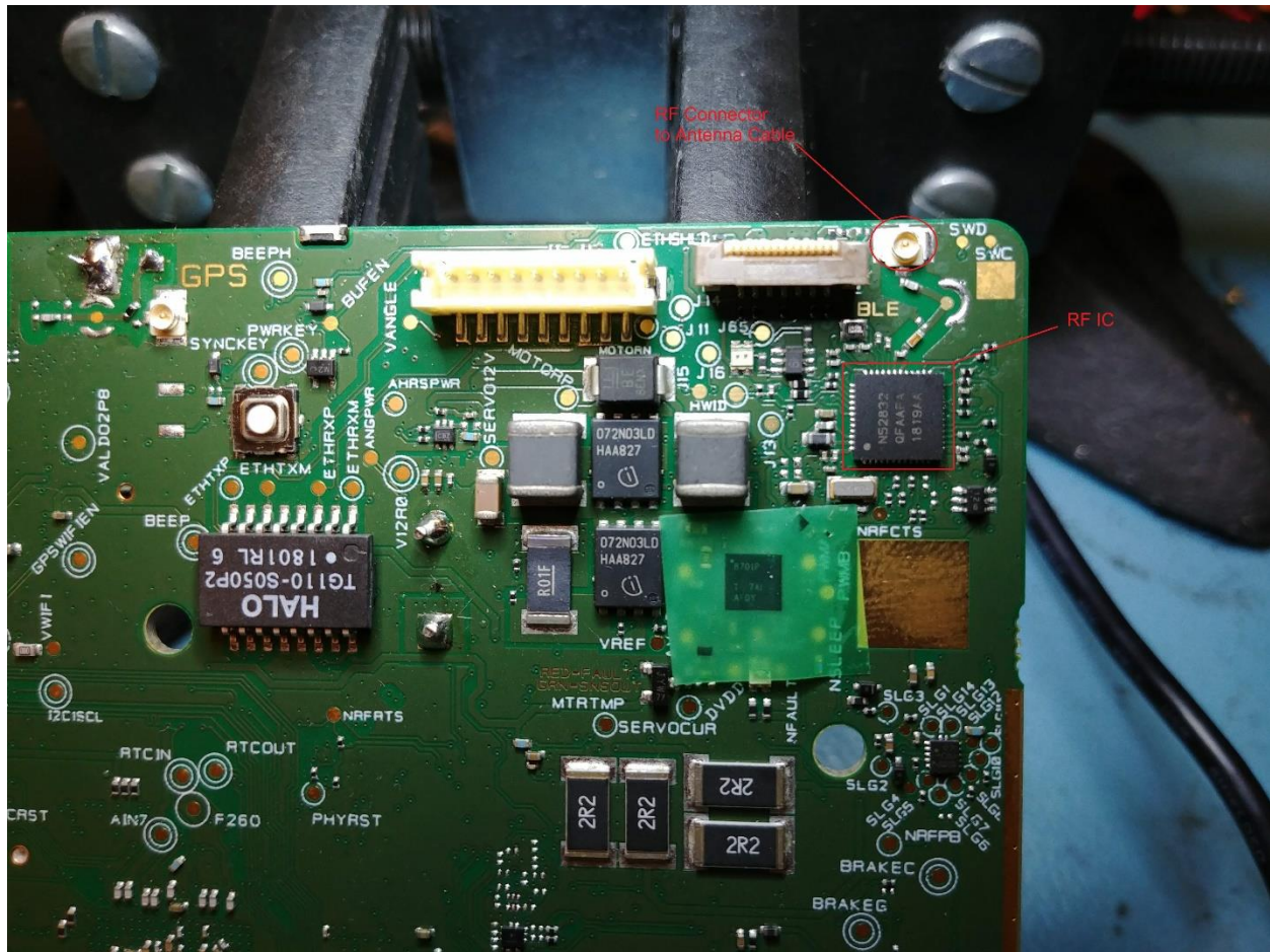
BLE Radio section, antenna connector
