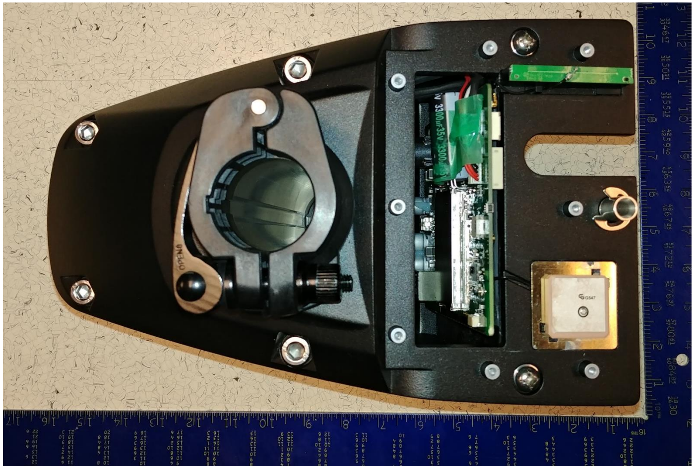
Top view, no cover
