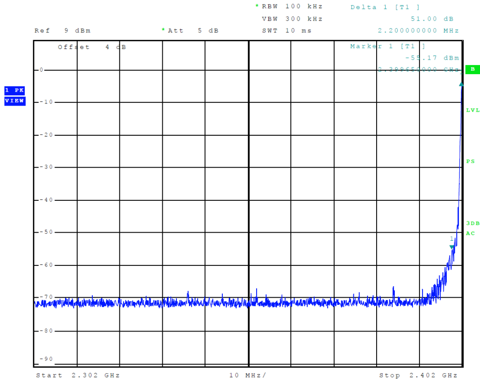
Figure 9 Plot of Transmitter Emissions (Low Band Edge, ANT mode 1)
