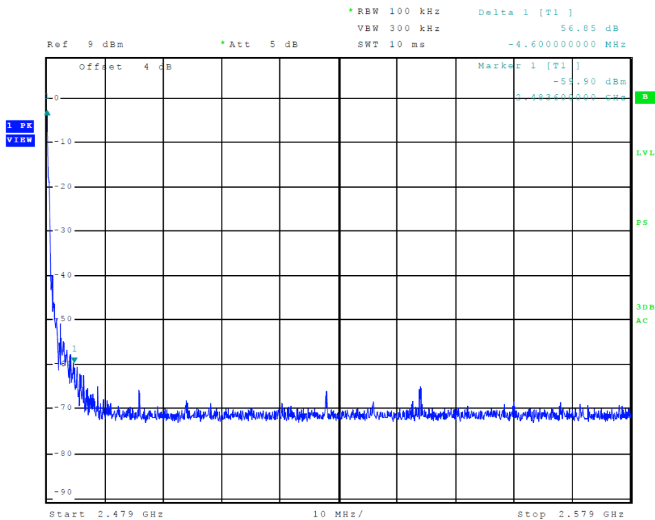
Figure 10 Plot of Transmitter Emissions (High Band Edge, ANT mode 1)
