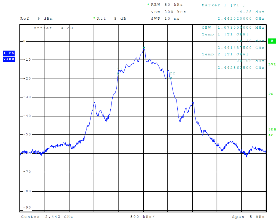
Figure 12 Plot of Transmitter Emissions (99% Occupied Bandwidth, BLE mode 2)
