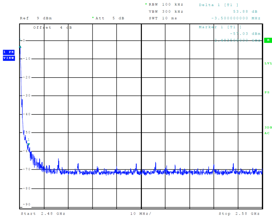
Figure 14 Plot of Transmitter Emissions (High Band Edge, BLE mode 2)
