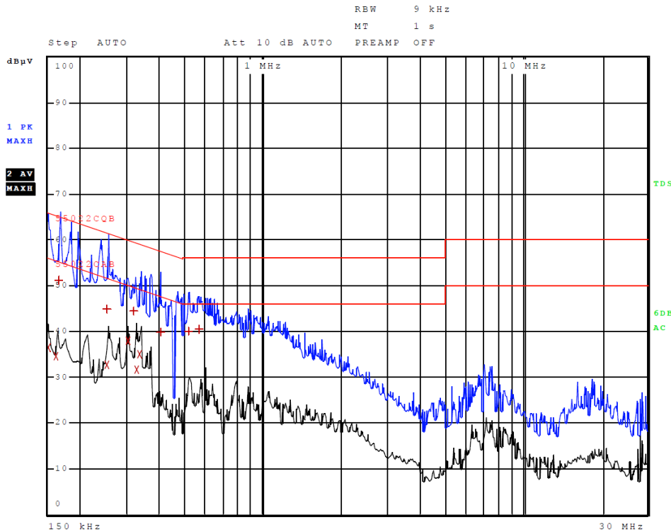
Figure 5 AC Line Conducted emissions of EUT line 1 (#4, EUT – USB – Computer)
