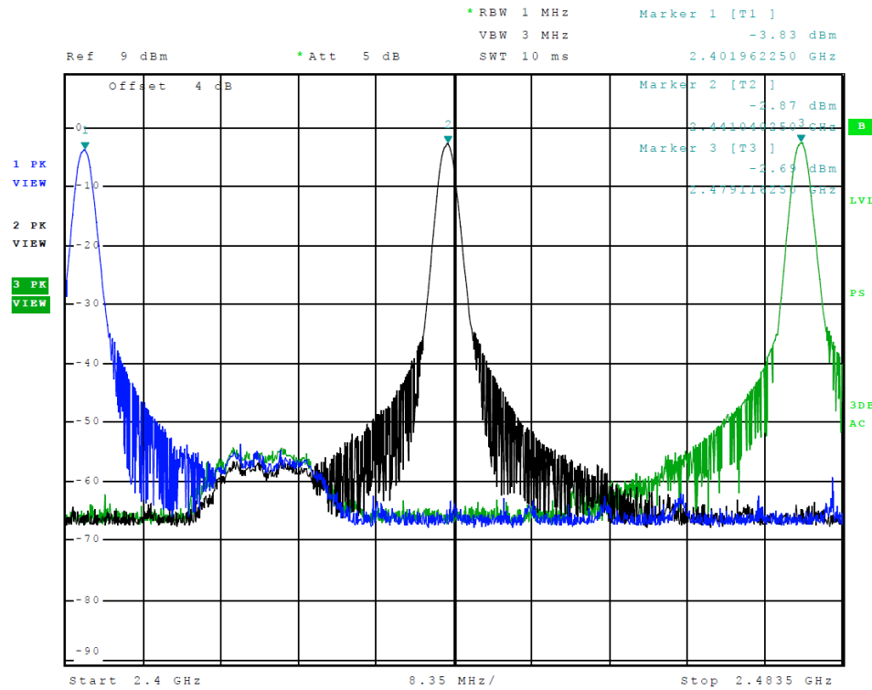
Figure 7 Plot of Transmitter Emissions (Operation in 2402-2480 MHz, ANT mode 1)
