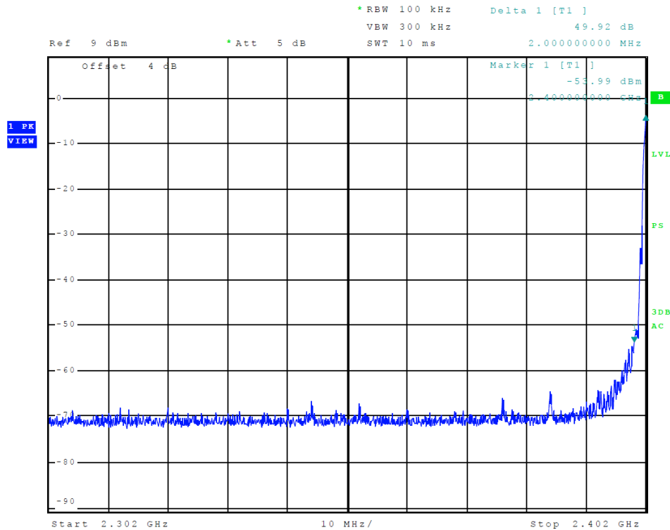
Figure 13 Plot of Transmitter Emissions (Low Band Edge, BLE mode 2)
