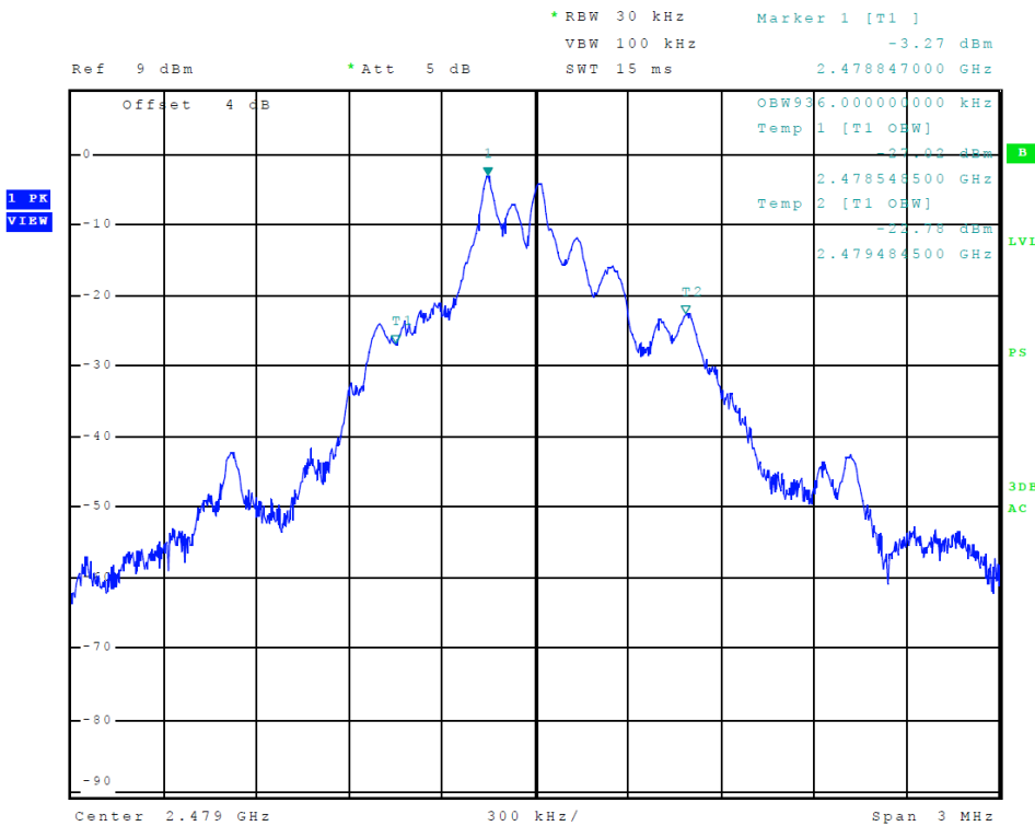
Figure 8 Plot of Transmitter Emissions (99% Occupied Bandwidth, ANT mode 1)
