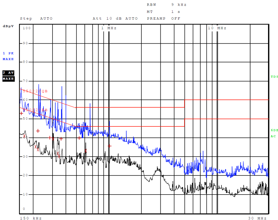
Figure 6 AC Line Conducted emissions of EUT line 2 (#4, EUT – USB – Computer)
