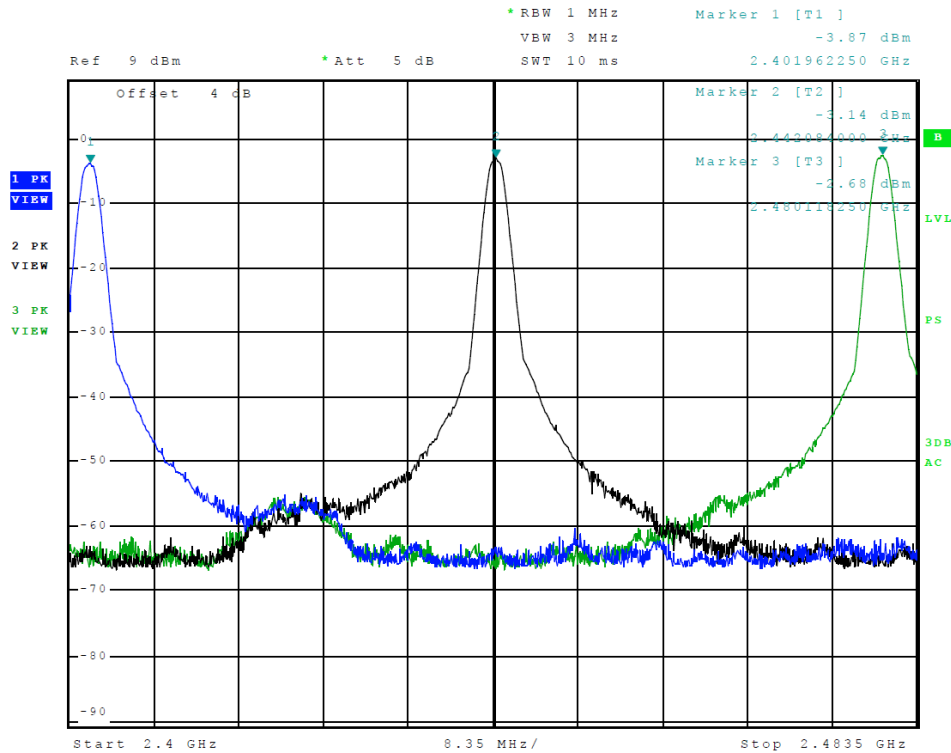
Figure 11 Plot of Transmitter Emissions (Operation in 2402-2480 MHz, BLE mode 2)
