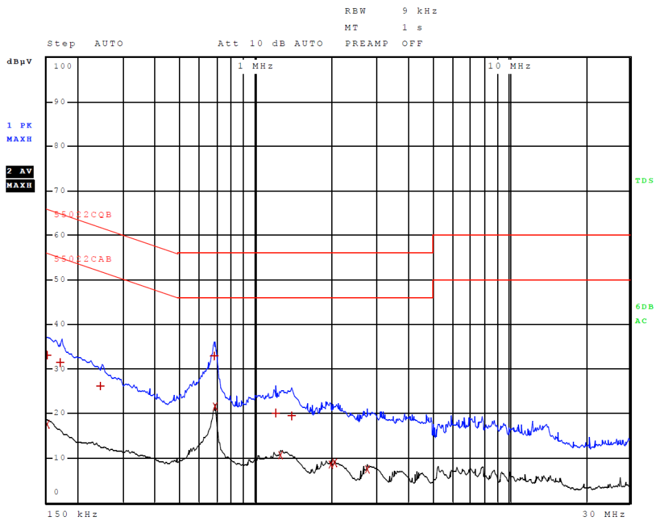
Figure 2 AC Line Conducted emissions of EUT line 2 (#2 and 3, EUT – 362-00096-00)
