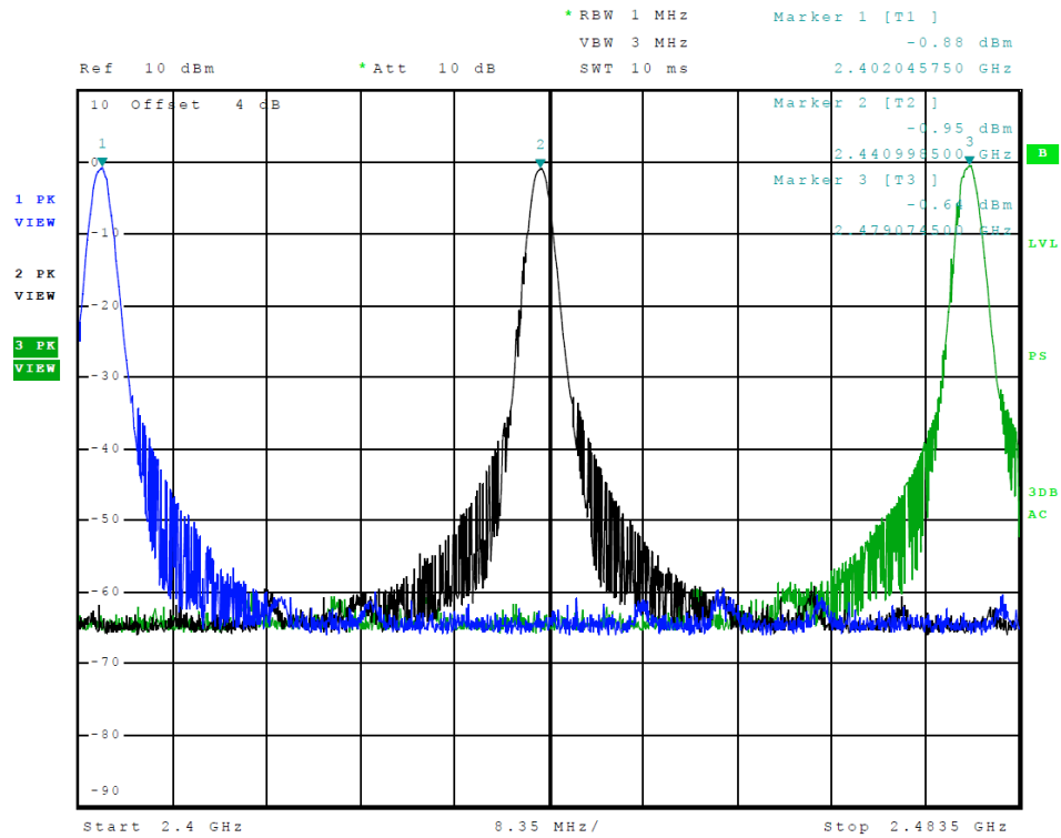
Figure 7 Plot of Transmitter Emissions (Operation in 2402-2480 MHz, ANT)
