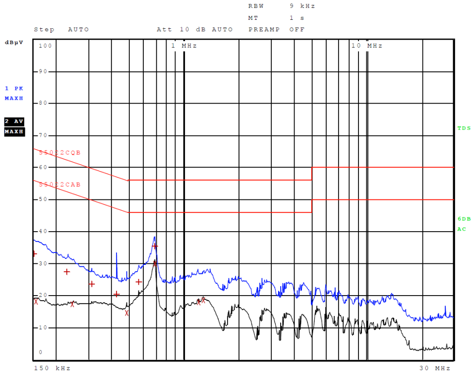
Figure 1 AC Line Conducted emissions of EUT line 1 (#2 and 3, EUT – 362-00096-00)
