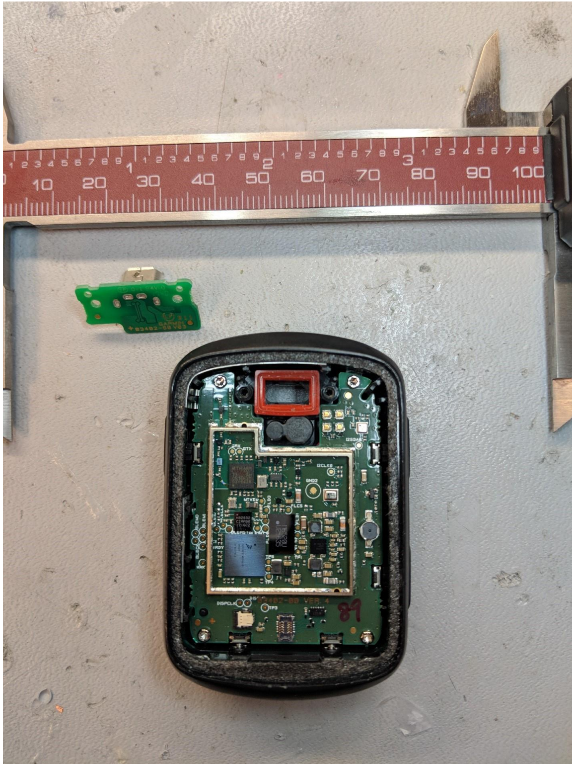
Main PCB side A with shield cover removed and Micro USB PCB
