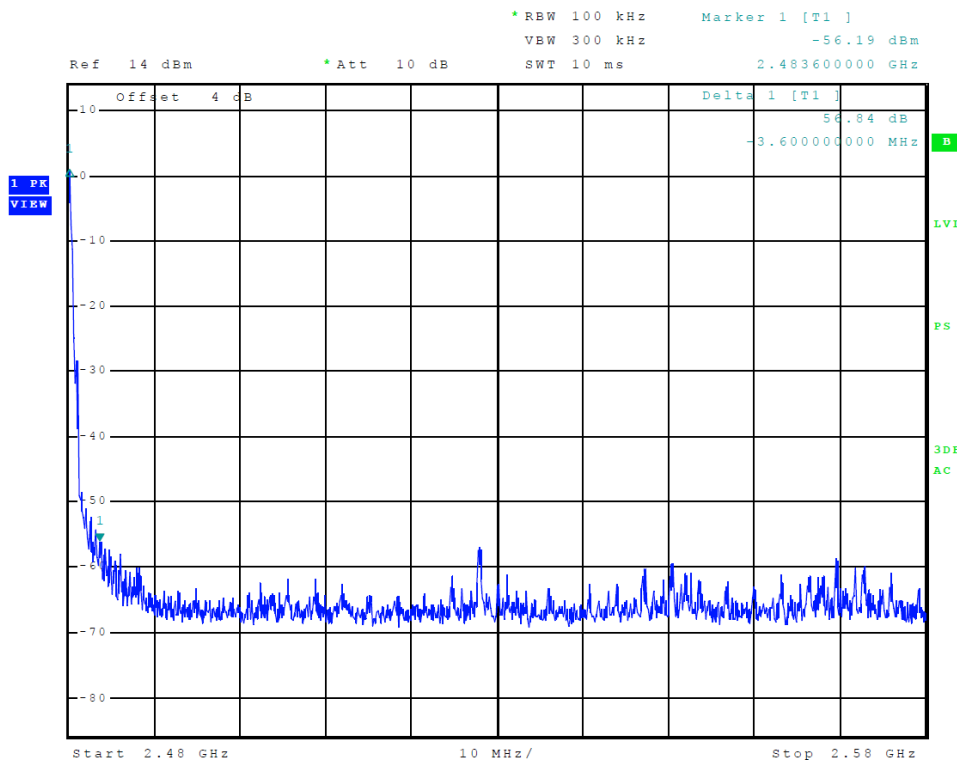
Figure 12 Plot of Transmitter Emissions (High Band Edge, BLE R)
