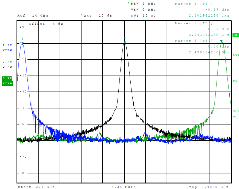
Figure 1 Plot of Transmitter Emissions (Operation in 2402-2479 MHz, ANT)
