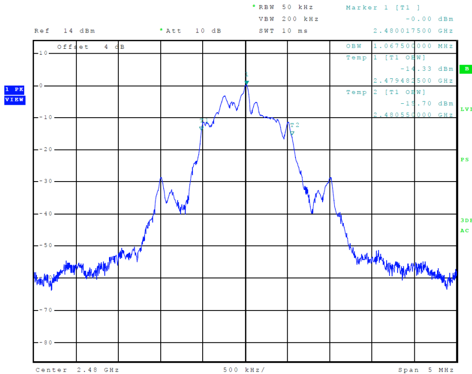
Figure 10 Plot of Transmitter Emissions (99% Occupied Bandwidth, BLE R)
