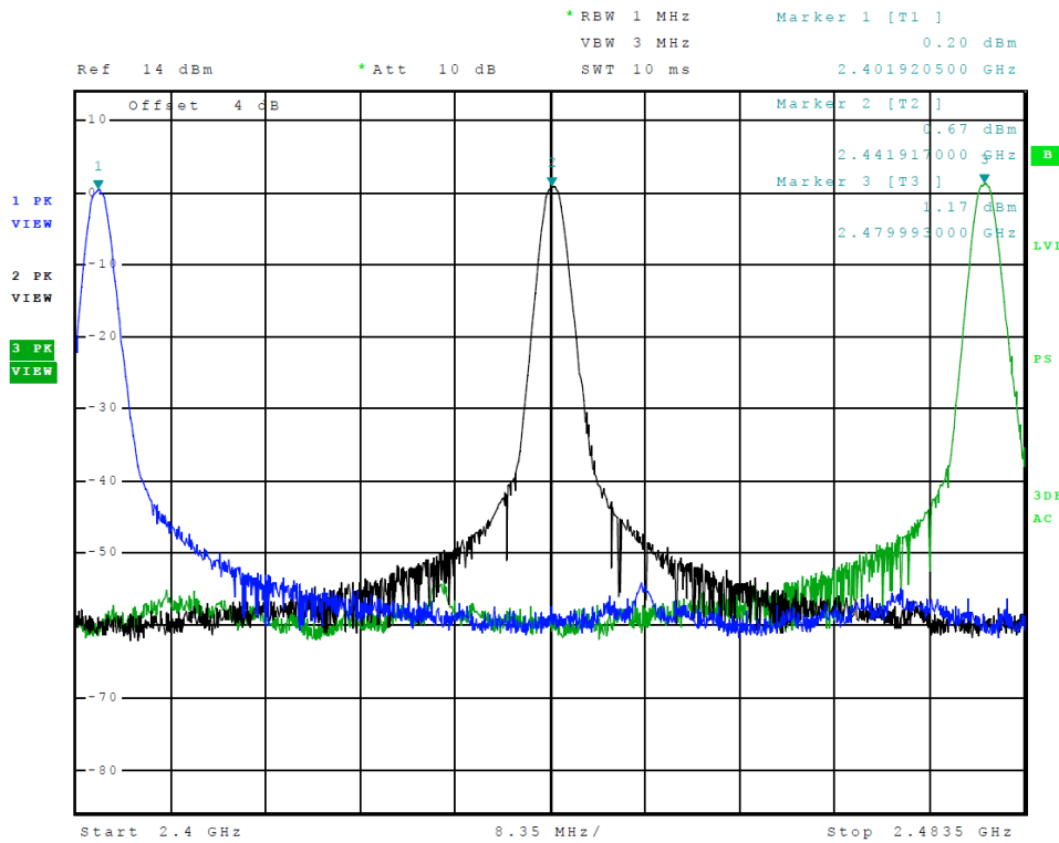
Figure 9 Plot of Transmitter Emissions (Operation in 2402-2480 MHz, BLE R)
