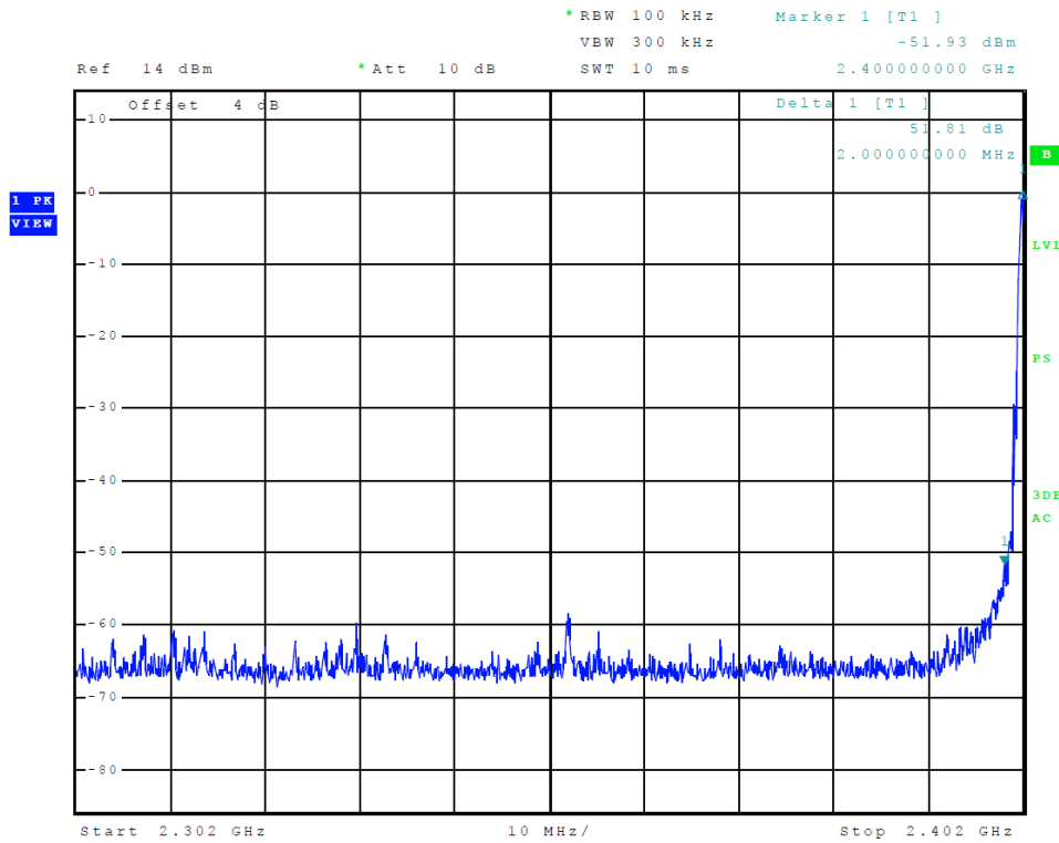
Figure 11 Plot of Transmitter Emissions (Low Band Edge, BLE R)
