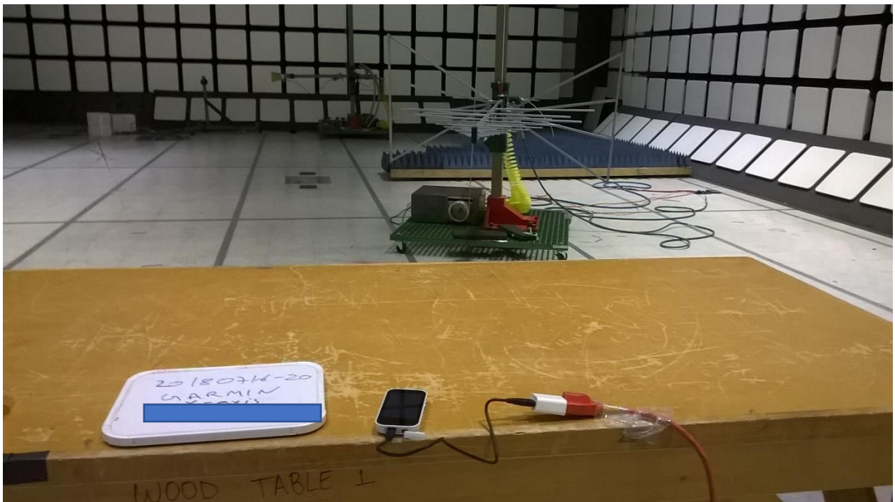
Figure 2 - Radiated Emissions Test Setup, 30 MHz - 1 GHz (EUT not shown)
