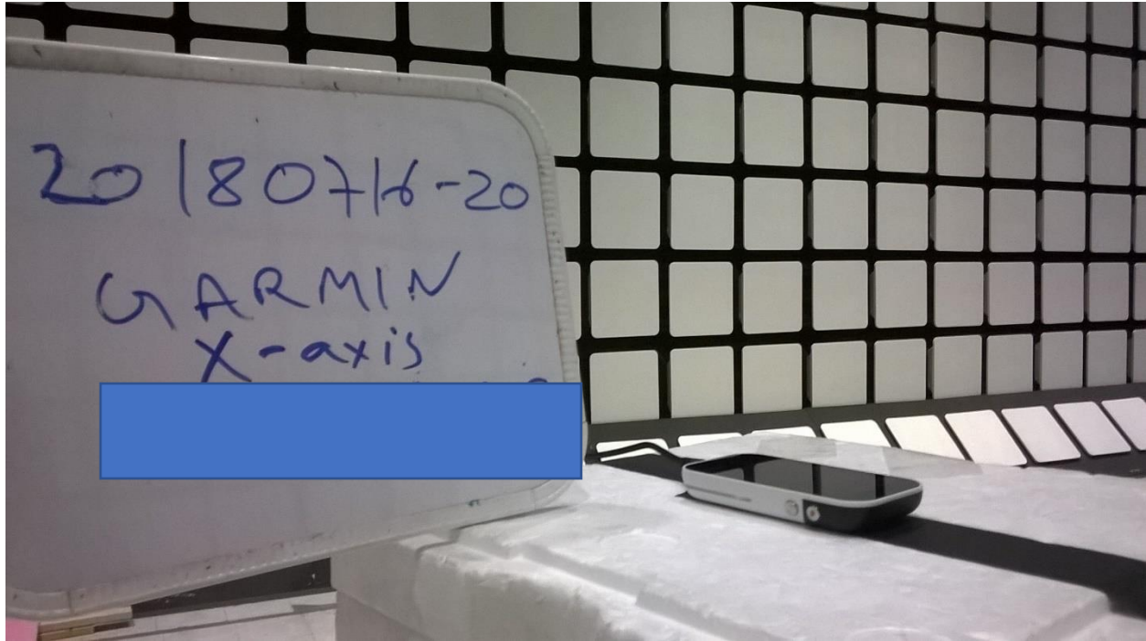
Figure 3 - Radiated Emissions Test Setup, X-axis
