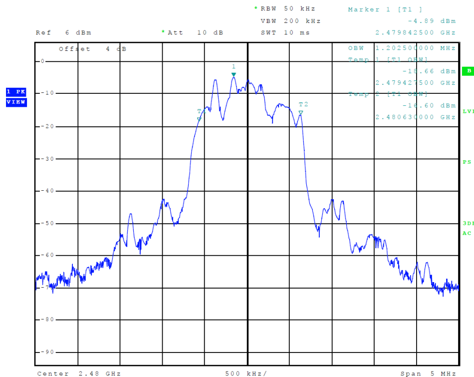
Figure 16 Plot of Transmitter Emissions (99% Occupied Bandwidth, BT 3EDR)
