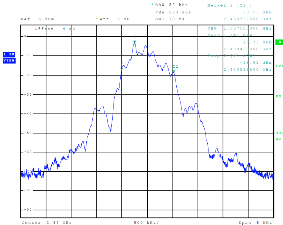
Figure 8 Plot of Transmitter Emissions (99% Occupied Bandwidth, BLE)
