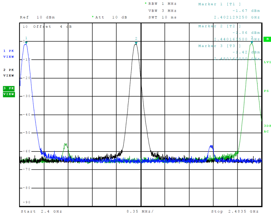
Figure 7 Plot of Transmitter Emissions (Operation in 2402-2480 MHz, BLE)
