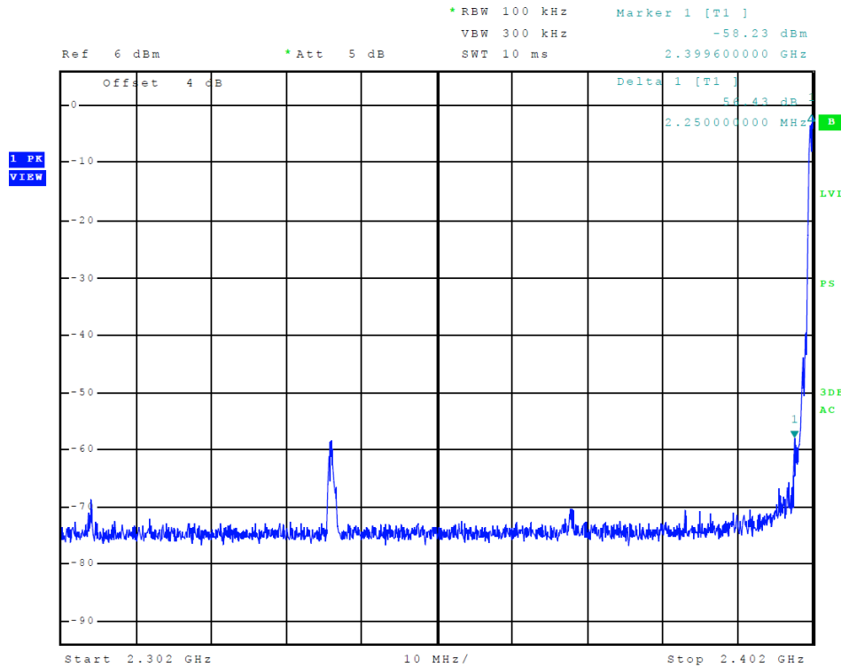
Figure 13 Plot of Transmitter Emissions (Low Band Edge, BT 2EDR)
