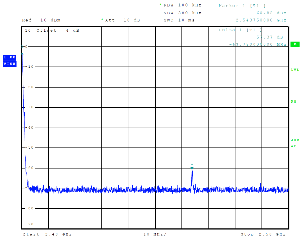
Figure 10 Plot of Transmitter Emissions (High Band Edge, BLE)
