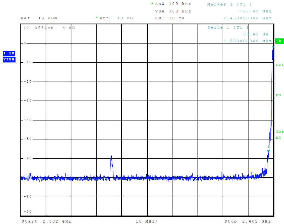
Figure 17 Plot of Transmitter Emissions (Low Band Edge, BT 3EDR)
