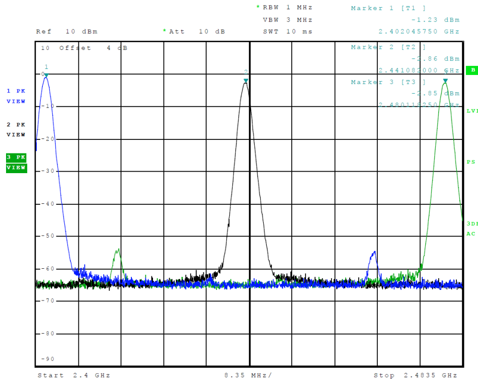
Figure 15 Plot of Transmitter Emissions (Operation in 2402-2480 MHz, 3EDR)
