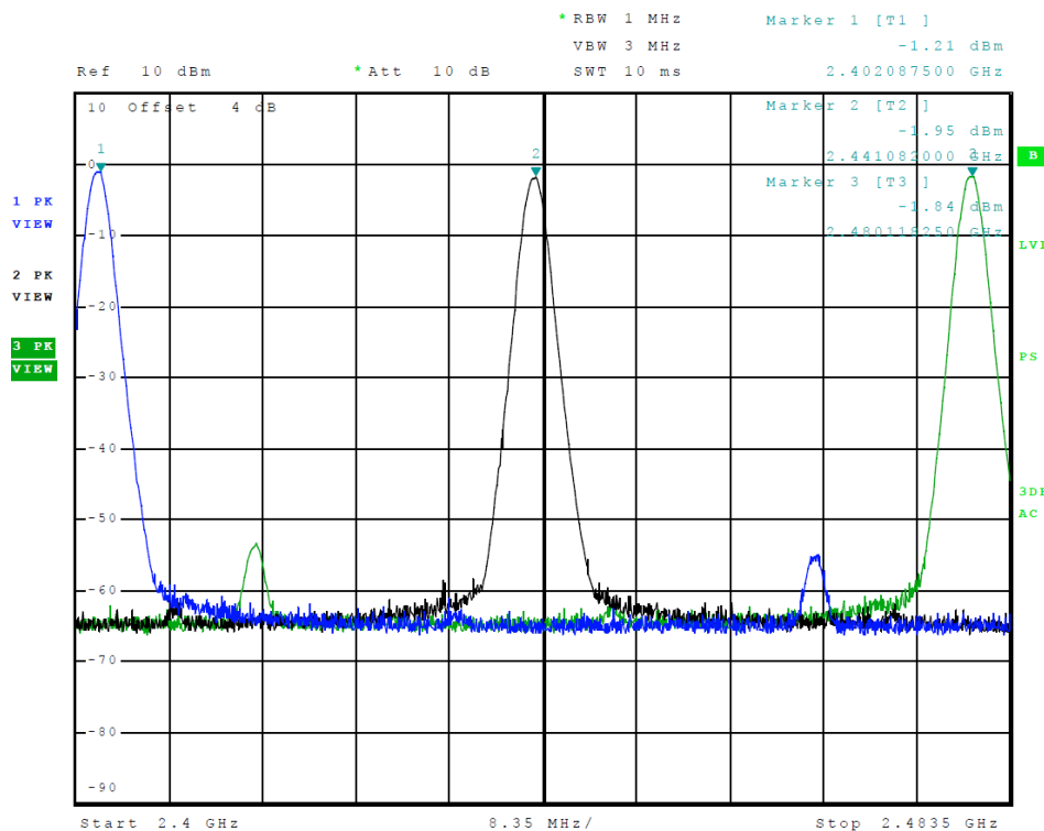
Figure 11 Plot of Transmitter Emissions (Operation in 2402-2480 MHz, BT 2EDR)
