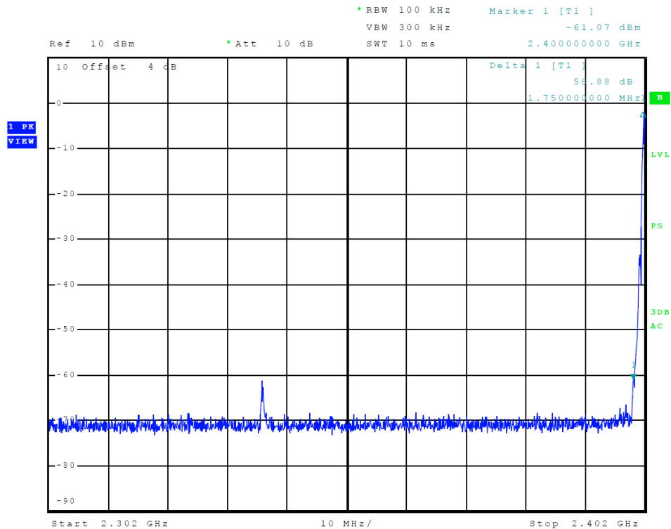
Figure 9 Plot of Transmitter Emissions (Low Band Edge, BLE)
