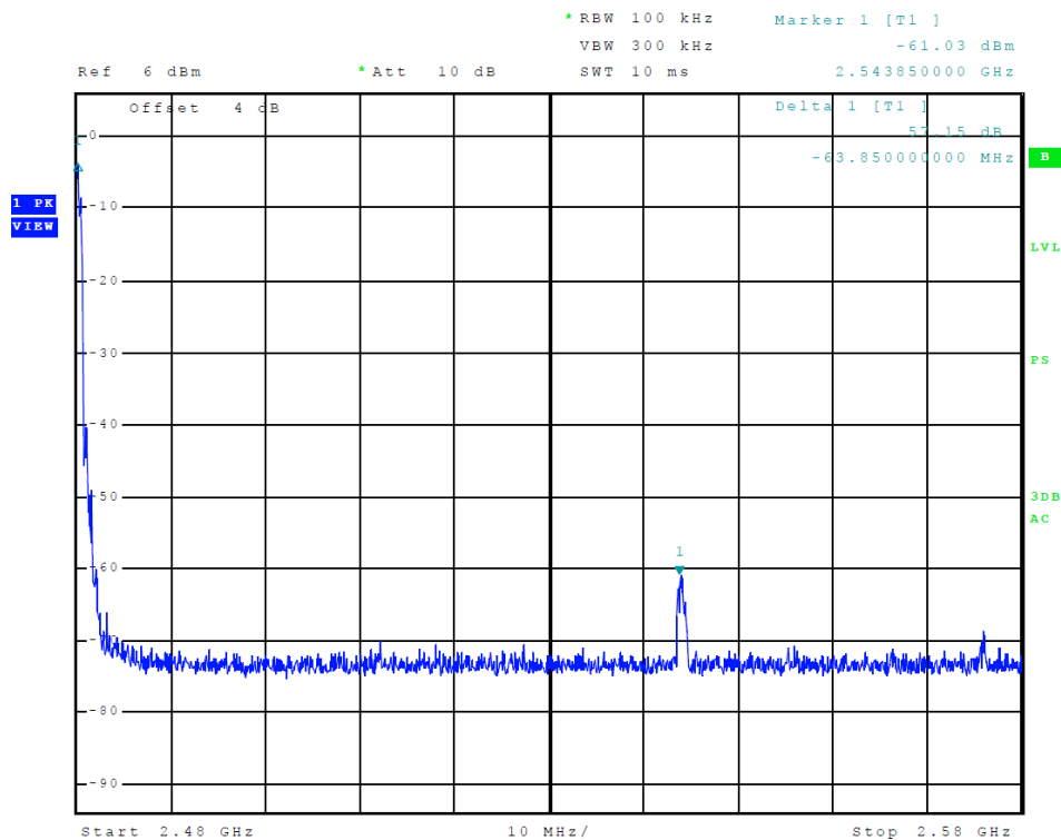
Figure 18 Plot of Transmitter Emissions (High Band Edge, BT 3EDR)
