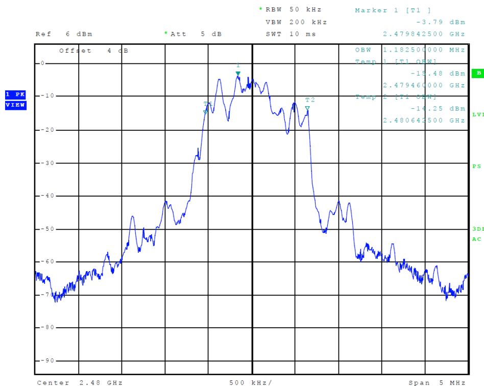
Figure 12 Plot of Transmitter Emissions (99% Occupied Bandwidth, BT 2EDR)
