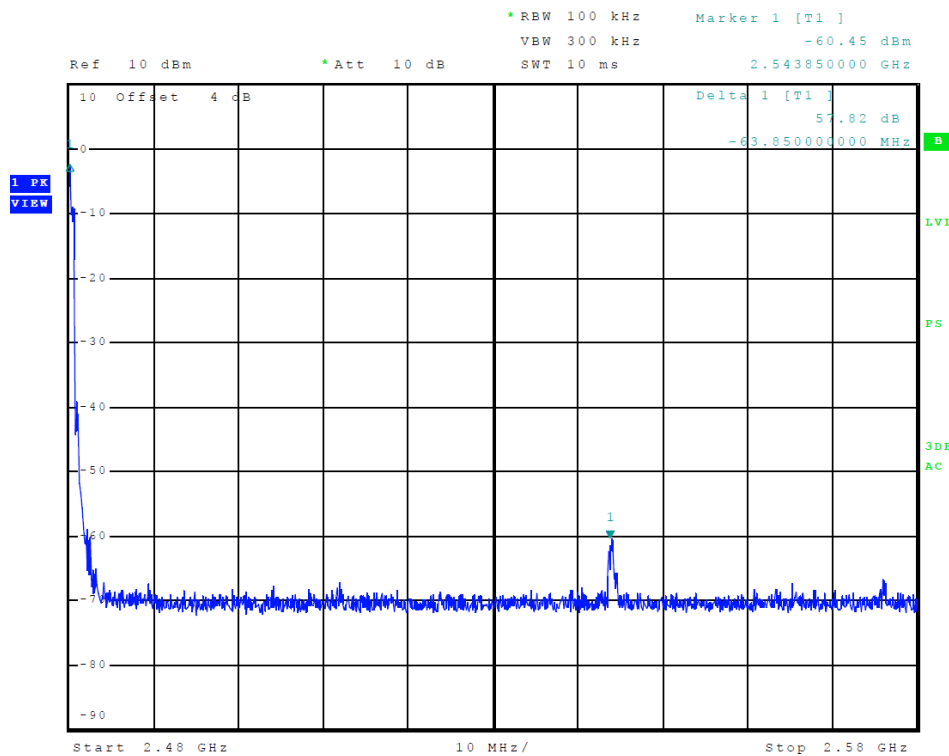
Figure 14 Plot of Transmitter Emissions (High Band Edge, BT 2EDR)
