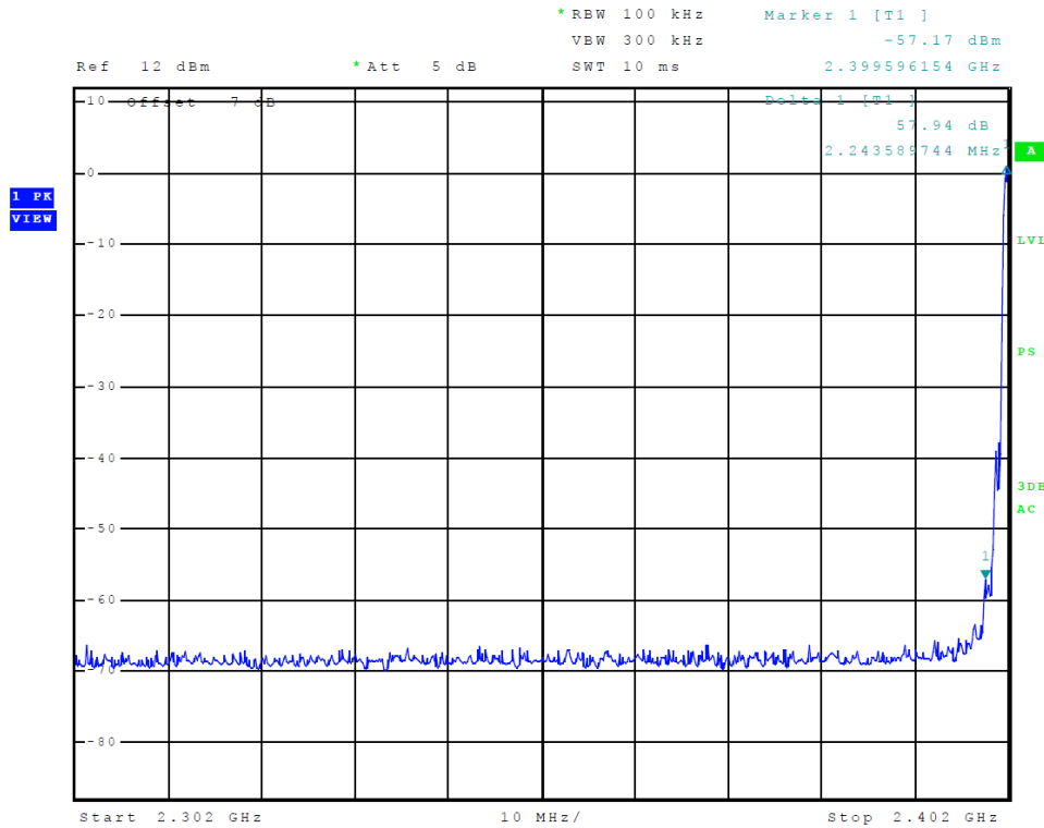
Figure 15 Plot of Transmitter Emissions (Low Band Edge, BT PI/4DQPSK)
