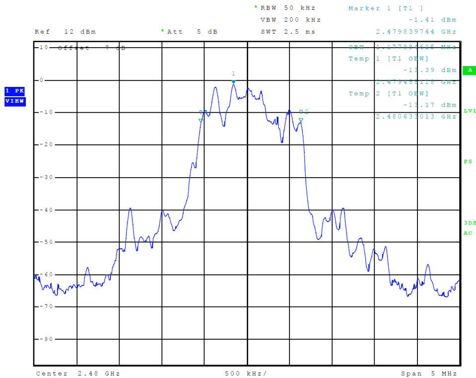
Figure 14 Plot of Transmitter Emissions (99% Occupied Bandwidth, BT PI/4DQPSK)
