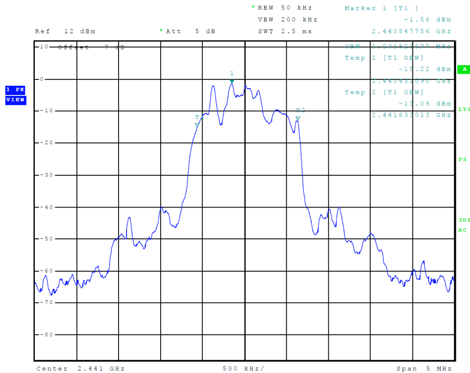
Figure 18 Plot of Transmitter Emissions (99% Occupied Bandwidth, BT 8-DPSK)
