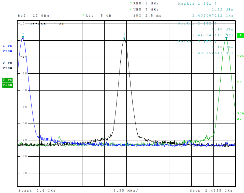
Figure 13 Plot of Transmitter Emissions (Operation in 2402-2480 MHz, BT PI/4DQPSK)
