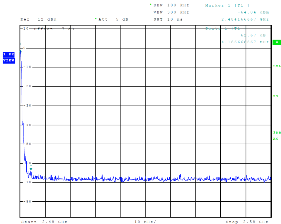
Figure 16 Plot of Transmitter Emissions (High Band Edge, BT PI/4DQPSK)
