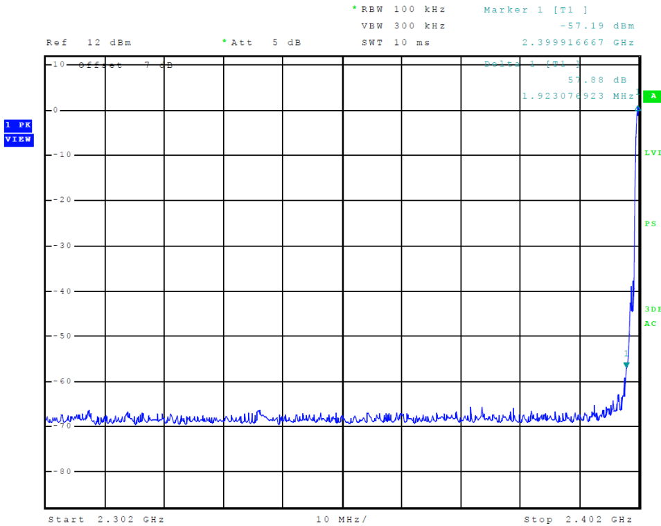
Figure 19 Plot of Transmitter Emissions (Low Band Edge, BT 8-DPSK)
