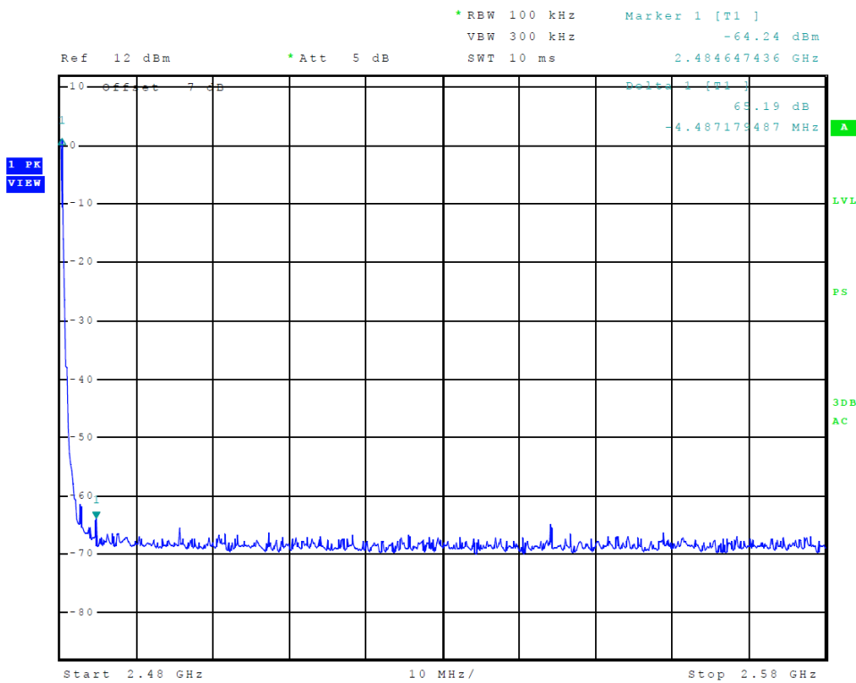
Figure 12 Plot of Transmitter Emissions (High Band Edge, BT GFSK)
