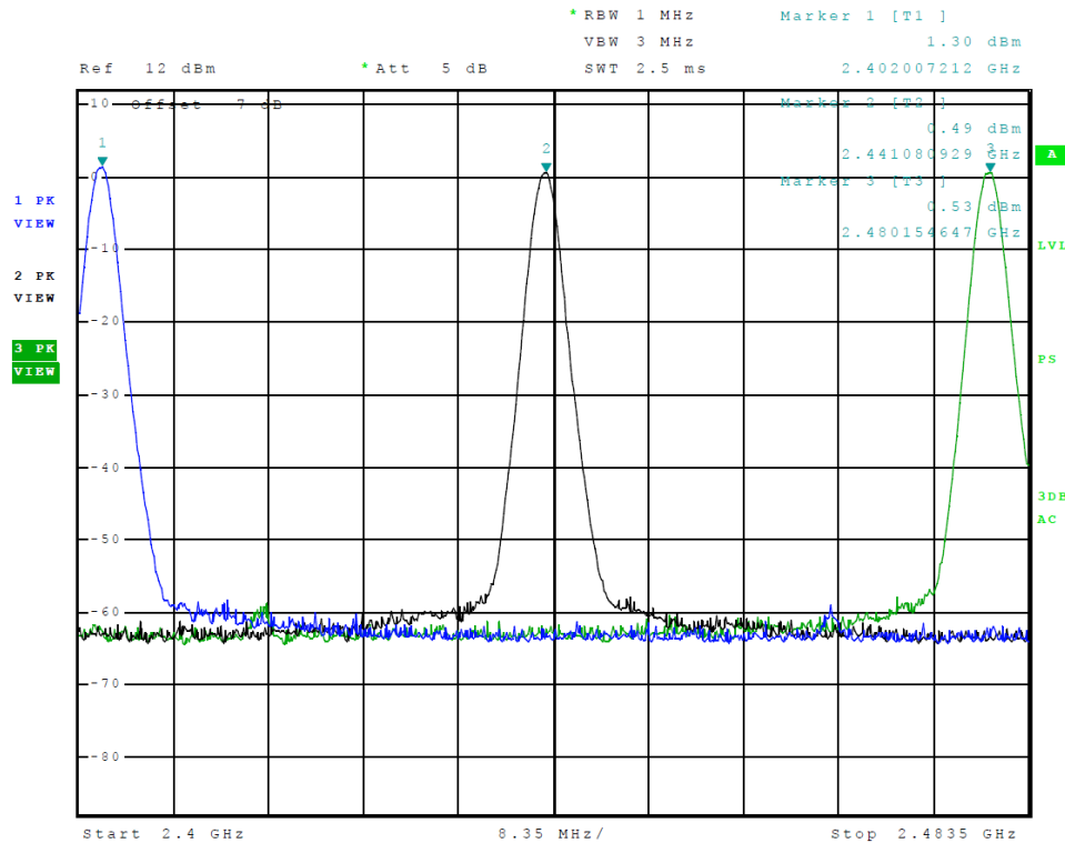
Figure 17 Plot of Transmitter Emissions (Operation in 2402-2480 MHz, BT 8-DPSK)
