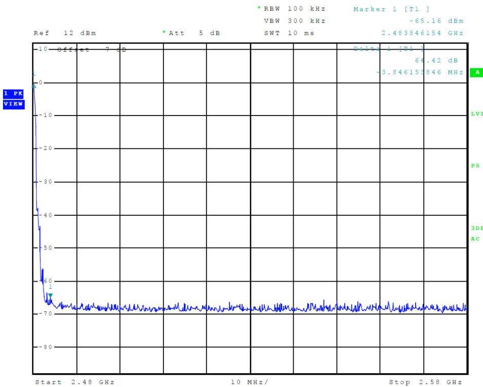
Figure 20 Plot of Transmitter Emissions (High Band Edge, BT 8-DPSK)
