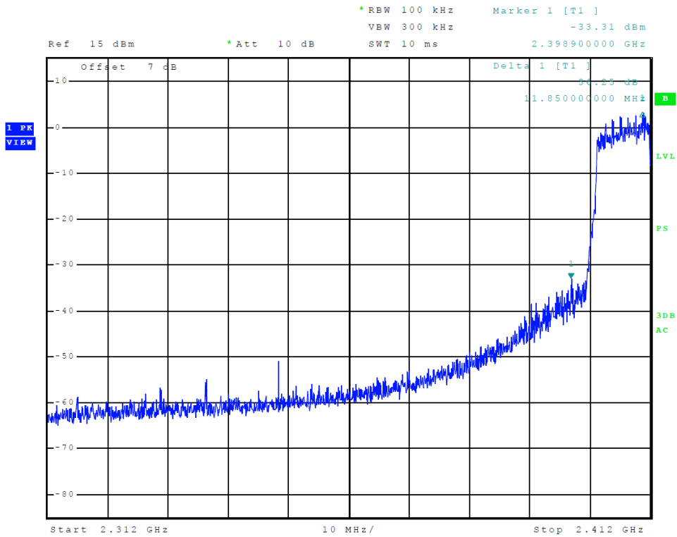
Figure 12 Plot of Lower Band Edge (802.11 n-mode)
