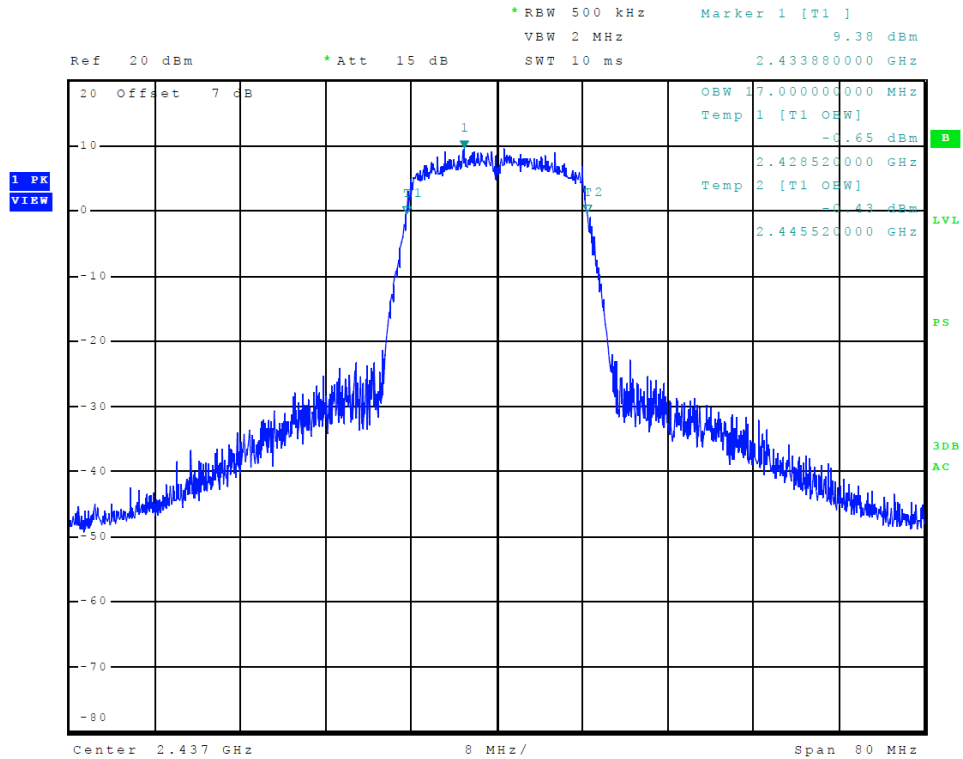
Figure 21 Plot of Transmitter 99% Occupied Bandwidth (802.11 g-mode)
