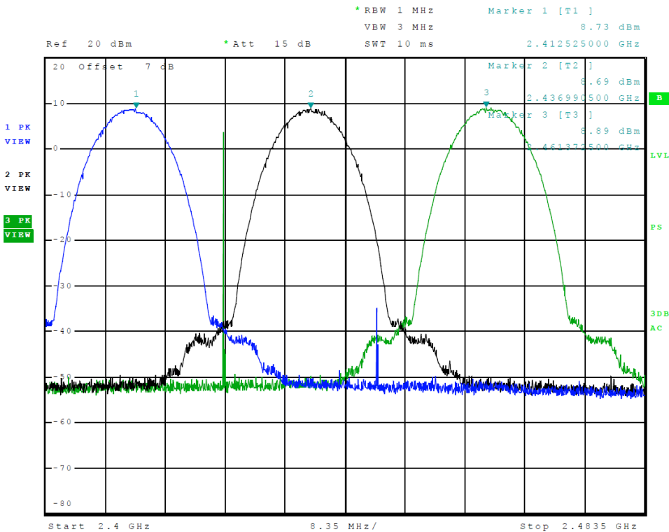
Figure 6 Plot of Transmitter Emissions in Operational Frequency (802.11 b-Mode)
