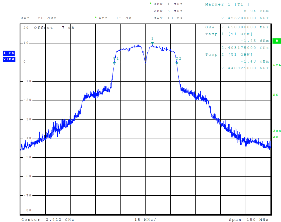
Figure 25 Plot of Transmitter 99% Occupied Bandwidth (802.11 n40-mode)
