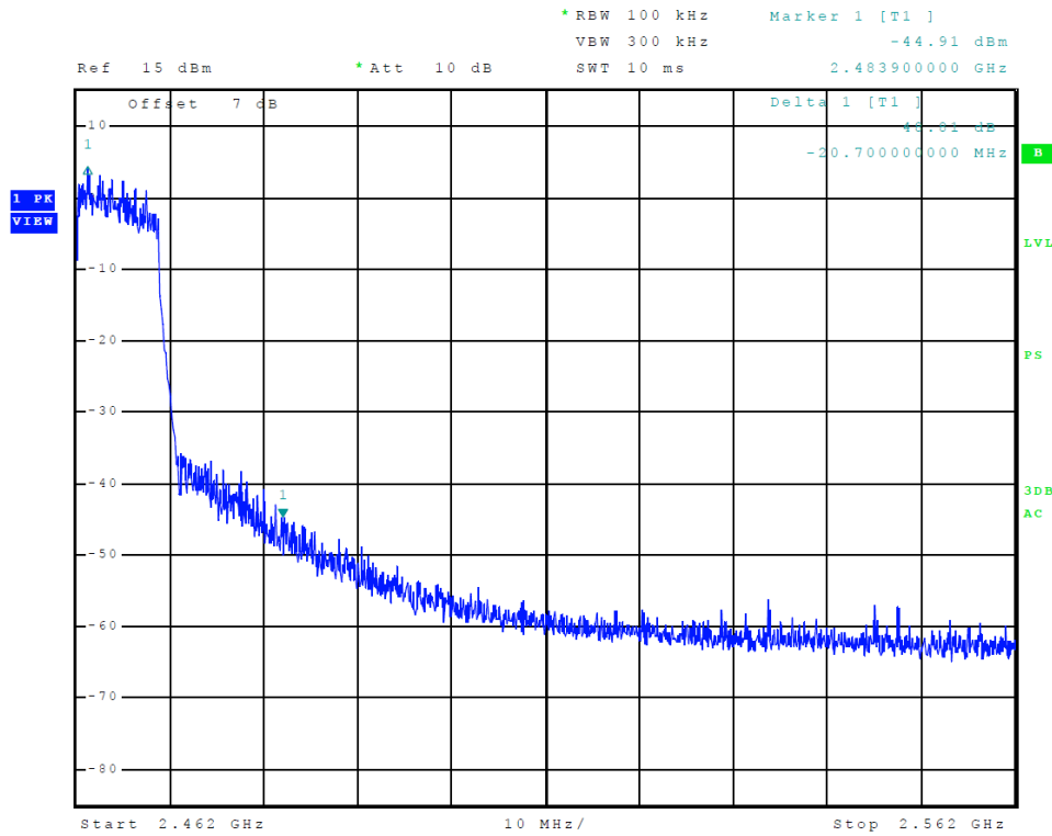
Figure 16 Plot of Upper Band Edge (802.11 n-mode)
