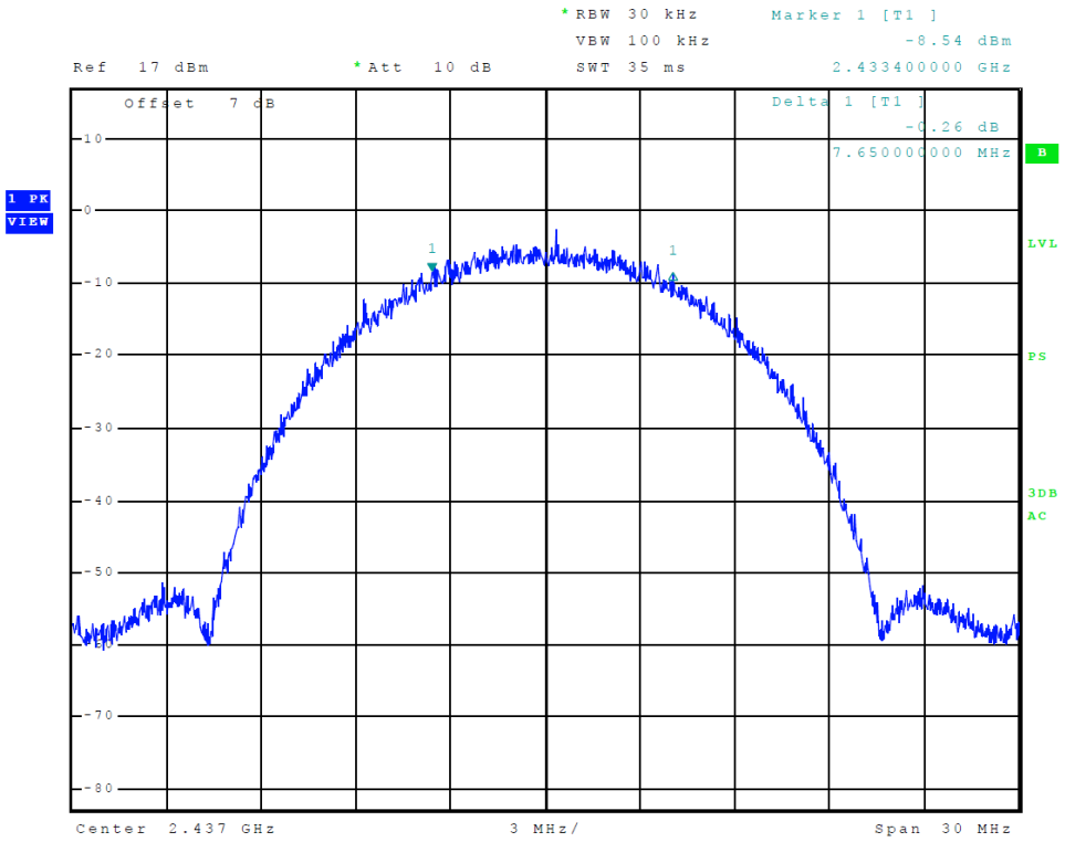
Figure 18 Plot of Transmitter 6-dB Occupied Bandwidth (802.11 b-mode)
