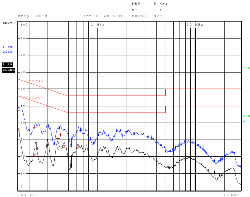
Figure 4 AC Line Conducted emissions of EUT line 2 (#3, EUT – 320-00086-01)
