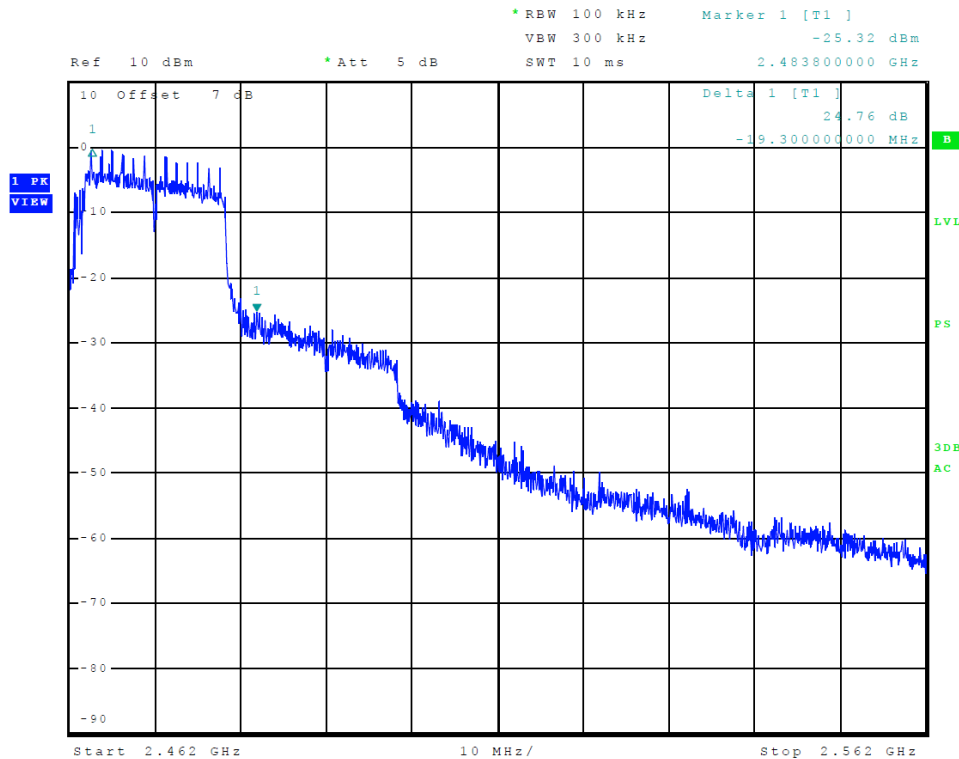
Figure 17 Plot of Upper Band Edge (802.11 n40-mode)
