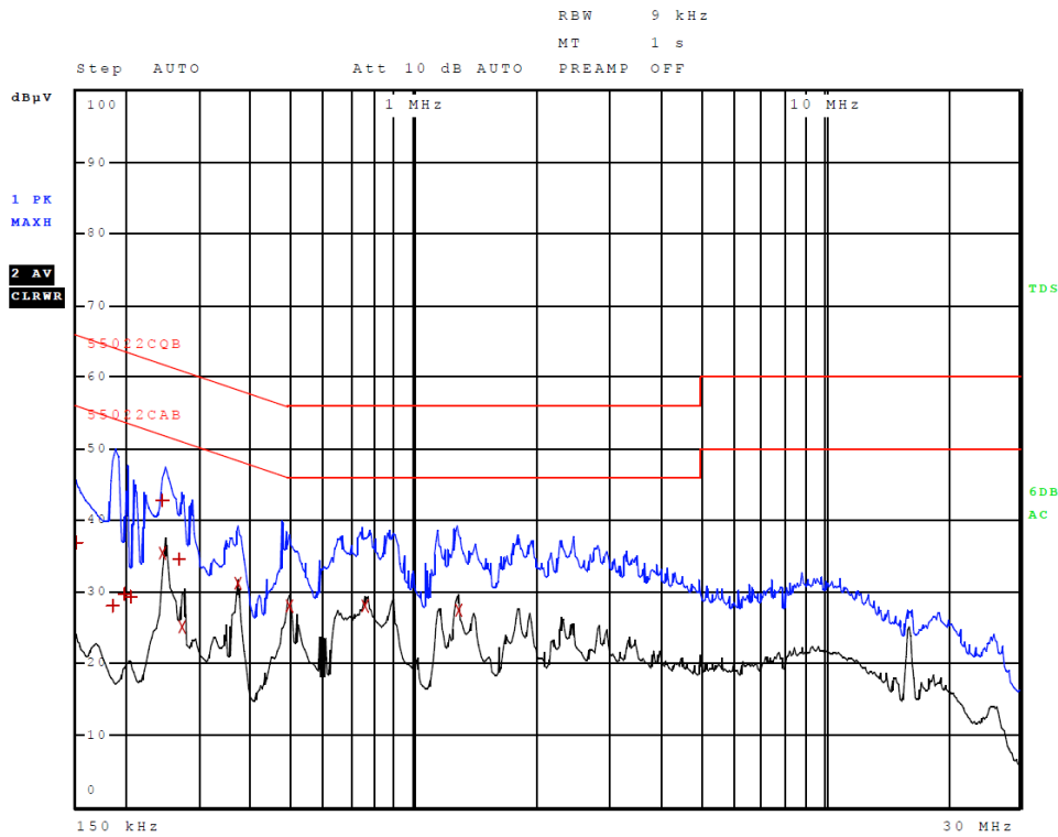
Figure 3 AC Line Conducted emissions of EUT line 1 (#3, EUT – 320-00086-01)
