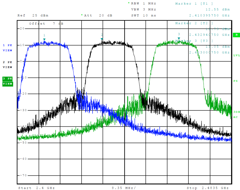
Figure 7 Plot of Transmitter Emissions in Operational Frequency (802.11 g-Mode)
