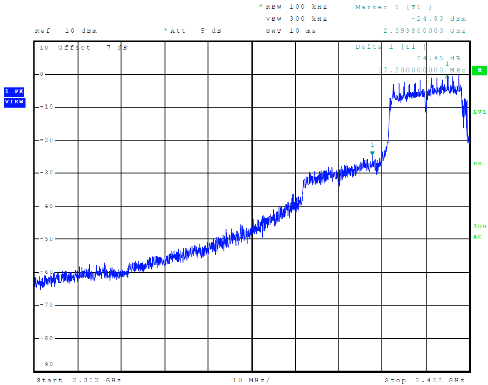
Figure 13 Plot of Lower Band Edge (802.11 n40-mode)
