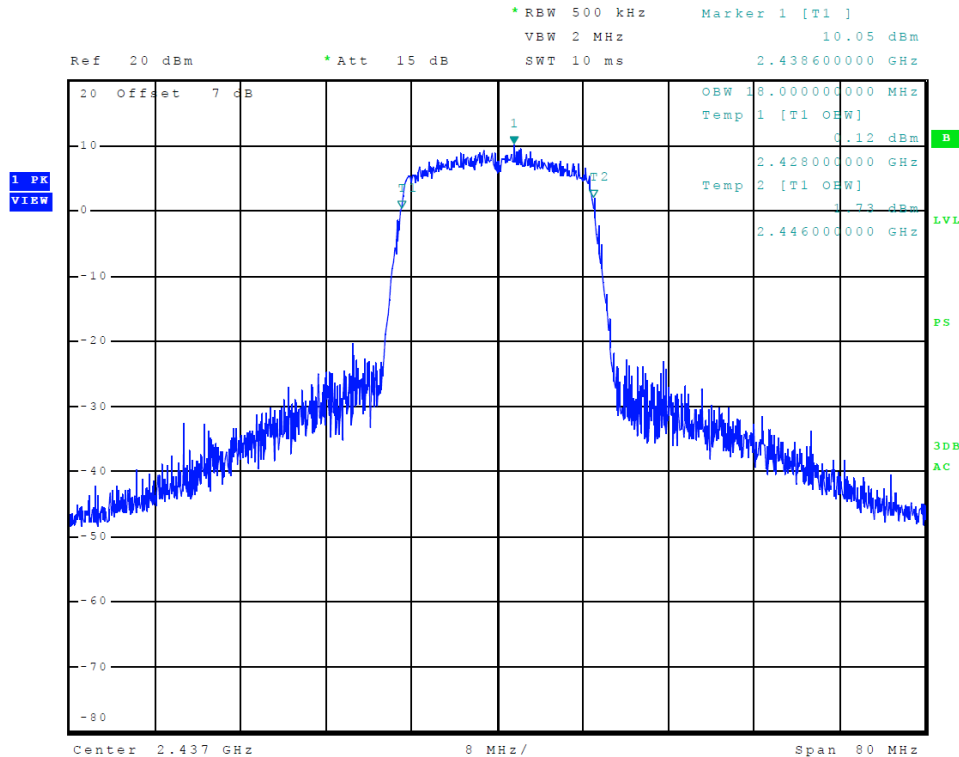
Figure 23 Plot of Transmitter 99% Occupied Bandwidth (802.11 n-mode)
