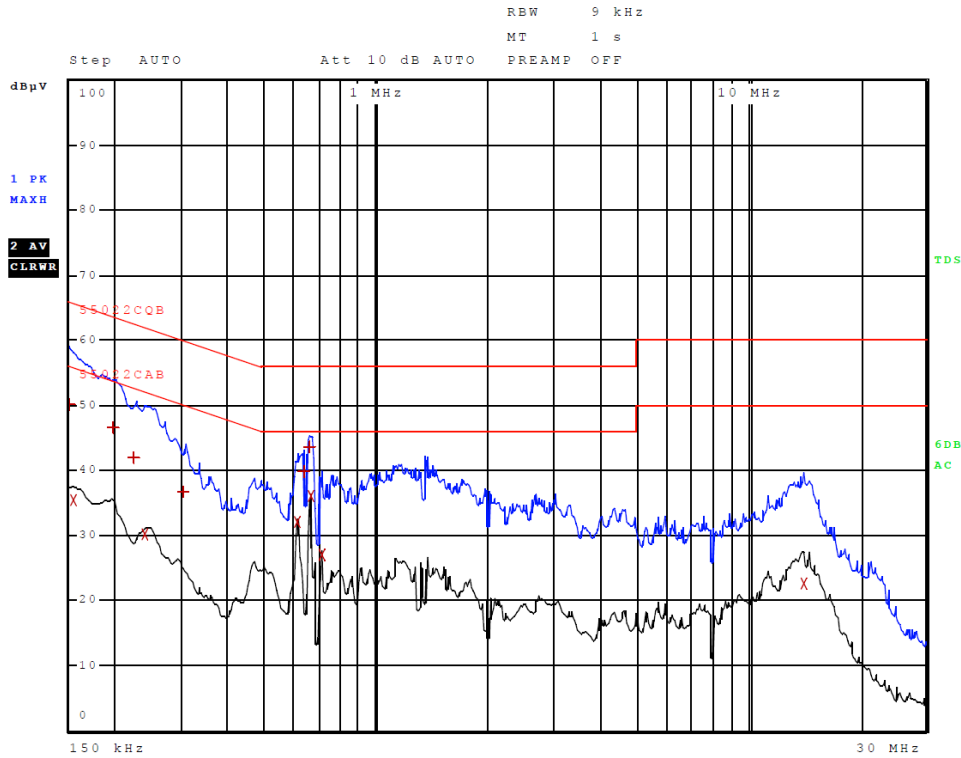
Figure 1 AC Line Conducted emissions of EUT line 1 (#2, EUT – 320-00096-xx)
