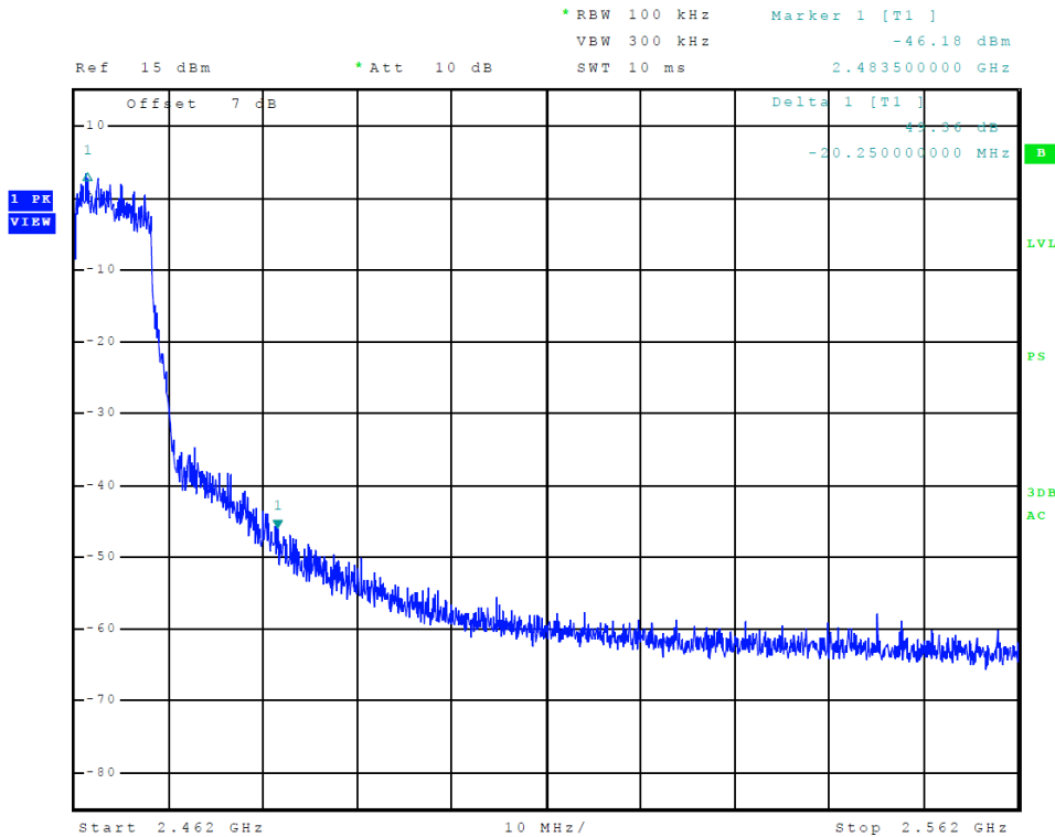
Figure 15 Plot of Upper Band Edge (802.11 g-mode)
