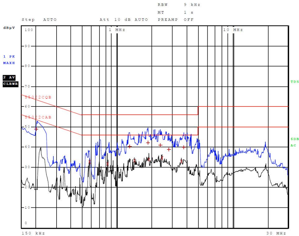
Figure 5 AC Line Conducted emissions of EUT line 1 (#4, EUT – CPU)
