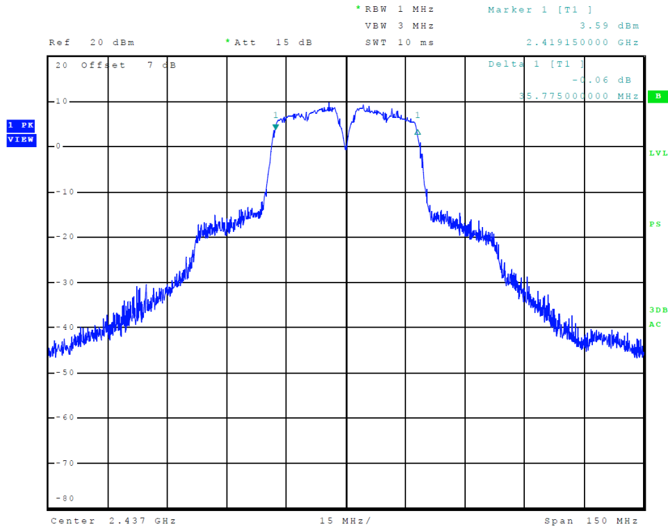
Figure 24 Plot of Transmitter 6-dB Occupied Bandwidth (802.11 n40-mode)
