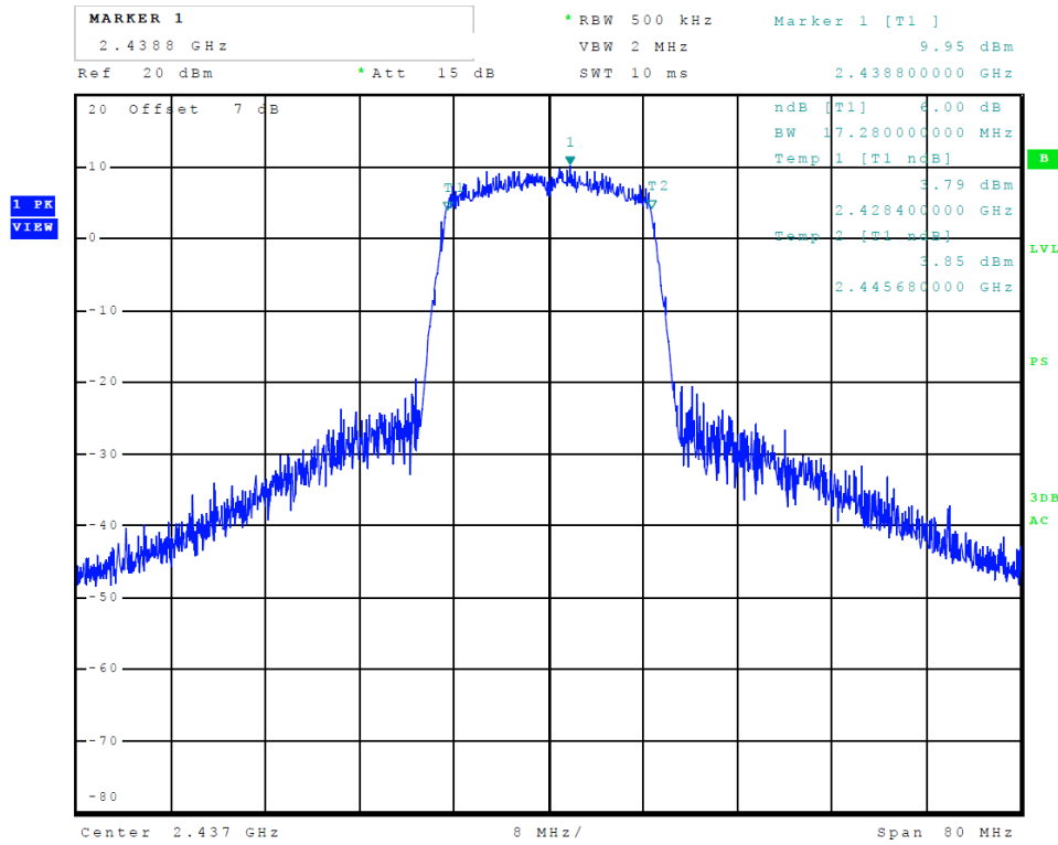
Figure 22 Plot of Transmitter 6-dB Occupied Bandwidth (802.11 n-mode)
