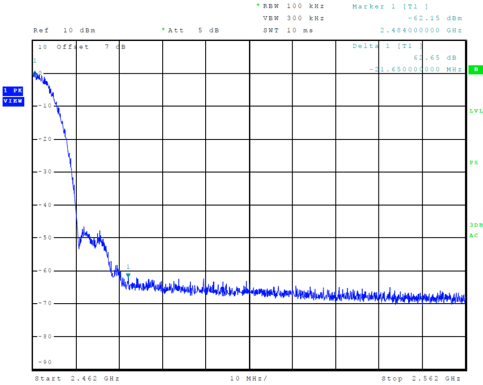
Figure 14 Plot of Upper Band Edge (802.11 b-mode)
