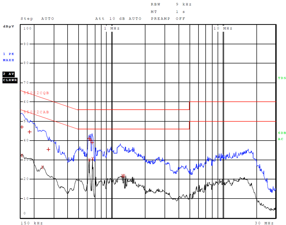
Figure 2 AC Line Conducted emissions of EUT line 2 (#2, EUT – 320-00096-xx)
