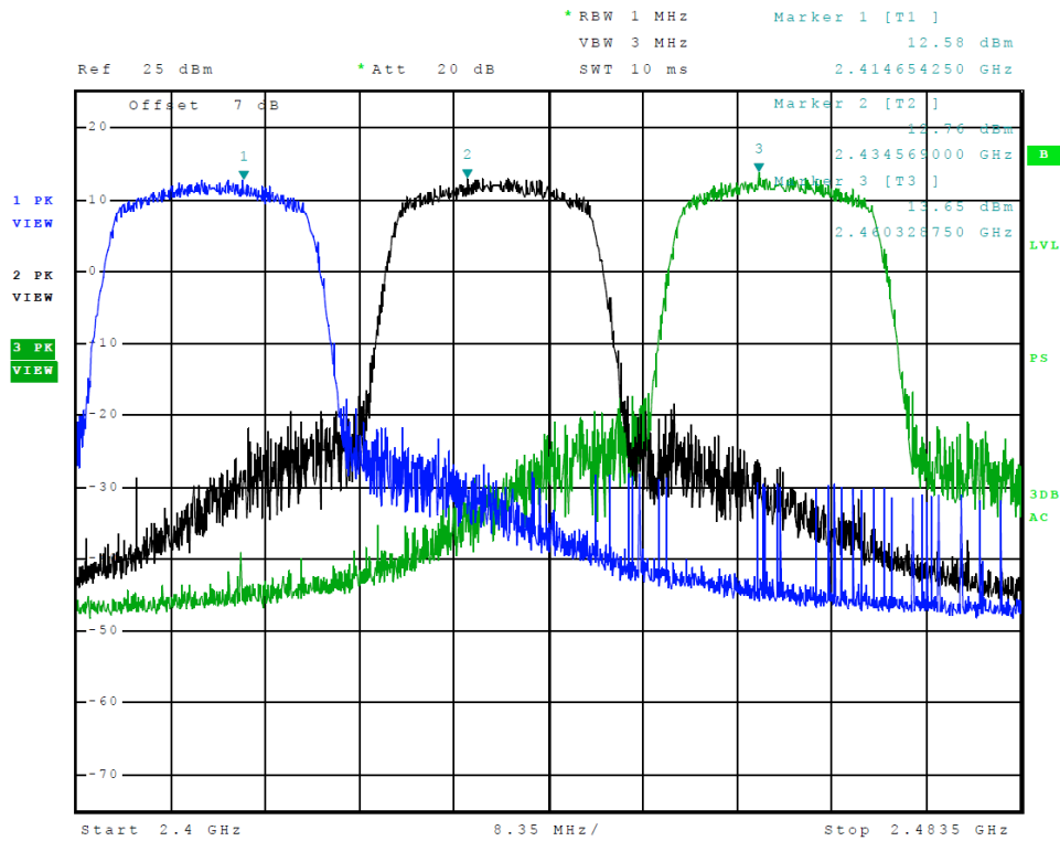
Figure 8 Plot of Transmitter Emissions in Operational Frequency (802.11 n-Mode)
