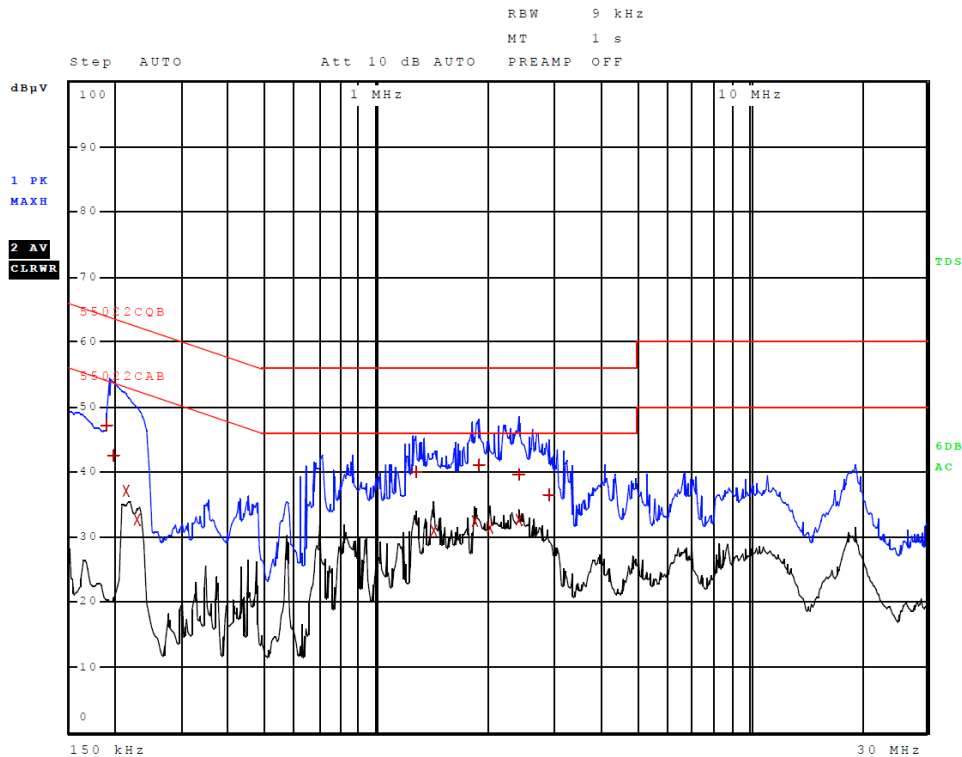
Figure 6 AC Line Conducted emissions of EUT line 2 (#4, EUT – CPU)
