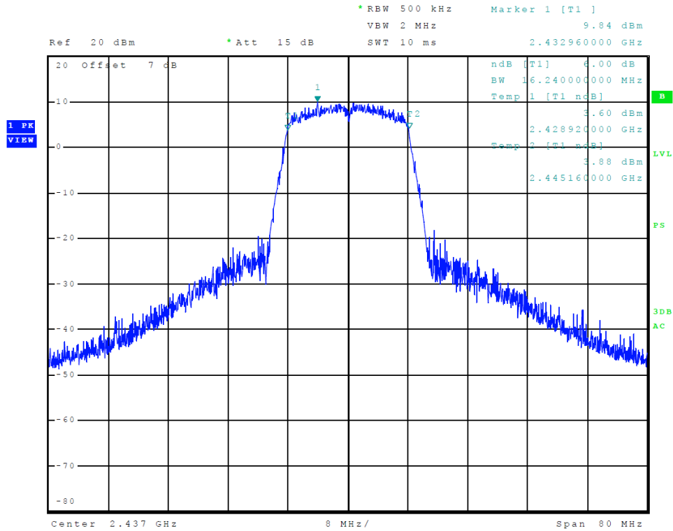
Figure 20 Plot of Transmitter 6-dB Occupied Bandwidth (802.11 g-mode)
