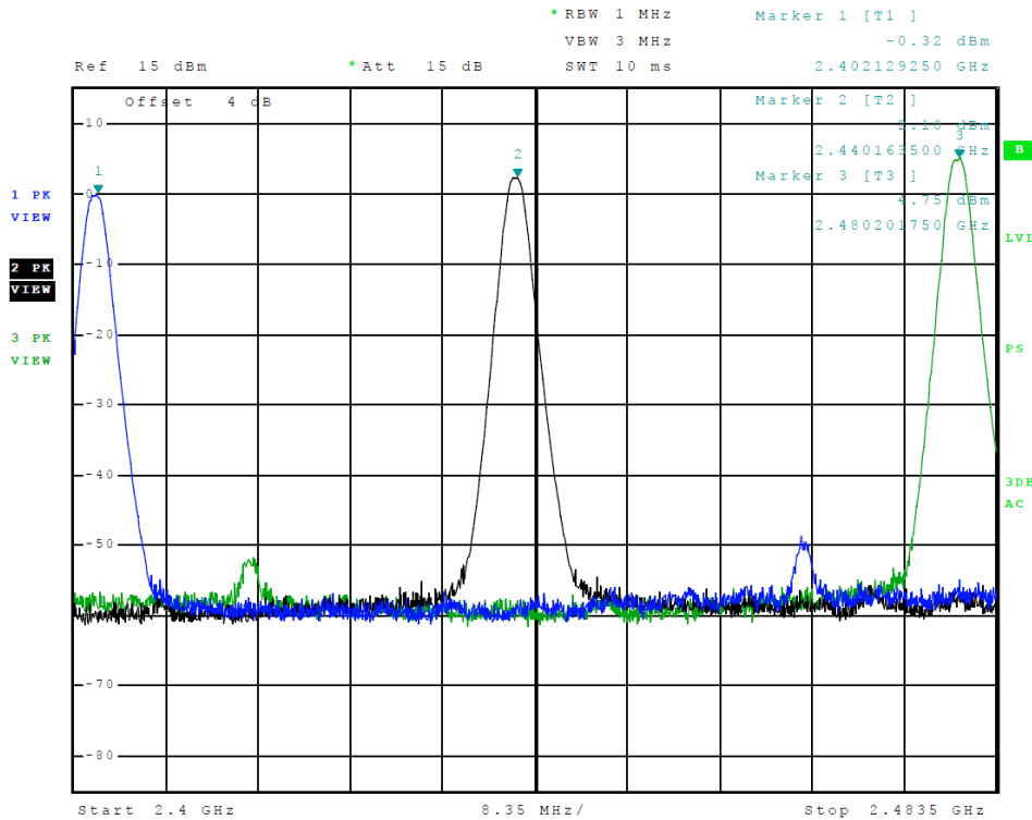
Figure 13 Plot of Transmitter Emissions (Operation in 2402-2480 MHz, BLE GMSK)
