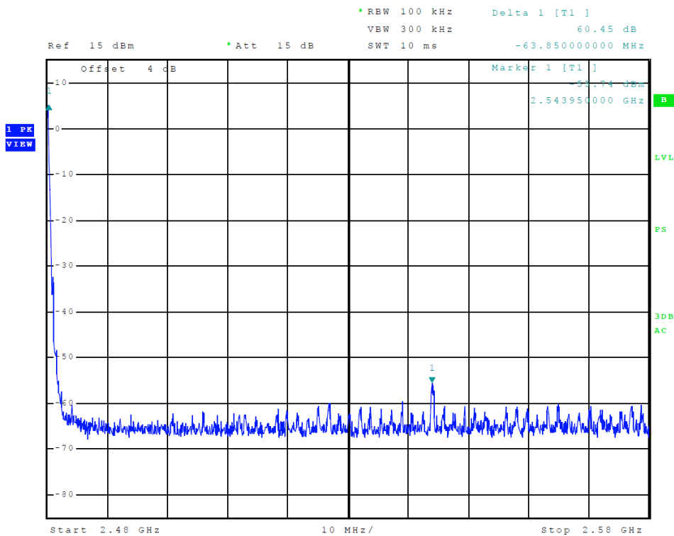
Figure 8 Plot of Transmitter Emissions (High Band Edge, ANT GFSK)
