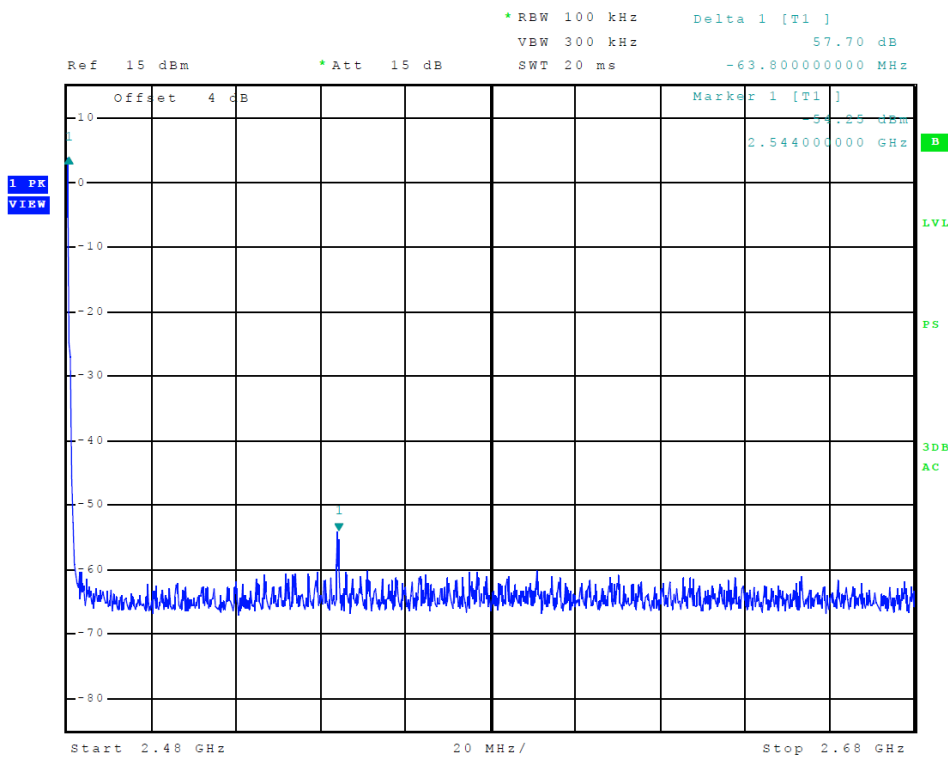
Figure 16 Plot of Transmitter Emissions (High Band Edge, BLE GMSK)
