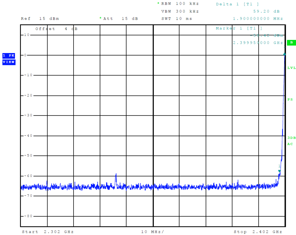
Figure 7 Plot of Transmitter Emissions (Low Band Edge, ANT GFSK)
