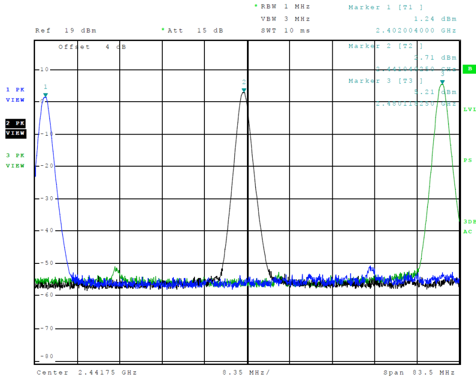
Figure 9 Plot of Transmitter Emissions (Operation in 2402-2480 MHz, BT GFSK)
