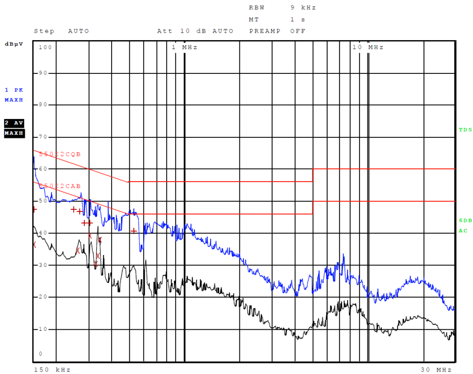
Figure 4 AC Line Conducted emissions of EUT line 2 (#3, EUT – USB – Computer)
