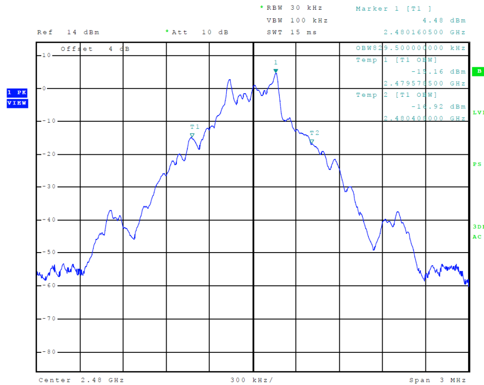
Figure 10 Plot of Transmitter Emissions (99% Occupied Bandwidth, BT GFSK)
