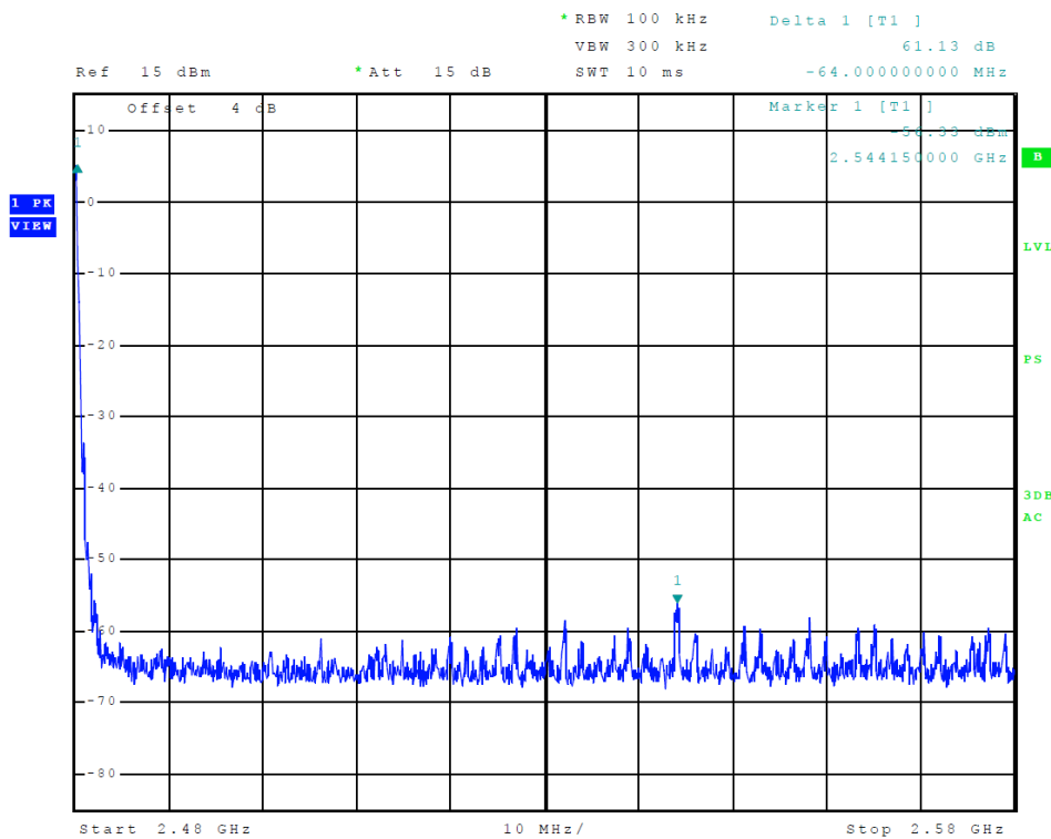
Figure 12 Plot of Transmitter Emissions (High Band Edge, BT GFSK)
