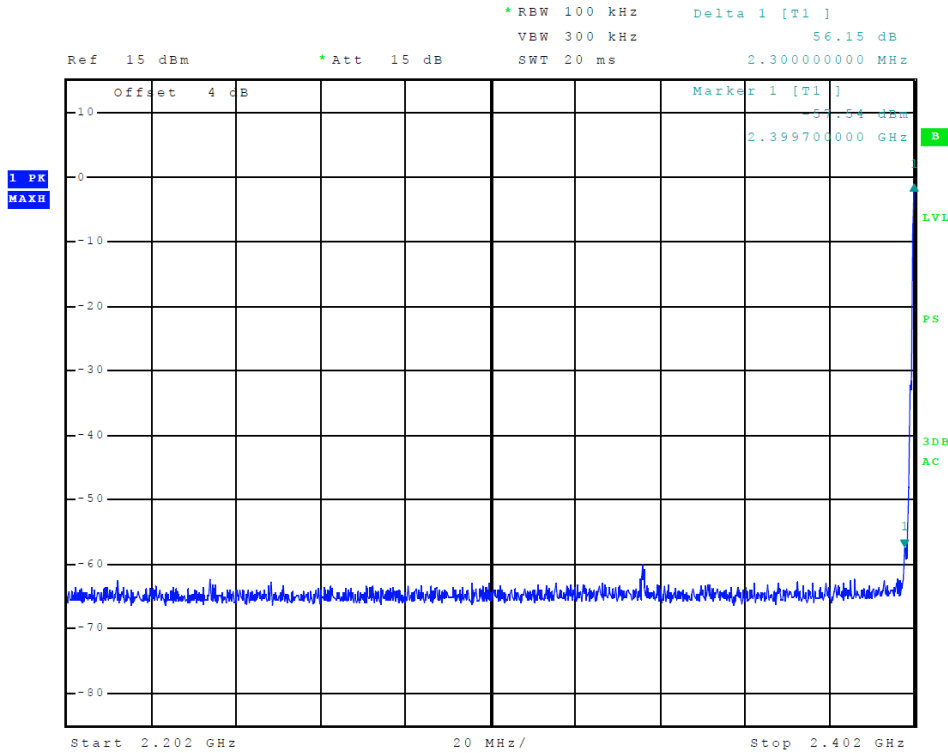
Figure 15 Plot of Transmitter Emissions (Low Band Edge, BLE GMSK)
