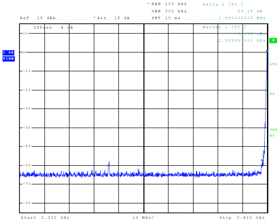
Figure 11 Plot of Transmitter Emissions (Low Band Edge, BT GFSK)
