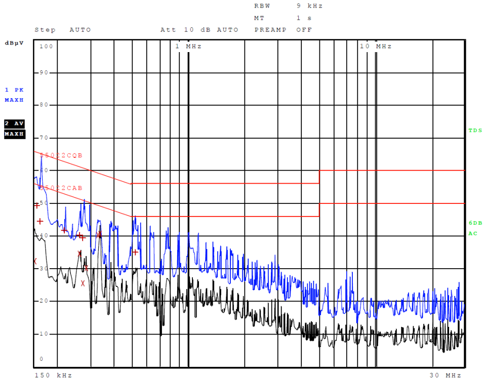
Figure 3 AC Line Conducted emissions of EUT line 1 (#3, EUT – USB – Computer)
