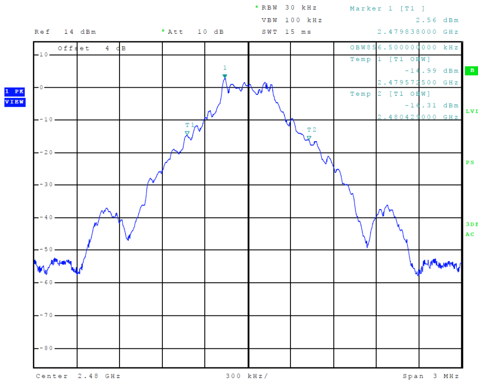
Figure 6 Plot of Transmitter Emissions (99% Occupied Bandwidth, ANT GFSK)
