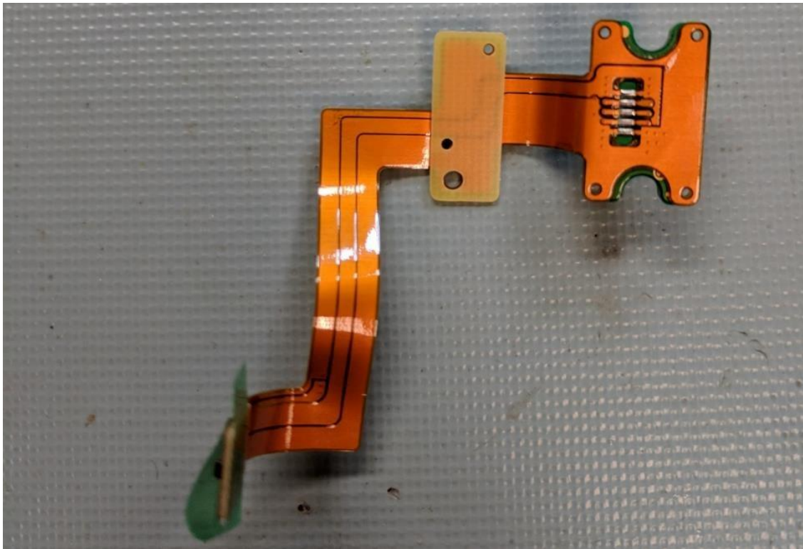
USB and Torch FPC back
