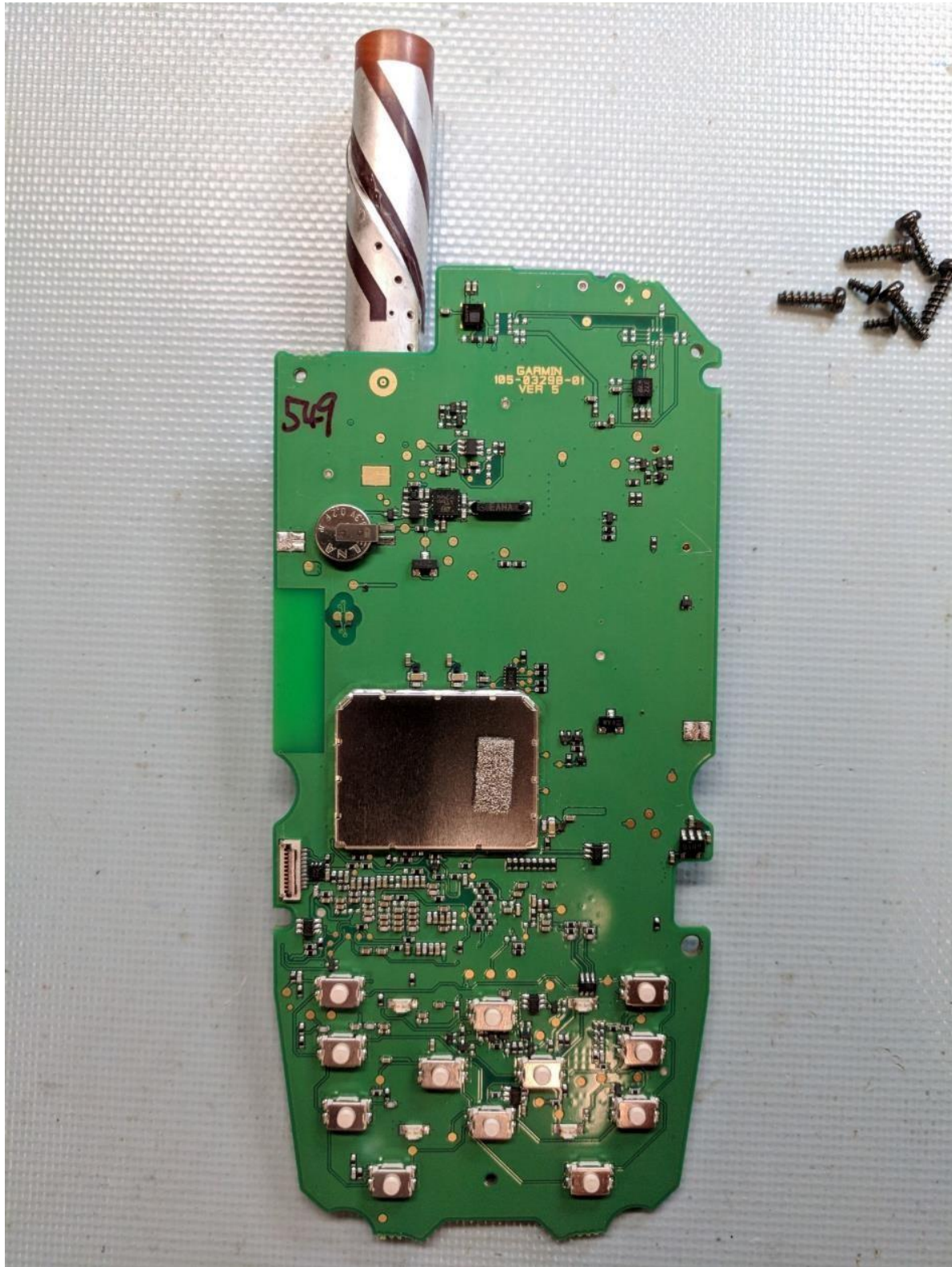
Main PCB with shield
