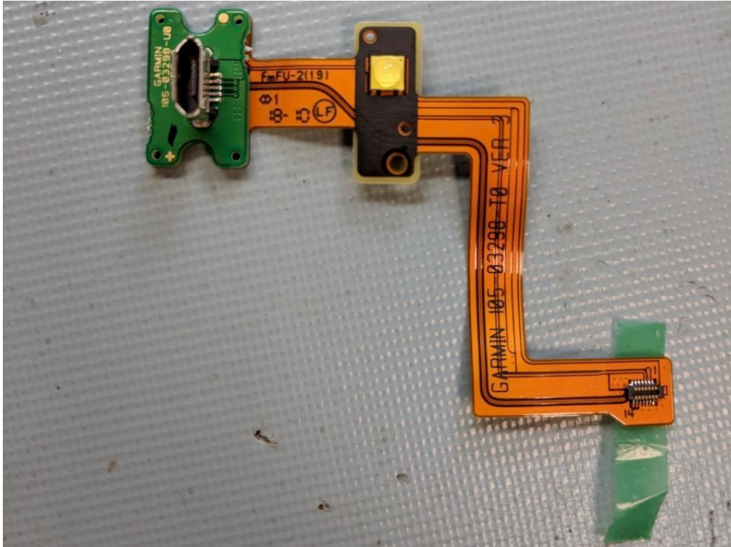
USB and Torch FPC back
