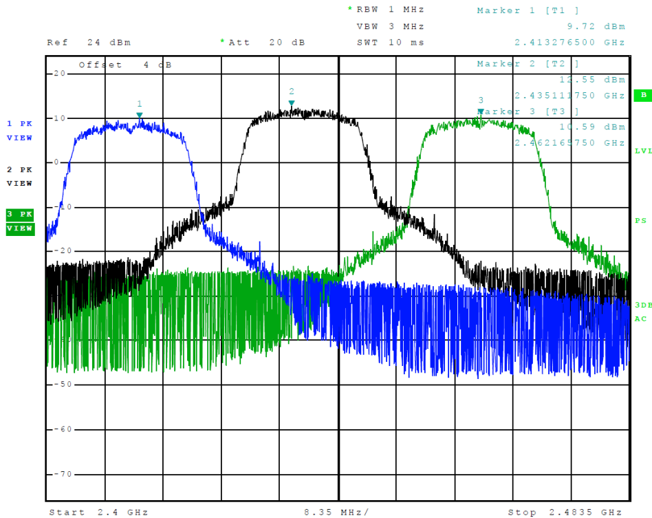
Figure 6 Plot of Transmitter Emissions in Operational Frequency (802.11 g-Mode 4)
