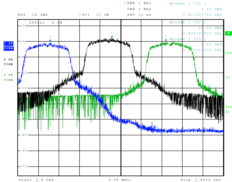
Figure 7 Plot of Transmitter Emissions in Operational Frequency (802.11 n-Mode 4)
