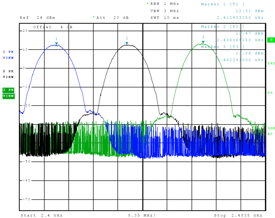
Figure 5 Plot of Transmitter Emissions in Operational Frequency (802.11 b-Mode 4)
