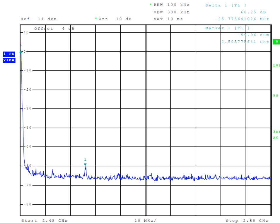
Figure 16 Plot of Transmitter Emissions High Band Edge (BLE (GMSK))
