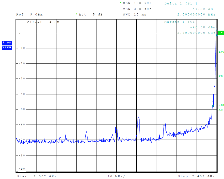
Figure 11 Plot of Transmitter Emissions Low Band Edge (3EDR (8DPSK))
