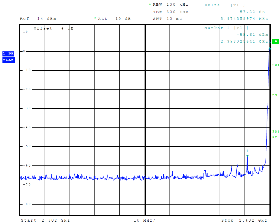
Figure 12 Plot of Transmitter Emissions Low Band Edge (BLE (GMSK))
