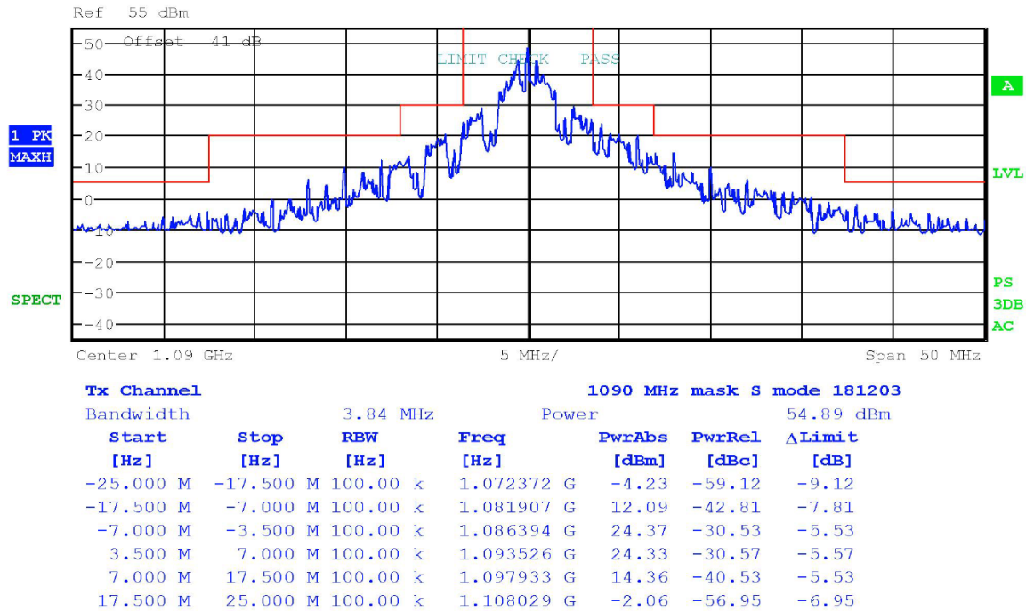
Figure 9 Emissions Mask (Mode-S)
