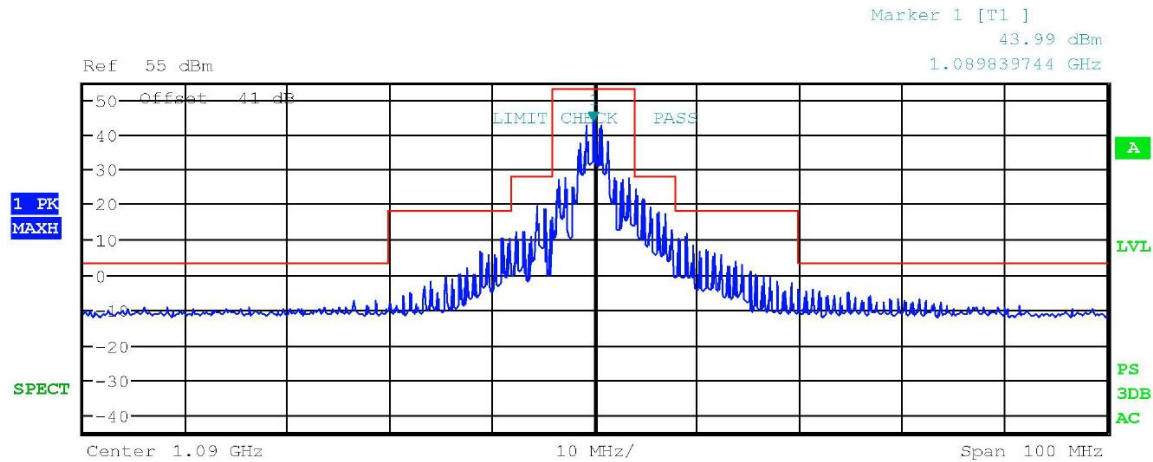
Figure 7 Spurious Emissions at Antenna Terminal
