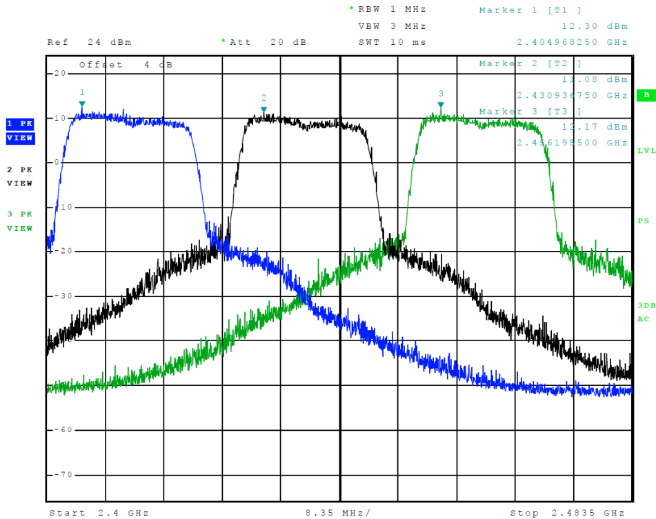
Figure 9 Plot of Transmitter Emissions in Operational Frequency (802.11 n-Mode)
