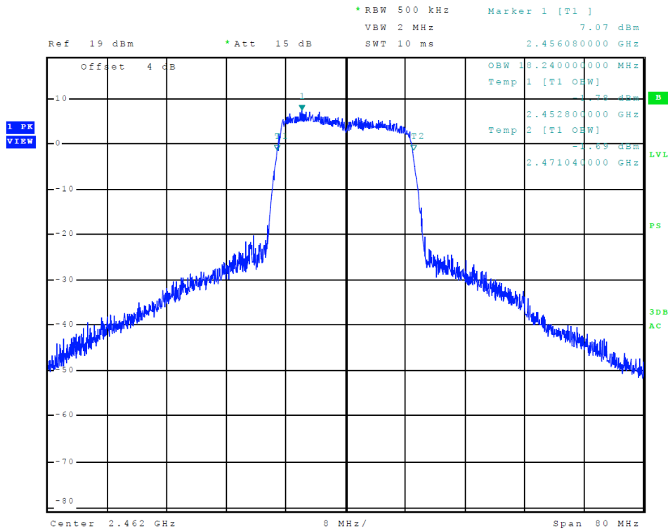
Figure 21 Plot of Transmitter 99% Occupied Bandwidth (802.11 n-mode)
