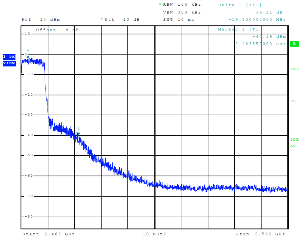
Figure 15 Plot of Upper Band Edge (802.11 n-mode)
