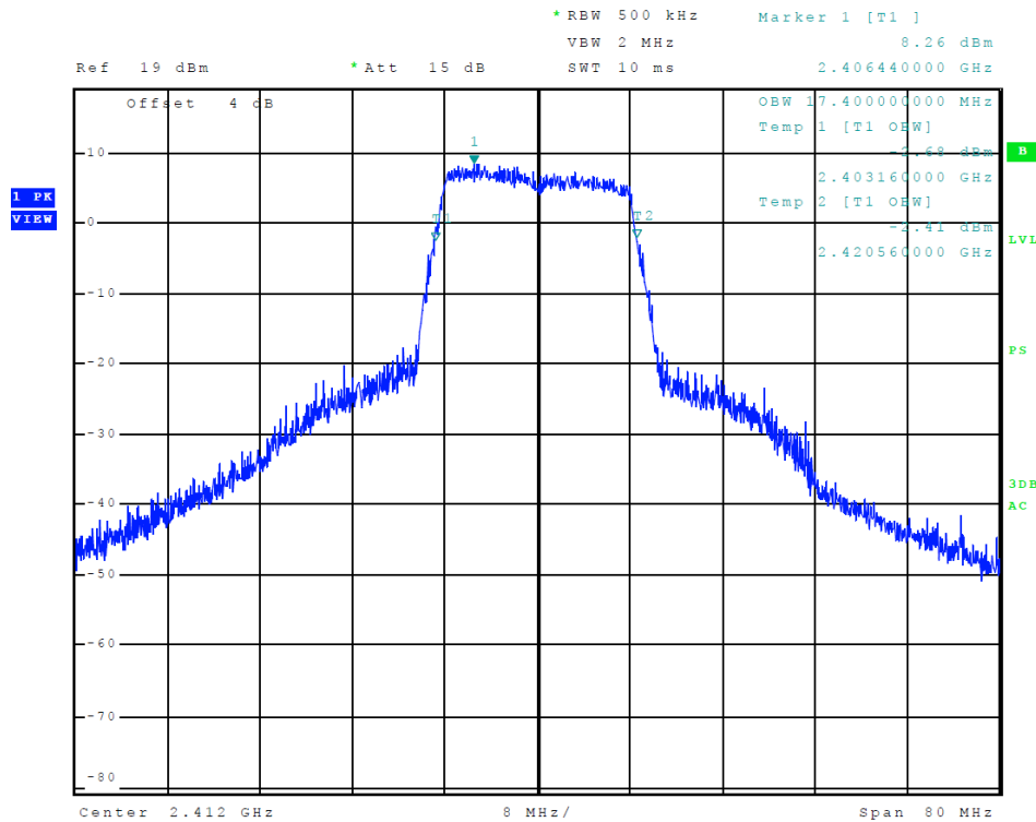
Figure 19 Plot of Transmitter 99% Occupied Bandwidth (802.11 g-mode)
