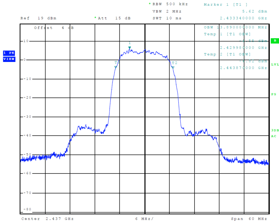
Figure 17 Plot of Transmitter 99% Occupied Bandwidth (802.11 b-mode)
