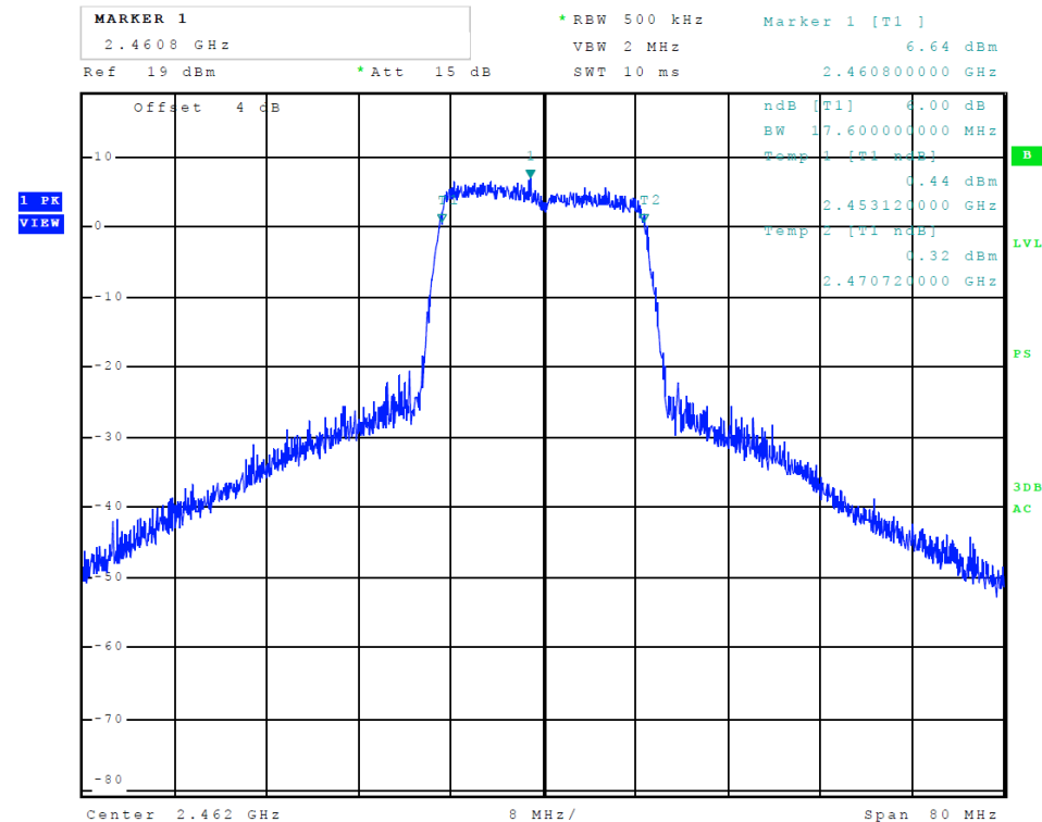
Figure 20 Plot of Transmitter 6-dB Occupied Bandwidth (802.11 n-mode)
