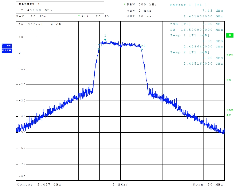
Figure 18 Plot of Transmitter 6-dB Occupied Bandwidth (802.11 g-mode)
