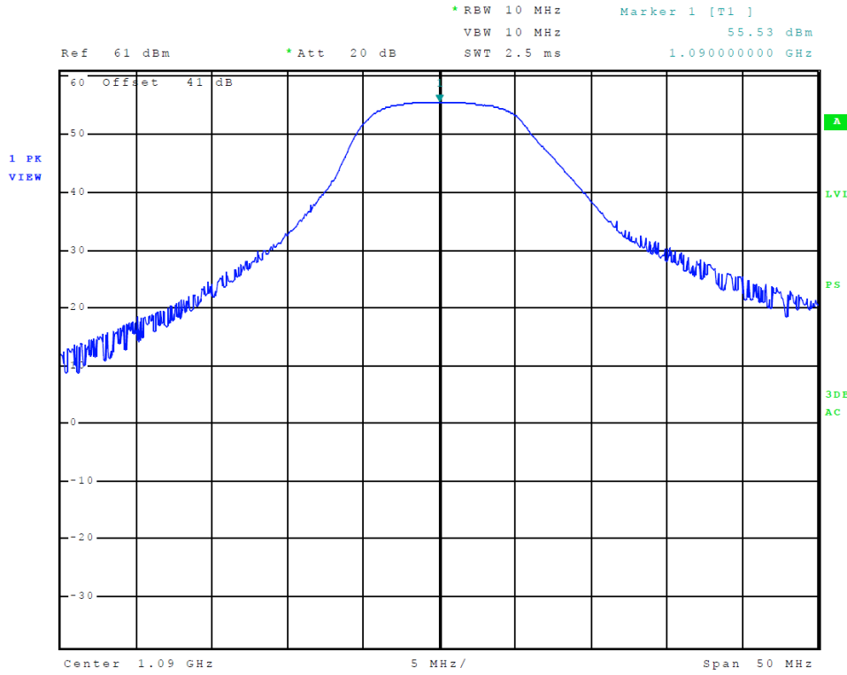
Figure 1 Maximum Power Output Mode-A
