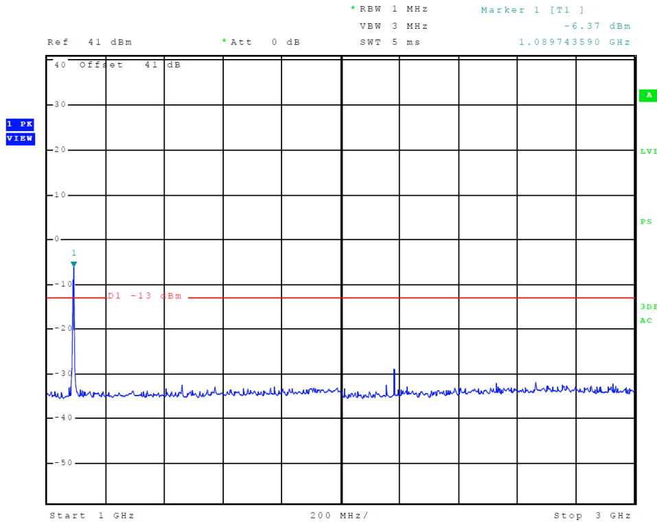
Figure 6 Spurious Emissions at Antenna Terminal (A-Mode)
