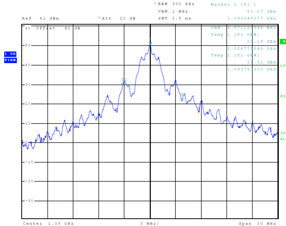
Figure 4 Occupied Band Width Mode S
