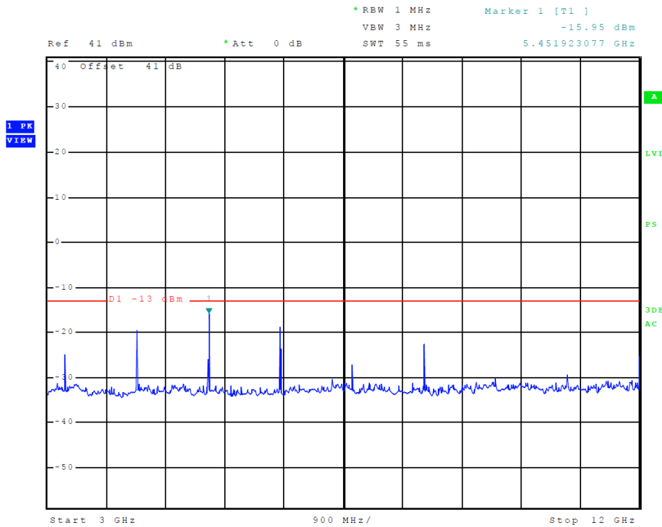
Figure 7 Spurious Emissions at Antenna Terminal (A-Mode)
