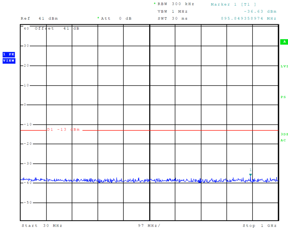
Figure 5 Spurious Emissions at Antenna Terminal (A-Mode)
