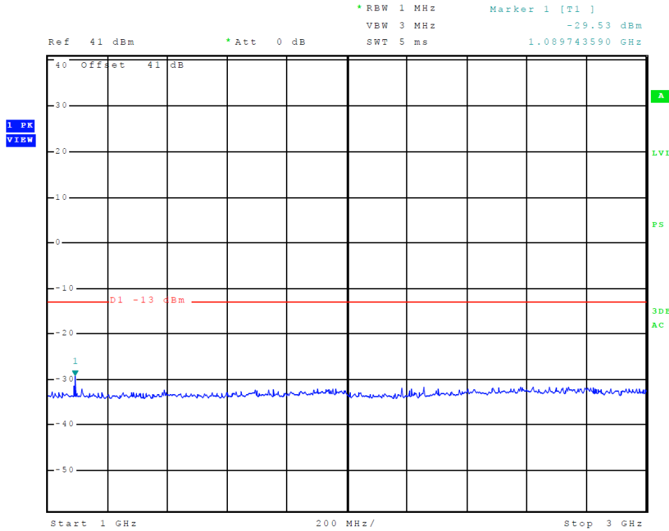
Figure 9 Spurious Emissions at Antenna Terminal (S-Mode)
