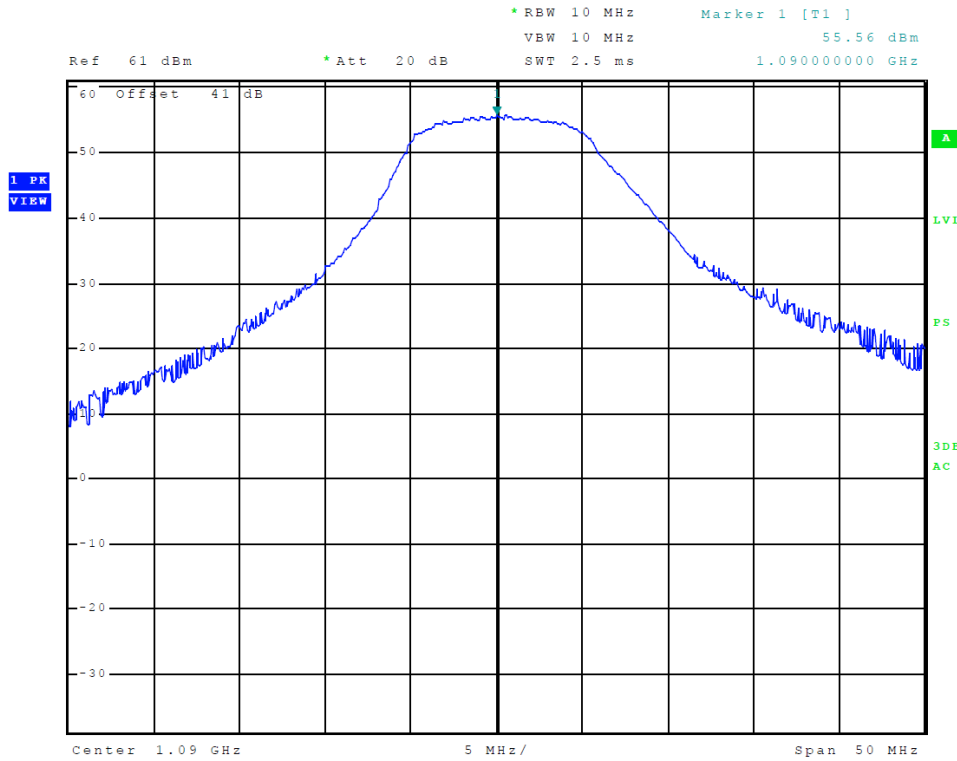
Figure 2 Maximum Power Output mode-S
