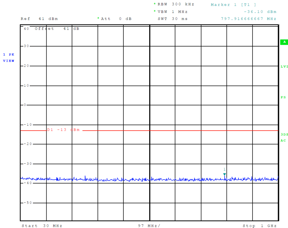
Figure 8 Spurious Emissions at Antenna Terminal (S-Mode)
