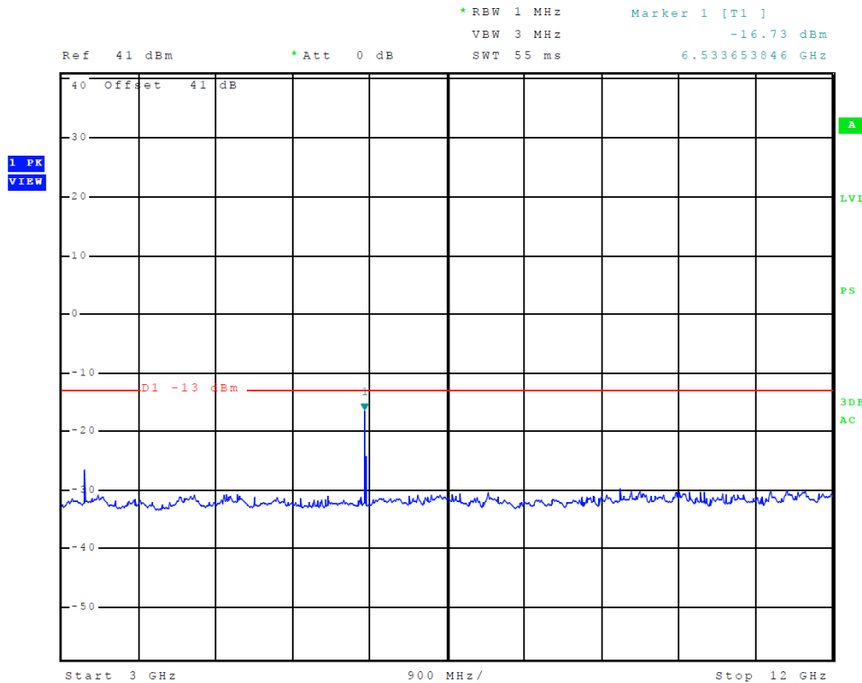
Figure 10 Spurious Emissions at Antenna Terminal (S-Mode)
