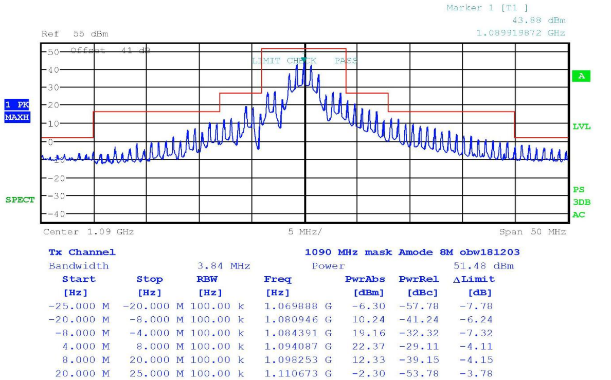
Figure 11 Emissions Mask (Mode-A)
