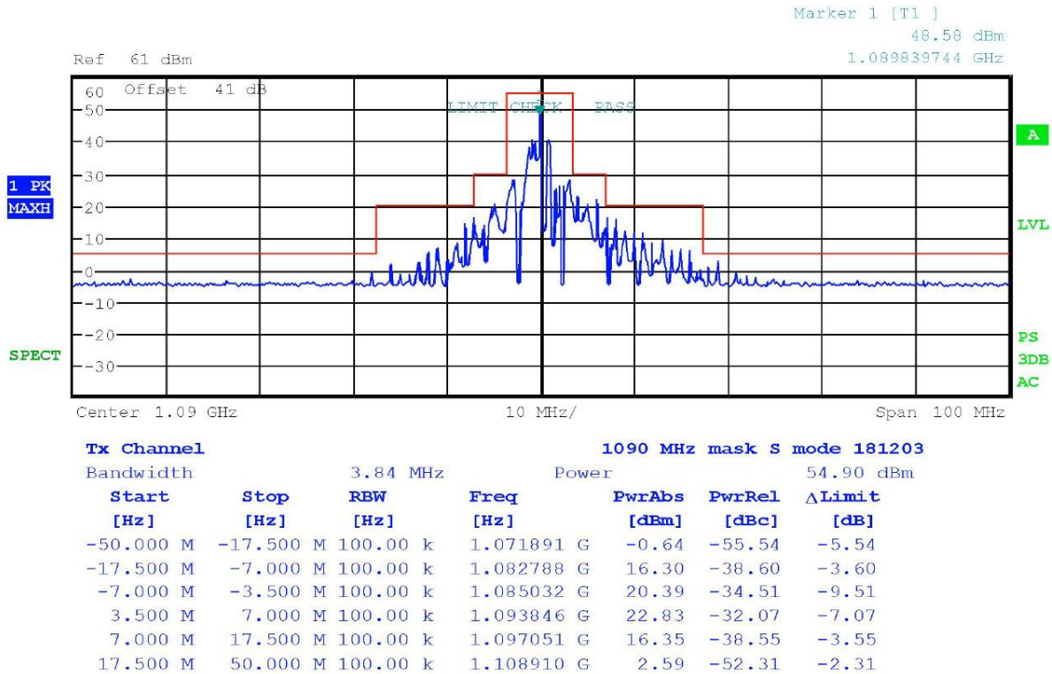
Figure 12 Emissions Mask (Mode-S)
