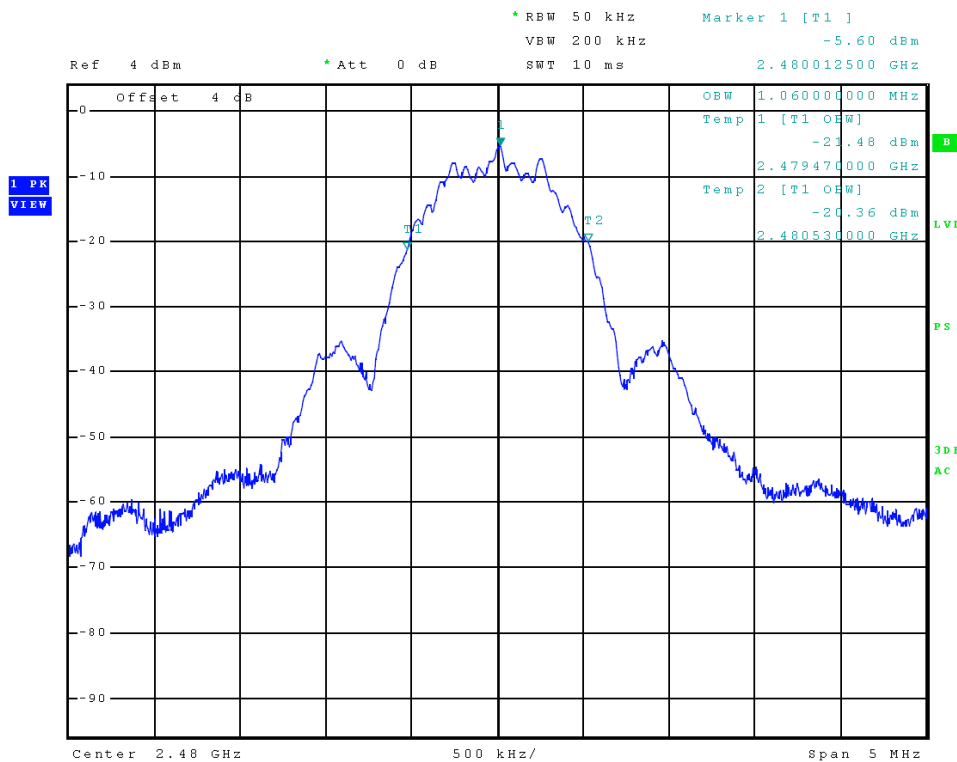
Figure 6 Plot of Transmitter Emissions (99% Occupied Bandwidth, BLE)
