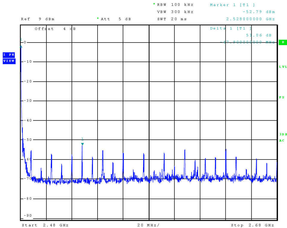
Figure 4 Plot of Transmitter Emissions (High Band Edge, ANT)
