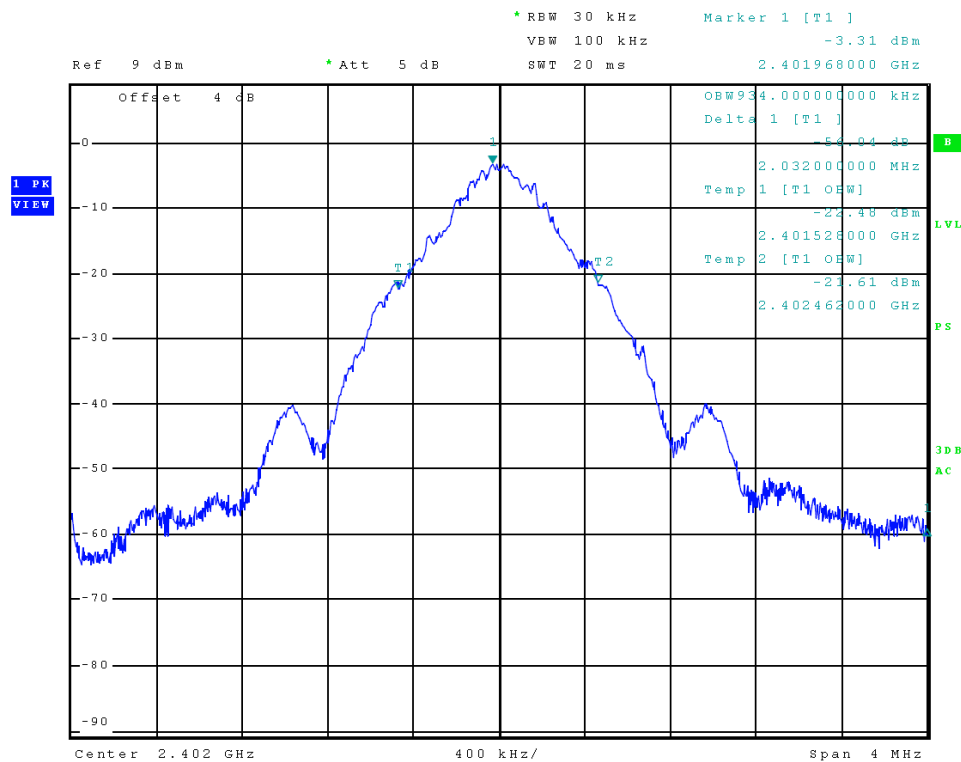
Figure 2 Plot of Transmitter Emissions (99% Occupied Bandwidth, ANT)
