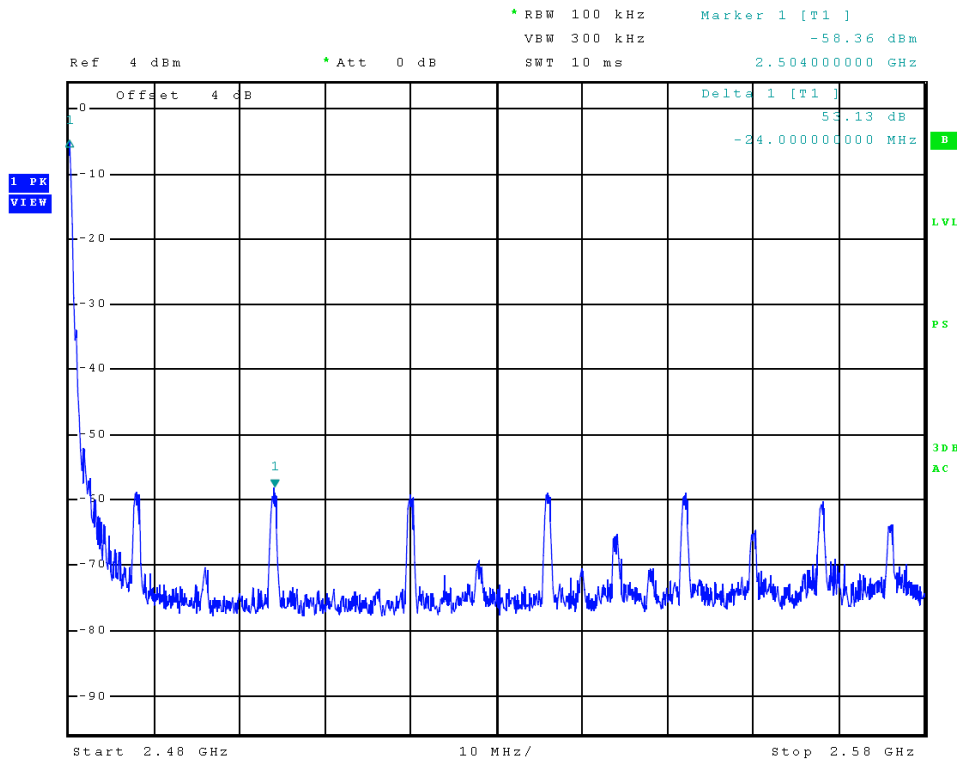
Figure 8 Plot of Transmitter Emissions (High Band Edge, BLE)
