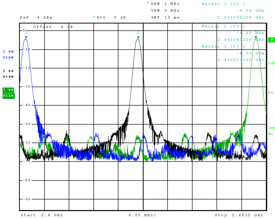
Figure 5 Plot of Transmitter Emissions (Operation in 2402-2480 MHz, BLE)
