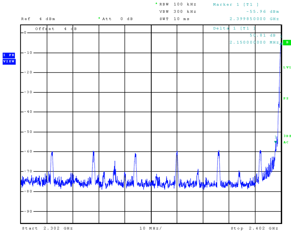
Figure 7 Plot of Transmitter Emissions (Low Band Edge, BLE)
