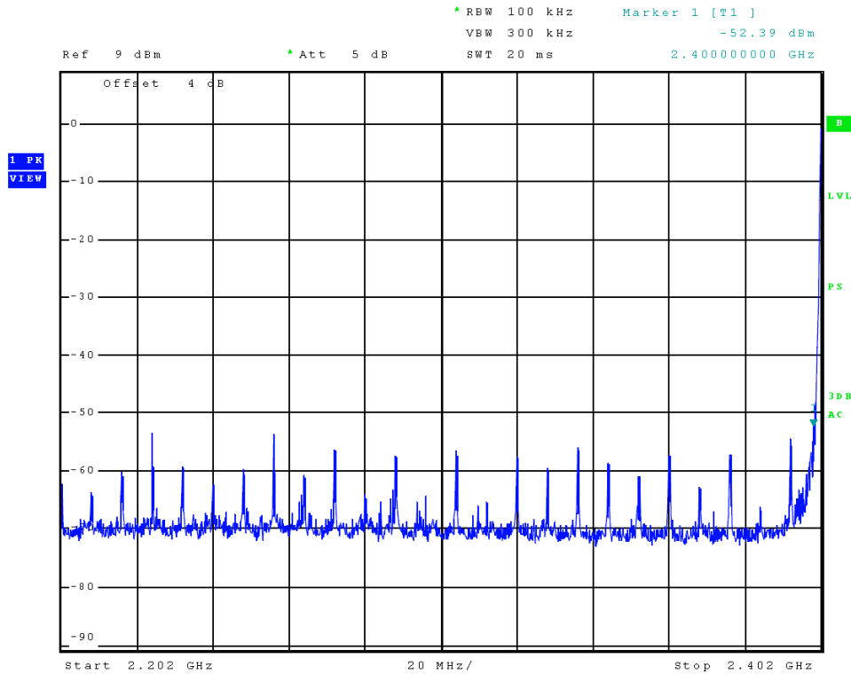
Figure 3 Plot of Transmitter Emissions (Low Band Edge, ANT)
