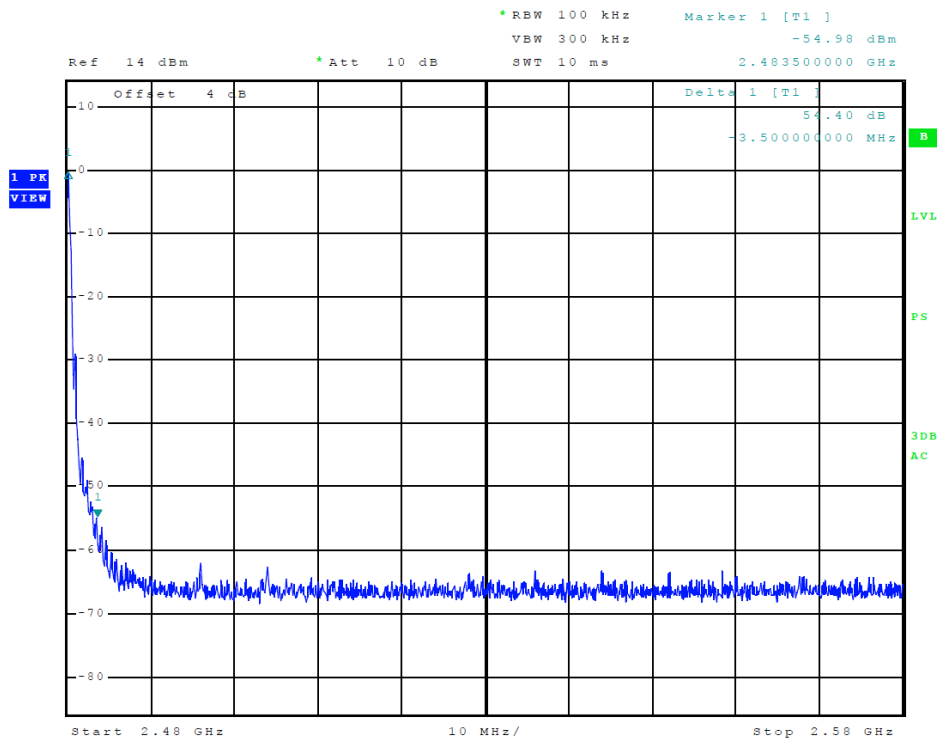
Figure 14 Plot of Transmitter Emissions (High Band Edge, BLE)
