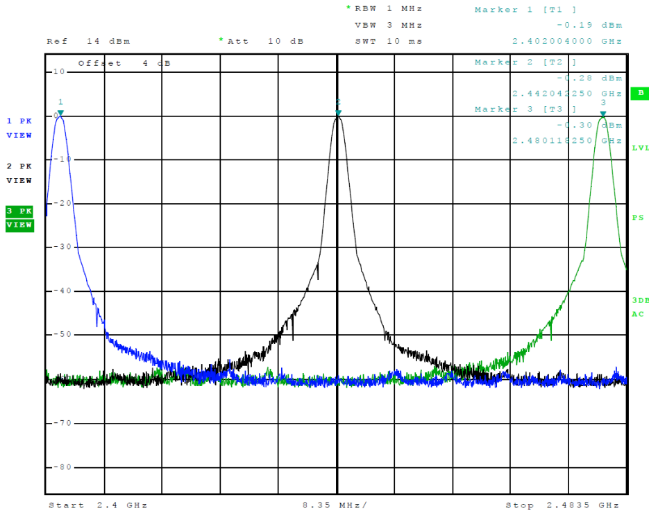
Figure 11 Plot of Transmitter Emissions (Operation in 2402-2480 MHz, BLE)
