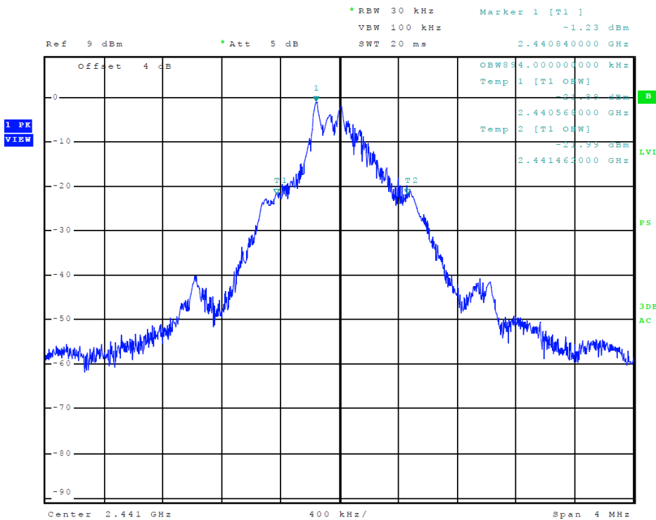
Figure 8 Plot of Transmitter Emissions (99% Occupied Bandwidth, ANT)
