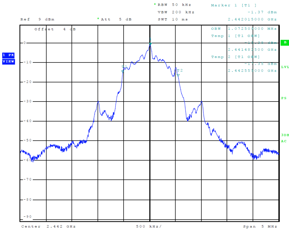
Figure 12 Plot of Transmitter Emissions (99% Occupied Bandwidth, BLE)
