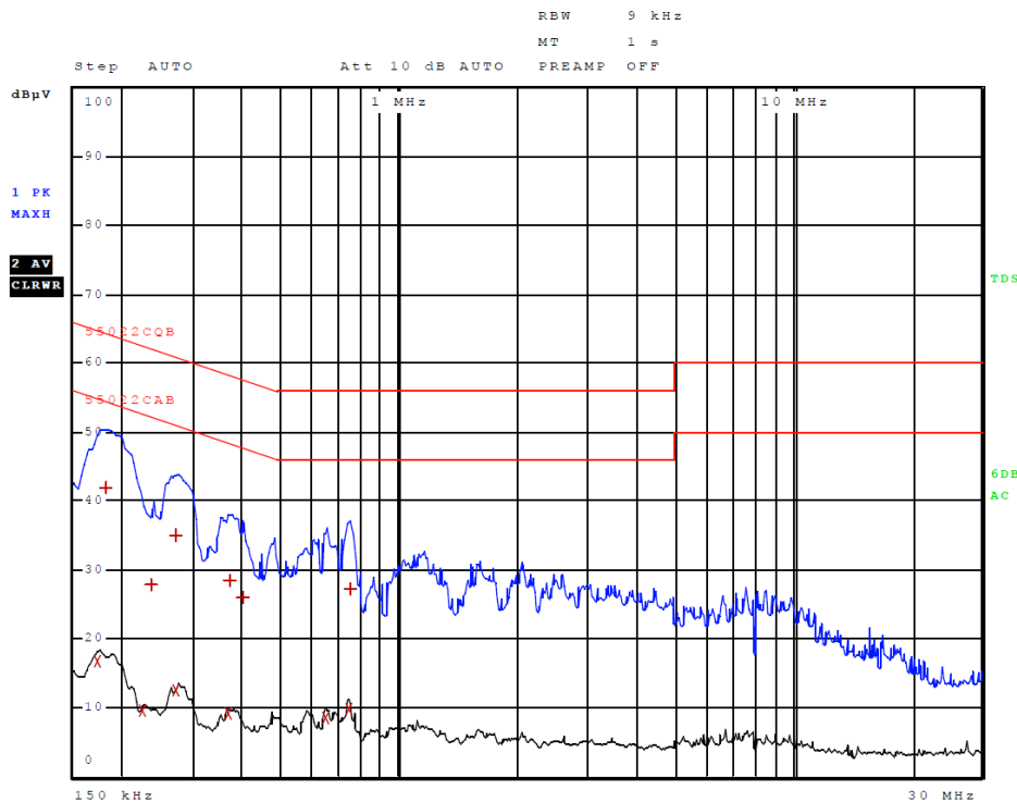
Figure 6 AC Line Conducted emissions of EUT line 2 (#4, EUT - AC Adapter)
