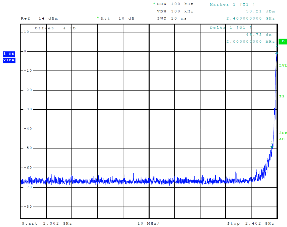
Figure 13 Plot of Transmitter Emissions (Low Band Edge, BLE)
