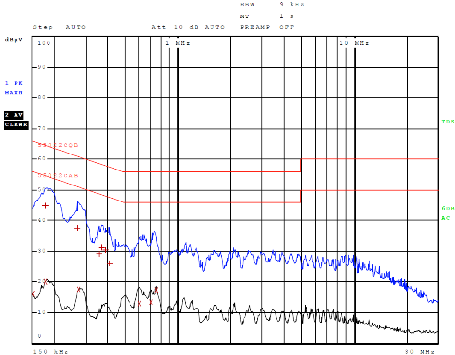
Figure 5 AC Line Conducted emissions of EUT line 1 (#4, EUT - AC Adapter)
