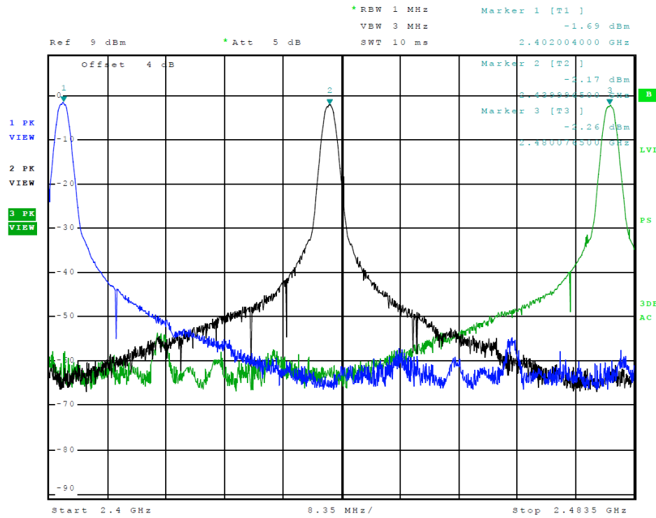
Figure 11 Plot of Transmitter Emissions (Operation in 2402-2480 MHz, BT)
