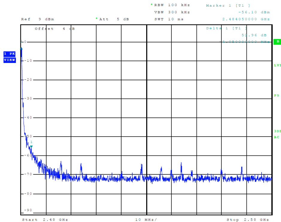
Figure 14 Plot of Transmitter Emissions (High Band Edge, BT)
