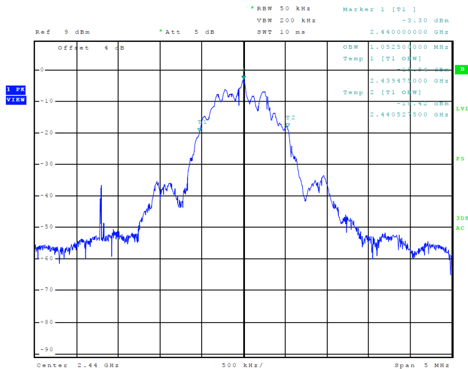
Figure 12 Plot of Transmitter Emissions (99% Occupied Bandwidth, BT)
