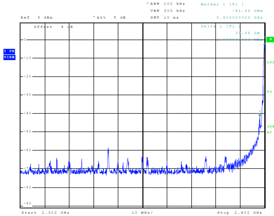
Figure 13 Plot of Transmitter Emissions (Low Band Edge, BT)
